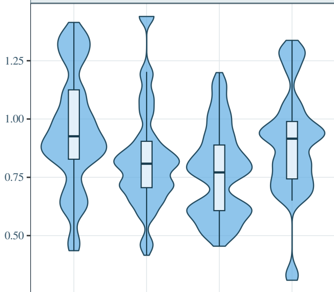
Steepness quartile
