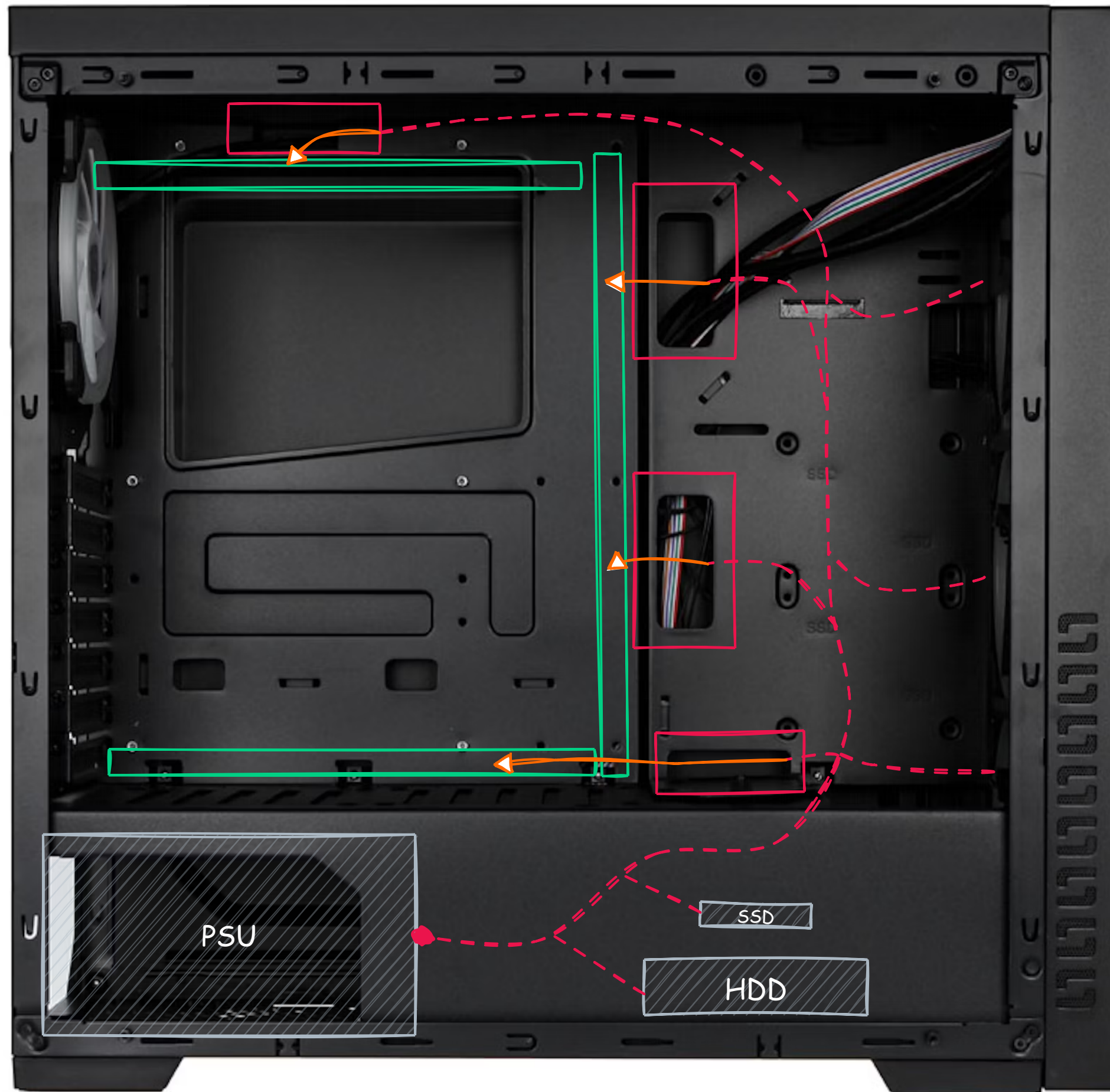
Left Side View (The side you can see into if the case has a glass/mesh side)
