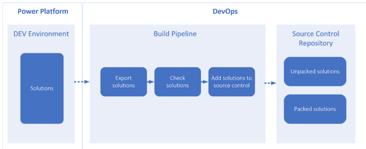
Figure 14.5 - Azure DevOps pipeline for automated Power Platform solution source control
