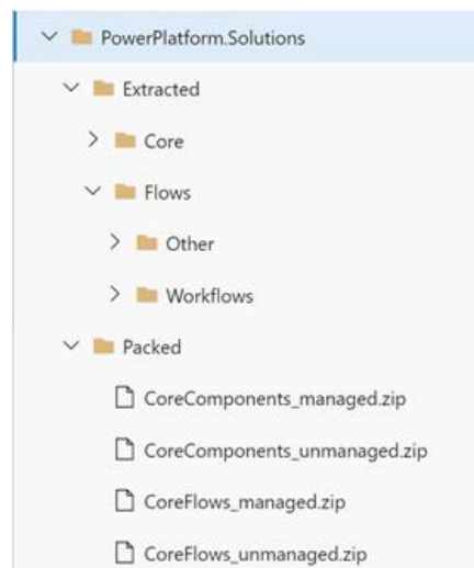
Figure 14.4 - Storing Power Platform solutions in source control
