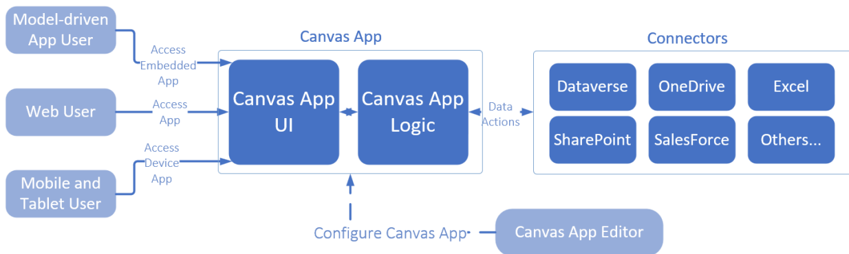
Figure 1.10 - Canvas Apps Architectural Overview
