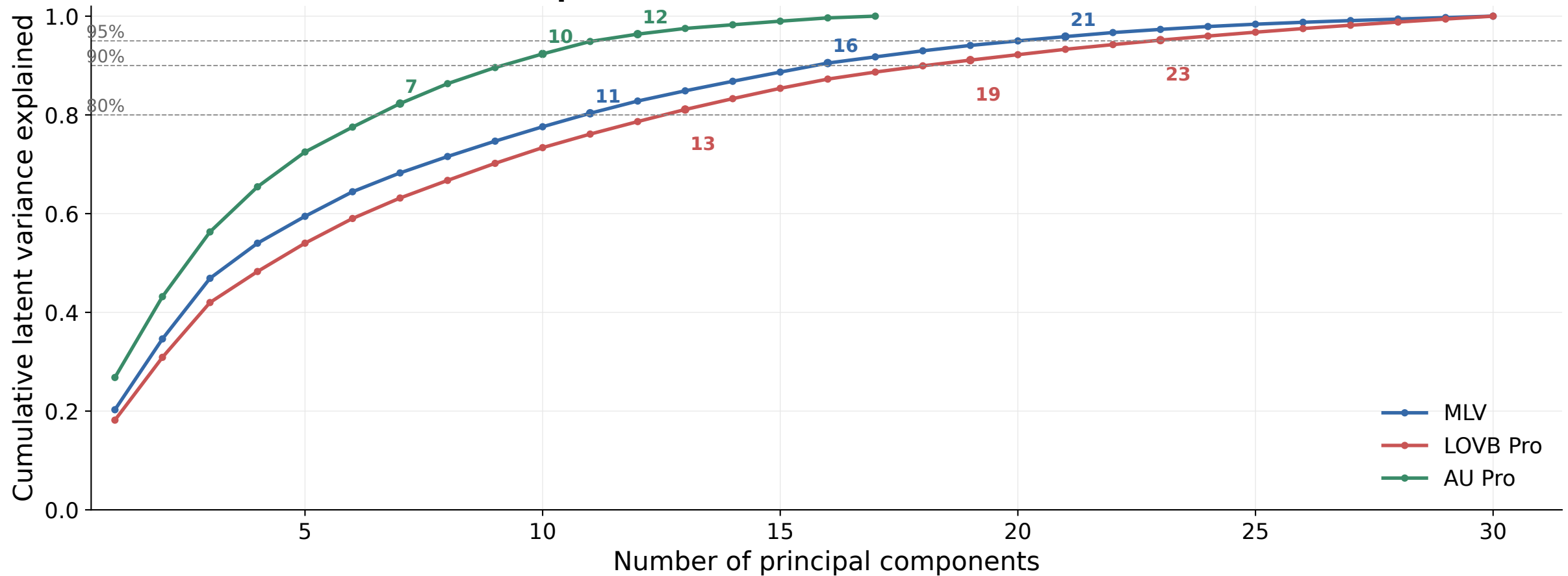
PCA of posterior-mean latent metric correlations
