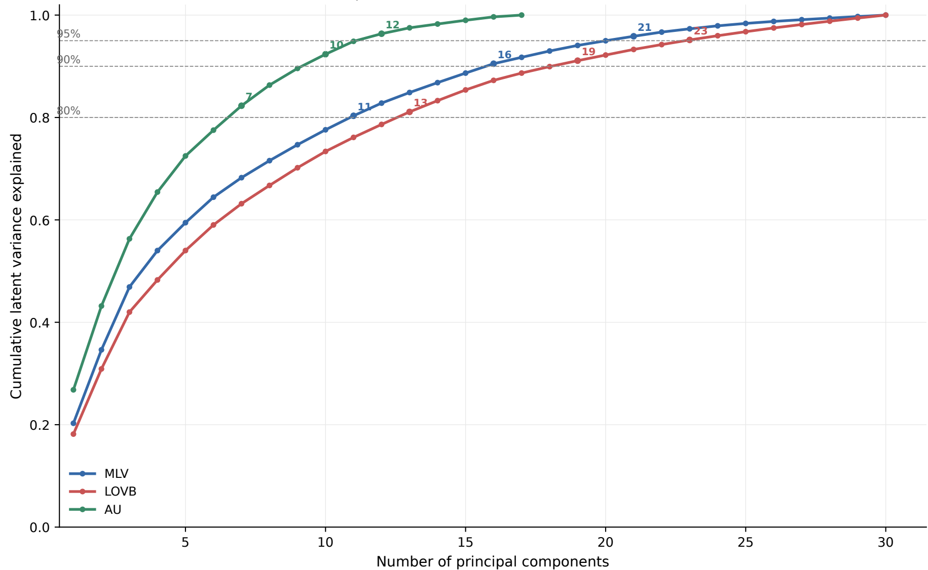
PCA of posterior-mean latent metric correlations
