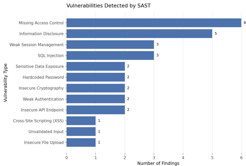
Figure 3: Frequency of each vulnerability category detected.
