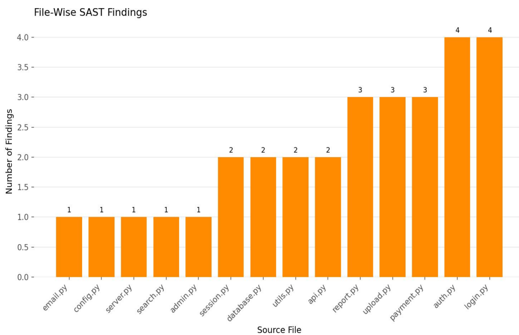
Figure 2: Number of findings per source file.
