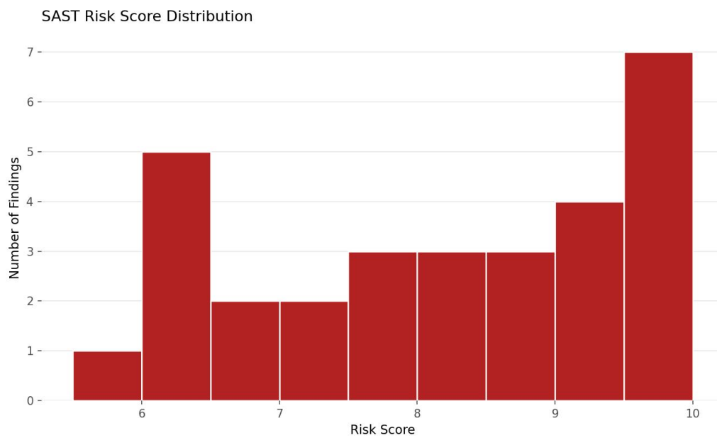
Figure 1: Distribution of risk scores across all SAST findings.
