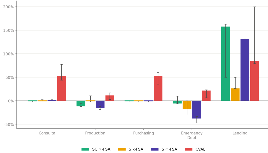
(b) 2-Gram differences between the baseline methods and our k -FSA-based method. Negative values indicate a decrease in entropy for the baseline methods, which is considered beneficial.
