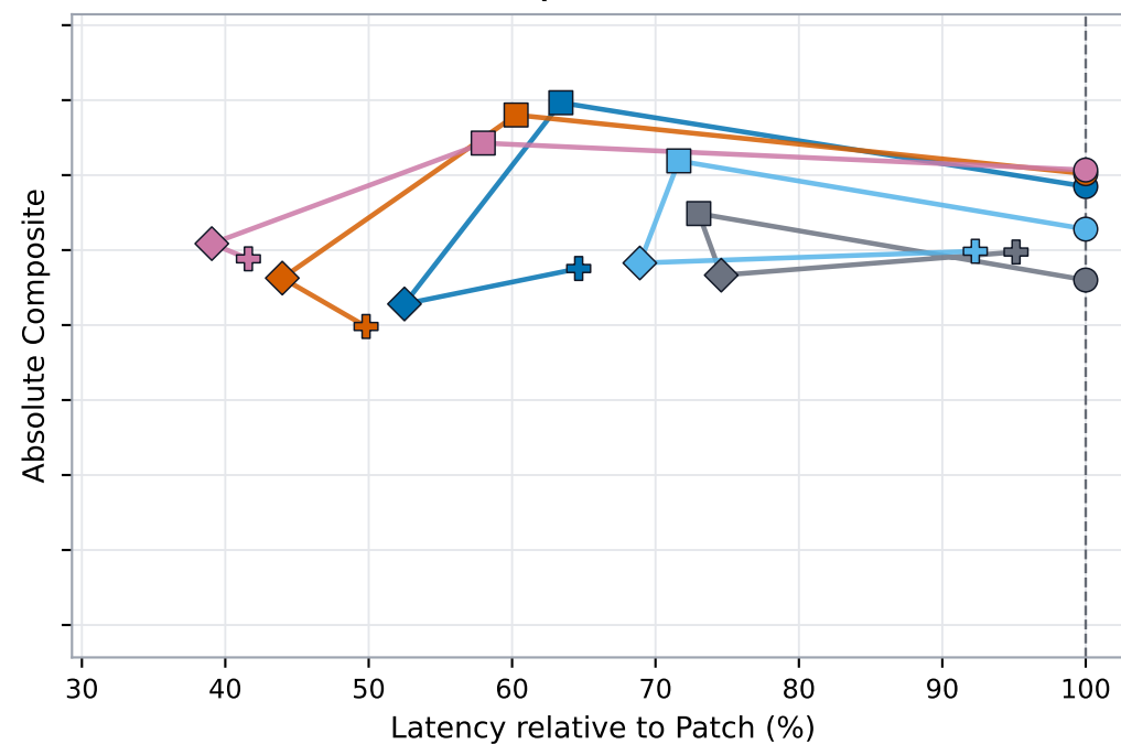
Qwen 2B
