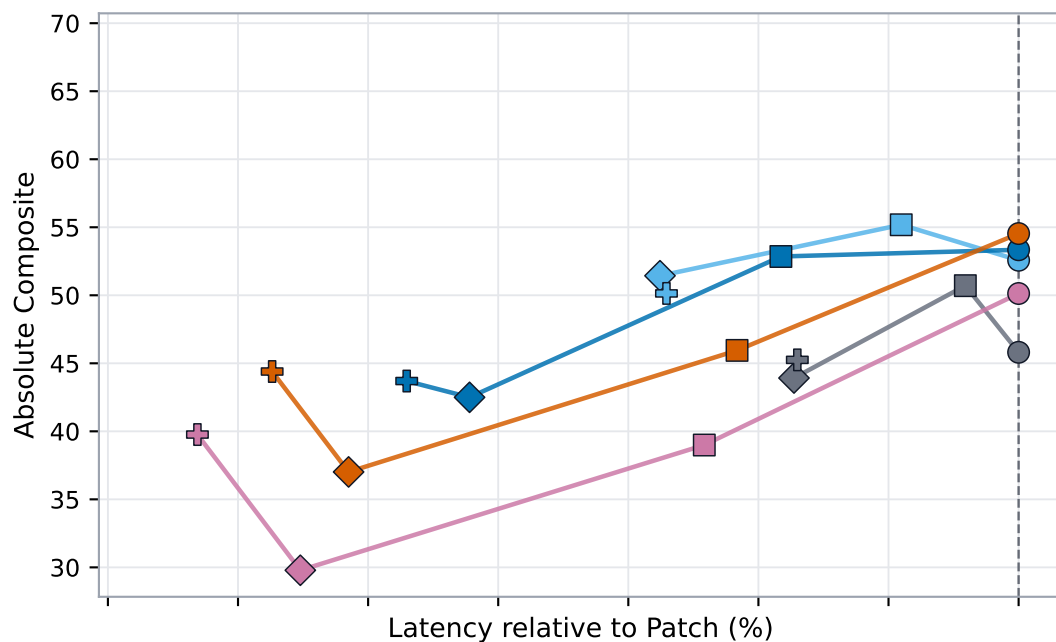
Granite 350M
