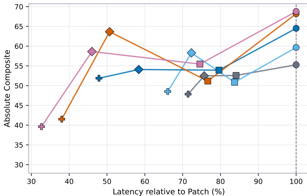
Granite 1B
