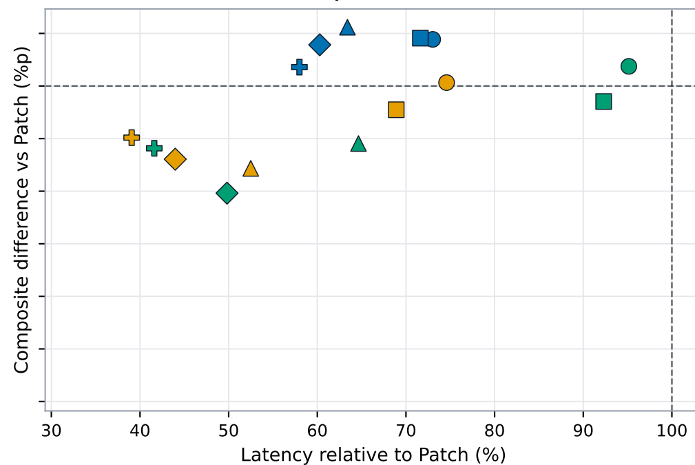
Qwen 2B
