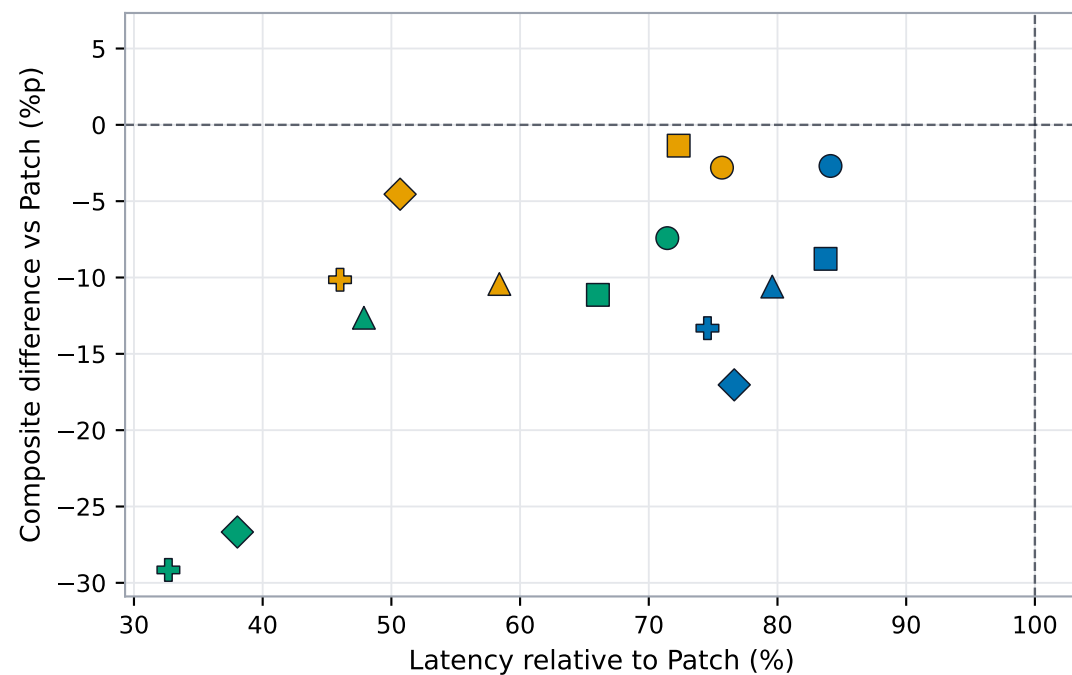
Granite 1B
