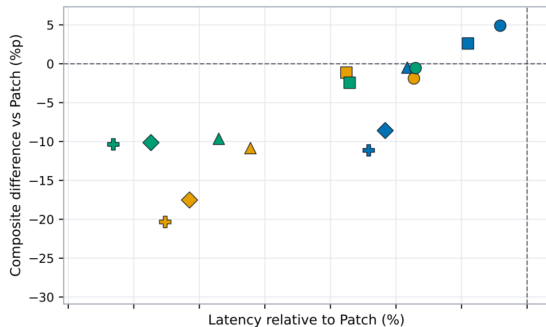
Granite 350M
