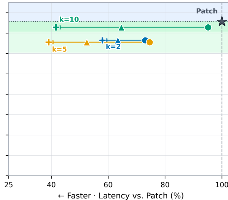
Qwen 2B
