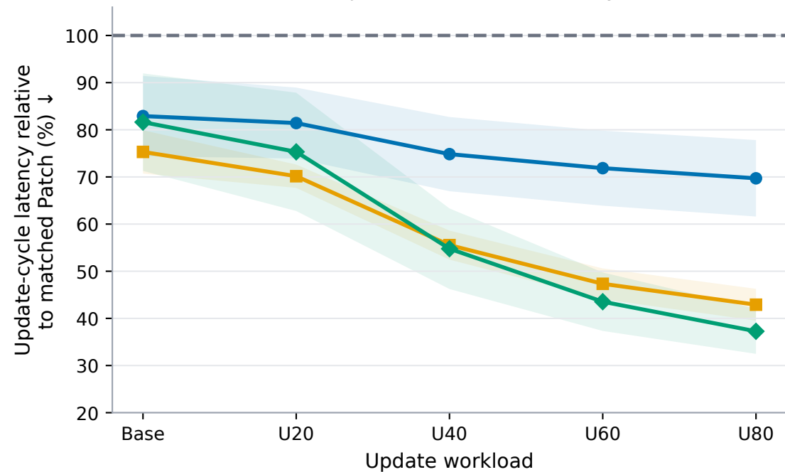
(a) Projected on-device latency
