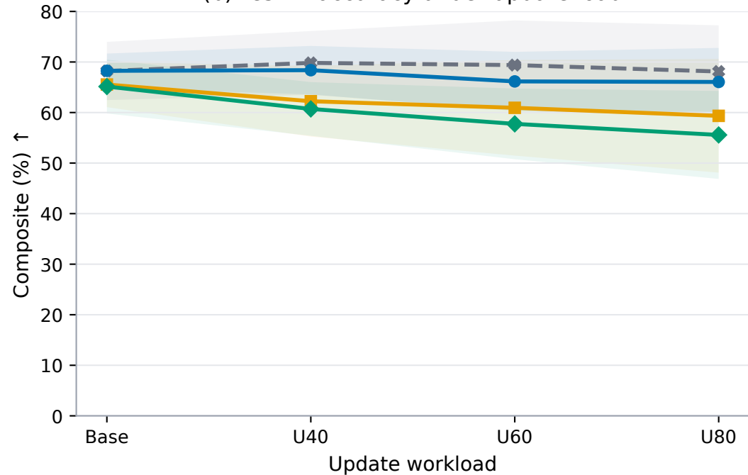
(b) Test24 accuracy under update load
