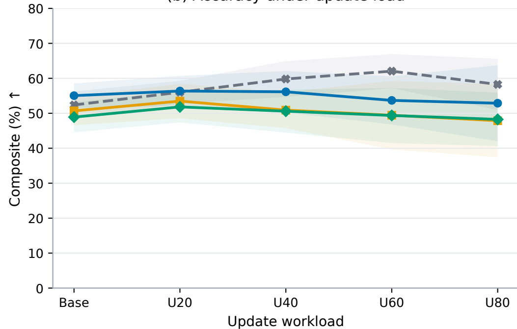
(b) Accuracy under update load
