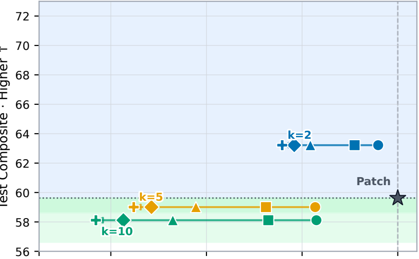
Granite 350M
