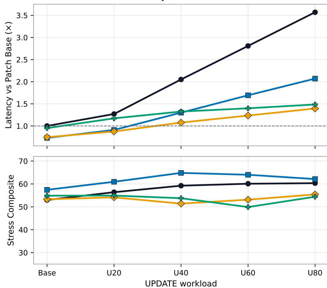
Qwen 2B
