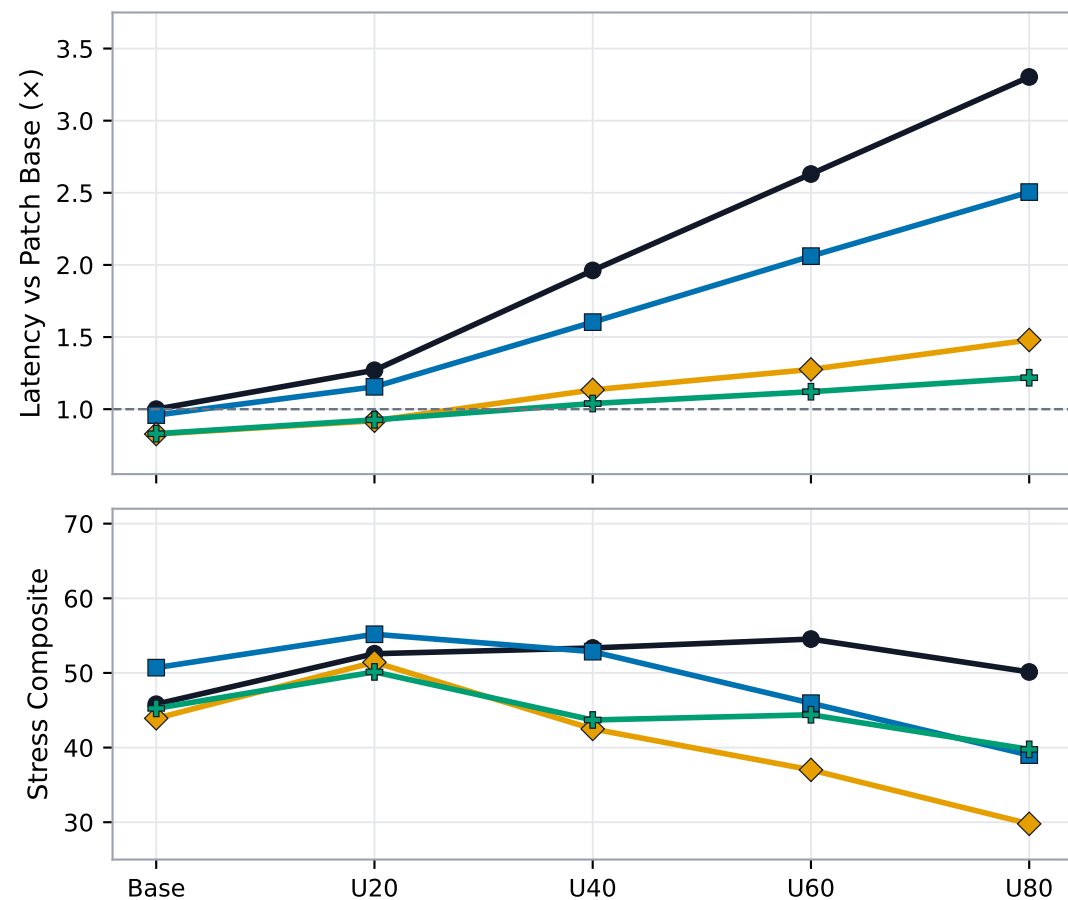
Granite 350M
