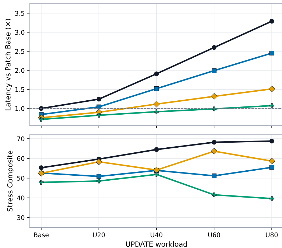
Granite 1B
