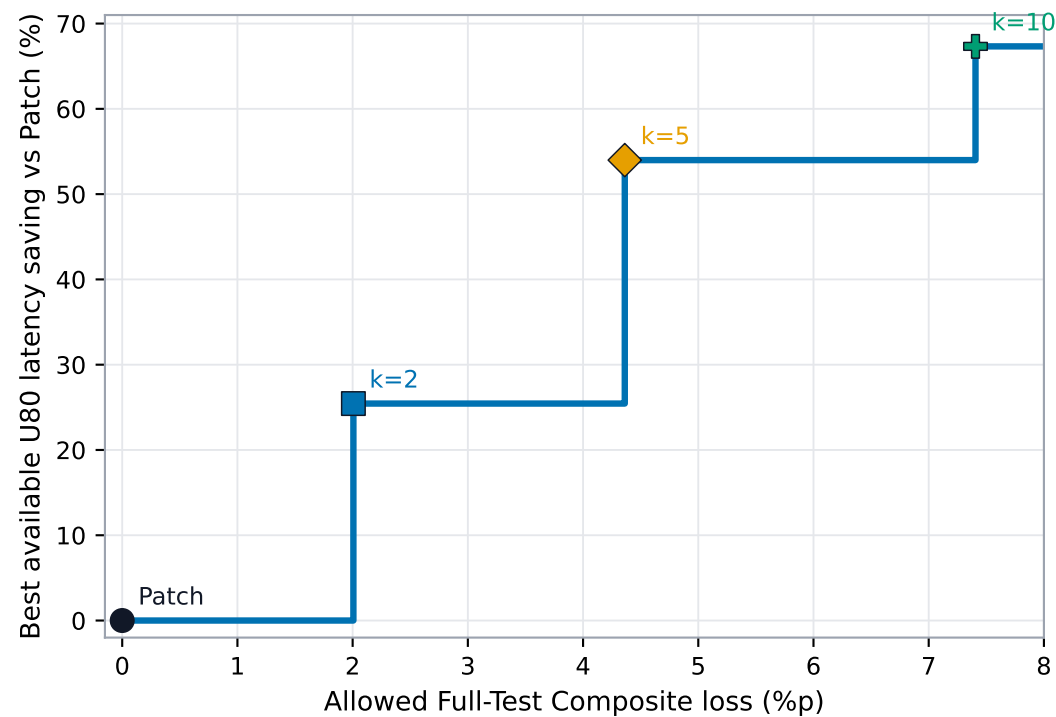
Granite 1B
