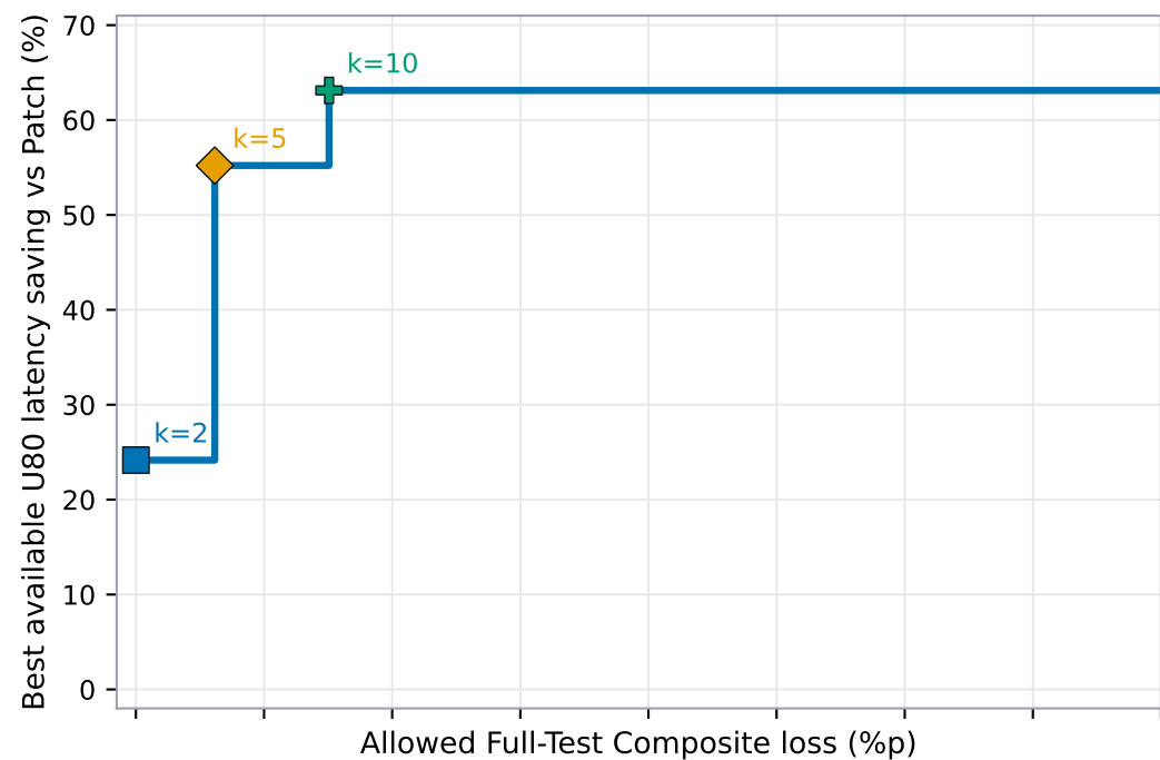
Granite 350M
