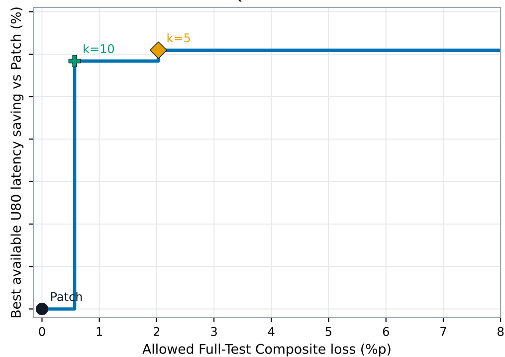
Qwen 2B
