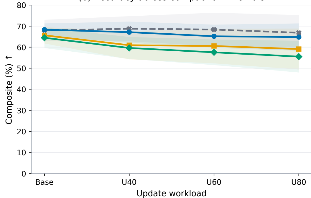
(b) Accuracy across compaction intervals
