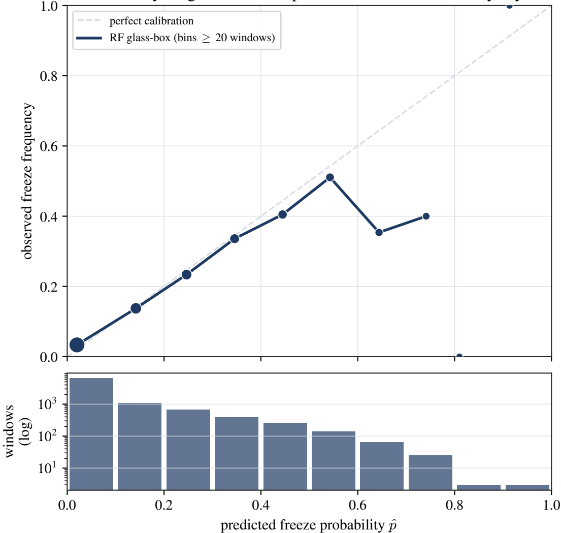
Reliability diagram -- do the probabilities mean what they say?
