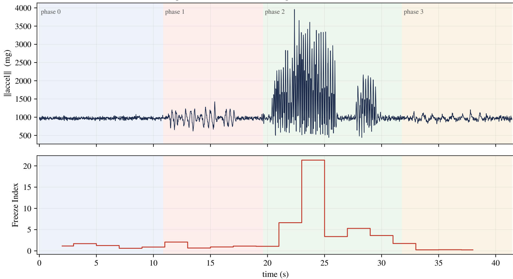
capture1 — accelerometer magnitude and Freeze Index
