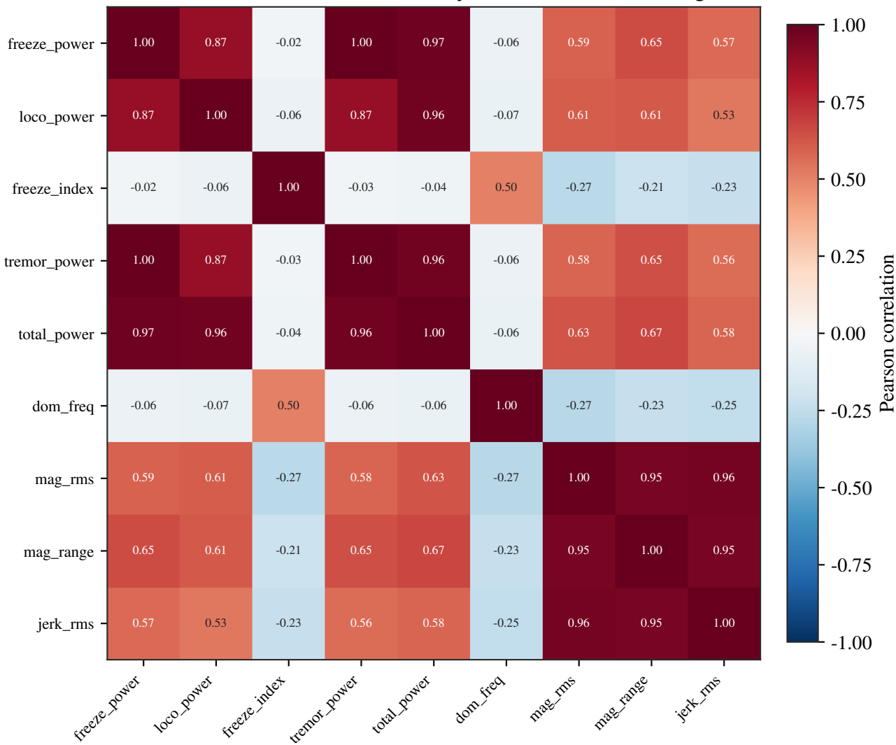
Feature correlation -- redundancy the model has to untangle
