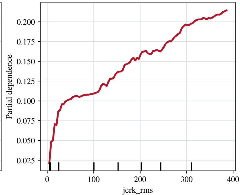
Partial dependence — P(\text{freeze}) vs. top features (9-feature RF, full cohort)
