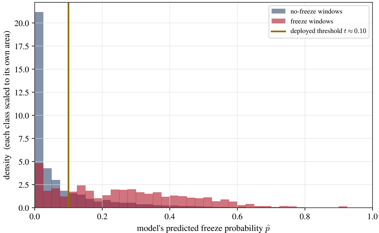
Score separation -- freezes are pushed right, calm gait left
