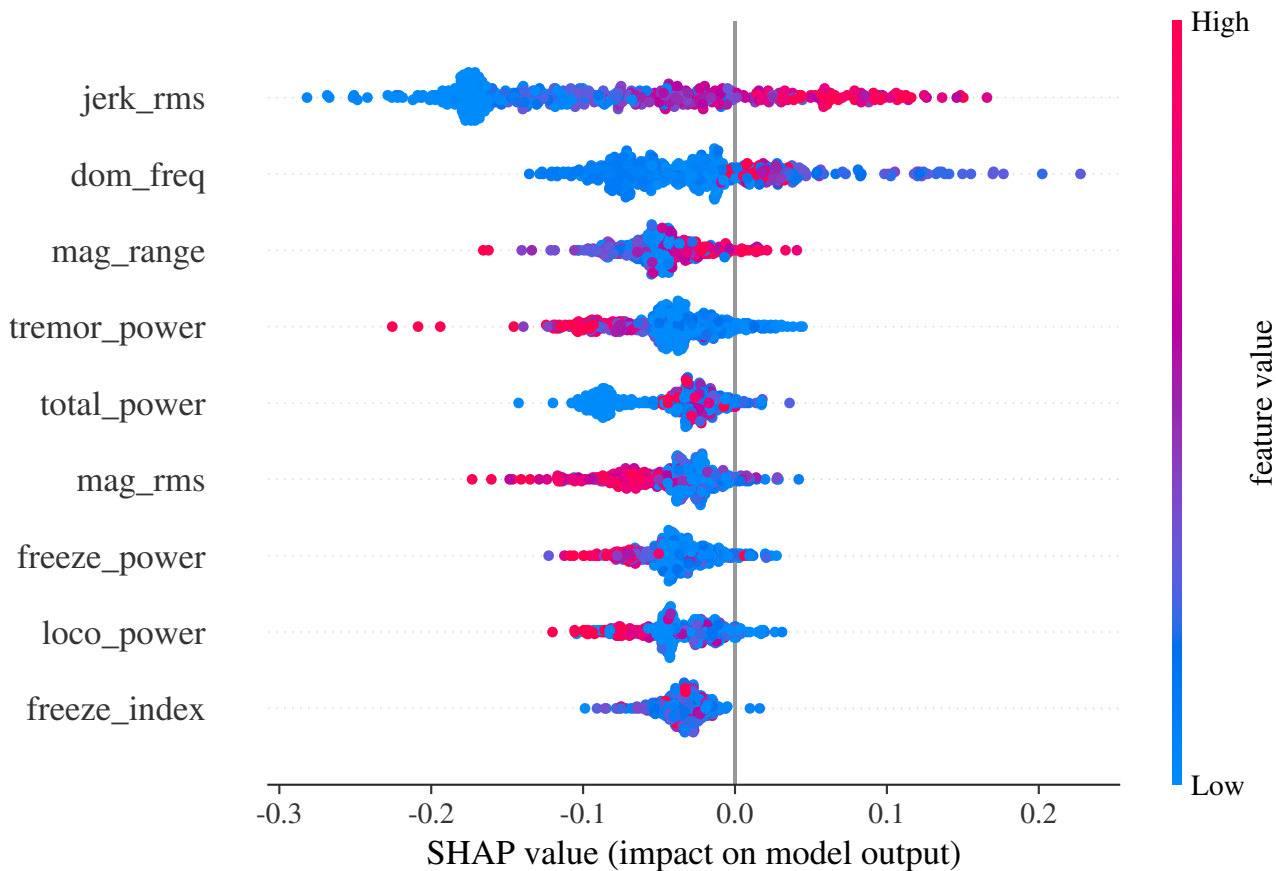
SHAP — per-window contribution to "freeze" (9-feature RF, out-of-fold)
