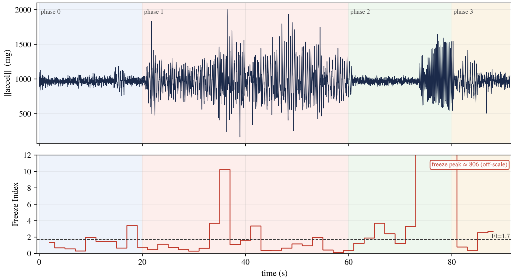
smoketest — accelerometer magnitude and Freeze Index
