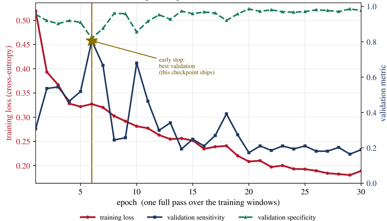
FoGNet learning on Daphnet ankle: loss falls as skill rises
