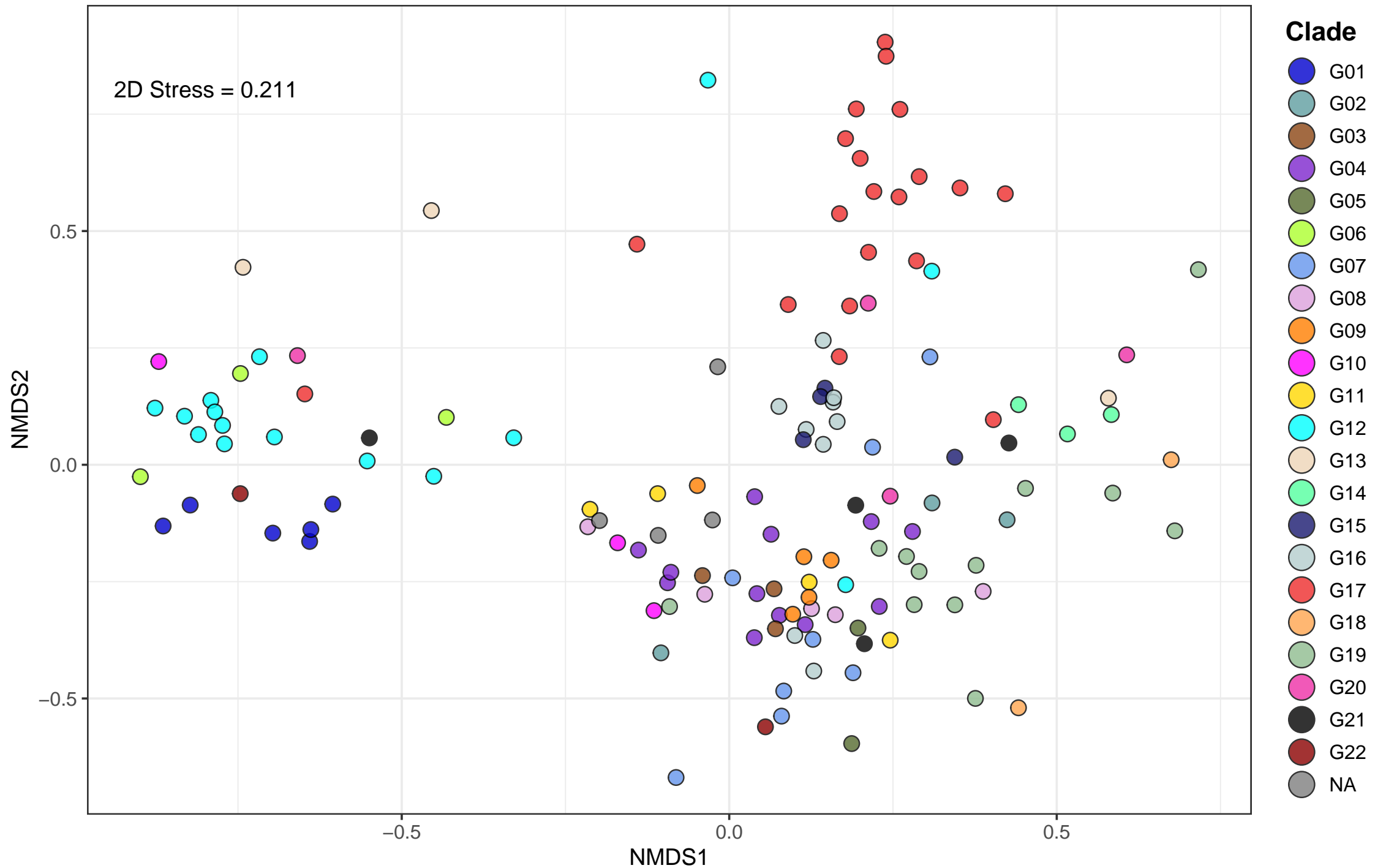
NMDS based on Bray–Curtis distances
