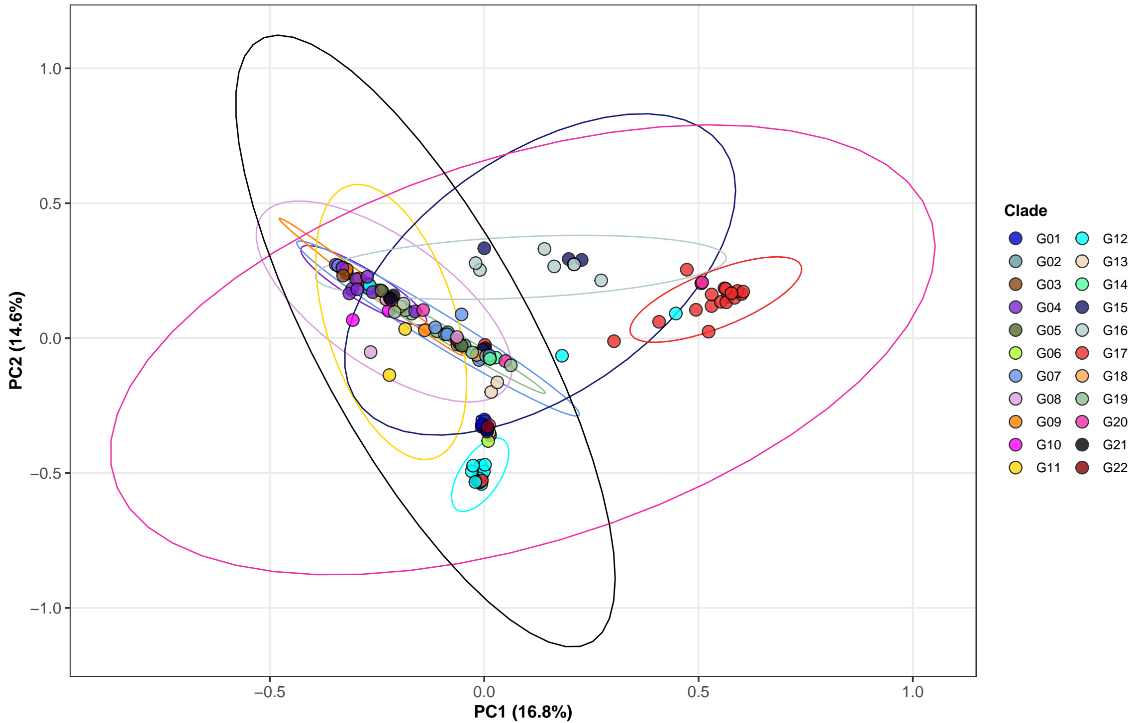
PCoA with 95% confidence ellipses
