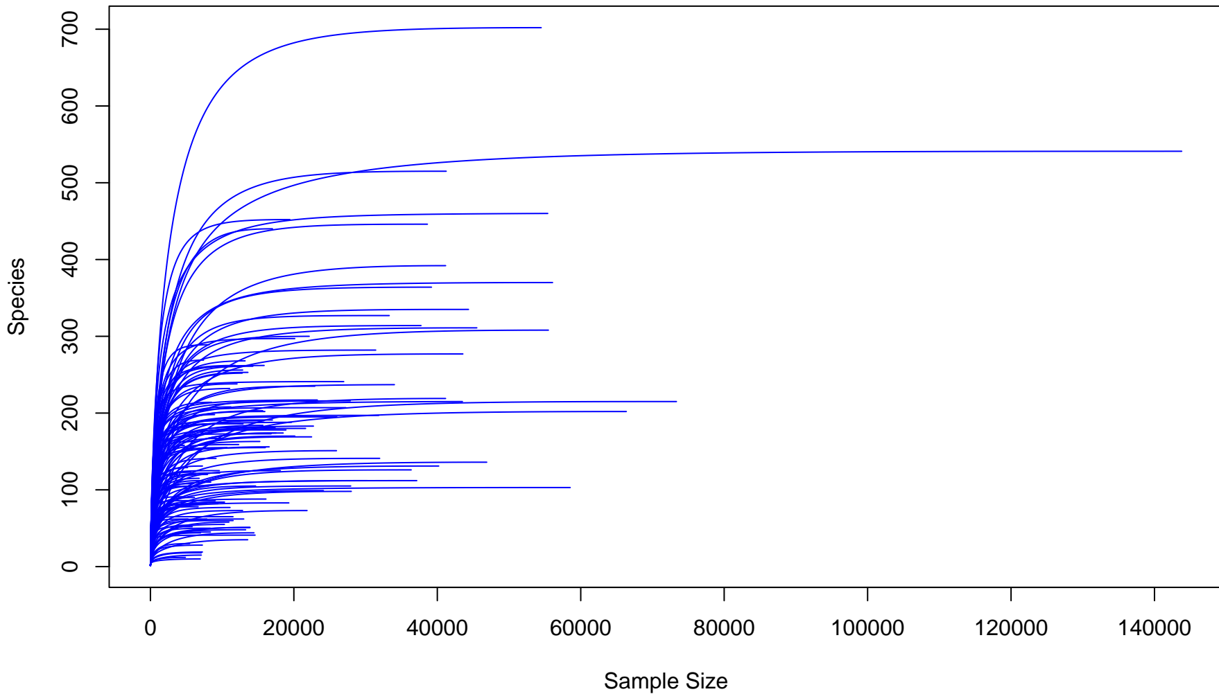
Rarefaction Curves
