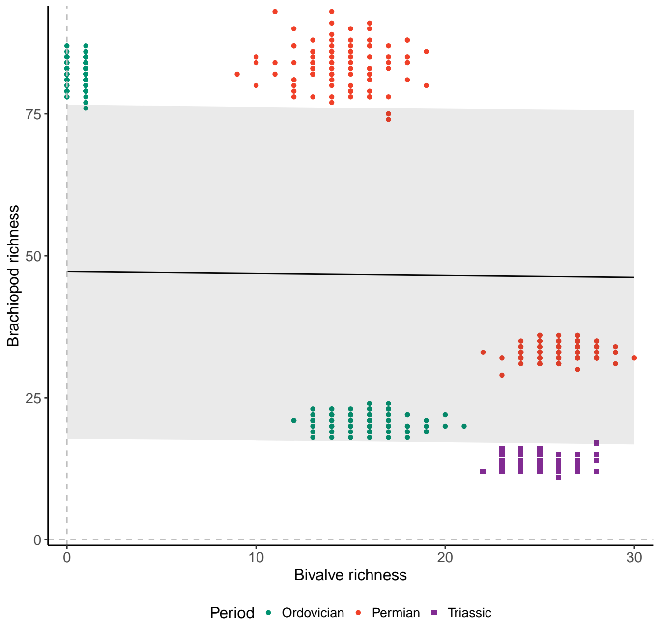
Genera, 200km grid cells, 4 sites, 200km radius, simple model
