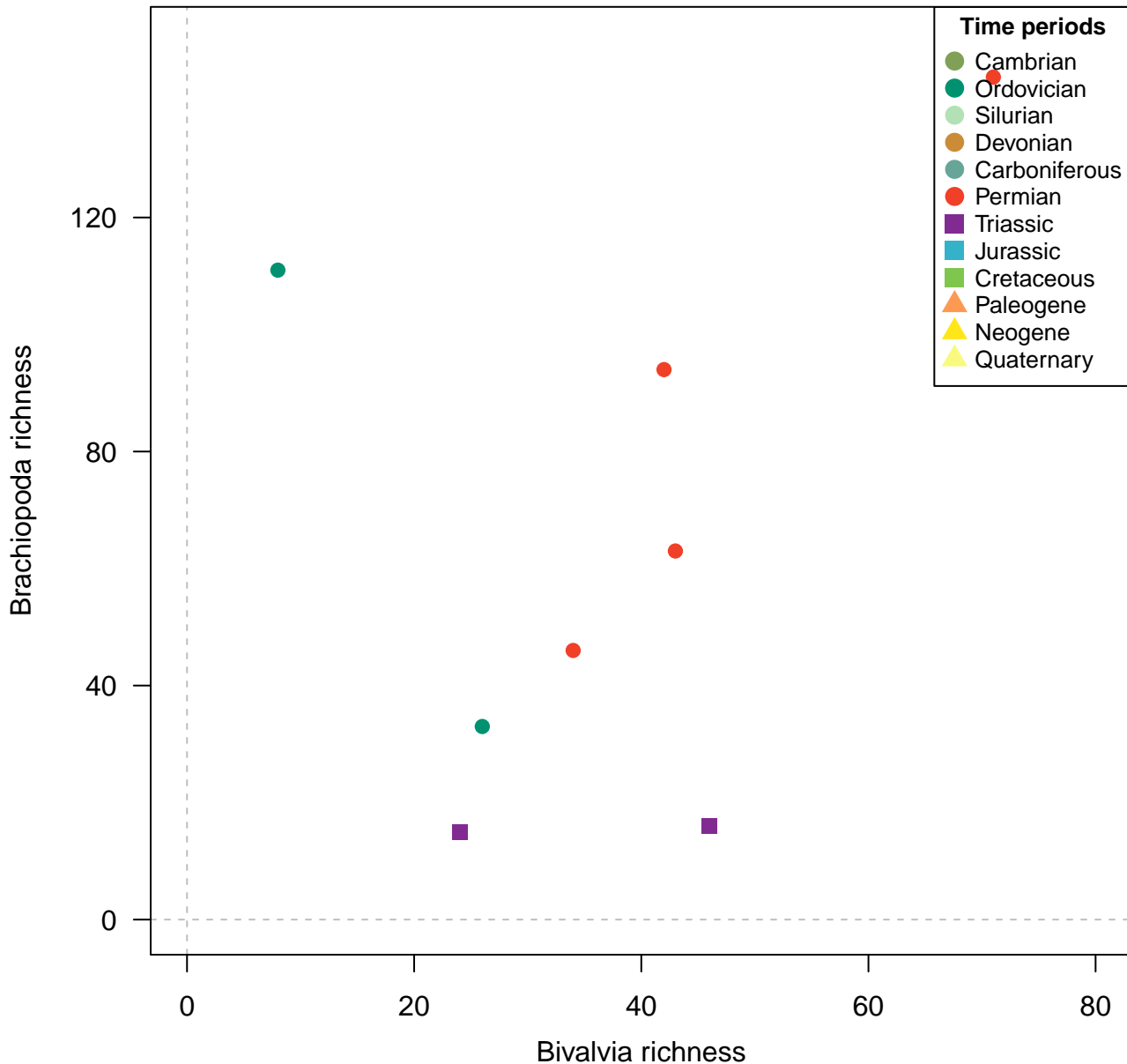
Genera, 100km grid cells, raw, 5 site minima, 1000km radius, 8 subsamples
