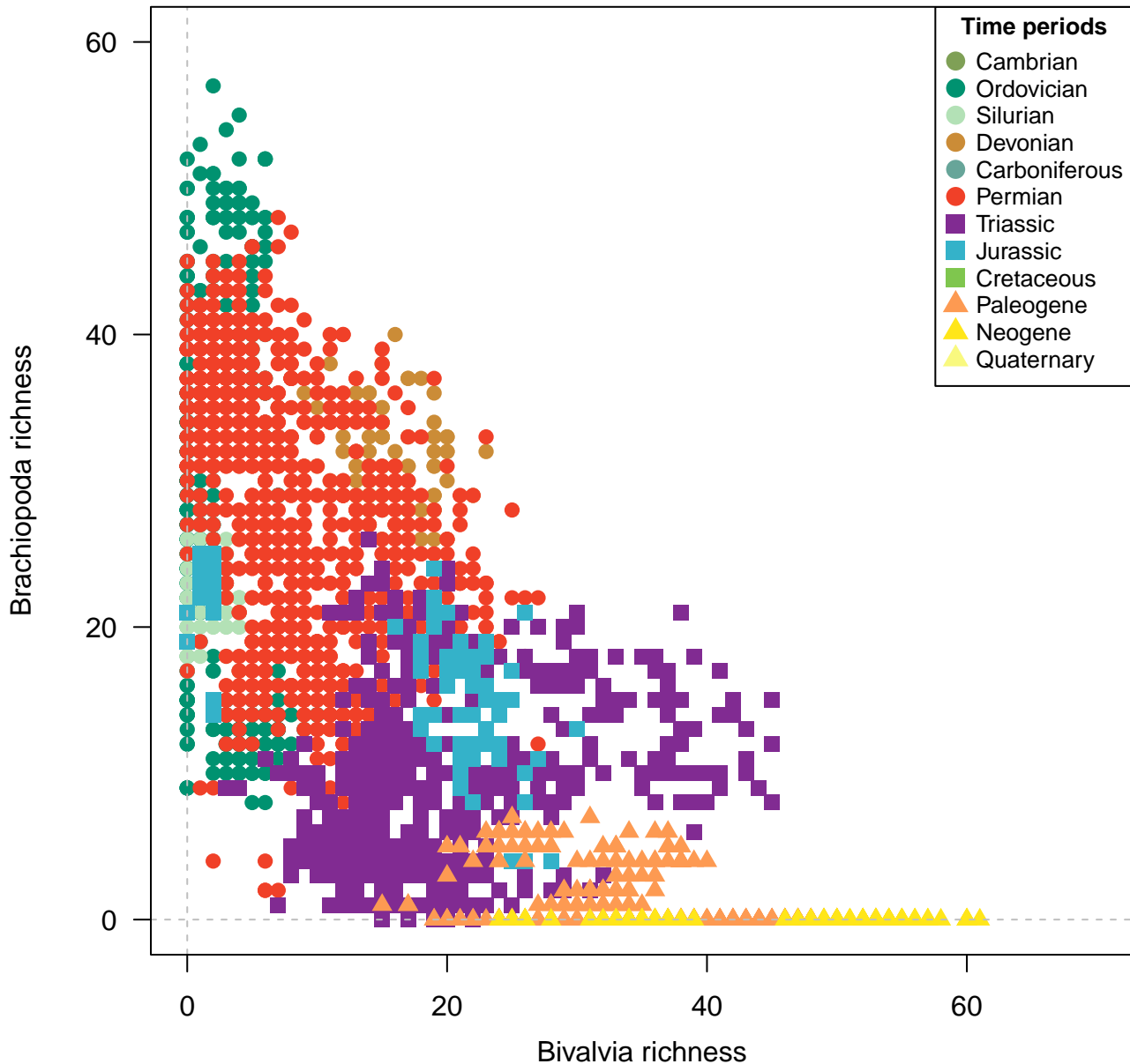
Genera, 100km grid cells, STO rarefaction, 3 site minima, 500km radius, 2800 subsamples
