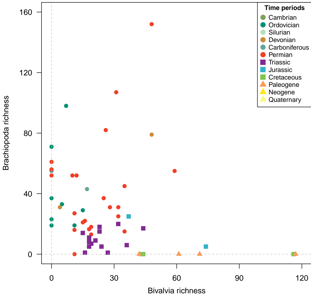
Genera, 200km grid cells, SR (minima sampled), 2 site minima, 200km radius, 61 subsamples
