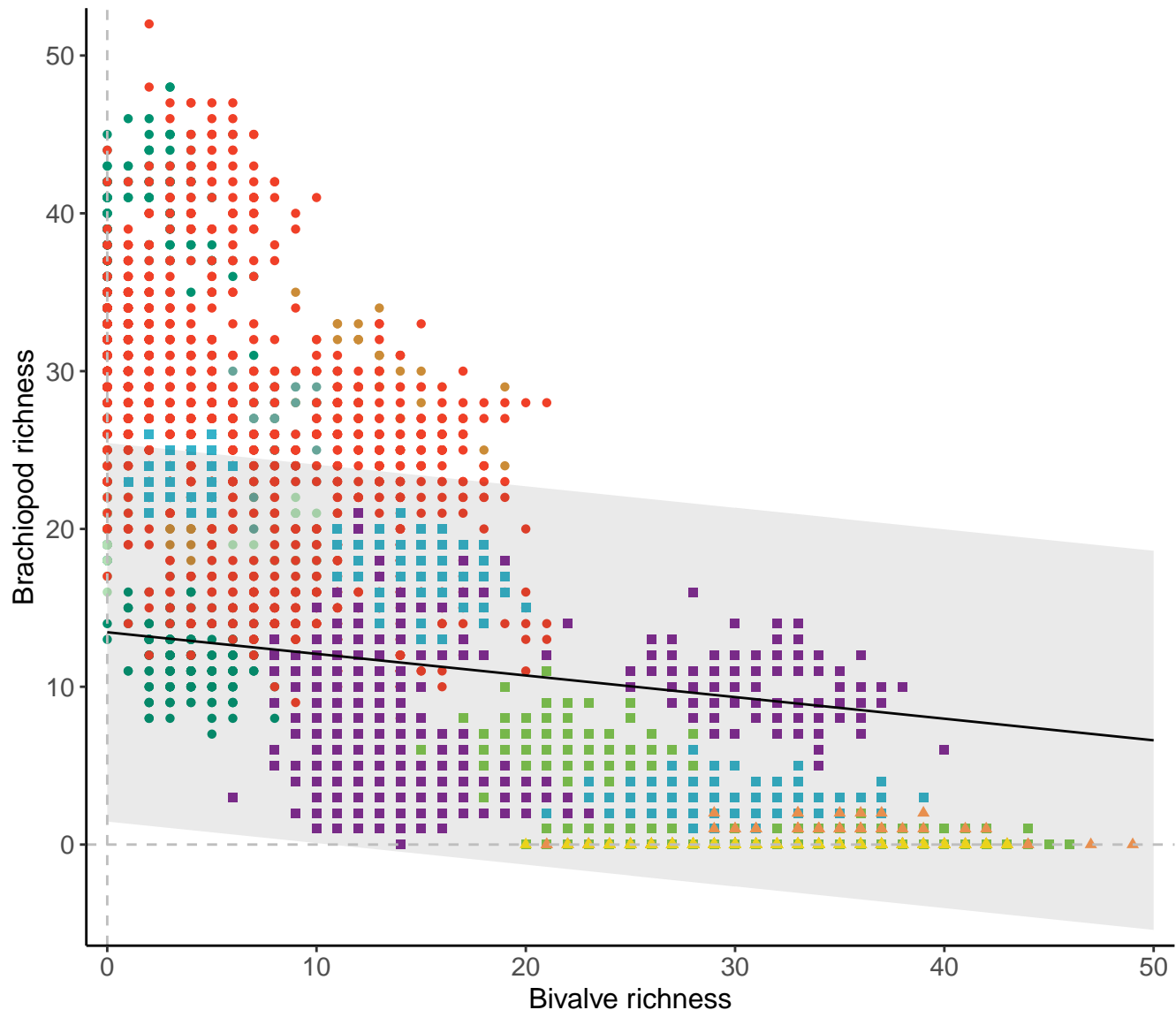
Genera, 200km grid cells, 2 sites, 200km radius, PTME as RE
