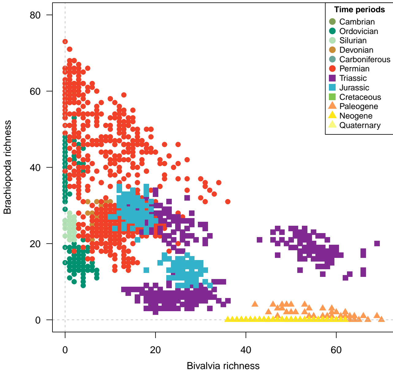
Species, 200km grid cells, STO rarefaction, 3 site minima, 1000km radius, 2100 subsamples
