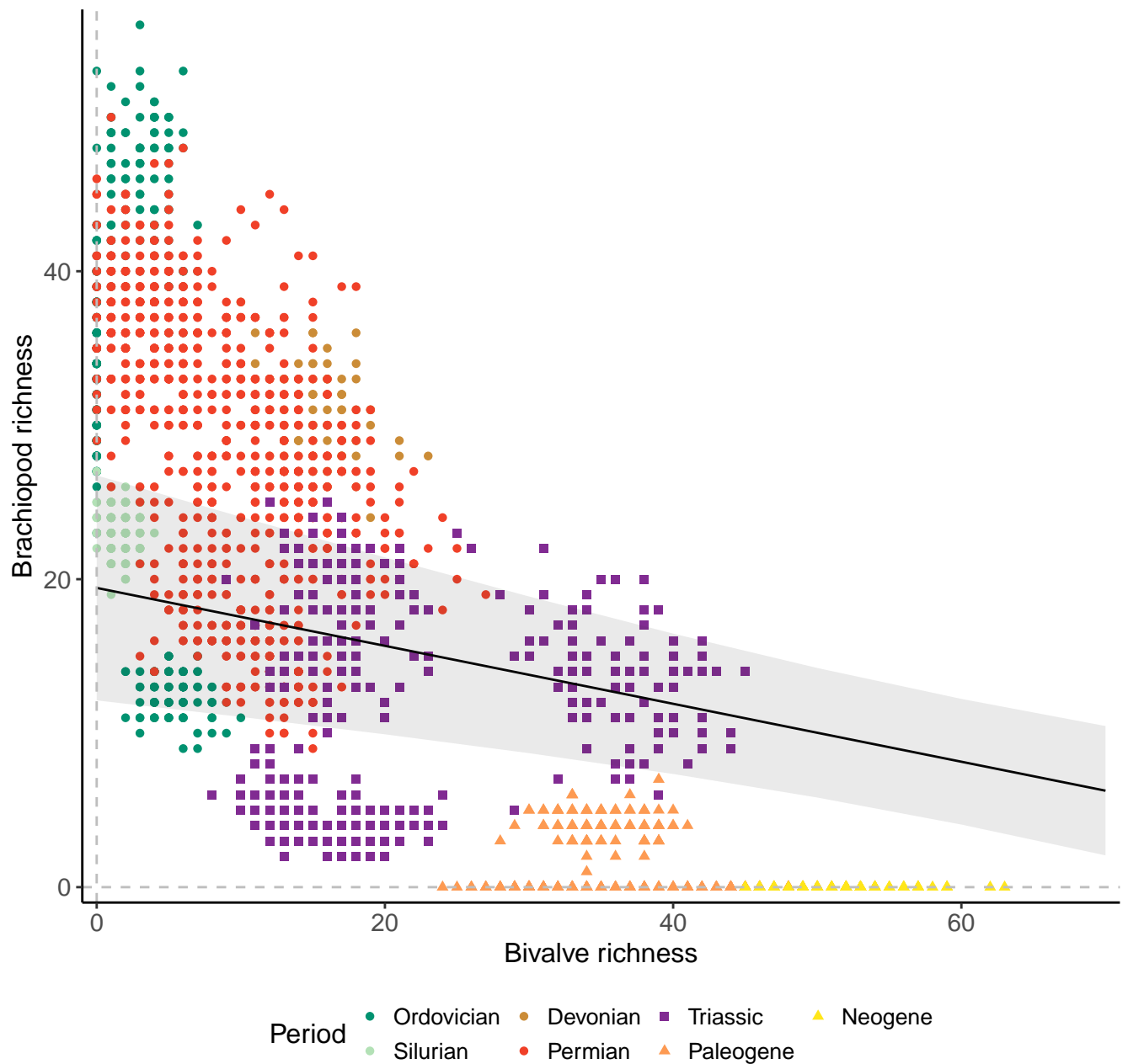
Genera, 100km grid cells, 3 sites, 500km radius
