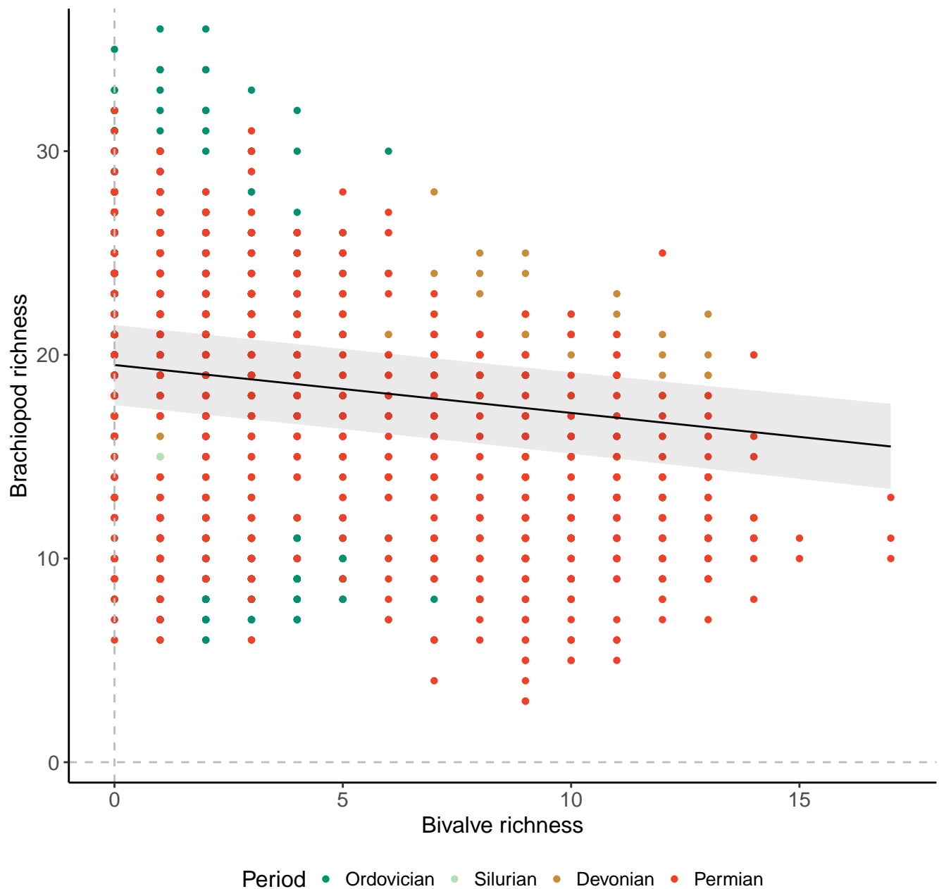
Genera, 100km grid cells, 2 sites, 200km radius, Pre-PTME
