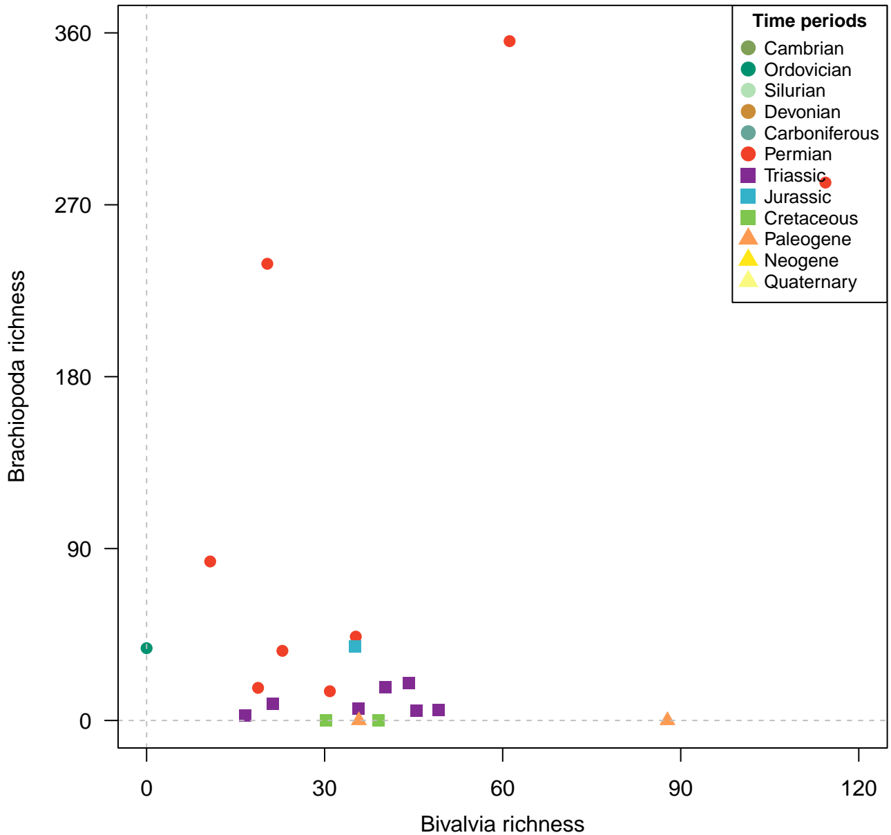
Species, 200km grid cells, SQS (q = 0.9), 2 site minima, 1000km radius, 22 subsamples
