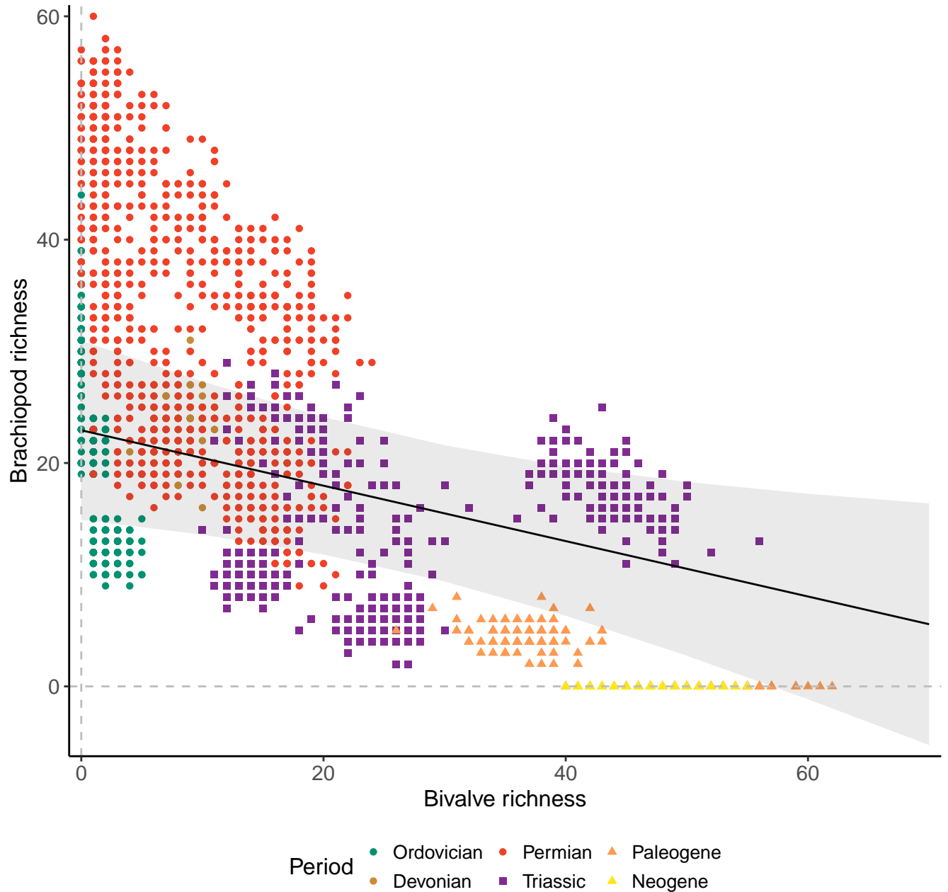
Species, 100km grid cells, 3 sites, 500km radius
