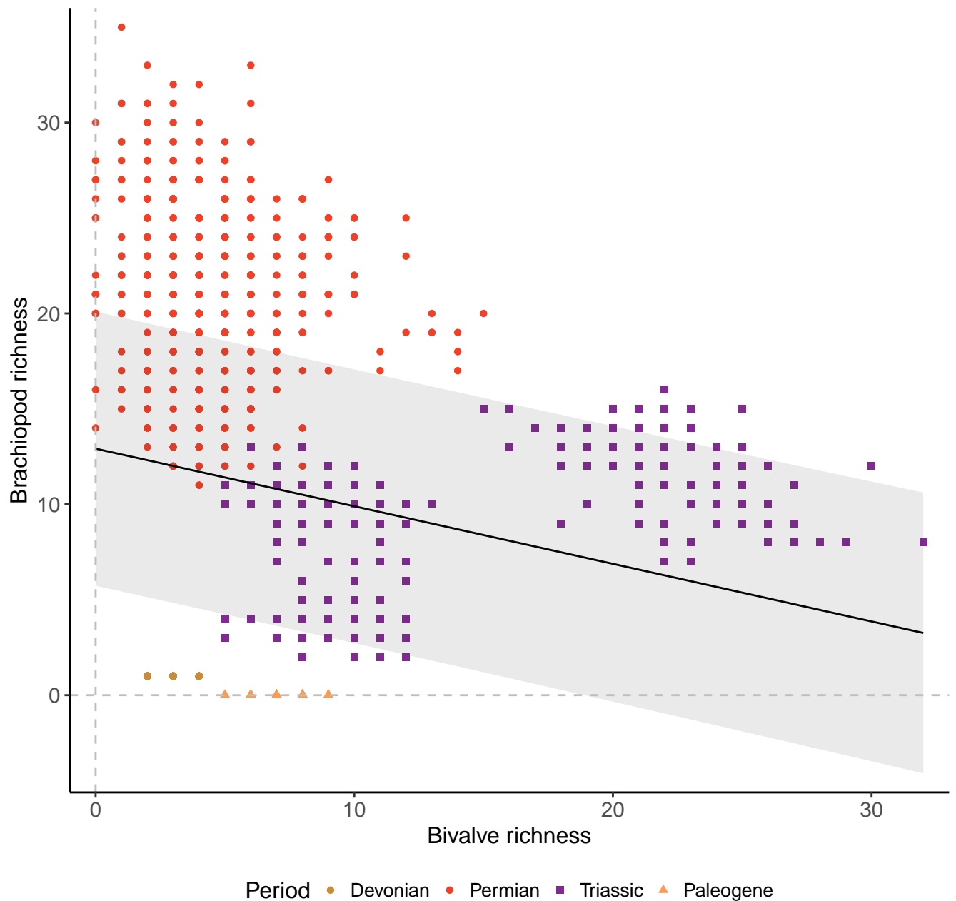
Species, 200km grid cells, 3 sites, 1000km radius, full model
