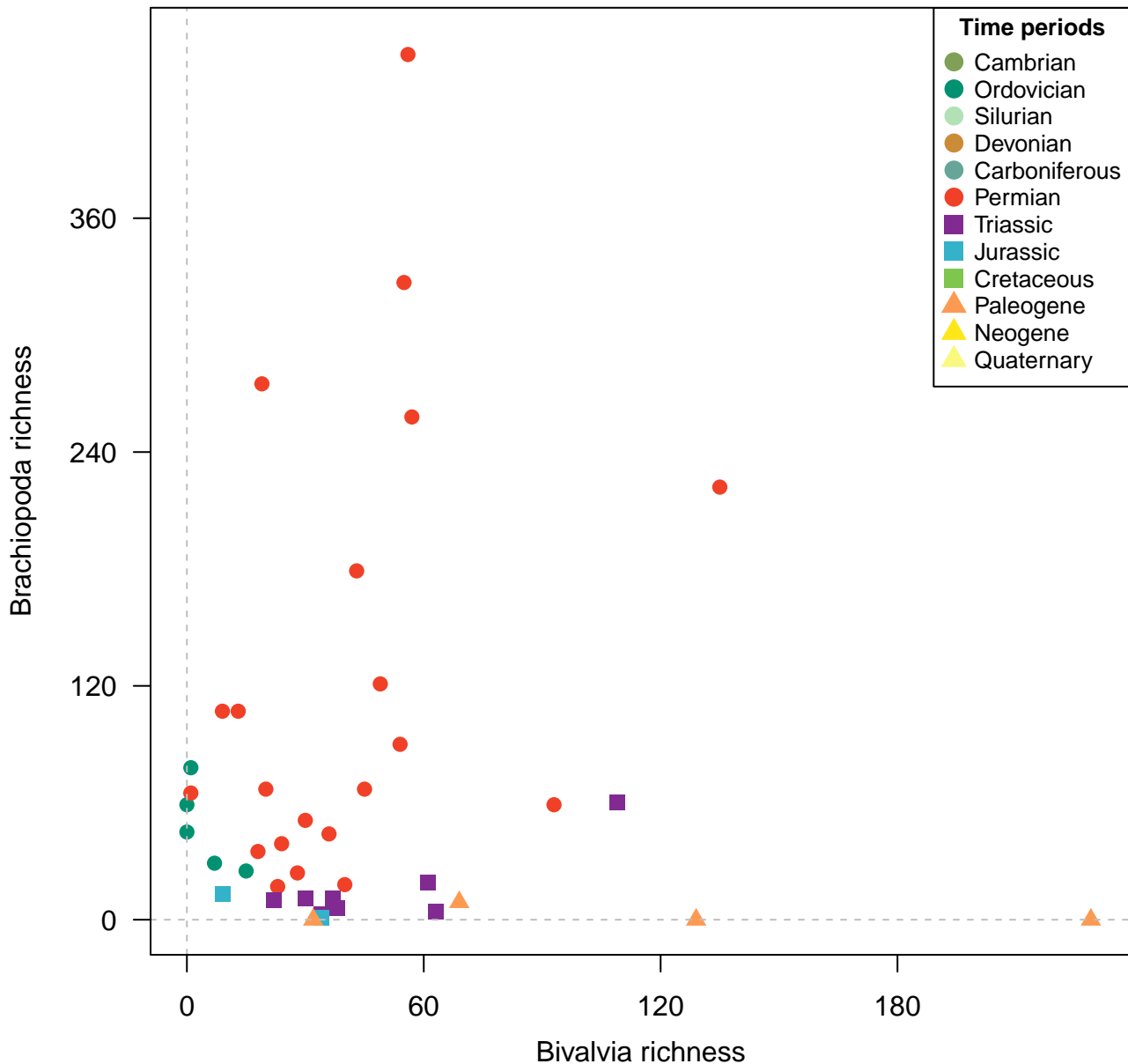
Species, 200km grid cells, raw, 2 site minima, 500km radius, 40 subsamples
