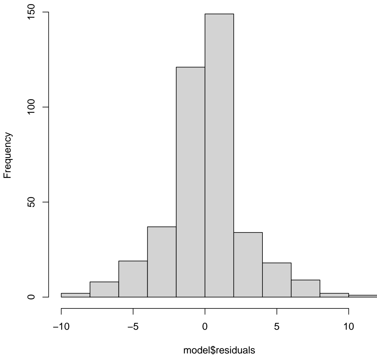
Histogram of model$residuals
