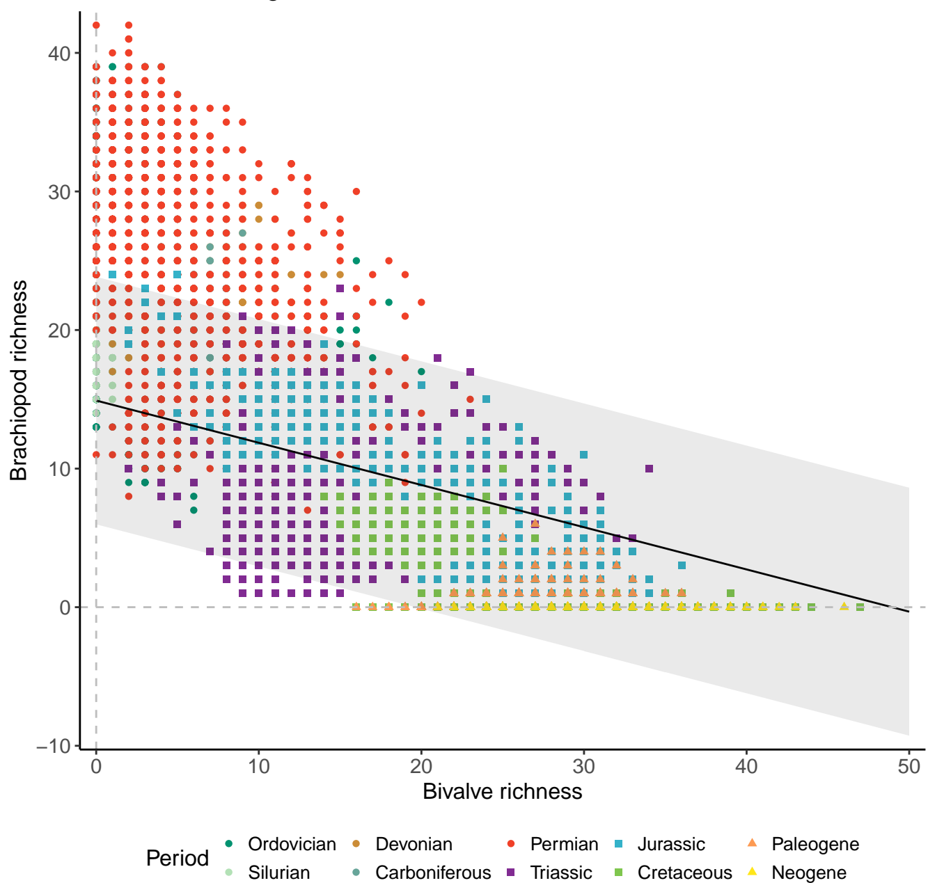
Genera, 200km grid cells, 2 sites, 1000km radius, eras as RE
