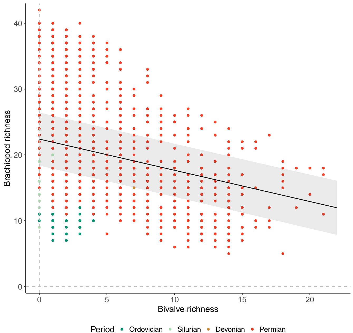
Species, 200km grid cells, 2 sites, 1000km radius, Pre-PTME
