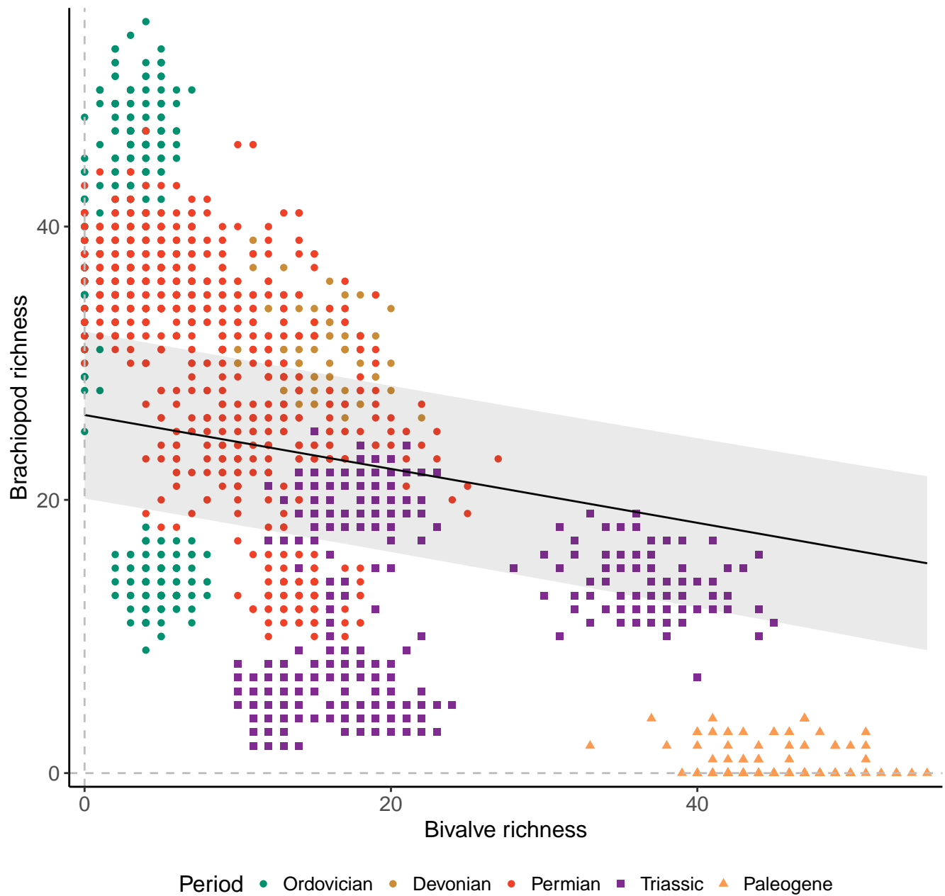
Genera, 100km grid cells, 4 sites, 1000km radius, simple model
