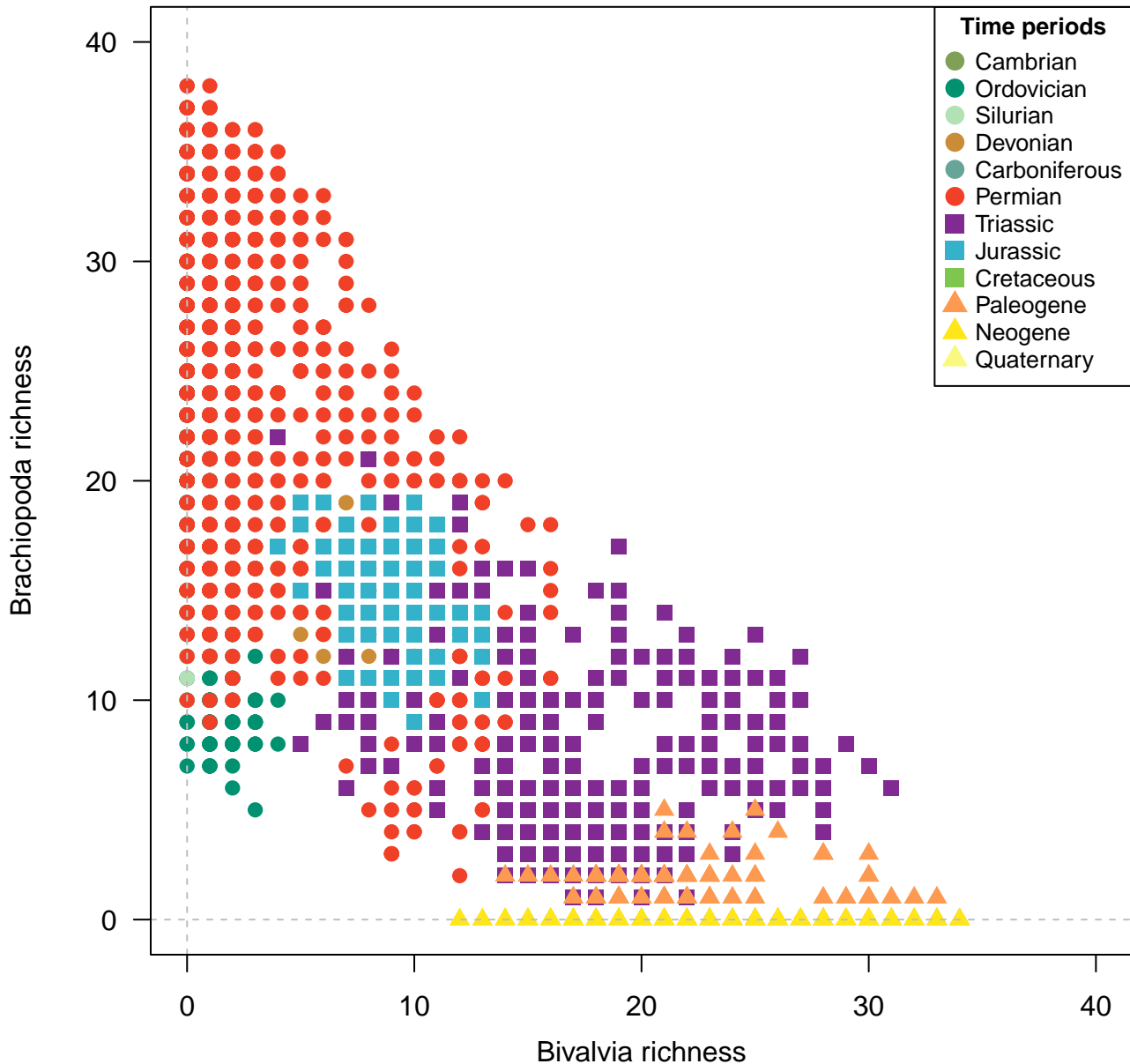
Species, 100km grid cells, STO rarefaction, 2 site minima, 1000km radius, 3800 subsamples
