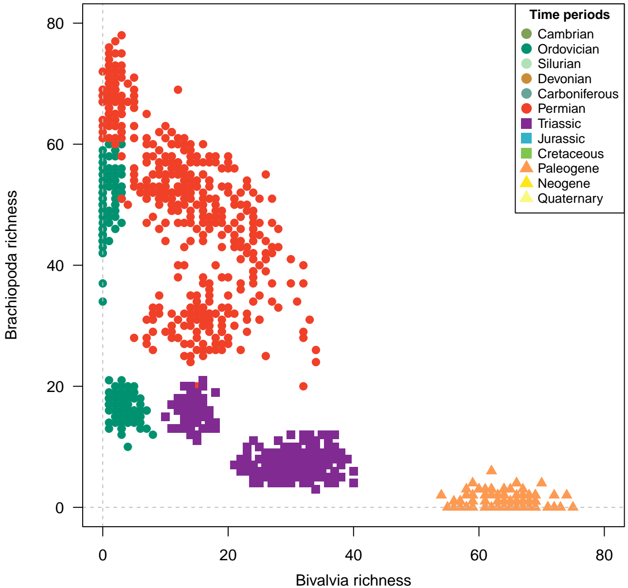
Species, 200km grid cells, STO rarefaction, 5 site minima, 1000km radius, 1200 subsamples
