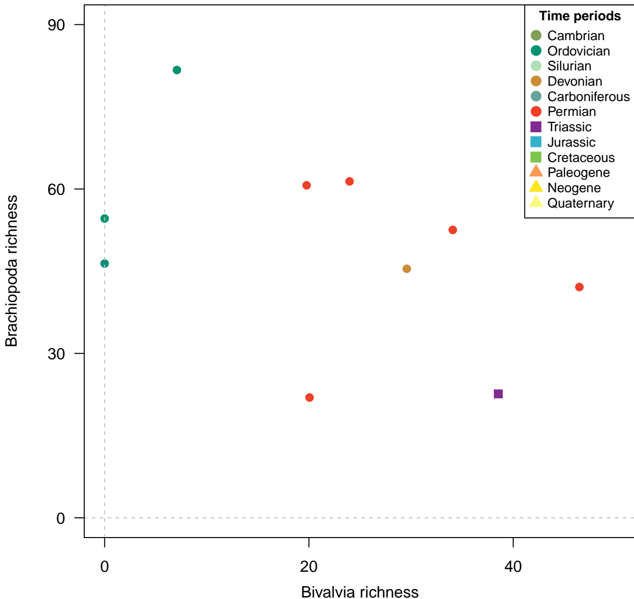
Genera, 100km grid cells, SQS (q = 0.9), 4 site minima, 200km radius, 10 subsamples
