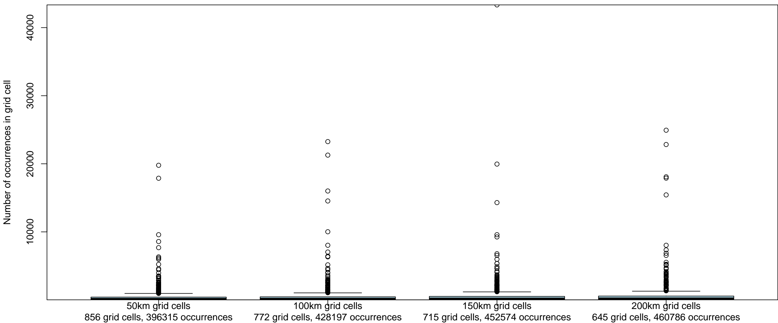
Number of occurrences in viable grid cells (no limit)
