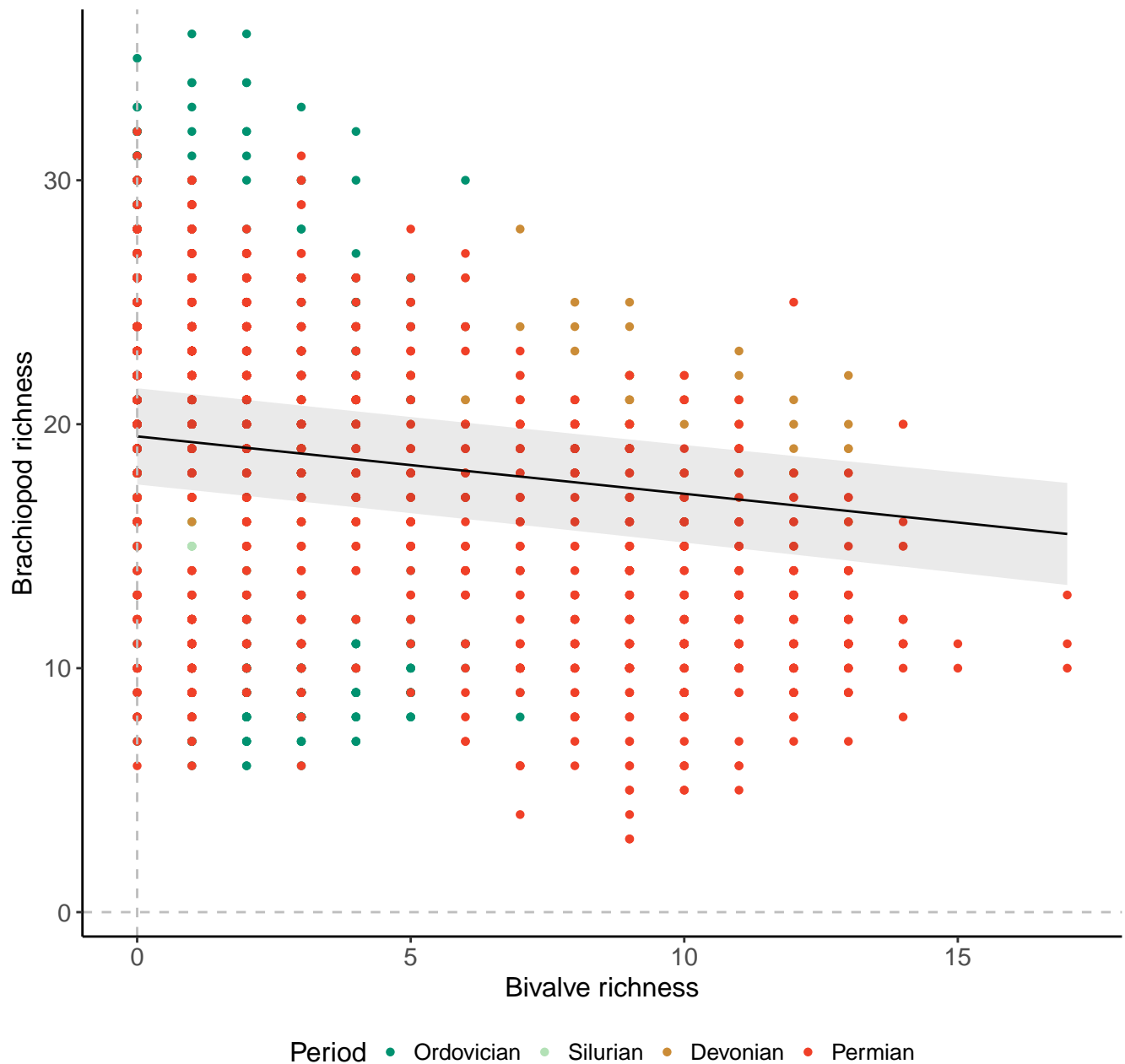
Genera, 100km grid cells, 2 sites, 200km radius, Paleozoic
