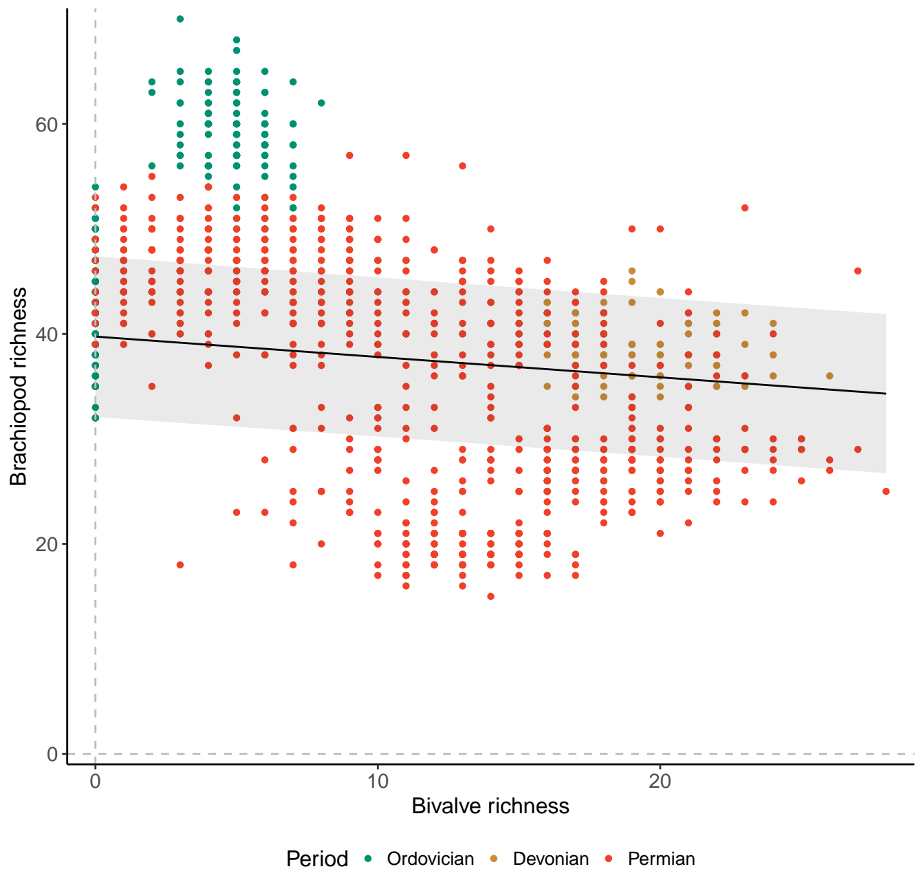
Genera, 100km grid cells, 4 sites, 500km radius, Pre-PTME
