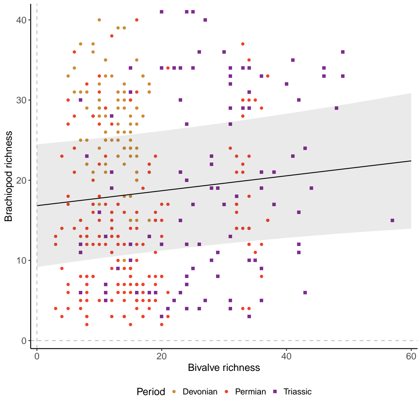
Species, 100km grid cells, 4 sites, 500km radius, simple model
