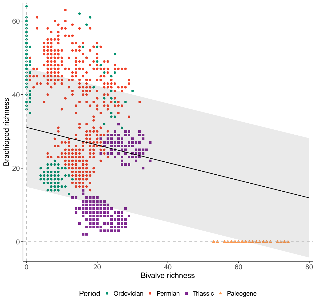
Genera, 200km grid cells, 4 sites, 500km radius, PTME as RE
