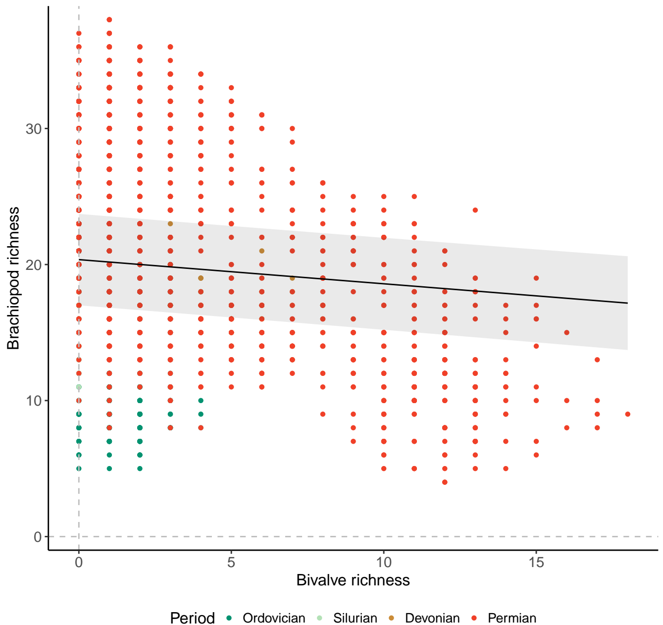
Species, 100km grid cells, 2 sites, 500km radius, Pre-PTME
