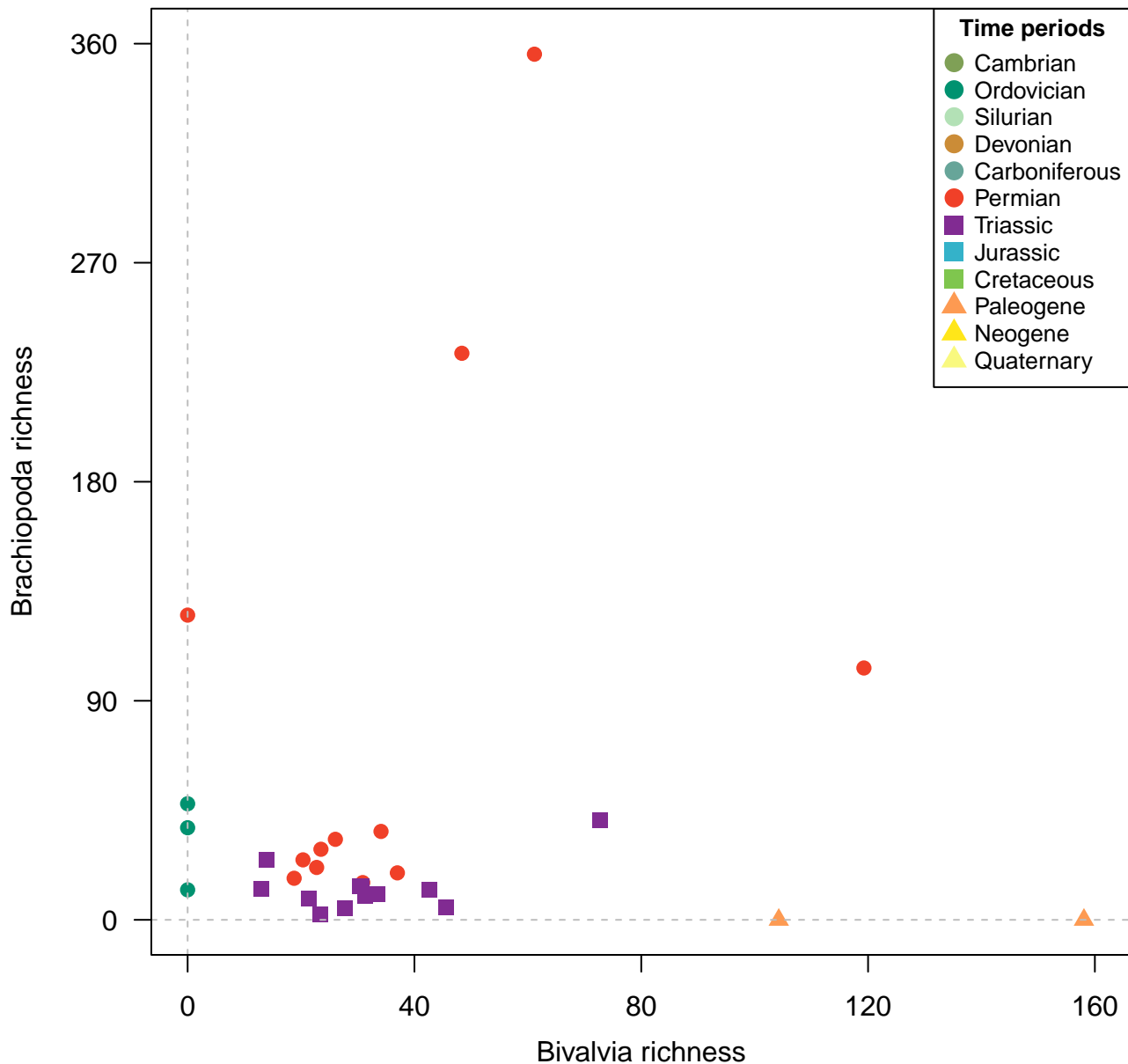
Species, 200km grid cells, SQS (q = 0.9), 2 site minima, 200km radius, 29 subsamples
