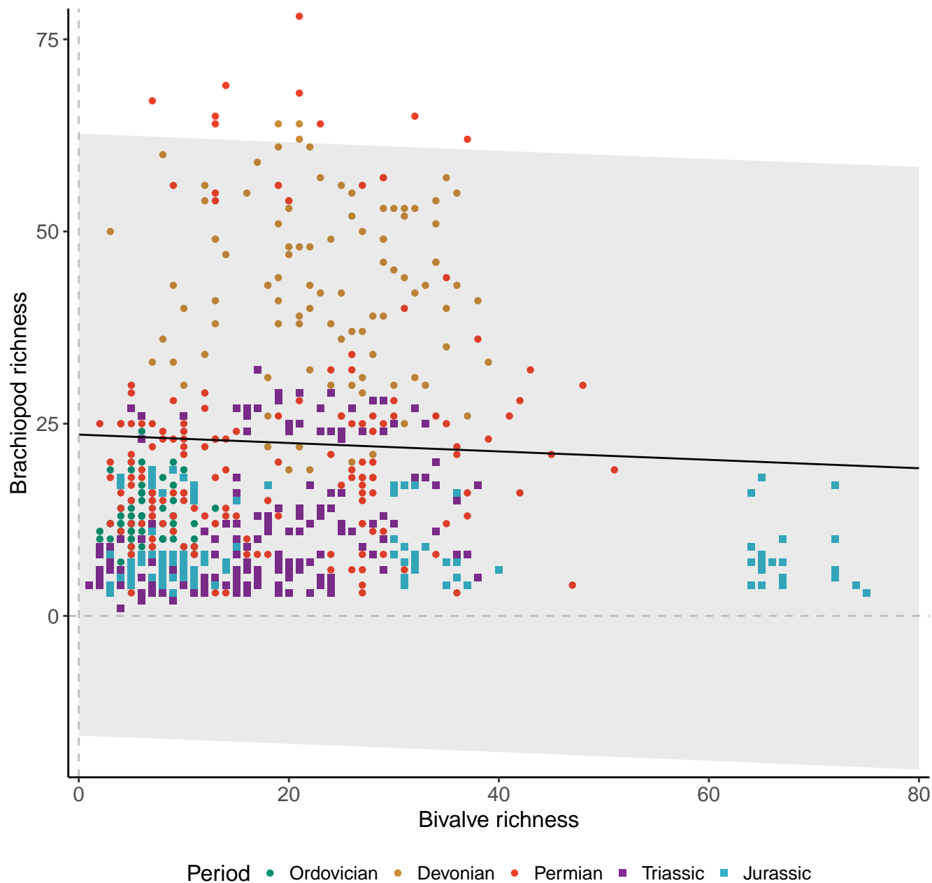
Genera, 200km grid cells, 4 sites, 1000km radius, full model
