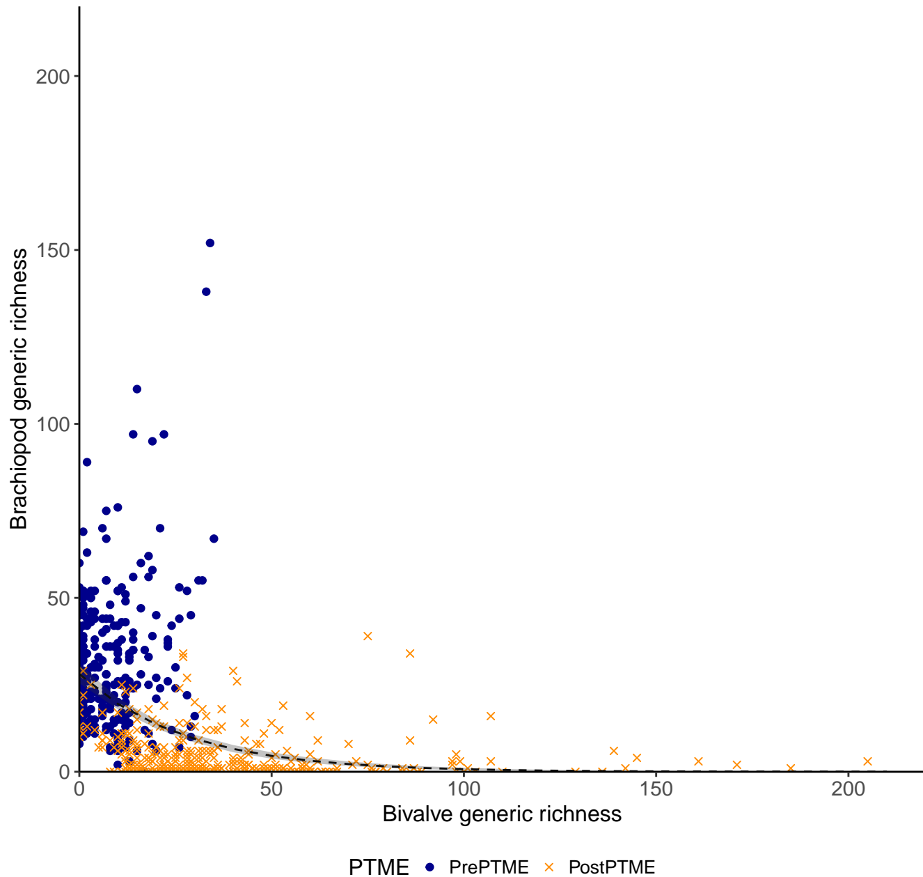
Generic richness, 50km grid cells, 100km radius, 2 cells
