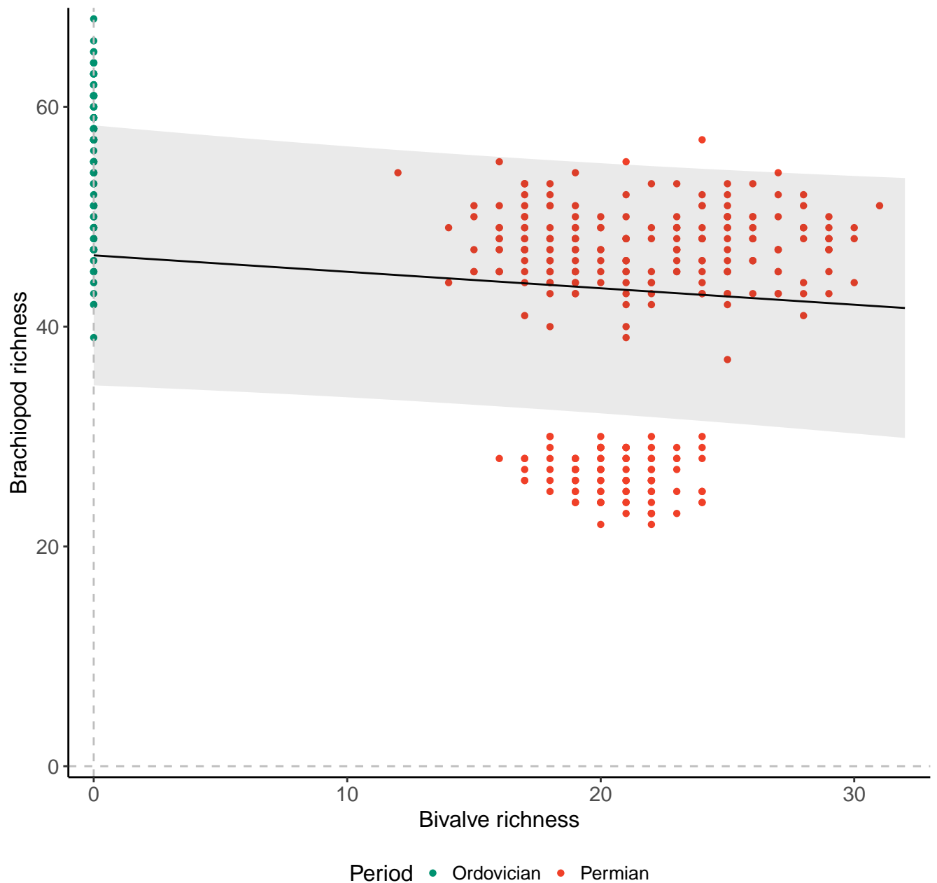
Genera, 100km grid cells, 5 sites, 200km radius, simple model
