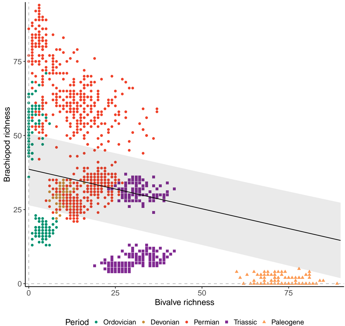
Species, 200km grid cells, 4 sites, 1000km radius, simple model
