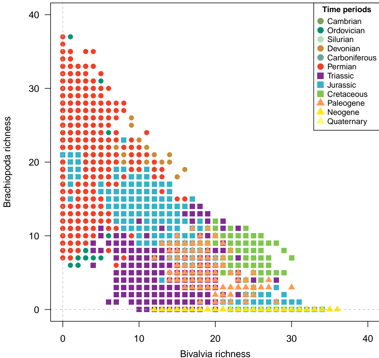
Genera, 100km grid cells, STO rarefaction, 2 site minima, 500km radius, 5900 subsamples
