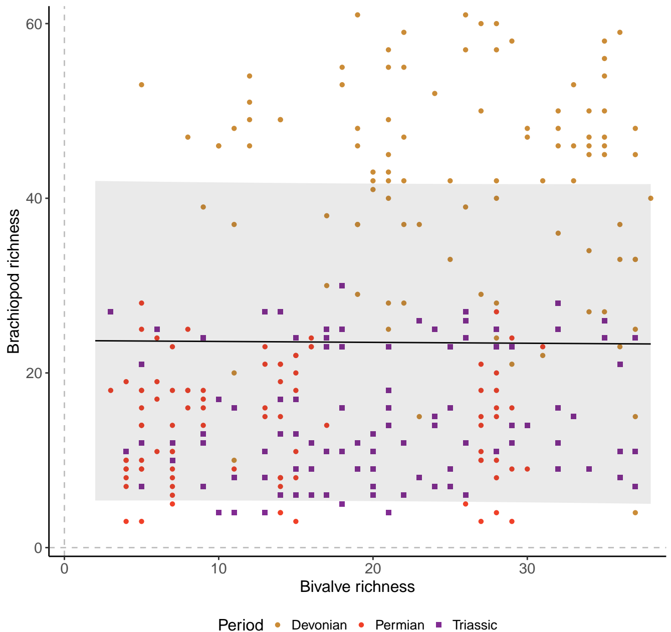
Genera, 100km grid cells, 5 sites, 500km radius, simple model
