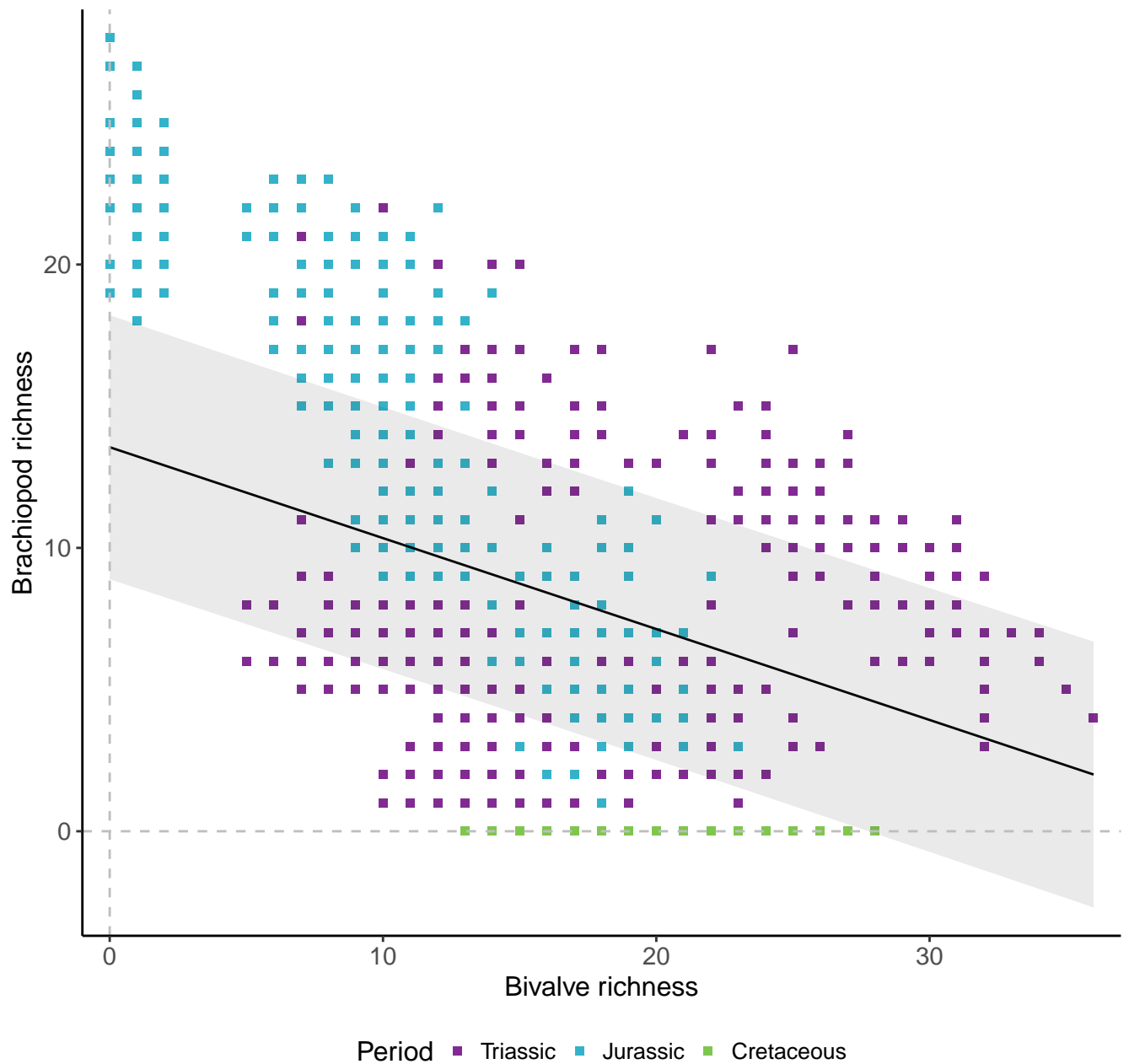
Species, 200km grid cells, 2 sites, 1000km radius, Mesozoic
