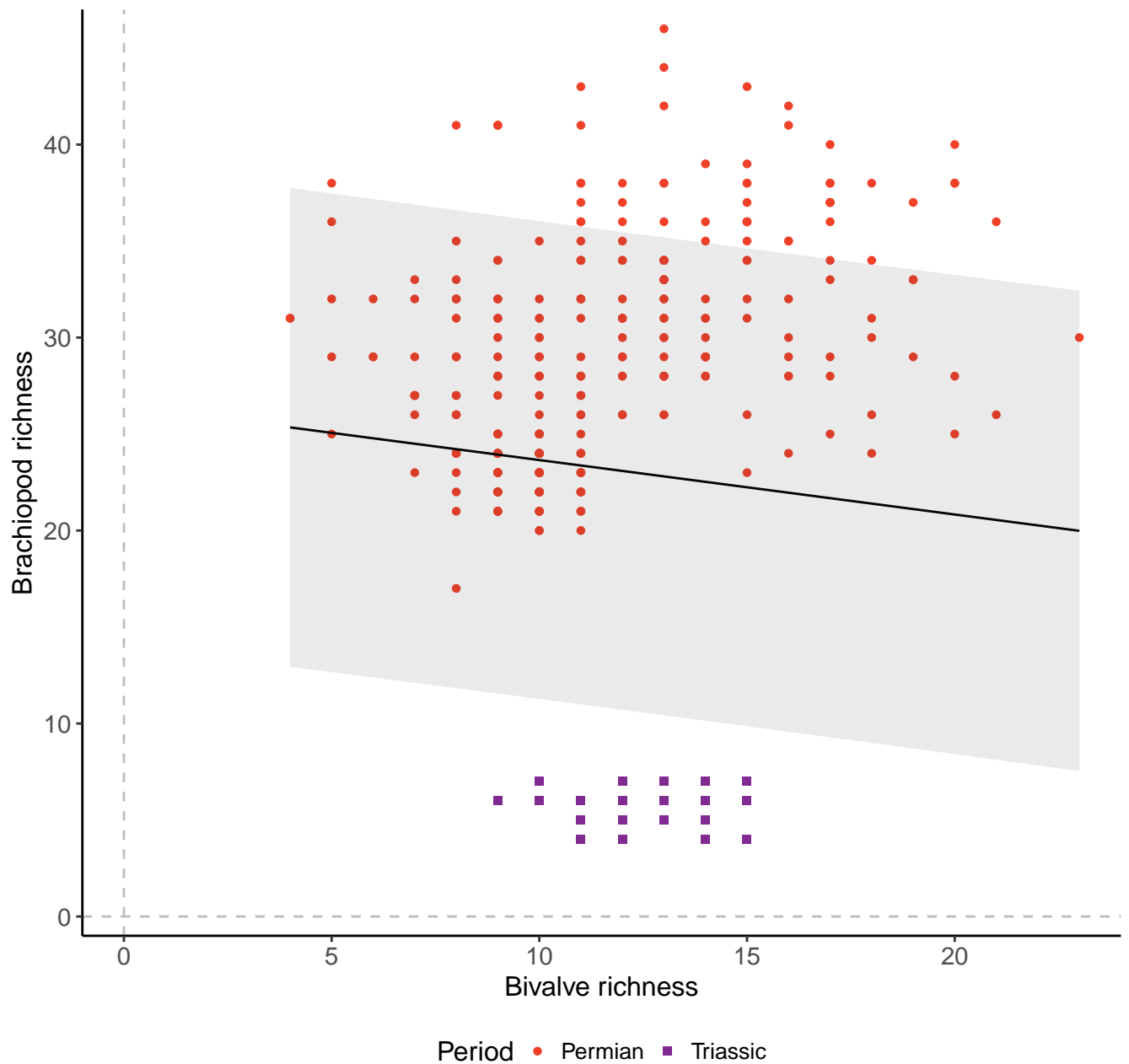
Genera, 100km grid cells, 5 sites, 1000km radius, simple model
