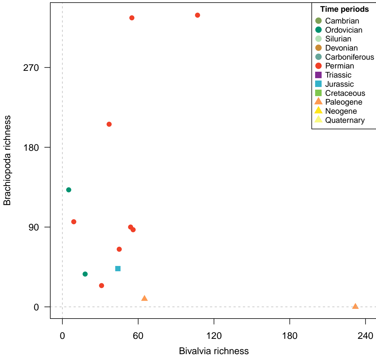
Species, 100km grid cells, raw, 3 site minima, 1000km radius, 13 subsamples
