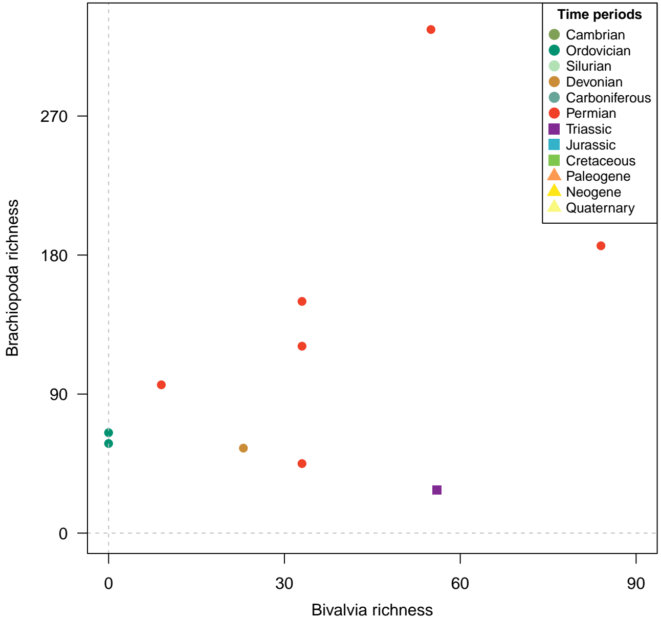
Species, 100km grid cells, raw, 4 site minima, 200km radius, 10 subsamples
