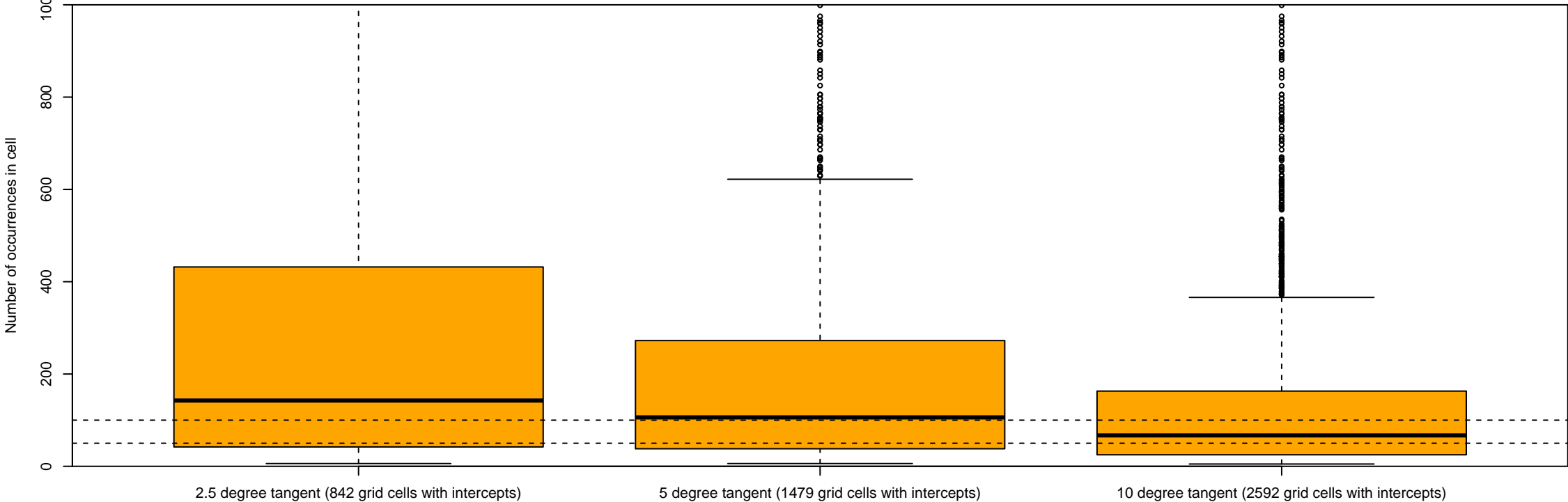
Number of occurrences in 100km grid cells with rarefaction curve intercepts (capped at 1000 occurrences)
