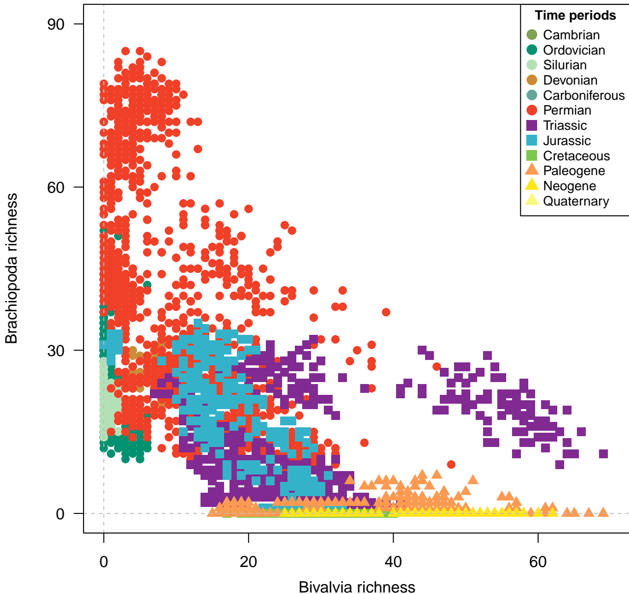
Species, 200km grid cells, STO rarefaction, 2 site minima, 1000km radius, 5000 subsamples
