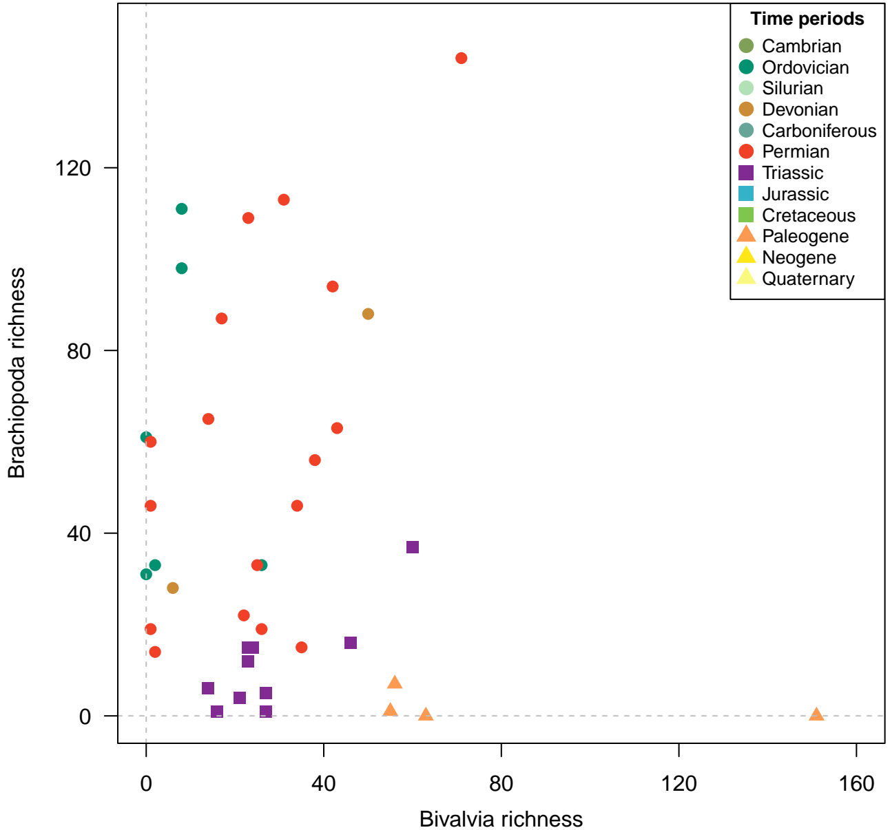
Genera, 100km grid cells, raw, 2 site minima, 1000km radius, 40 subsamples
