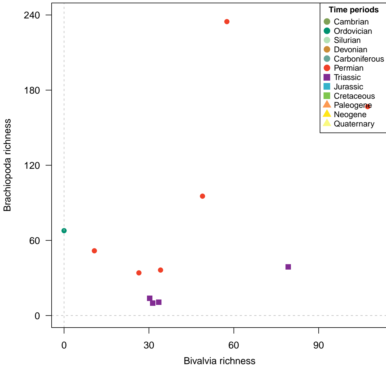
Species, 200km grid cells, SQS (q = 0.9), 3 site minima, 200km radius, 11 subsamples
