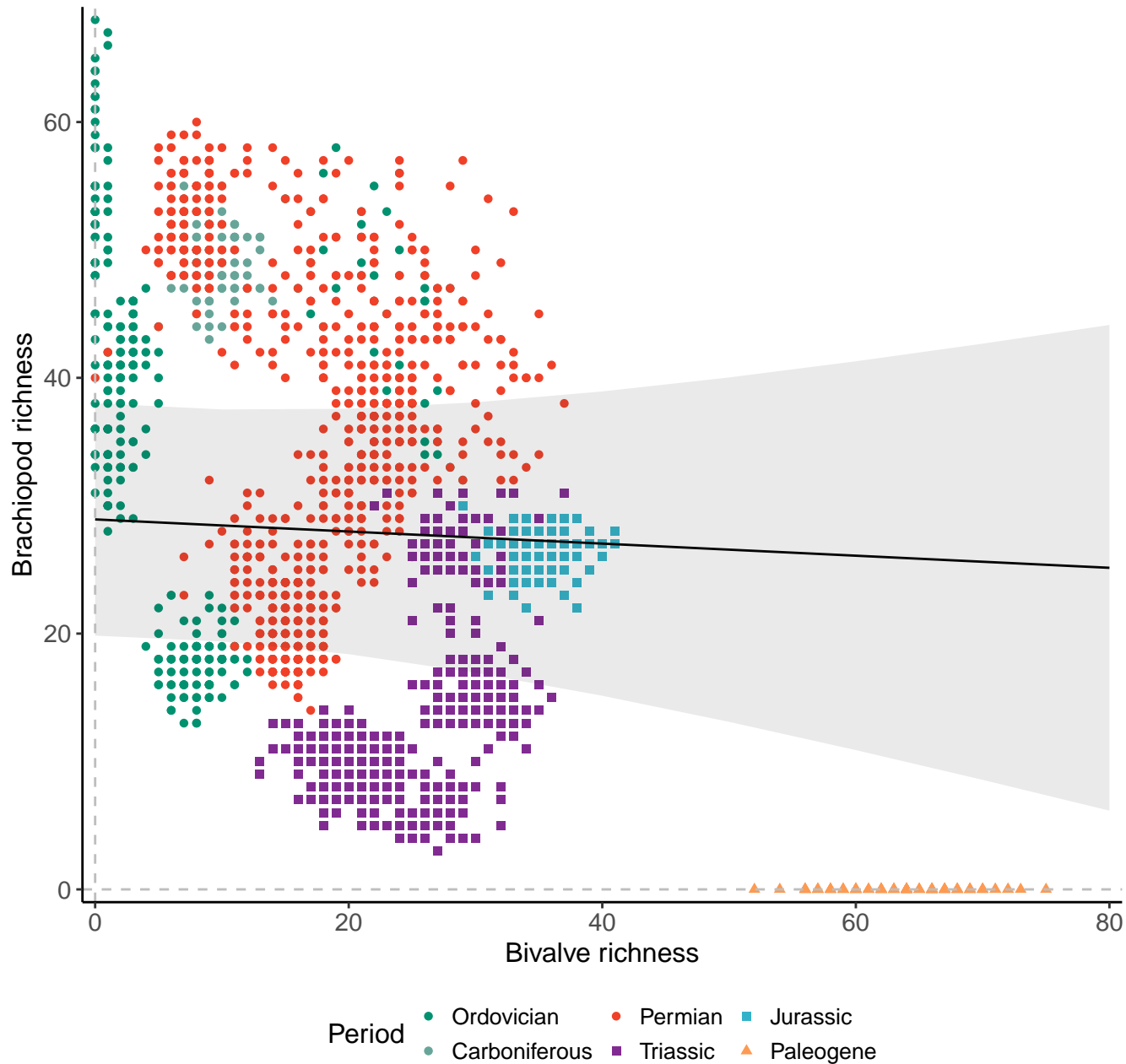
Genera, 200km grid cells, 4 sites, 500km radius
