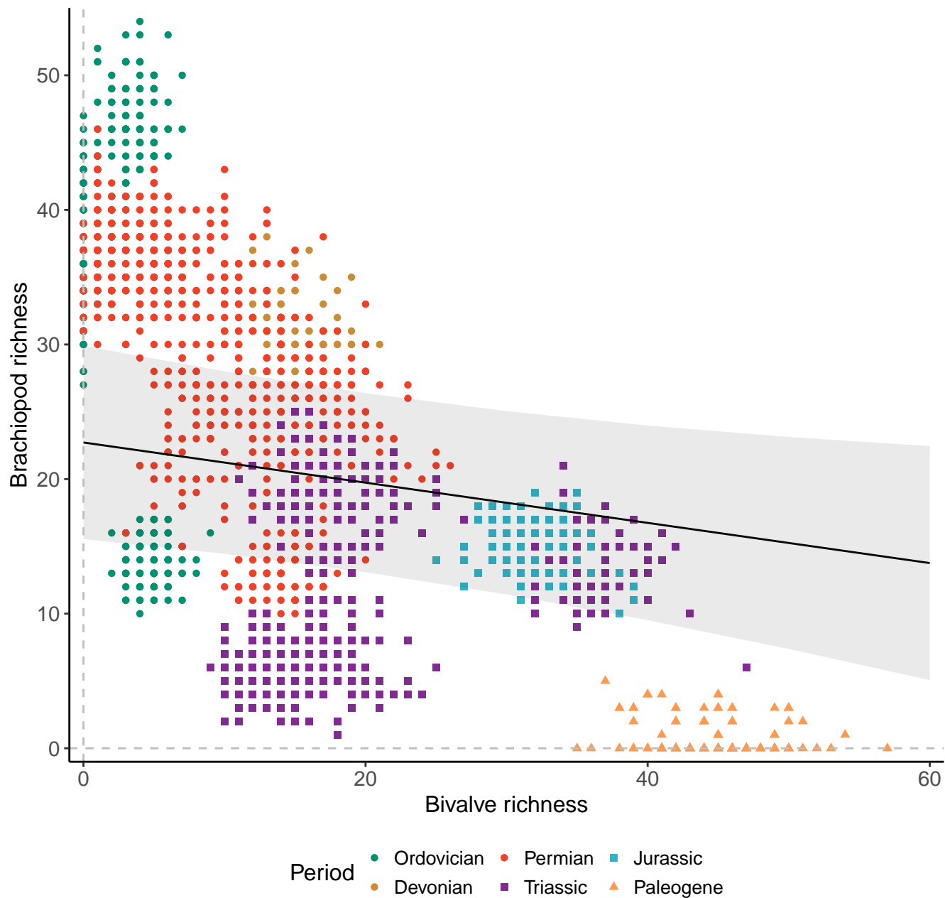
Genera, 100km grid cells, 4 sites, 1000km radius
