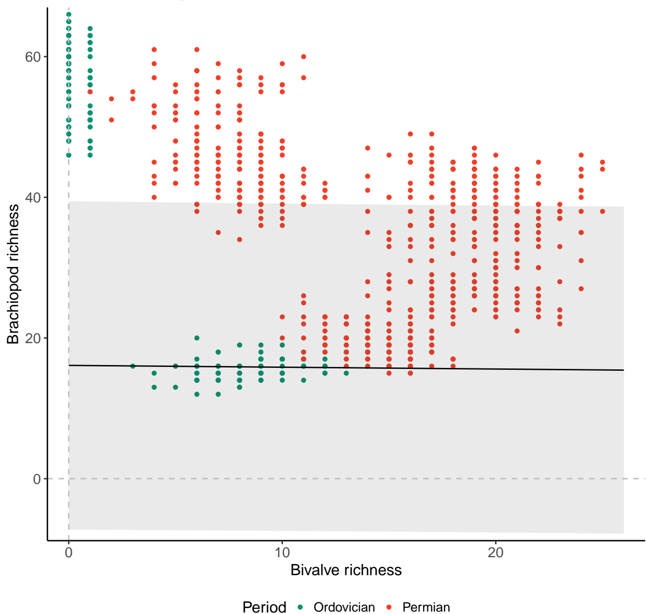
Genera, 200km grid cells, 3 sites, 200km radius, Pre-PTME
