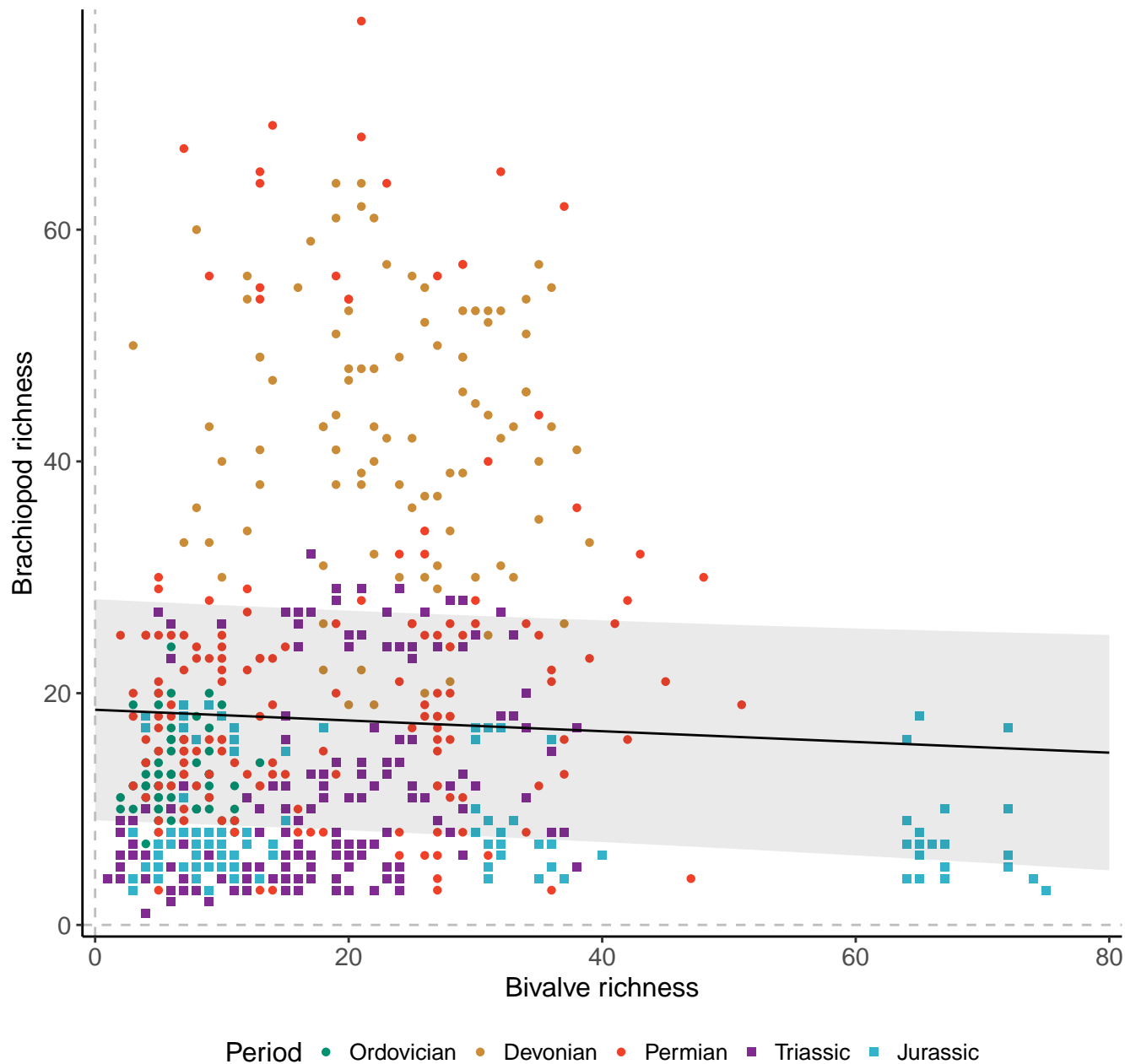
Genera, 200km grid cells, 4 sites, 1000km radius, simple model
