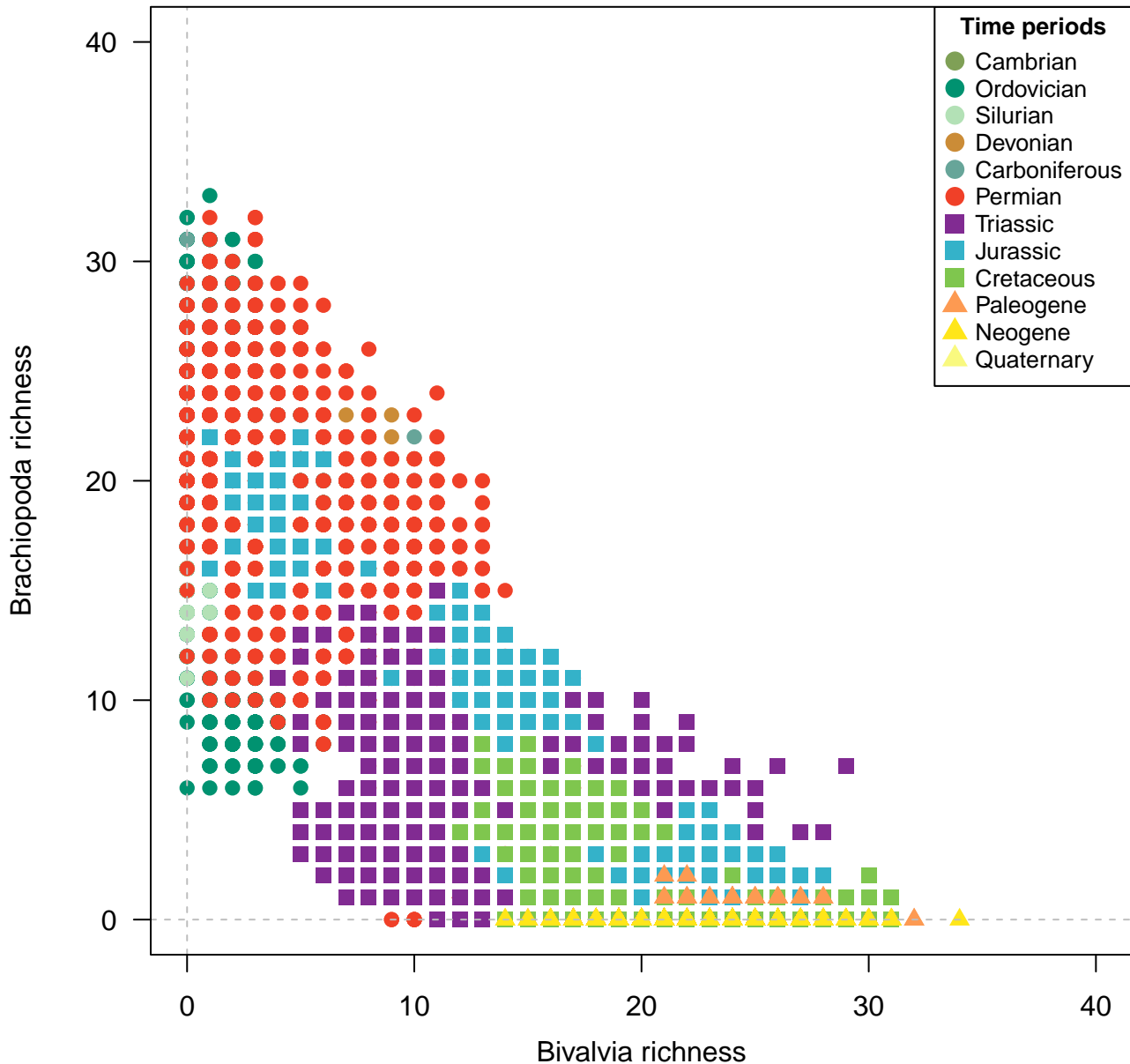
Genera, 200km grid cells, STO rarefaction, 2 site minima, 200km radius, 5900 subsamples
