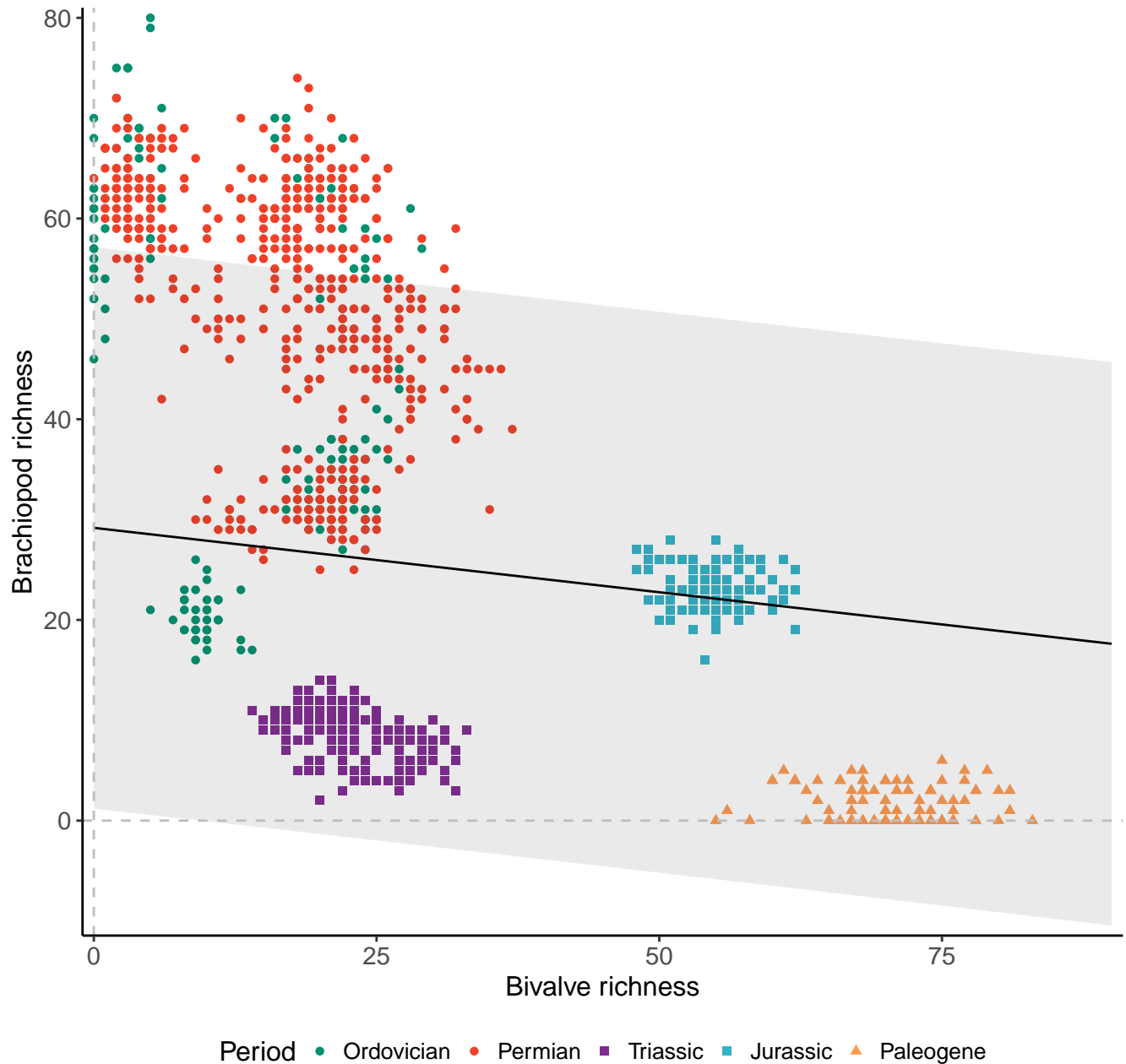
Genera, 200km grid cells, 5 sites, 1000km radius, PTME as RE
