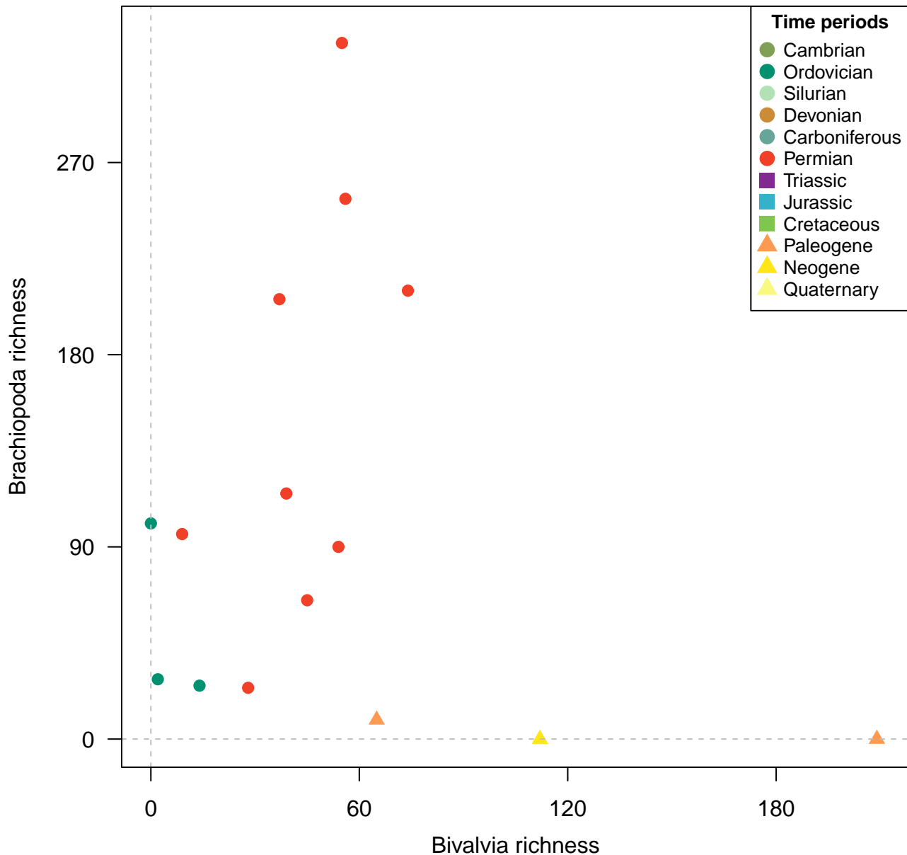
Species, 100km grid cells, raw, 3 site minima, 500km radius, 15 subsamples
