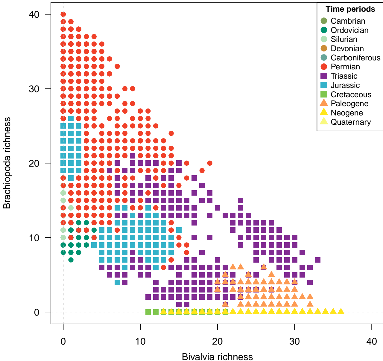
Species, 200km grid cells, STO rarefaction, 2 site minima, 500km radius, 4400 subsamples
