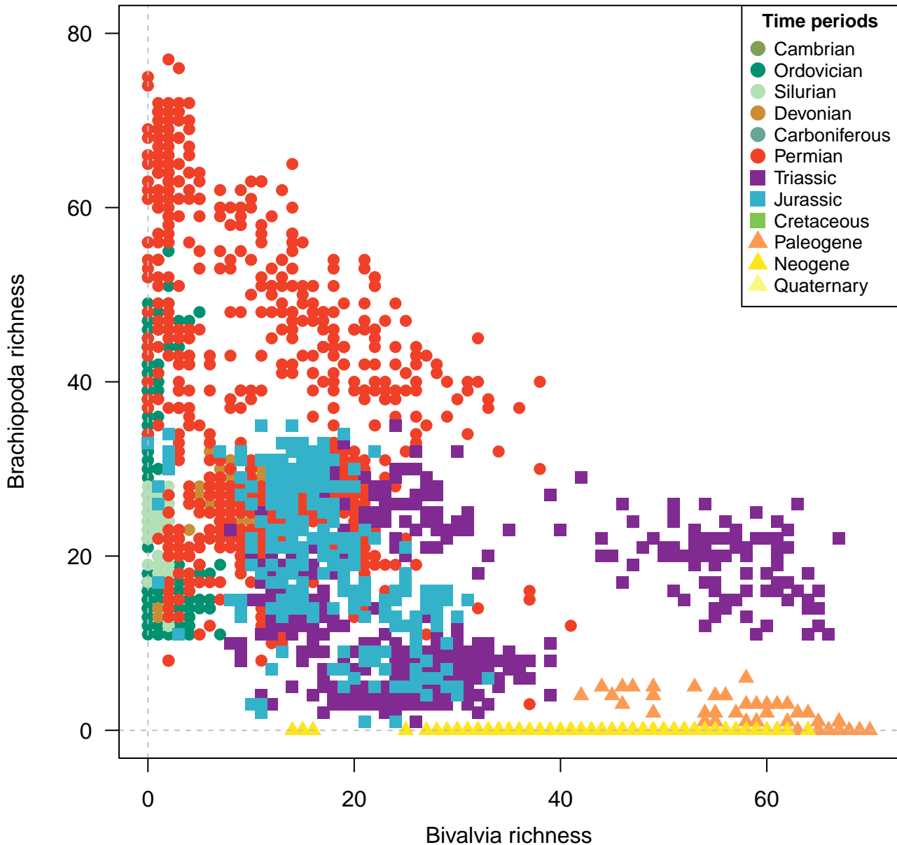
Species, 200km grid cells, STO rarefaction, 3 site minima, 1000km radius, 2500 subsamples
