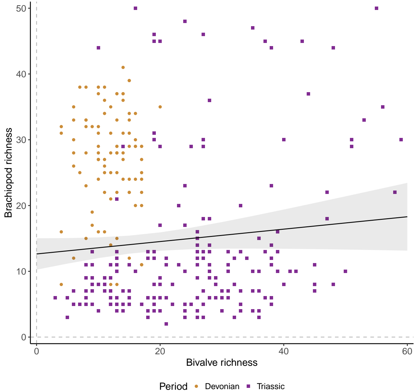
Species, 200km grid cells, 4 sites, 500km radius, full model
