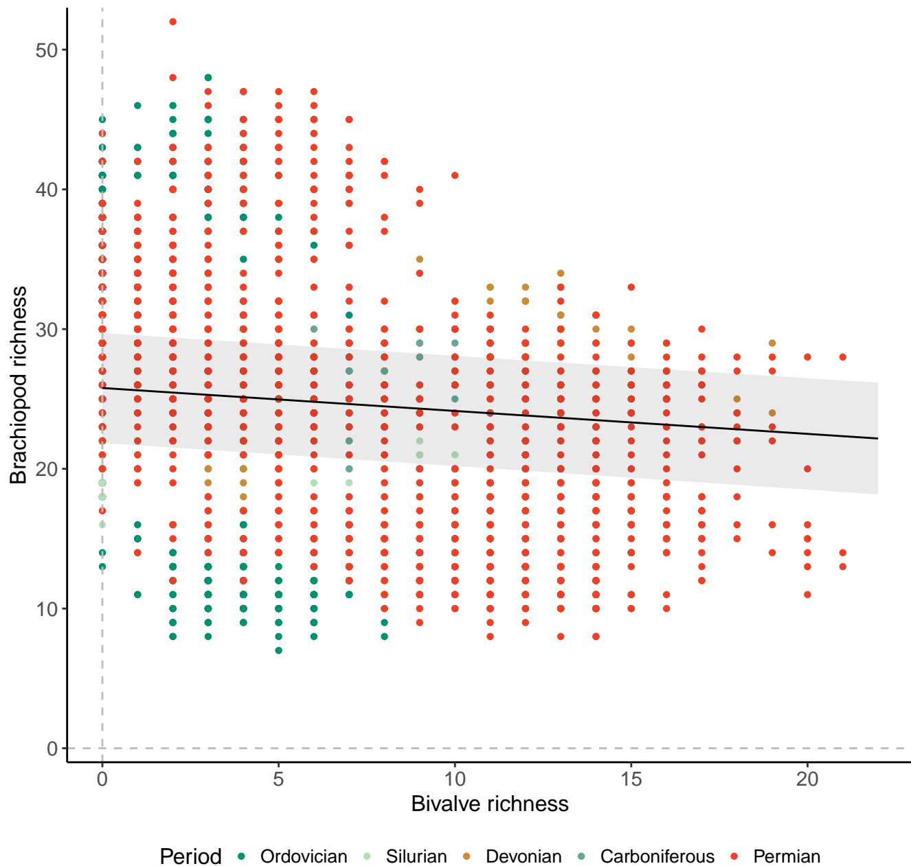
Genera, 200km grid cells, 2 sites, 200km radius, Paleozoic
