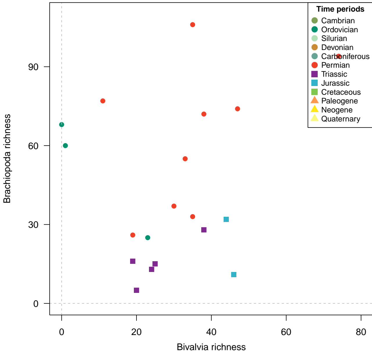
Genera, 200km grid cells, raw, 3 site minima, 200km radius, 19 subsamples
