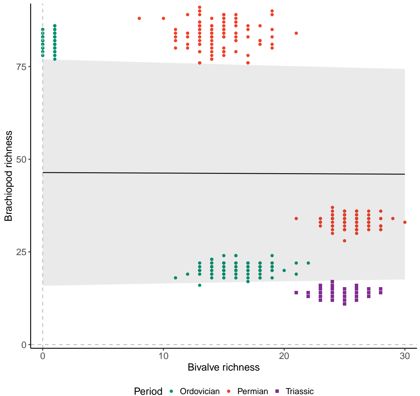
Genera, 200km grid cells, 4 sites, 200km radius
