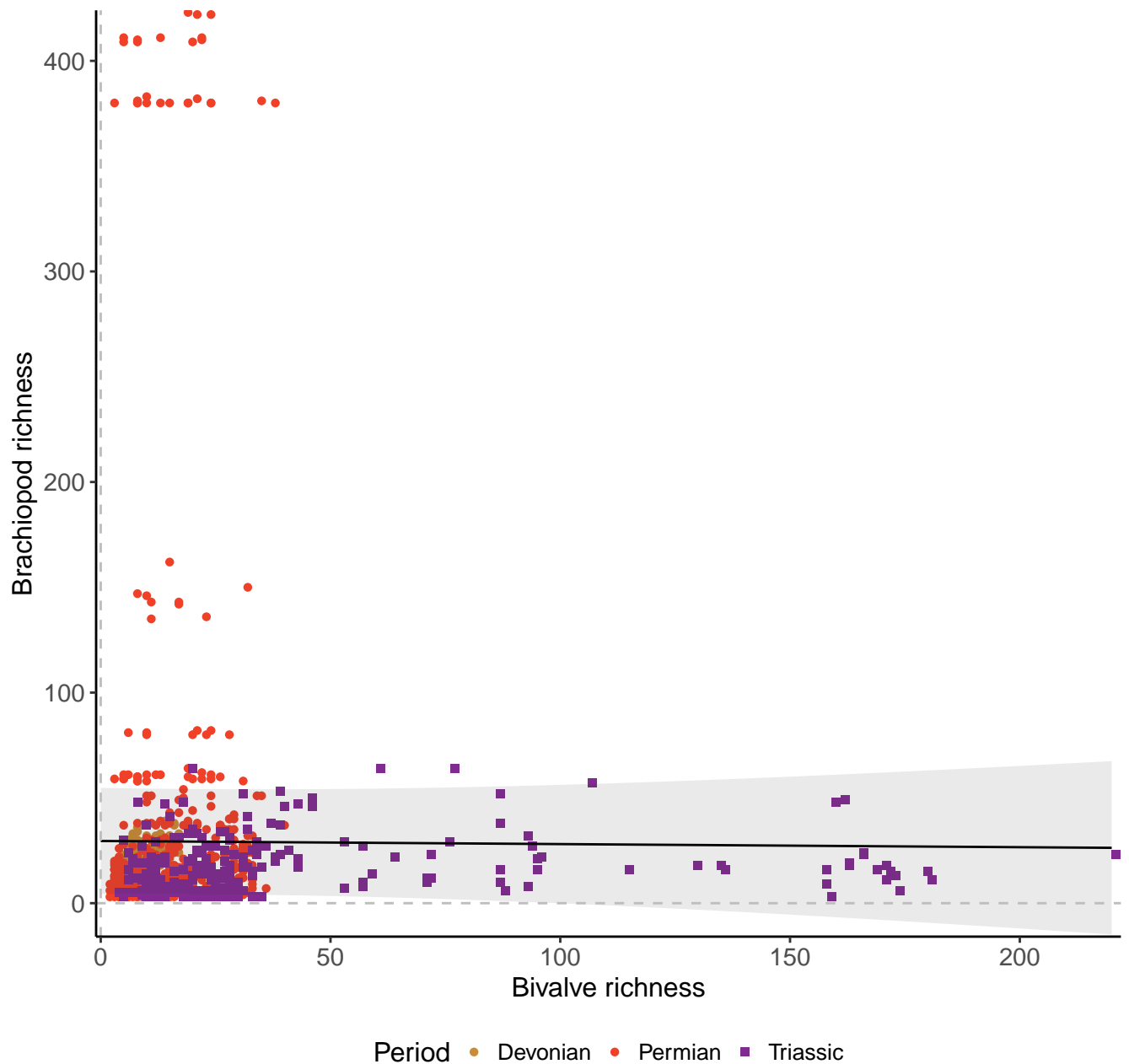
Species, 100km grid cells, 2 sites, 500km radius, simple model
