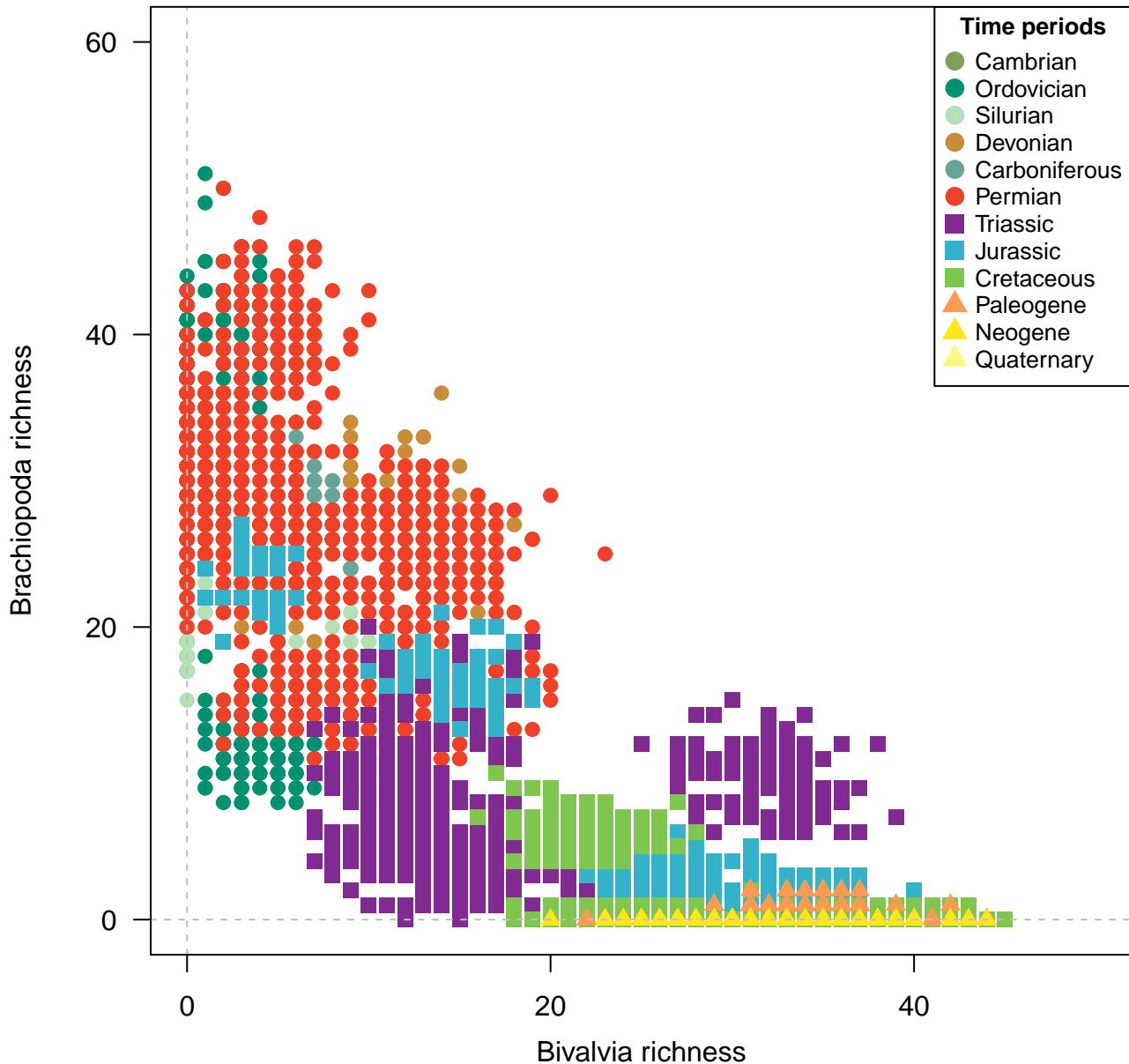
Genera, 200km grid cells, STO rarefaction, 2 site minima, 200km radius, 5100 subsamples
