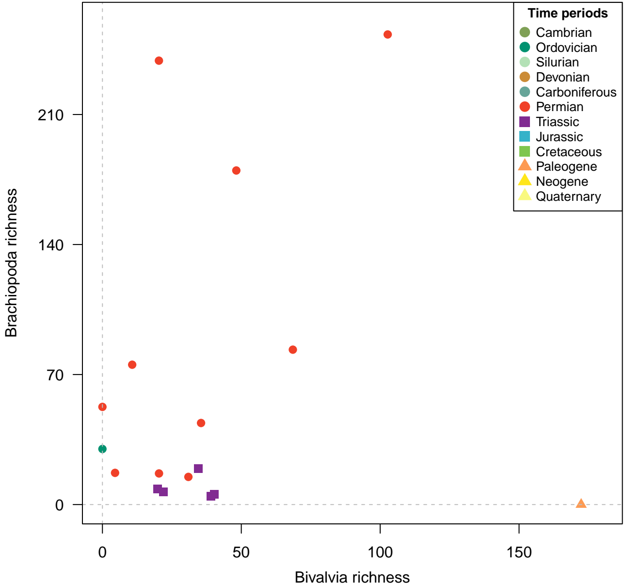
Species, 100km grid cells, SQS ( q = 0.9 ), 2 site minima, 1000km radius, 17 subsamples
