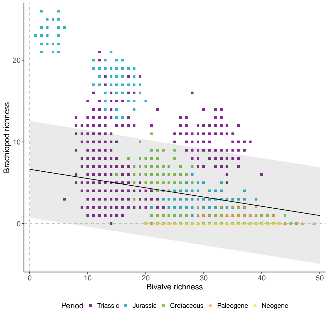
Genera, 200km grid cells, 2 sites, 200km radius, Post-PTME
