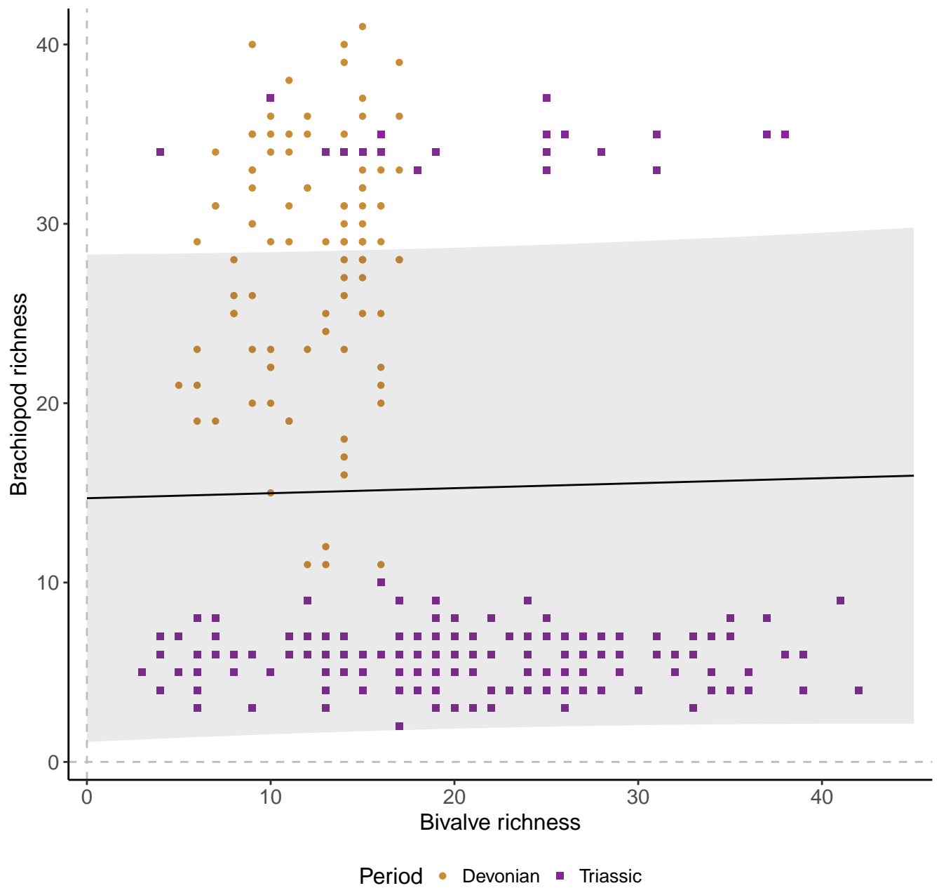
Species, 200km grid cells, 3 sites, 200km radius, simple model
