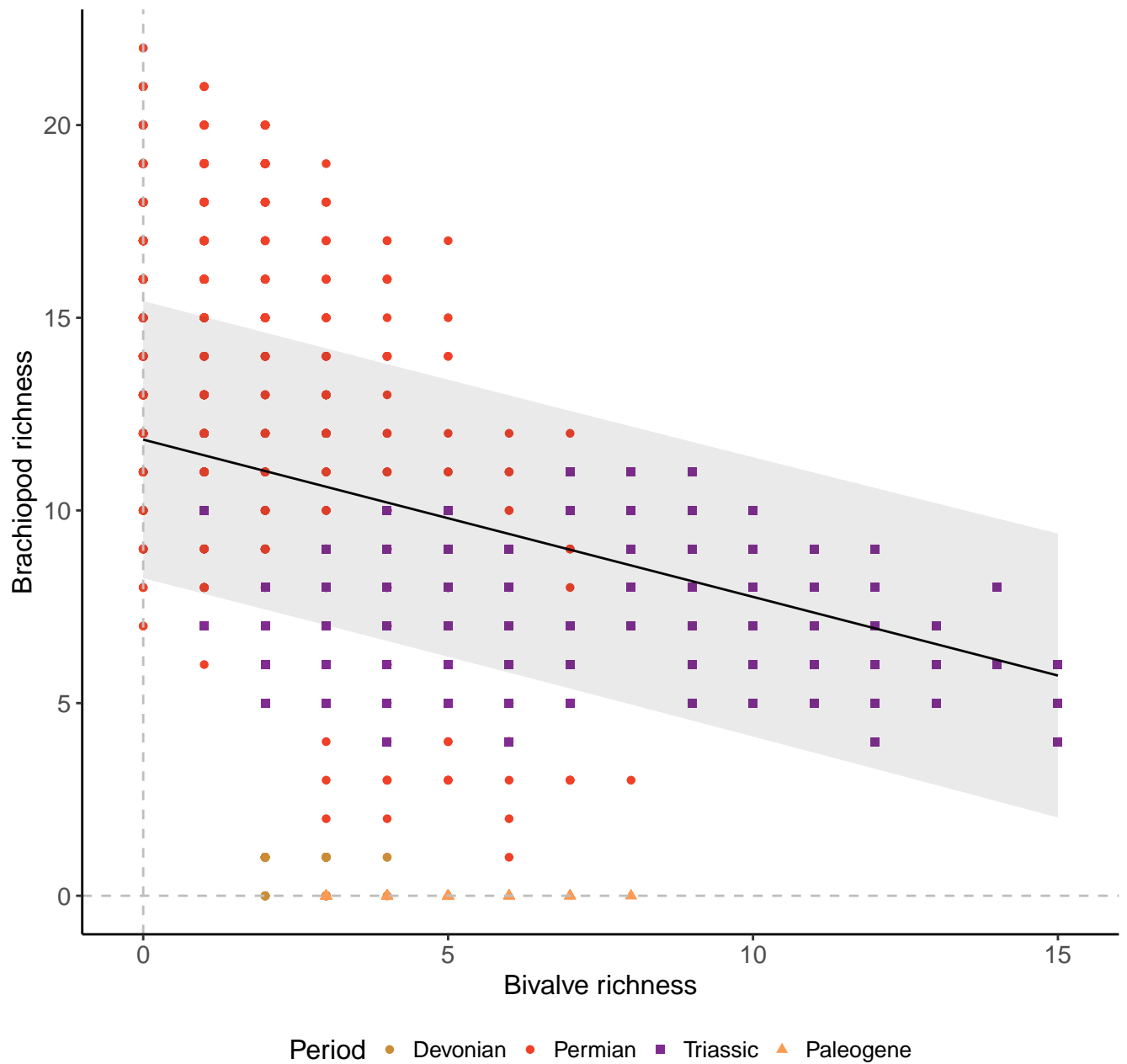
Species, 100km grid cells, 2 sites, 1000km radius, full model
