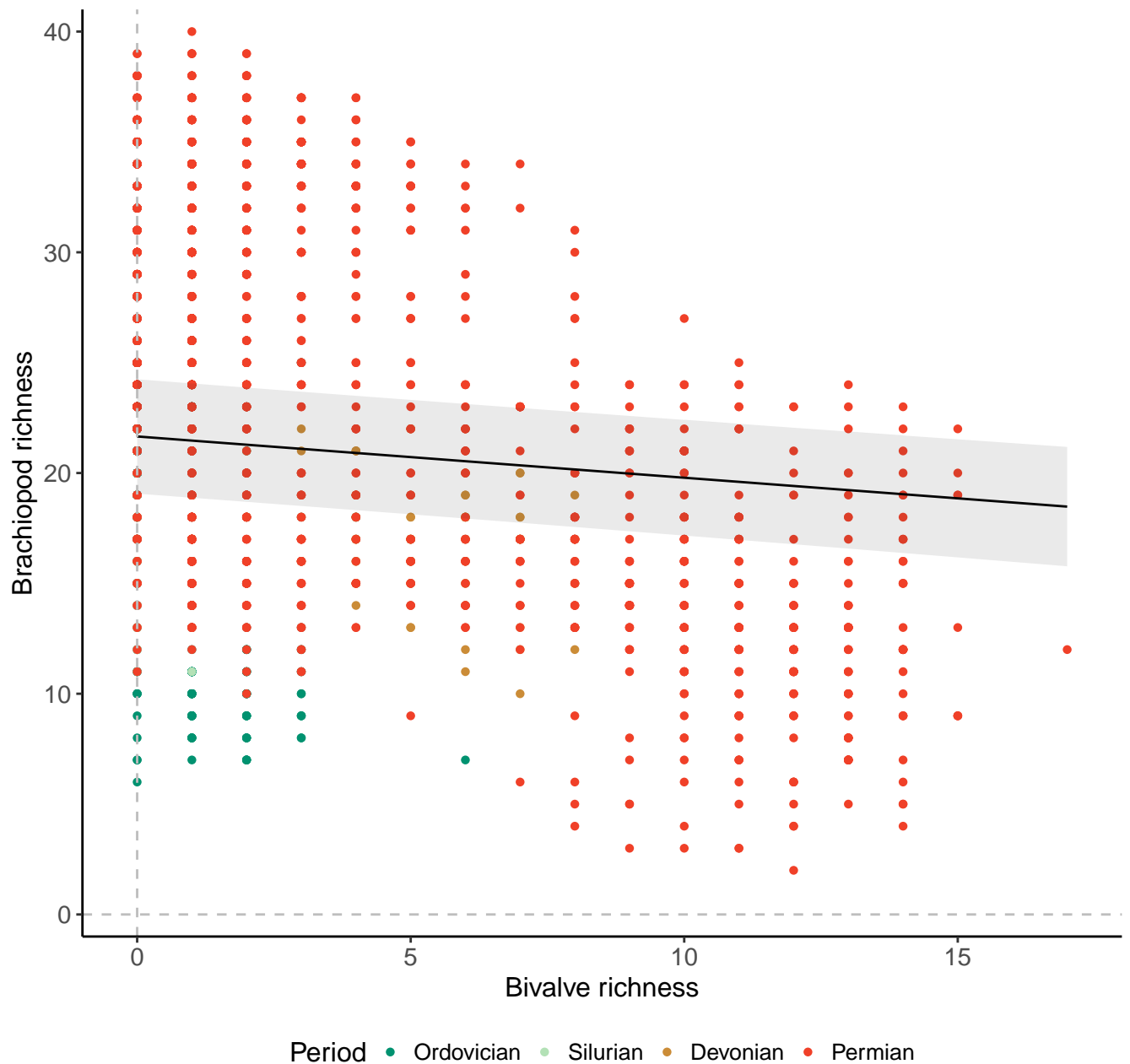
Species, 100km grid cells, 2 sites, 1000km radius, Pre-PTME
