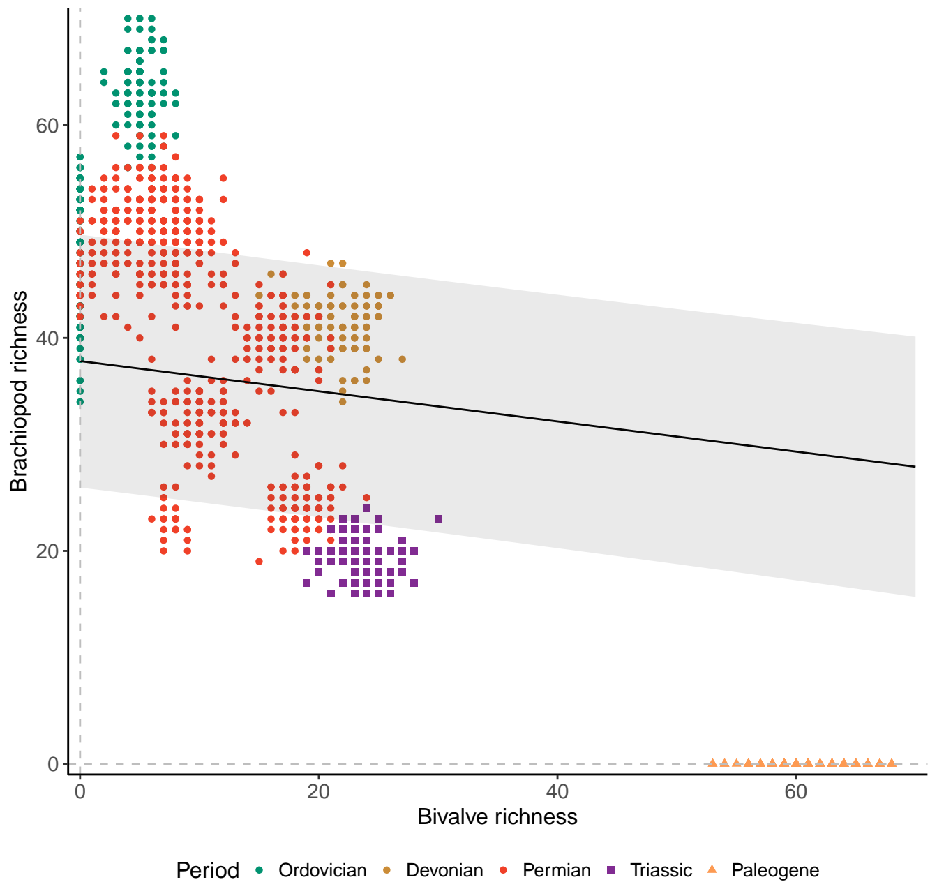
Genera, 100km grid cells, 4 sites, 200km radius, simple model
