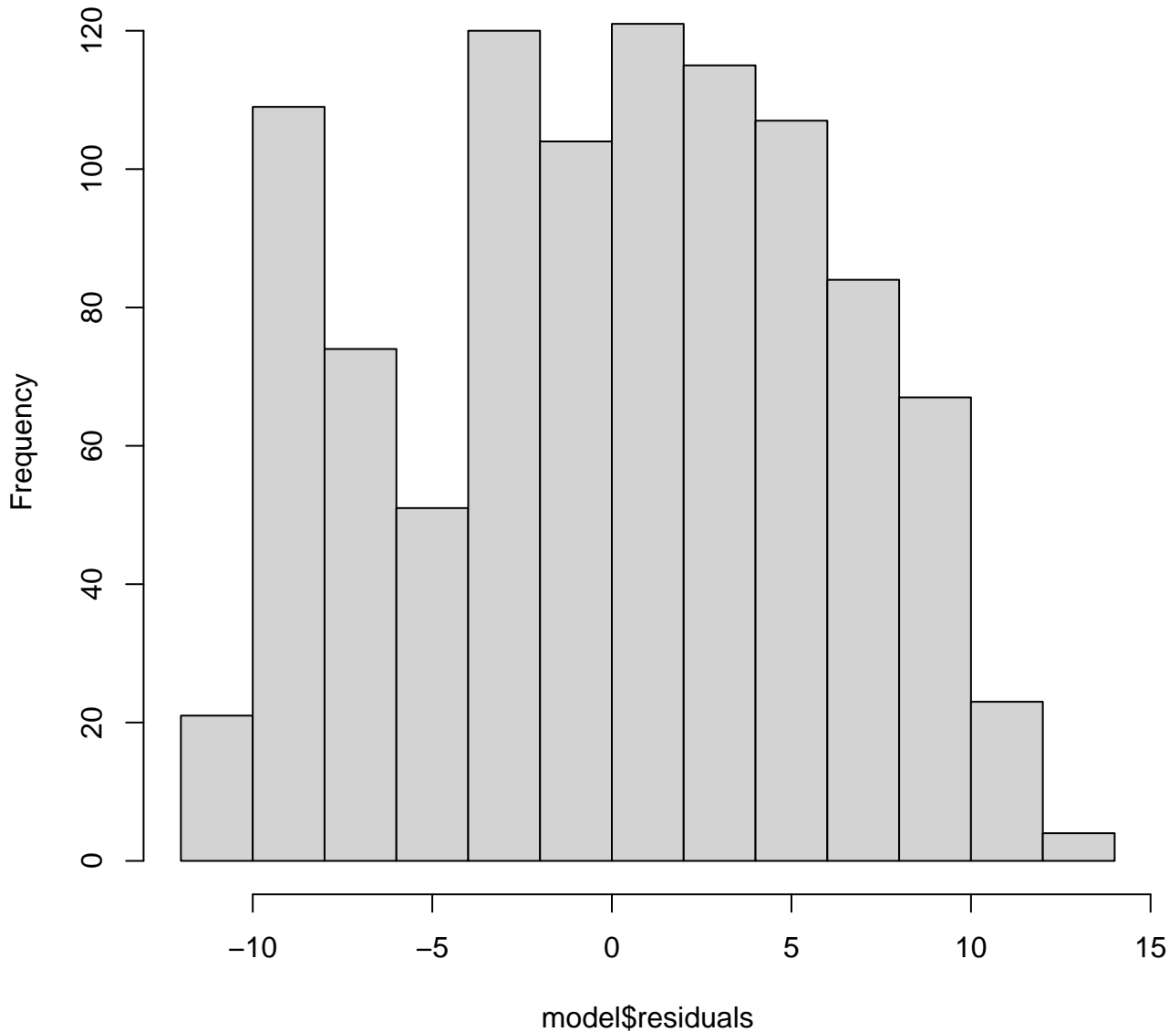
Histogram of model$residuals
