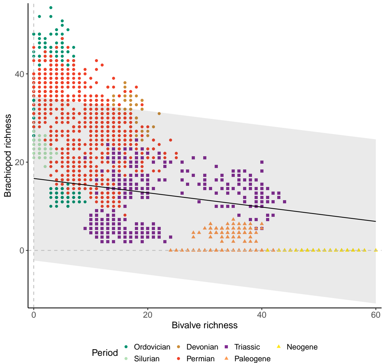
Genera, 100km grid cells, 3 sites, 500km radius, PTME as RE
