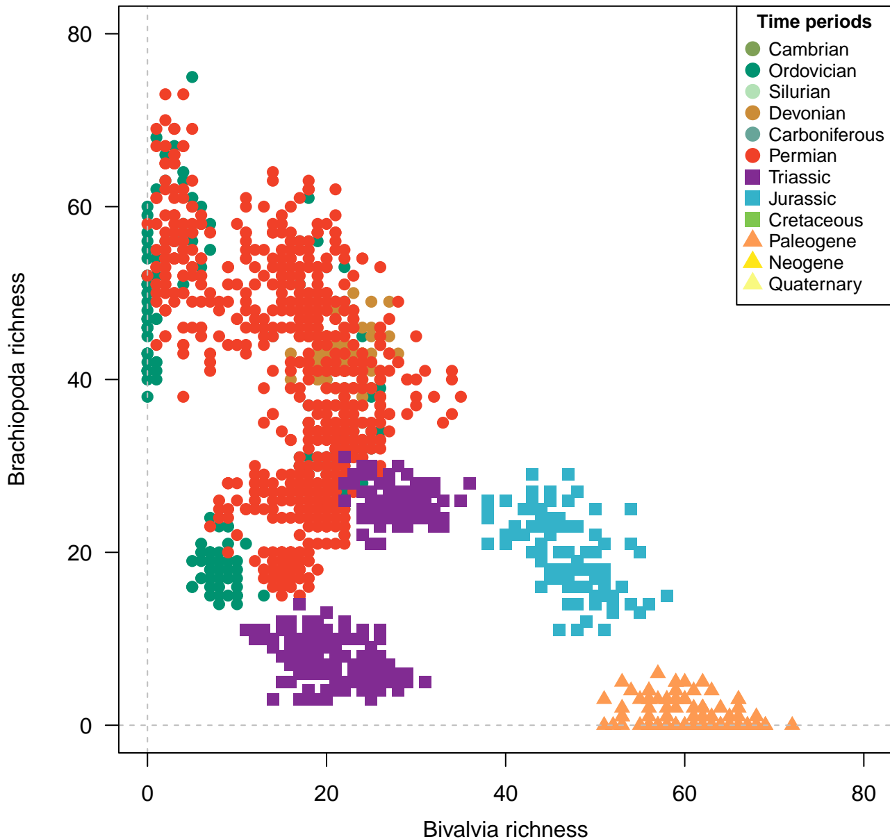
Genera, 200km grid cells, STO rarefaction, 4 site minima, 1000km radius, 1600 subsamples
