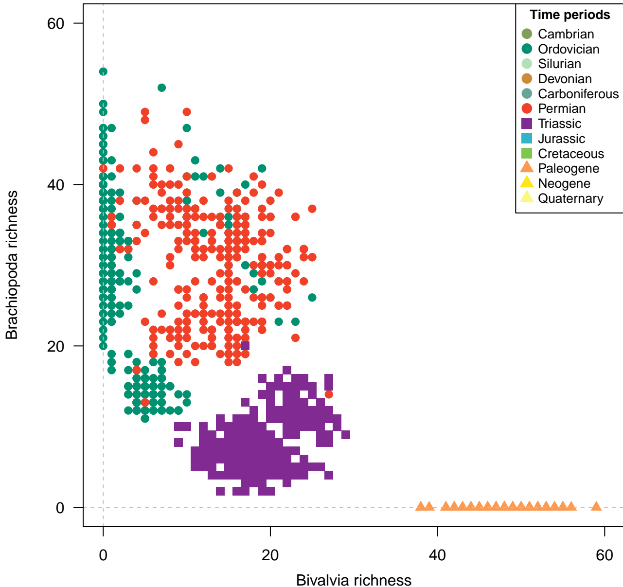
Genera, 200km grid cells, STO rarefaction, 5 site minima, 500km radius, 1100 subsamples
