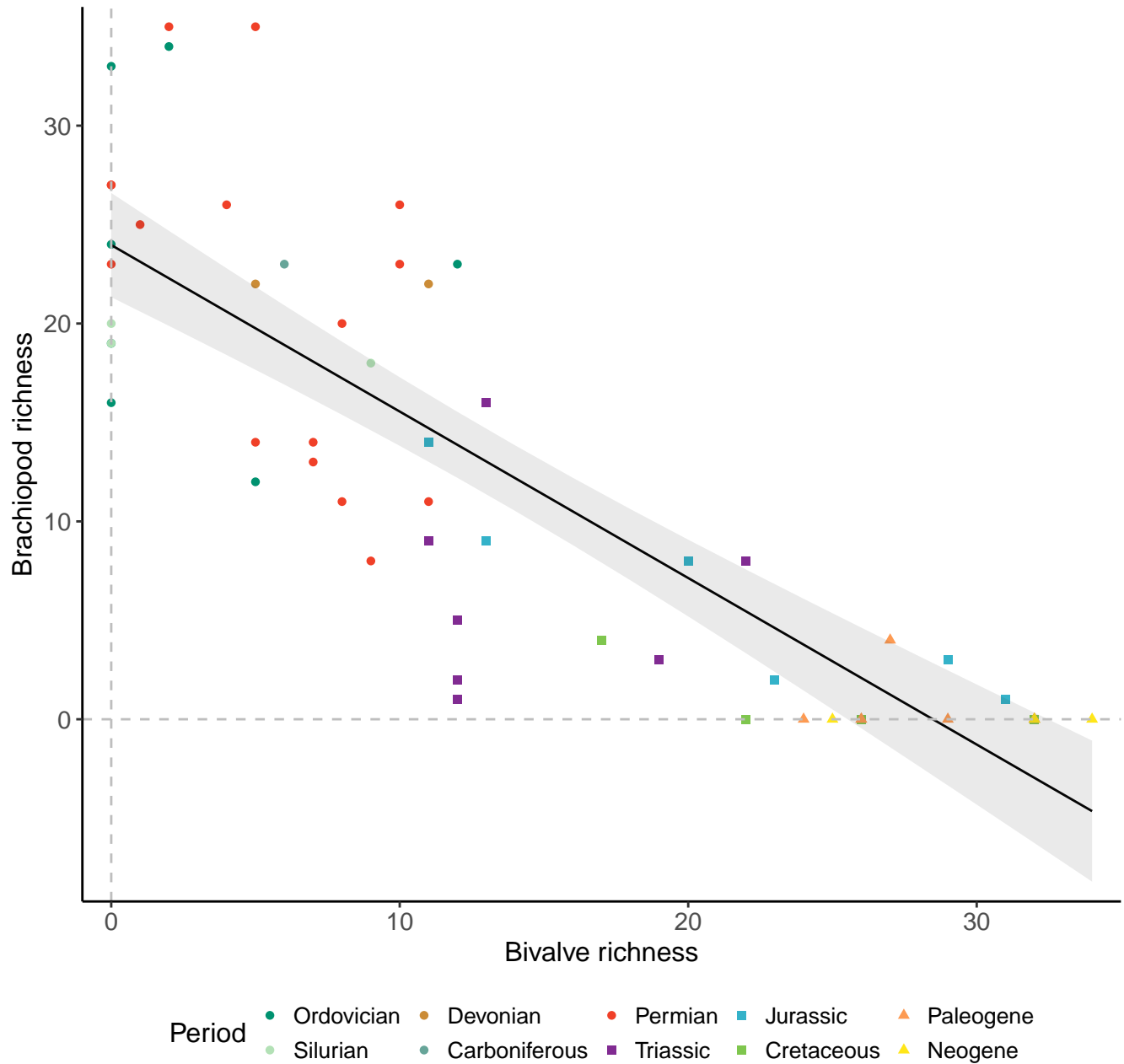
Genera, 200km grid cells, 2 sites, 500km radius, median richness
