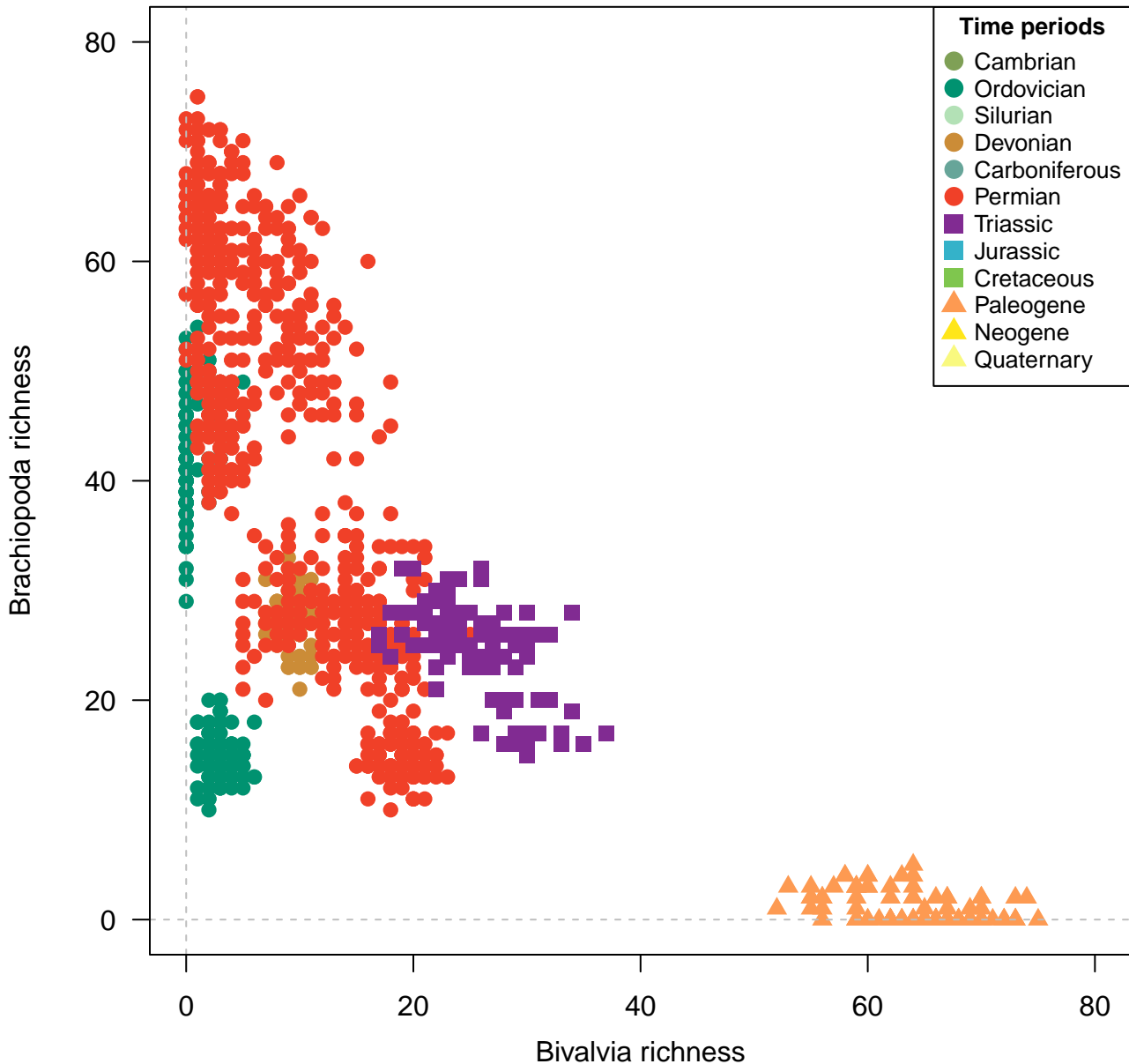
Species, 100km grid cells, STO rarefaction, 4 site minima, 1000km radius, 1200 subsamples
