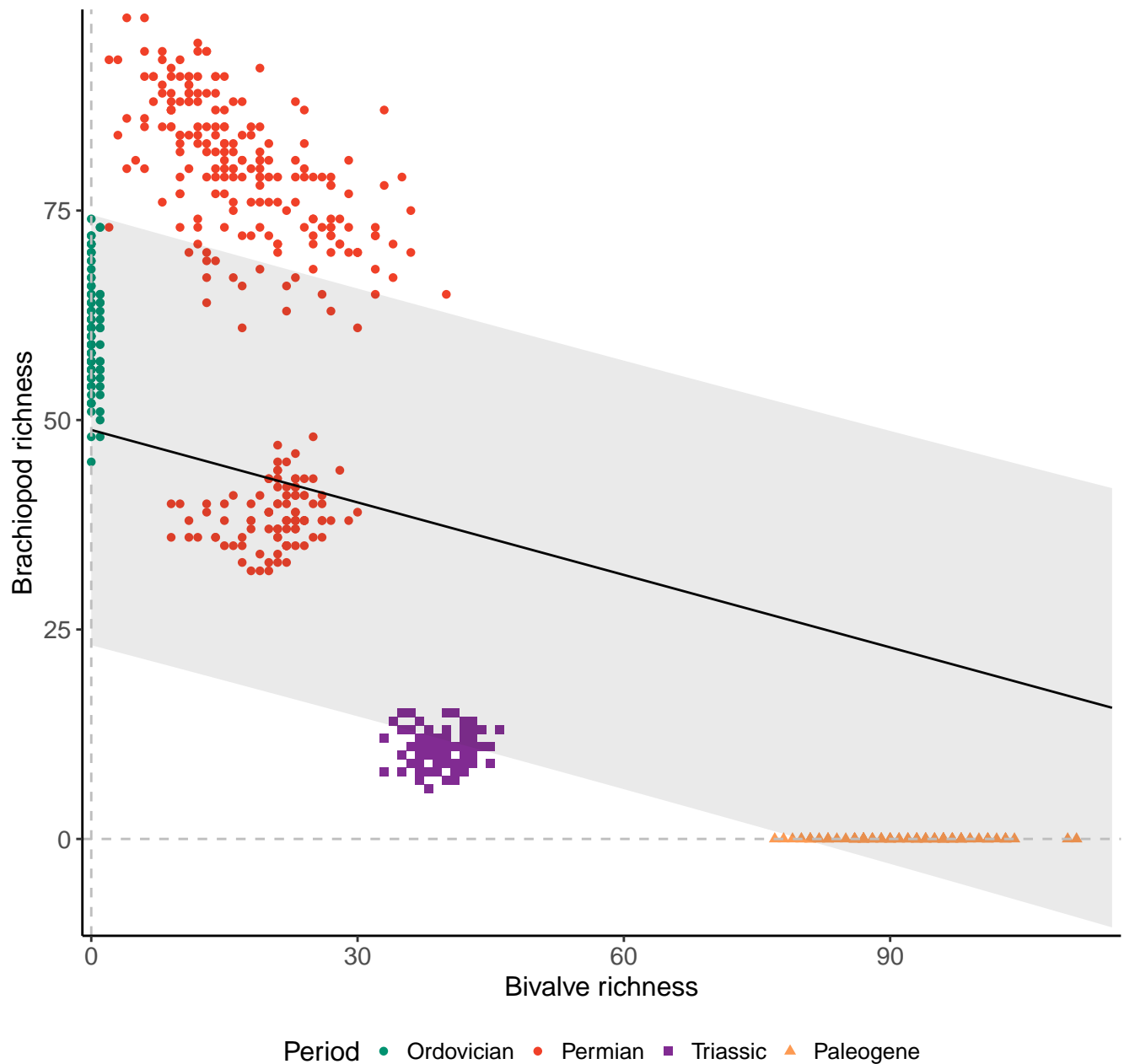
Species, 200km grid cells, 5 sites, 500km radius, full model
