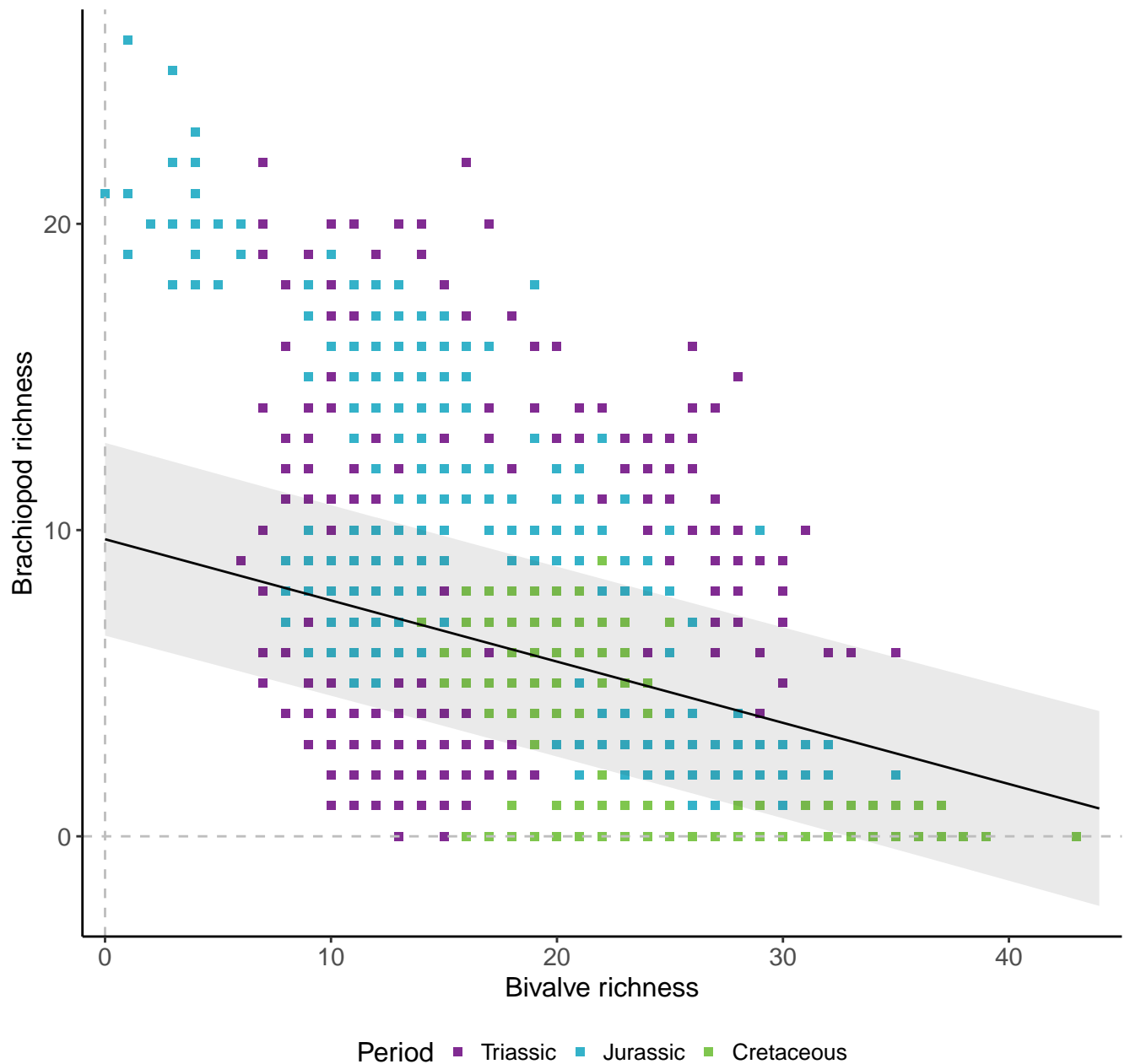
Genera, 200km grid cells, 2 sites, 500km radius, Mesozoic
