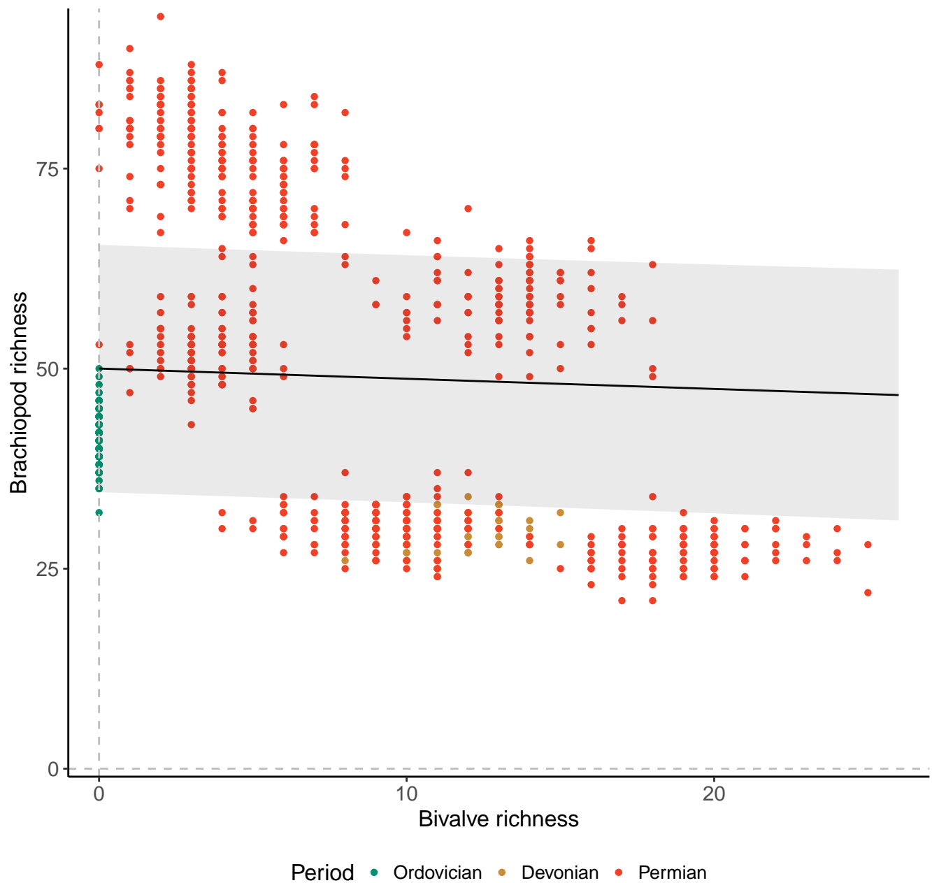
Species, 100km grid cells, 4 sites, 200km radius, Pre-PTME
