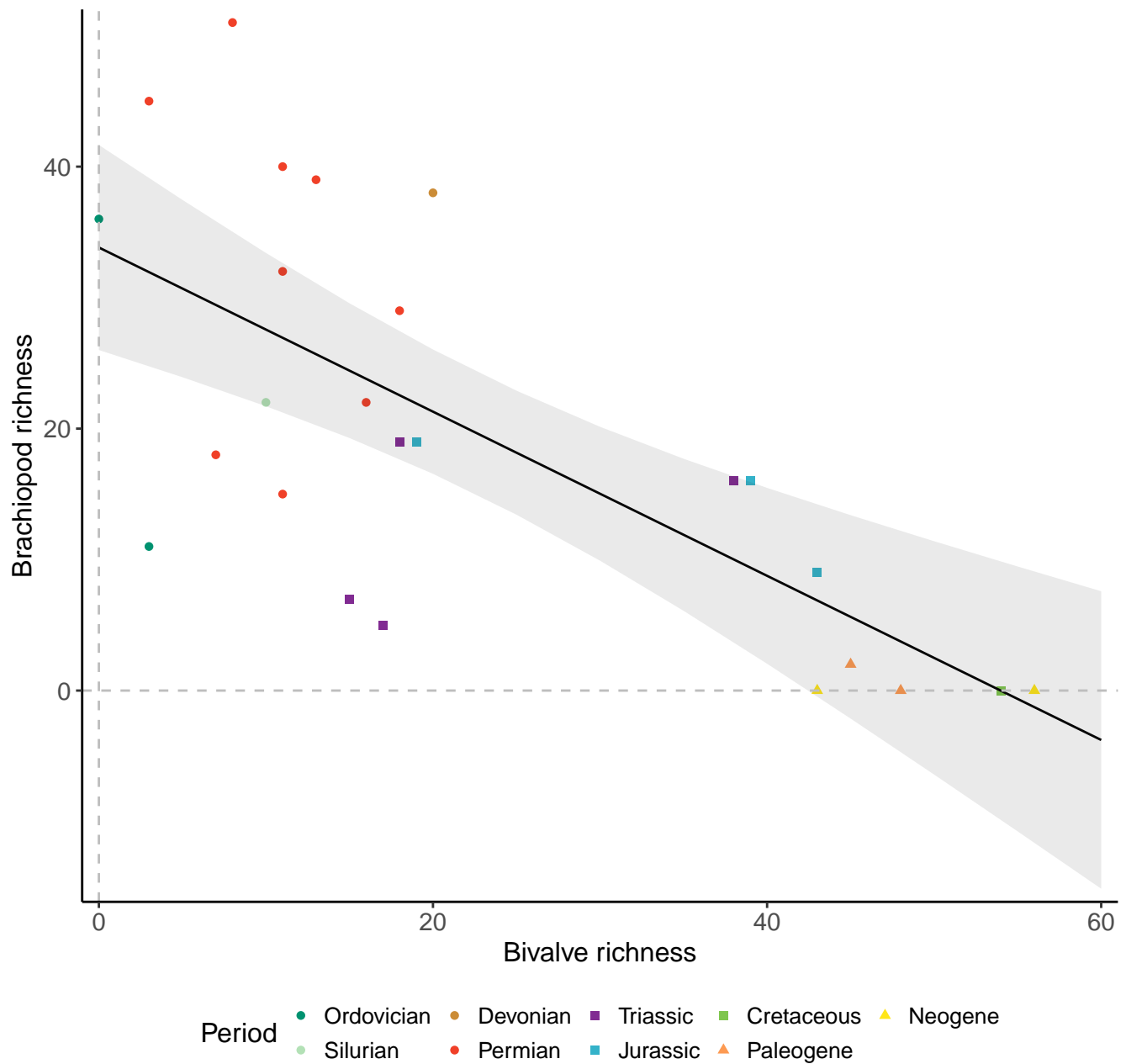
Genera, 200km grid cells, 3 sites, 1000km radius, median richness
