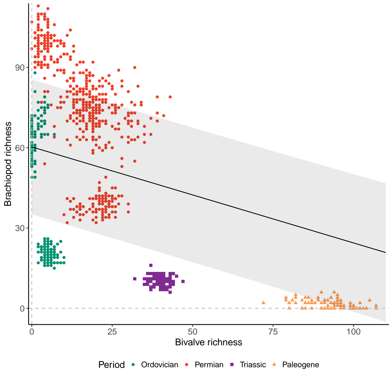
Species, 200km grid cells, 5 sites, 1000km radius, full model
