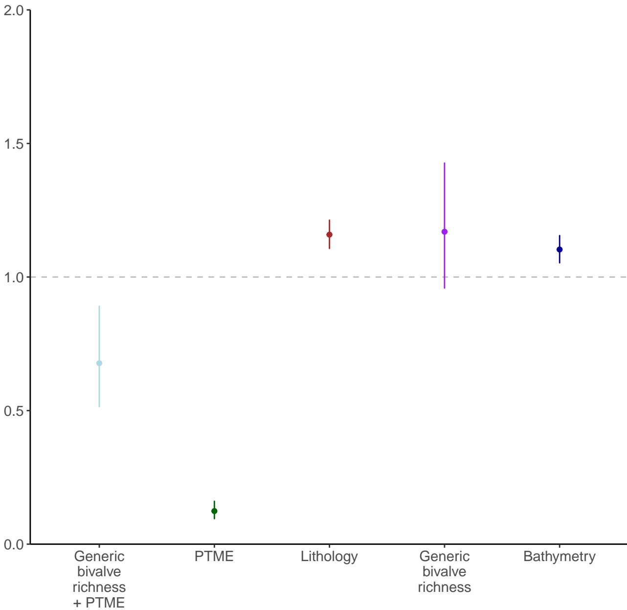
Model coefficients
