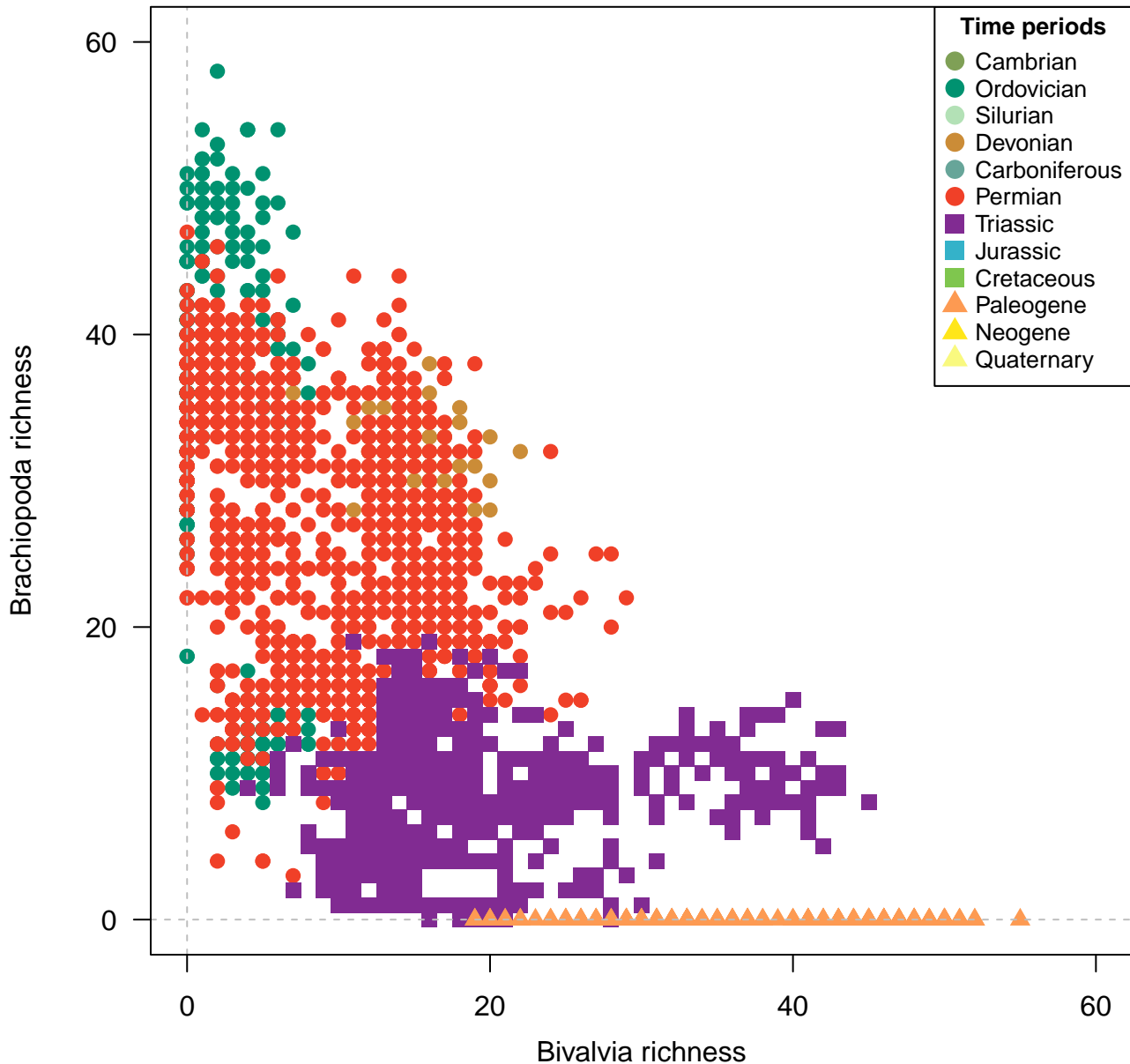
Genera, 100km grid cells, STO rarefaction, 3 site minima, 200km radius, 2500 subsamples
