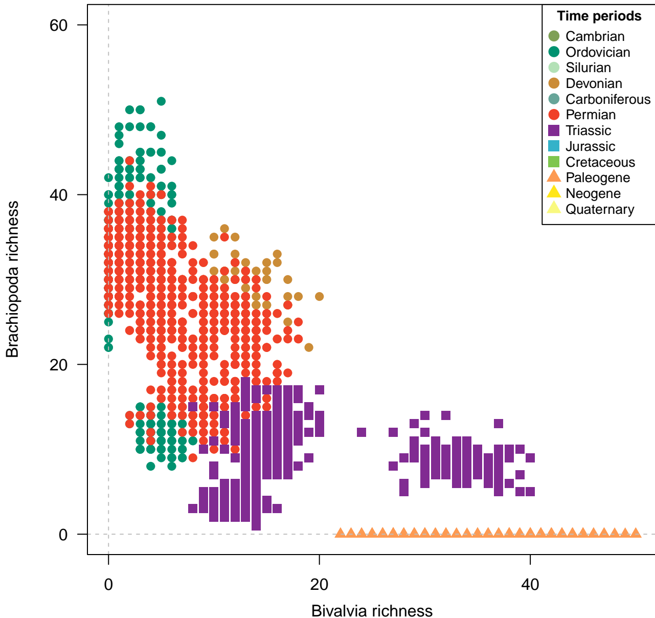
Genera, 100km grid cells, STO rarefaction, 3 site minima, 200km radius, 1900 subsamples
