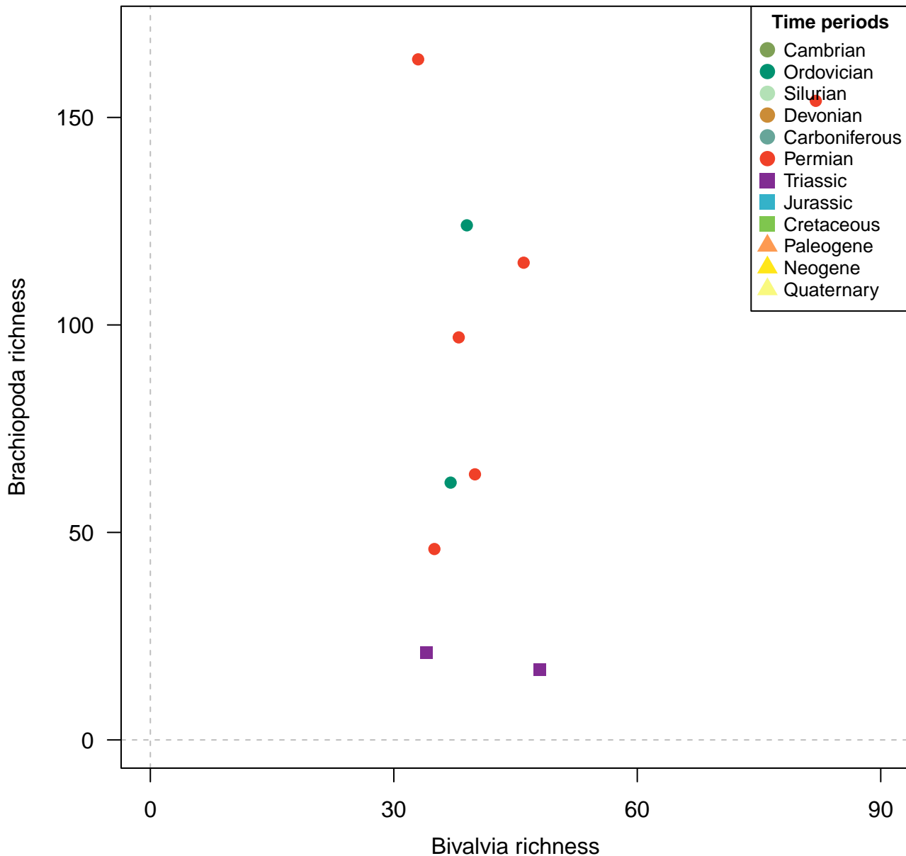
Genera, 200km grid cells, raw, 5 site minima, 1000km radius, 10 subsamples
