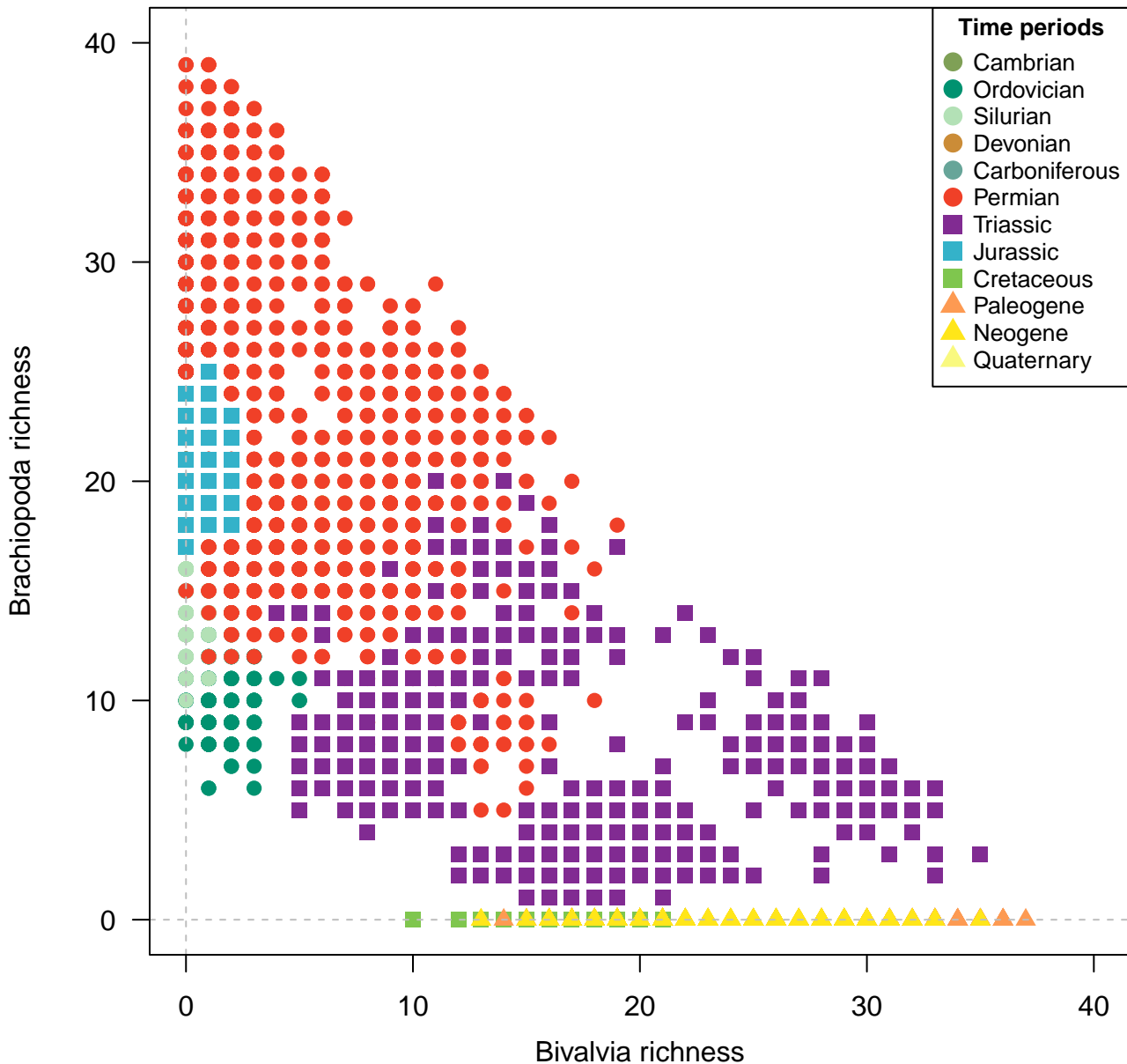
Species, 200km grid cells, STO rarefaction, 2 site minima, 200km radius, 3800 subsamples
