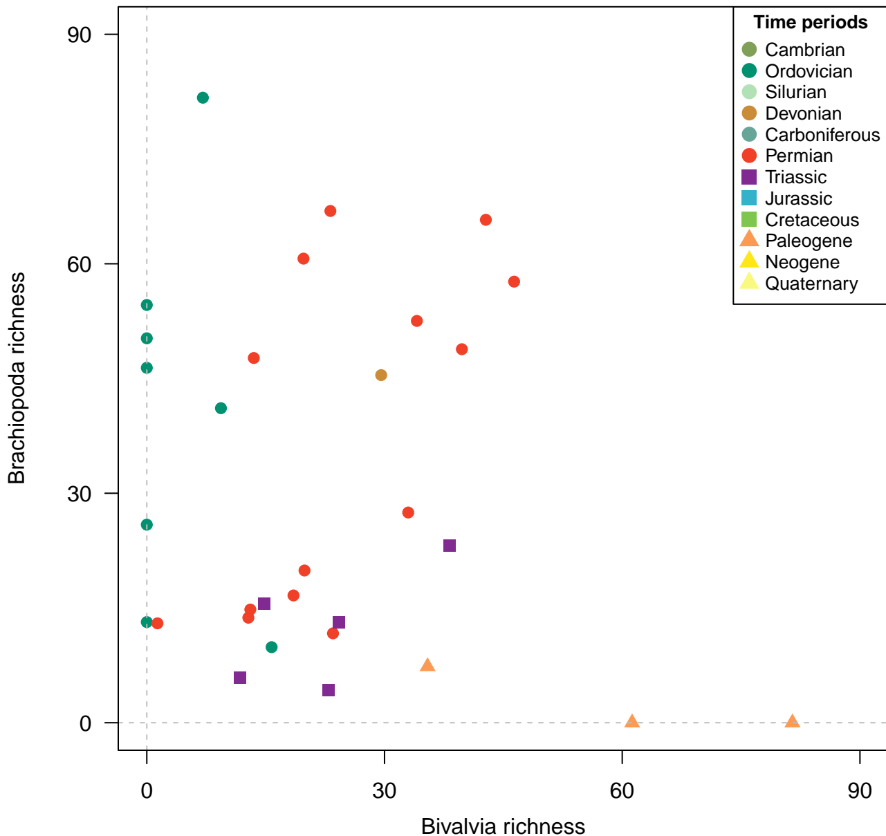
Genera, 100km grid cells, SQS (q = 0.9), 2 site minima, 200km radius, 32 subsamples
