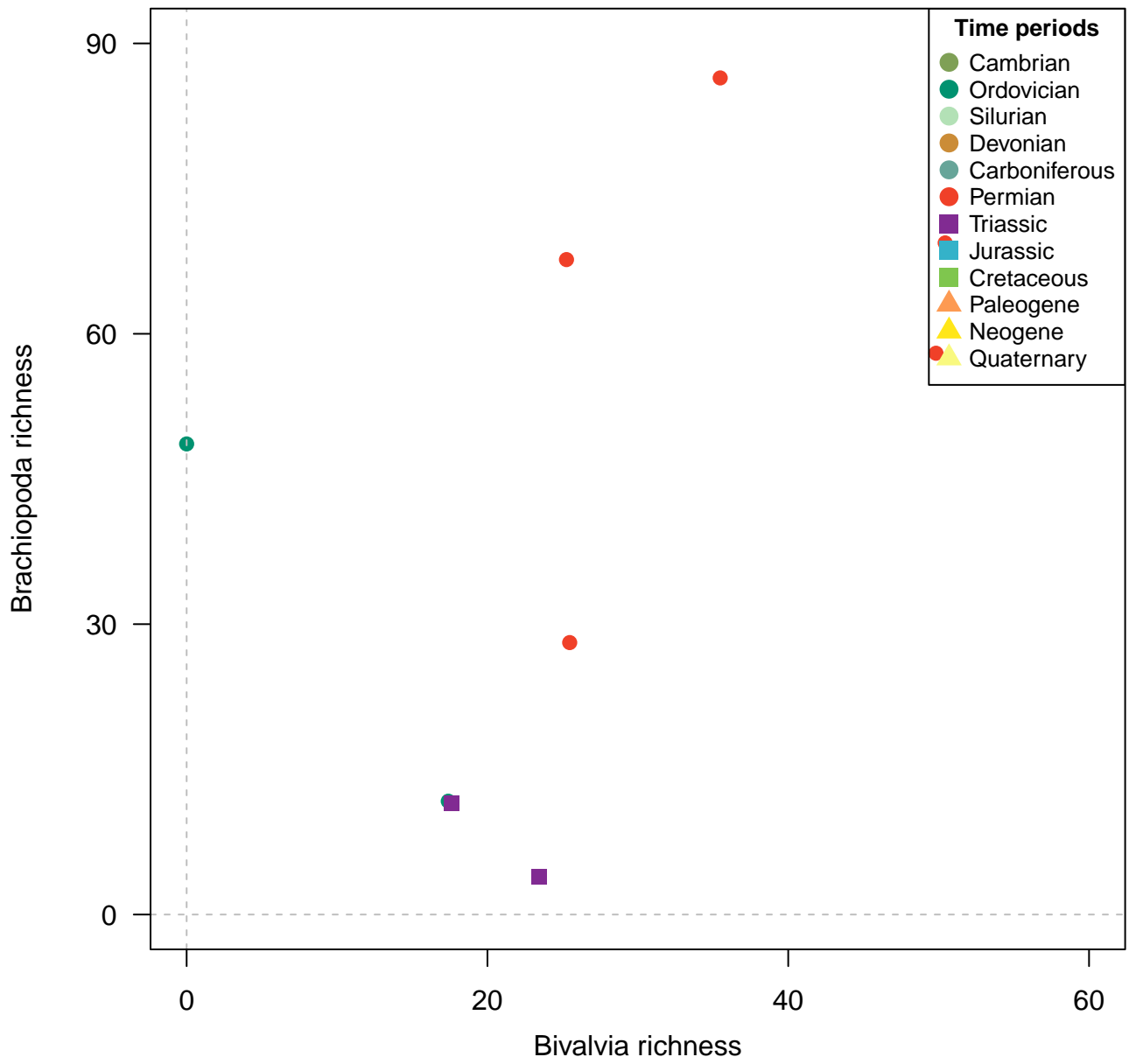
Genera, 200km grid cells, SQS (q = 0.9), 5 site minima, 500km radius, 9 subsamples
