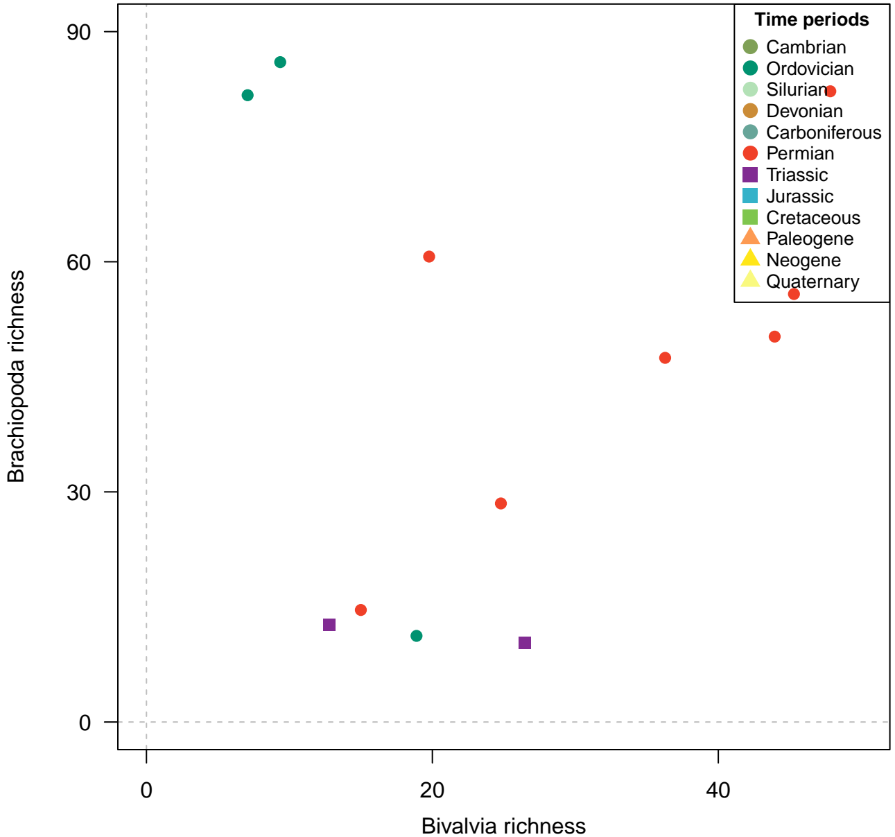
Genera, 100km grid cells, SQS (q = 0.9), 4 site minima, 1000km radius, 12 subsamples
