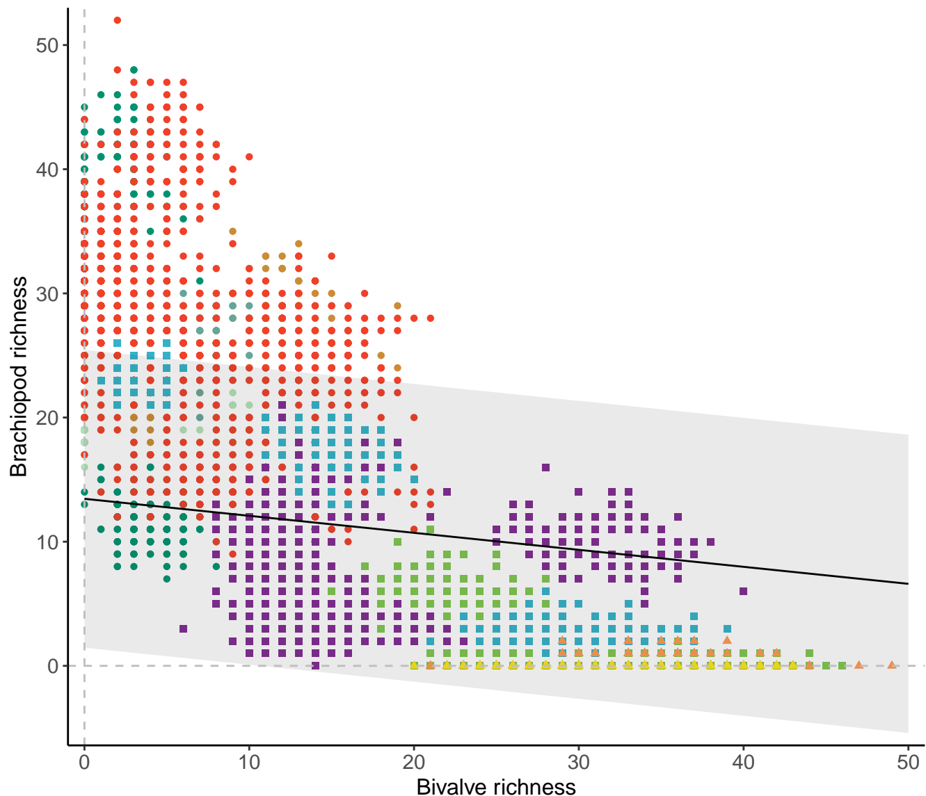
Genera, 200km grid cells, 2 sites, 200km radius, eras as RE
