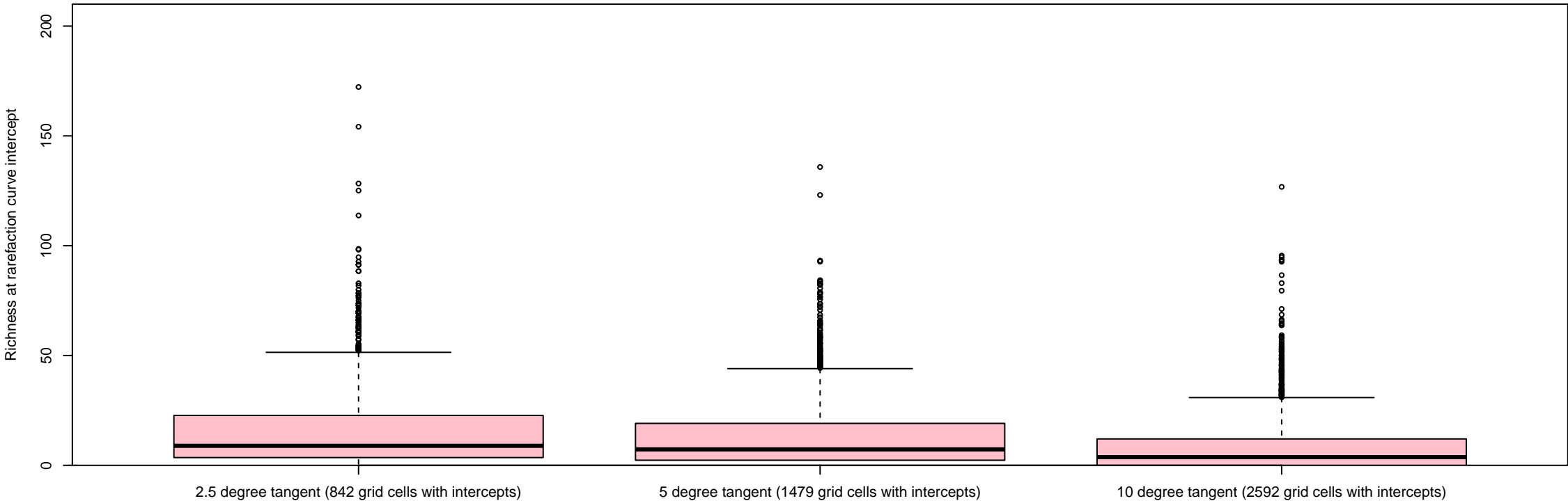
Richness at rarefaction curve intercept for 100km grid cells
