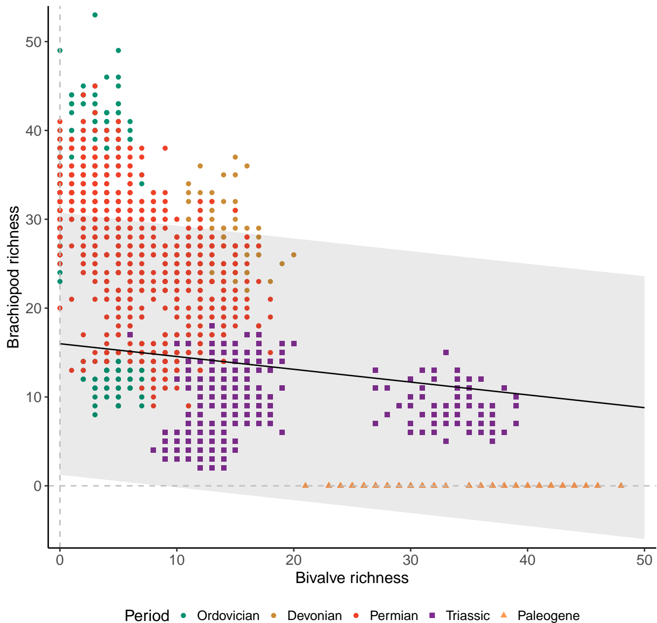
Genera, 100km grid cells, 3 sites, 200km radius, eras as RE
