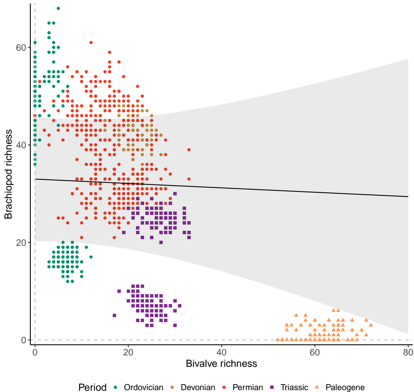
Genera, 100km grid cells, 5 sites, 1000km radius
