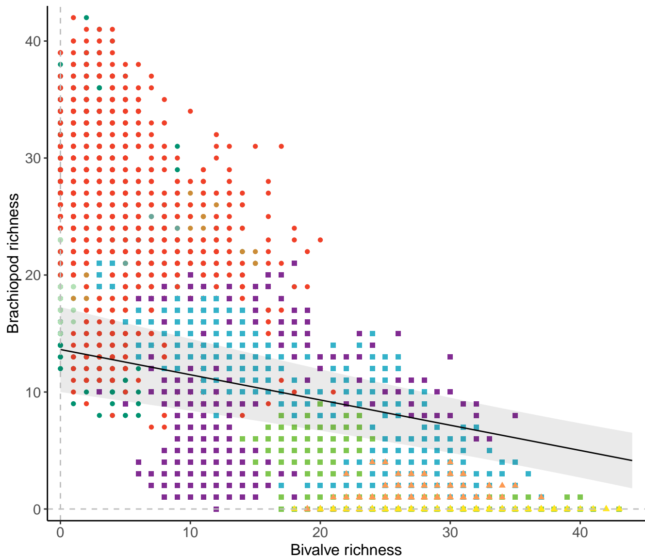
Genera, 200km grid cells, 2 sites, 1000km radius
