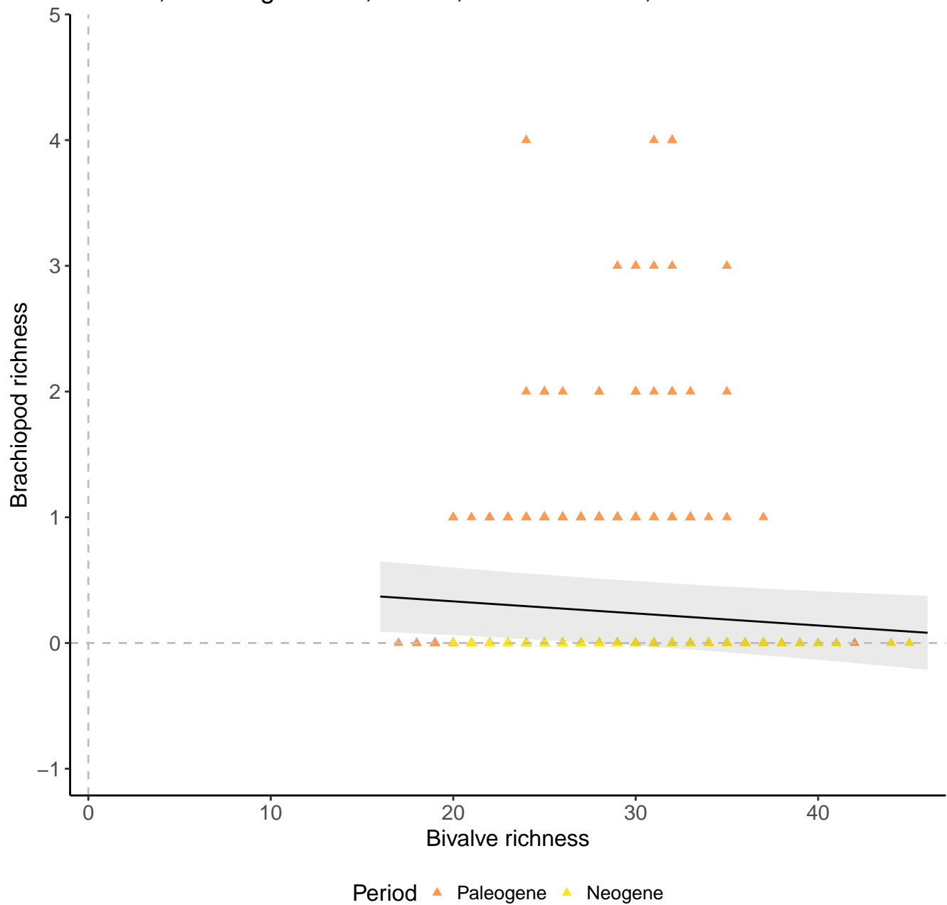
Genera, 200km grid cells, 2 sites, 1000km radius, Cenozoic
