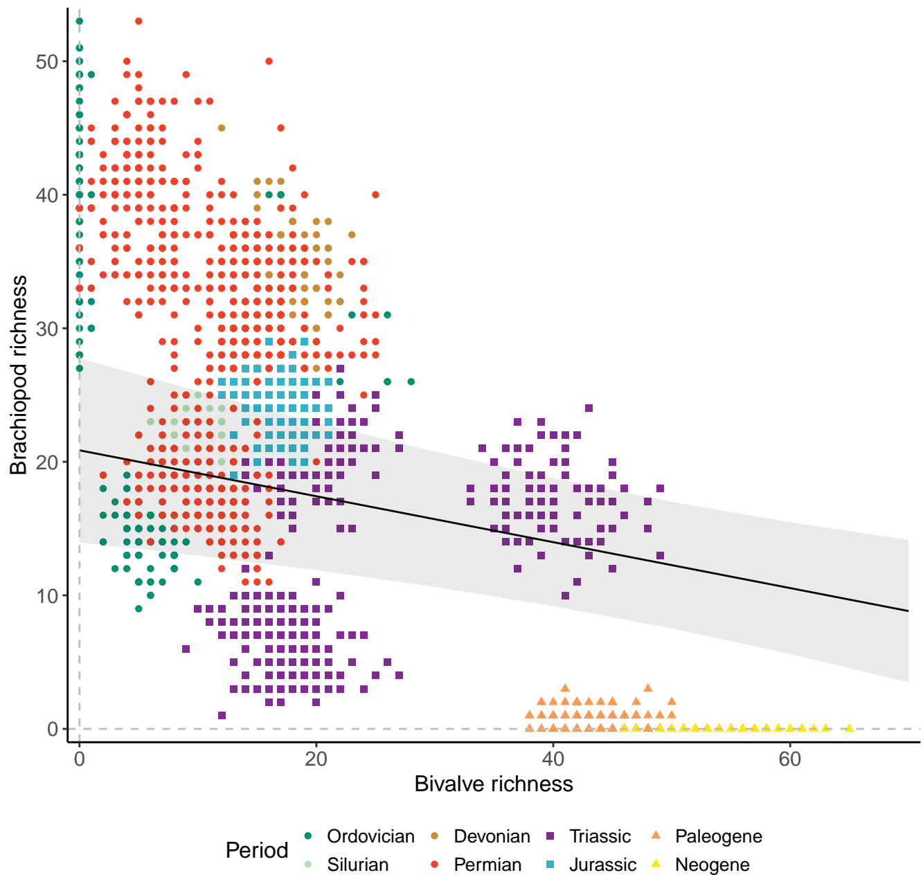
Genera, 200km grid cells, 3 sites, 500km radius
