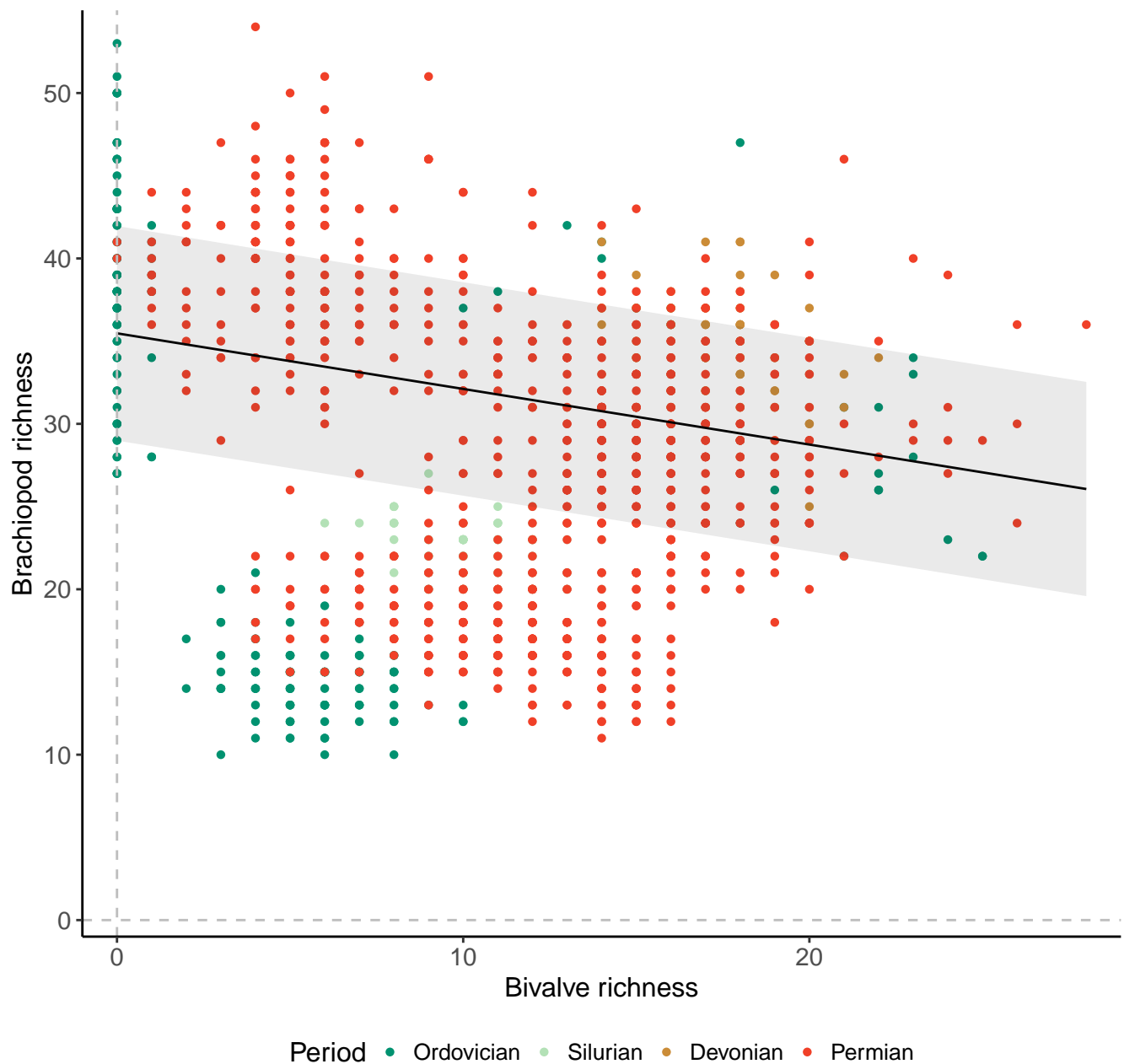
Genera, 200km grid cells, 3 sites, 500km radius, Pre-PTME
