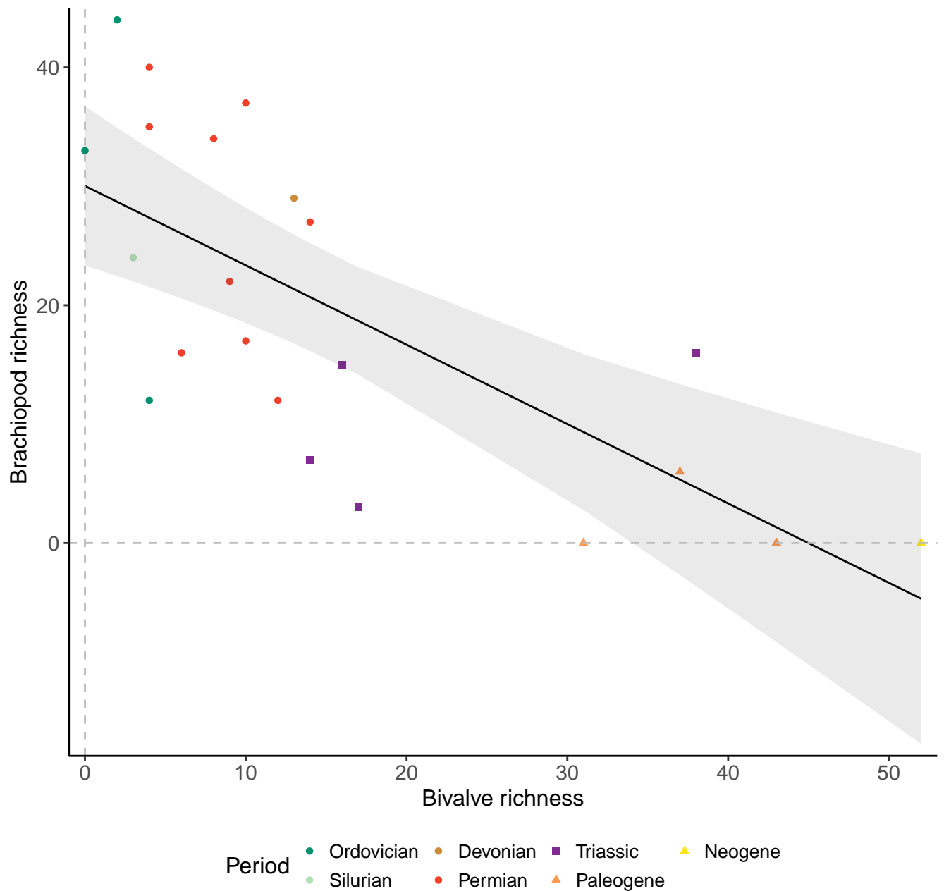
Genera, 100km grid cells, 3 sites, 500km radius, median richness
