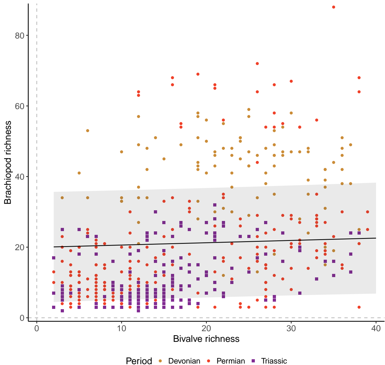
Genera, 100km grid cells, 4 sites, 500km radius, full model
