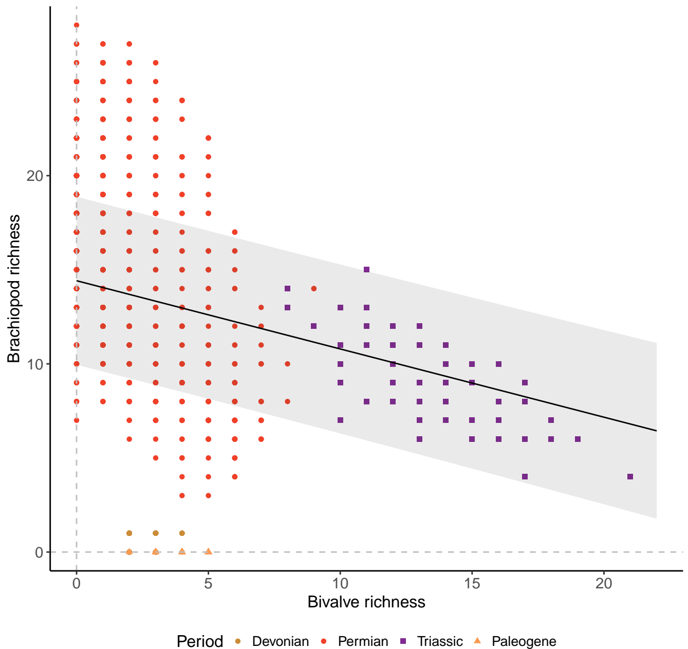
Species, 100km grid cells, 2 sites, 500km radius, full model
