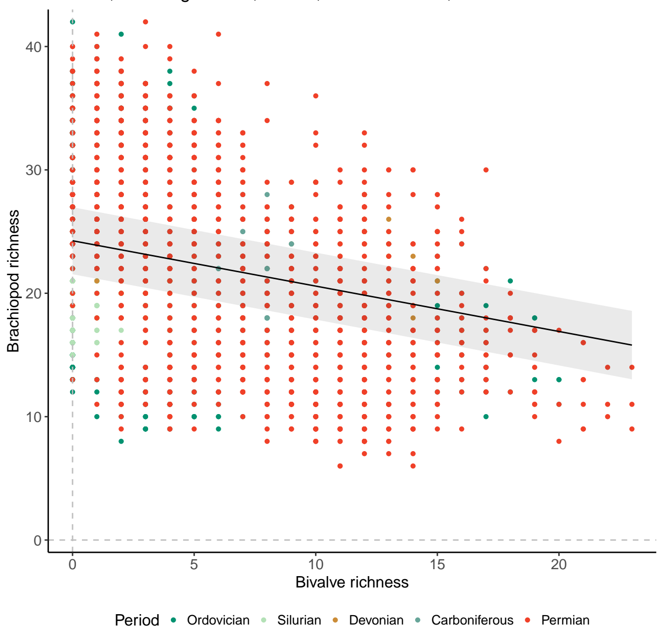
Genera, 200km grid cells, 2 sites, 1000km radius, Pre-PTME
