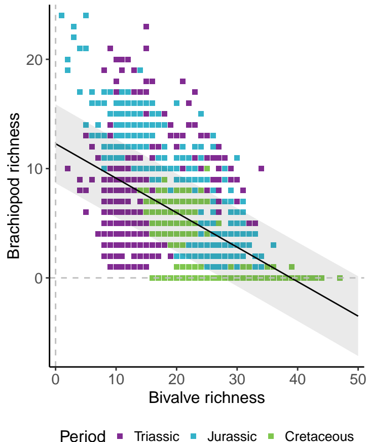
A Genera, 200km grid cells, 2 sites, 1000km radius, Mesozoic
