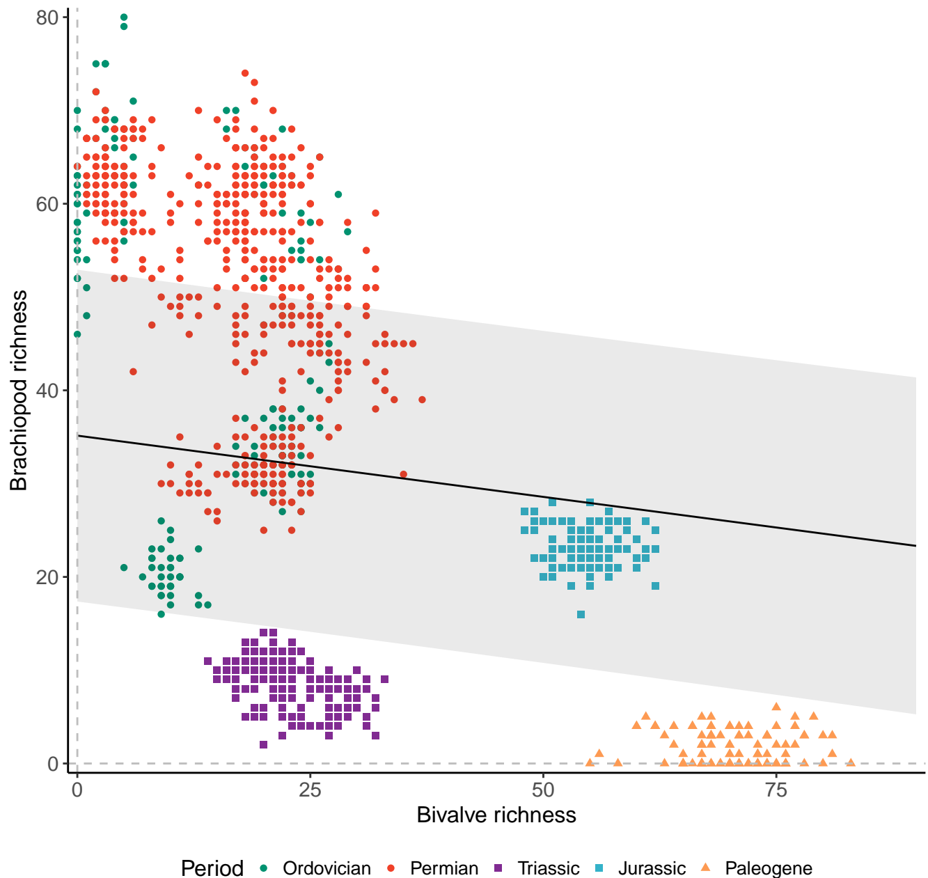
Genera, 200km grid cells, 5 sites, 1000km radius, full model
