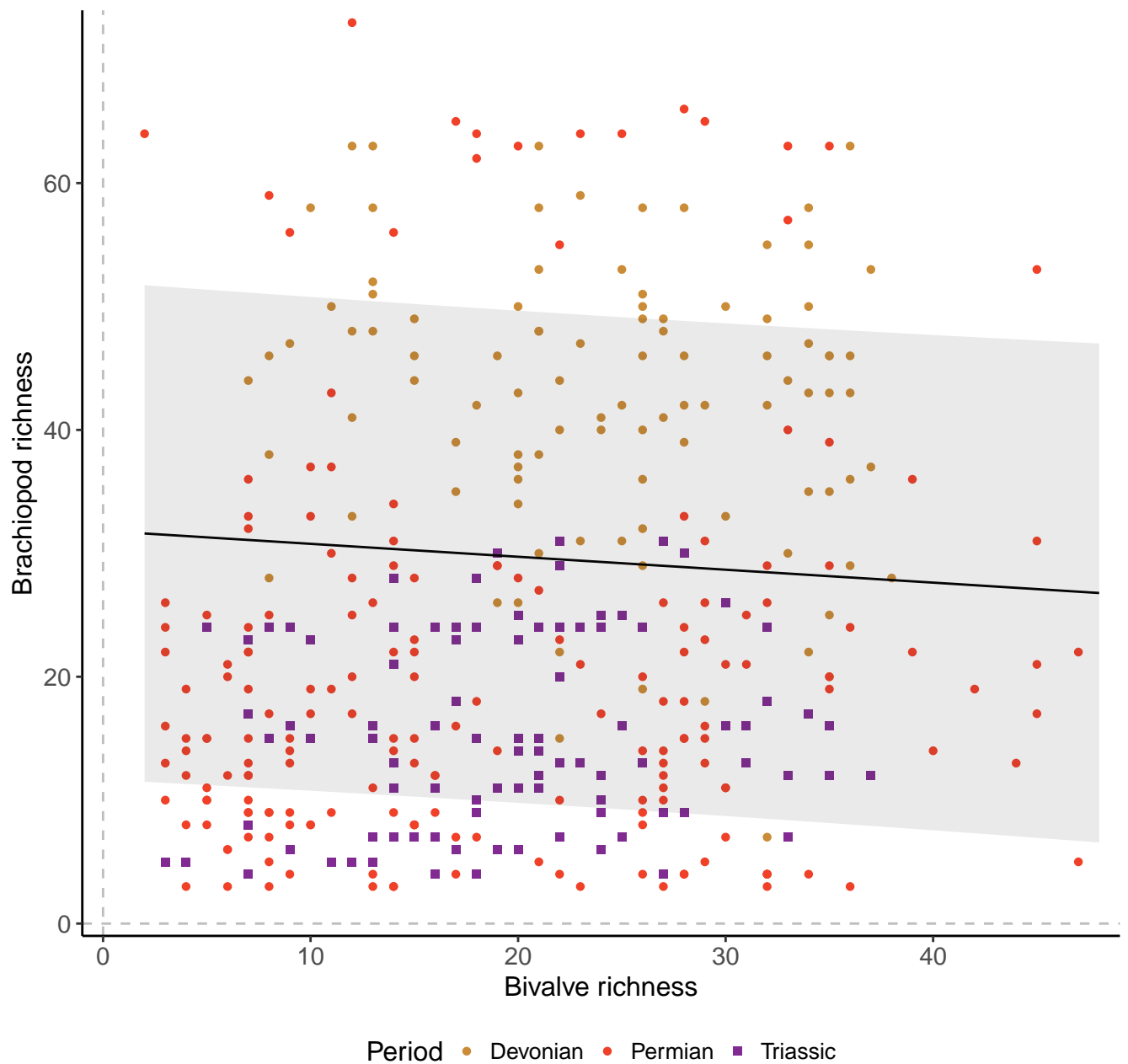
Genera, 100km grid cells, 5 sites, 1000km radius, full model
