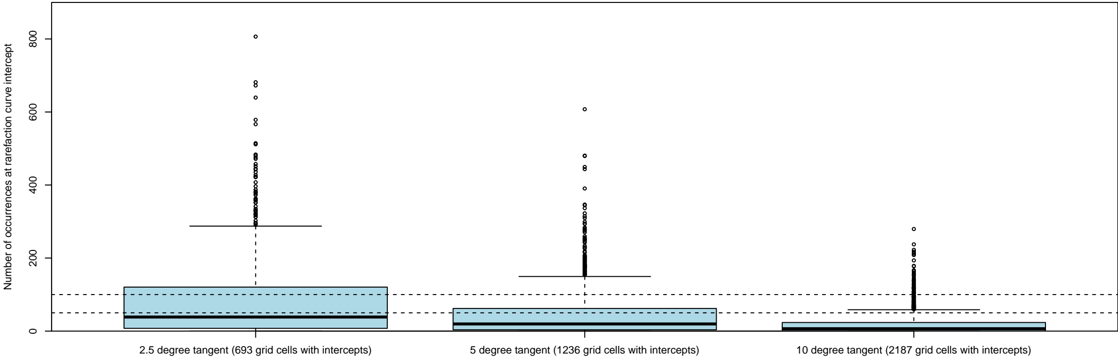
Number of occurrences at rarefaction curve intercept for 200km grid cells
