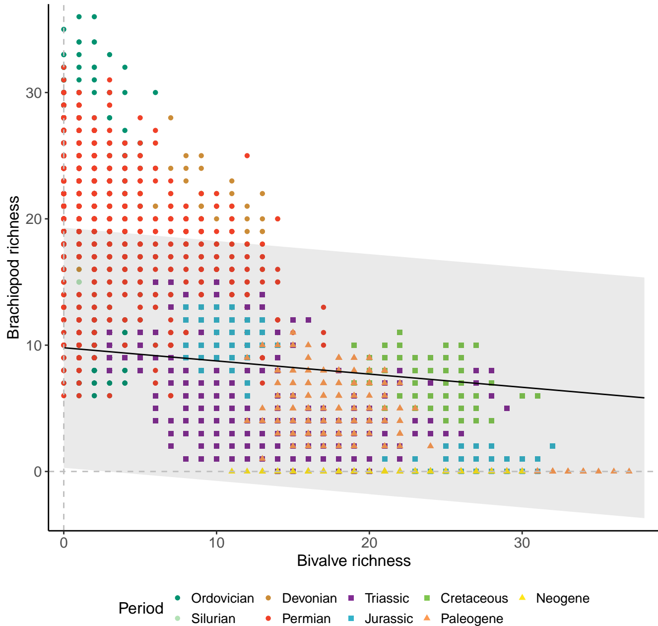
Genera, 100km grid cells, 2 sites, 200km radius, PTME as RE
