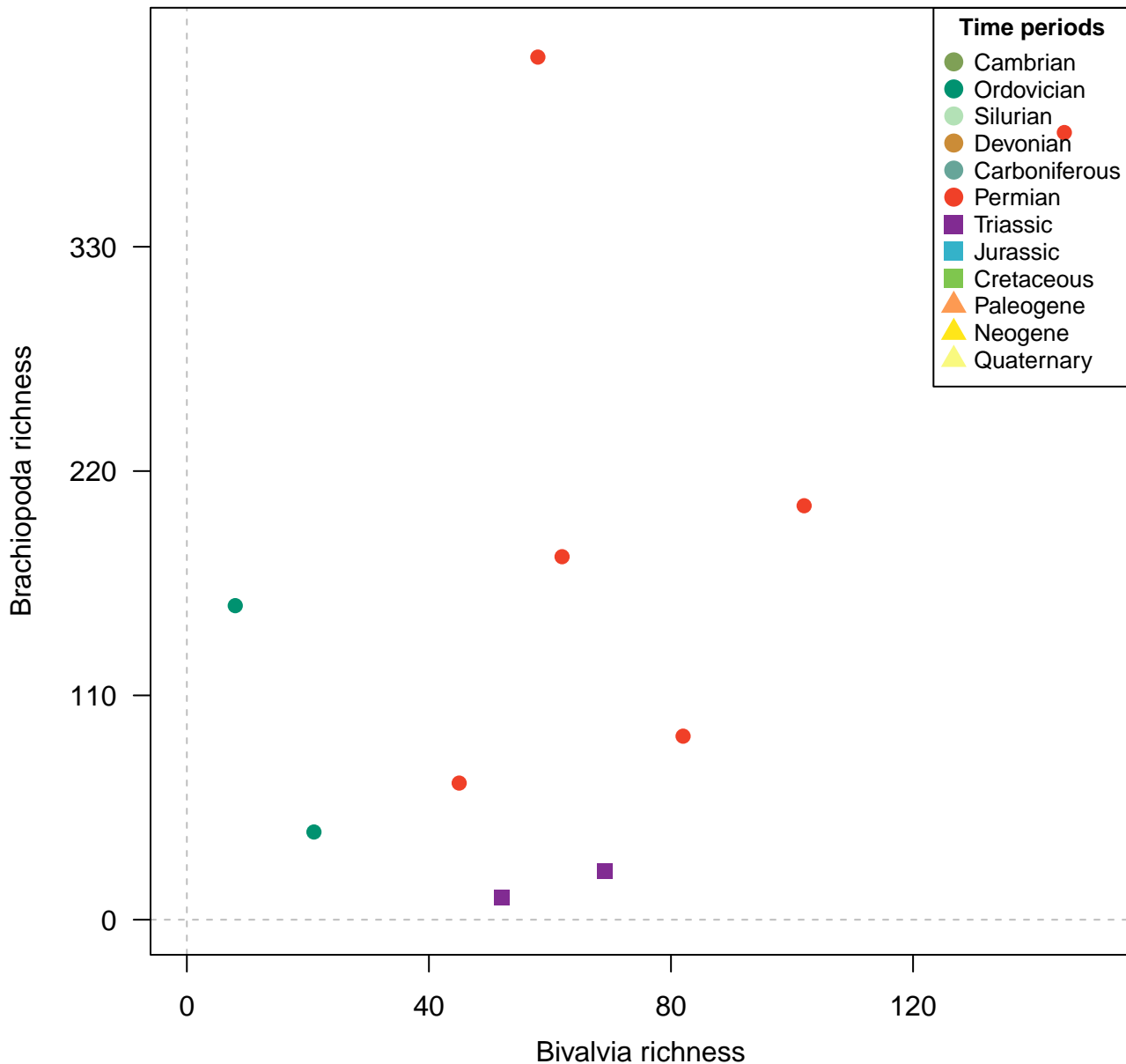
Species, 200km grid cells, raw, 5 site minima, 1000km radius, 10 subsamples
