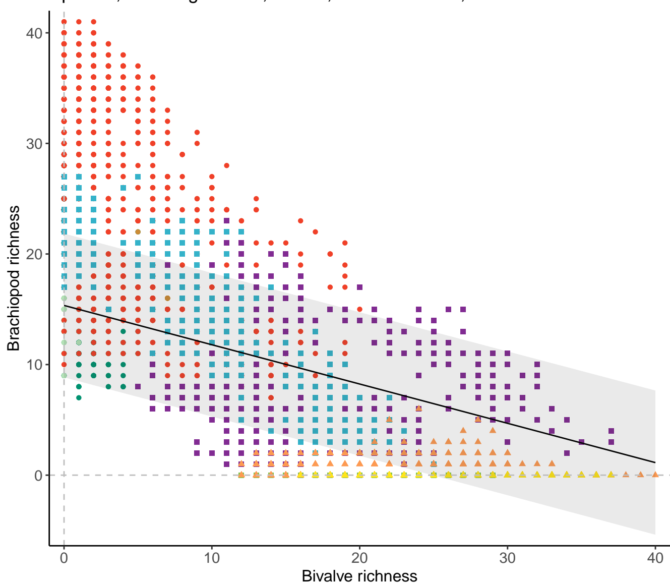
Species, 200km grid cells, 2 sites, 1000km radius, PTME as RE
