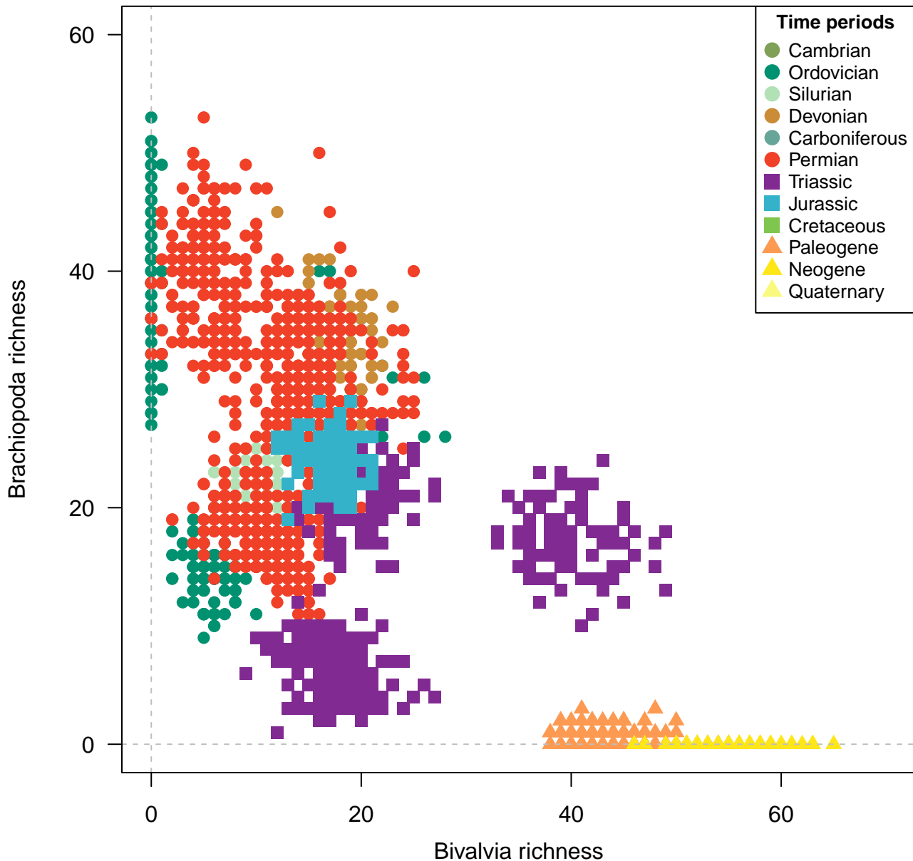
Genera, 200km grid cells, STO rarefaction, 3 site minima, 500km radius, 2000 subsamples
