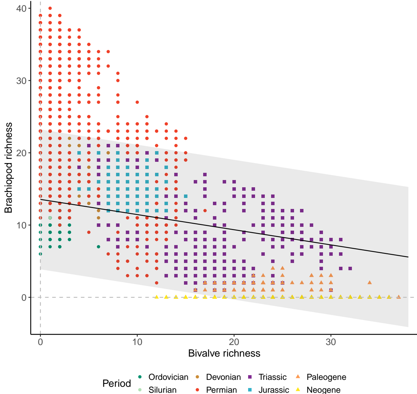
Species, 100km grid cells, 2 sites, 1000km radius, PTME as RE
