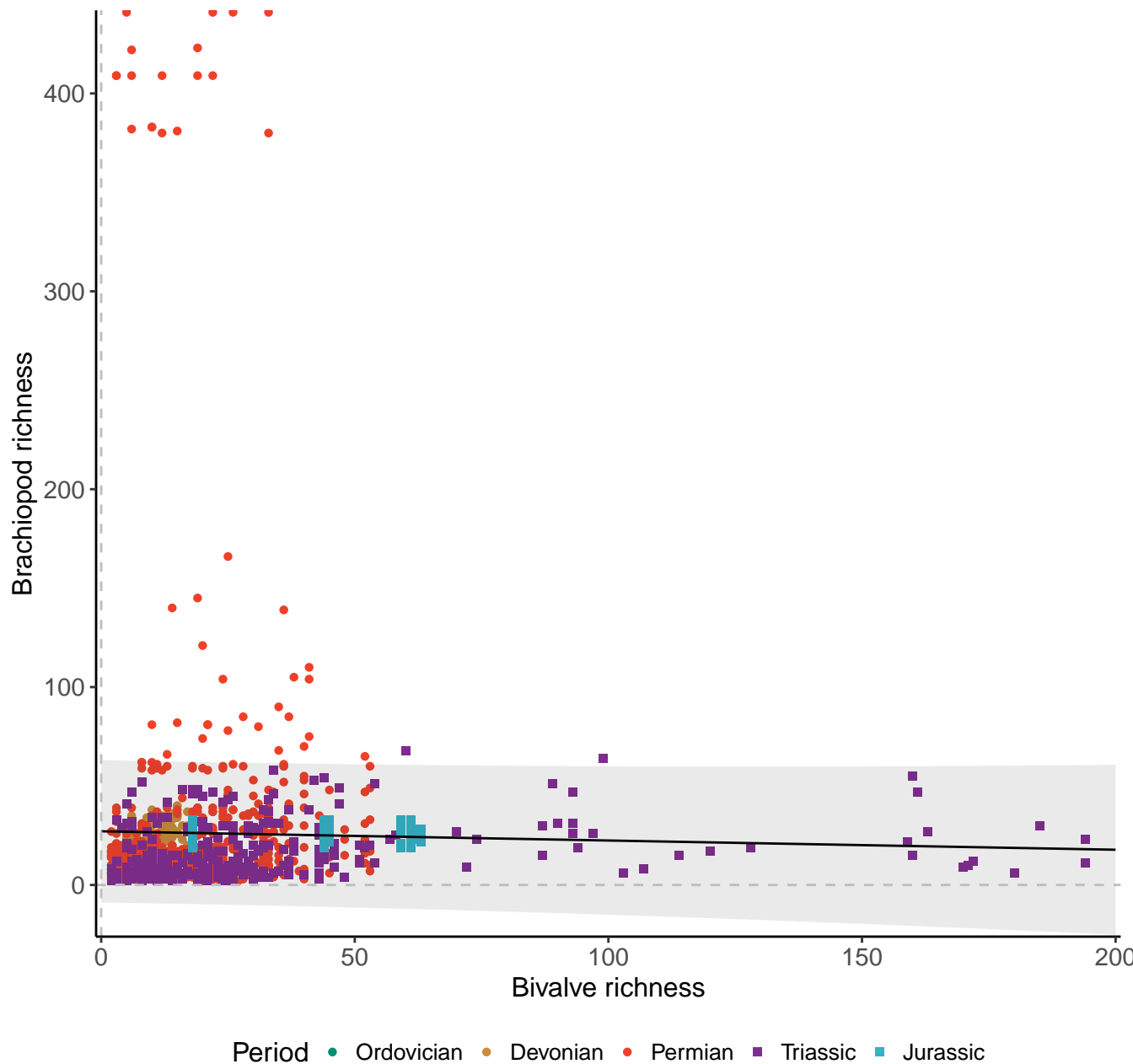
Species, 200km grid cells, 2 sites, 500km radius, full model
