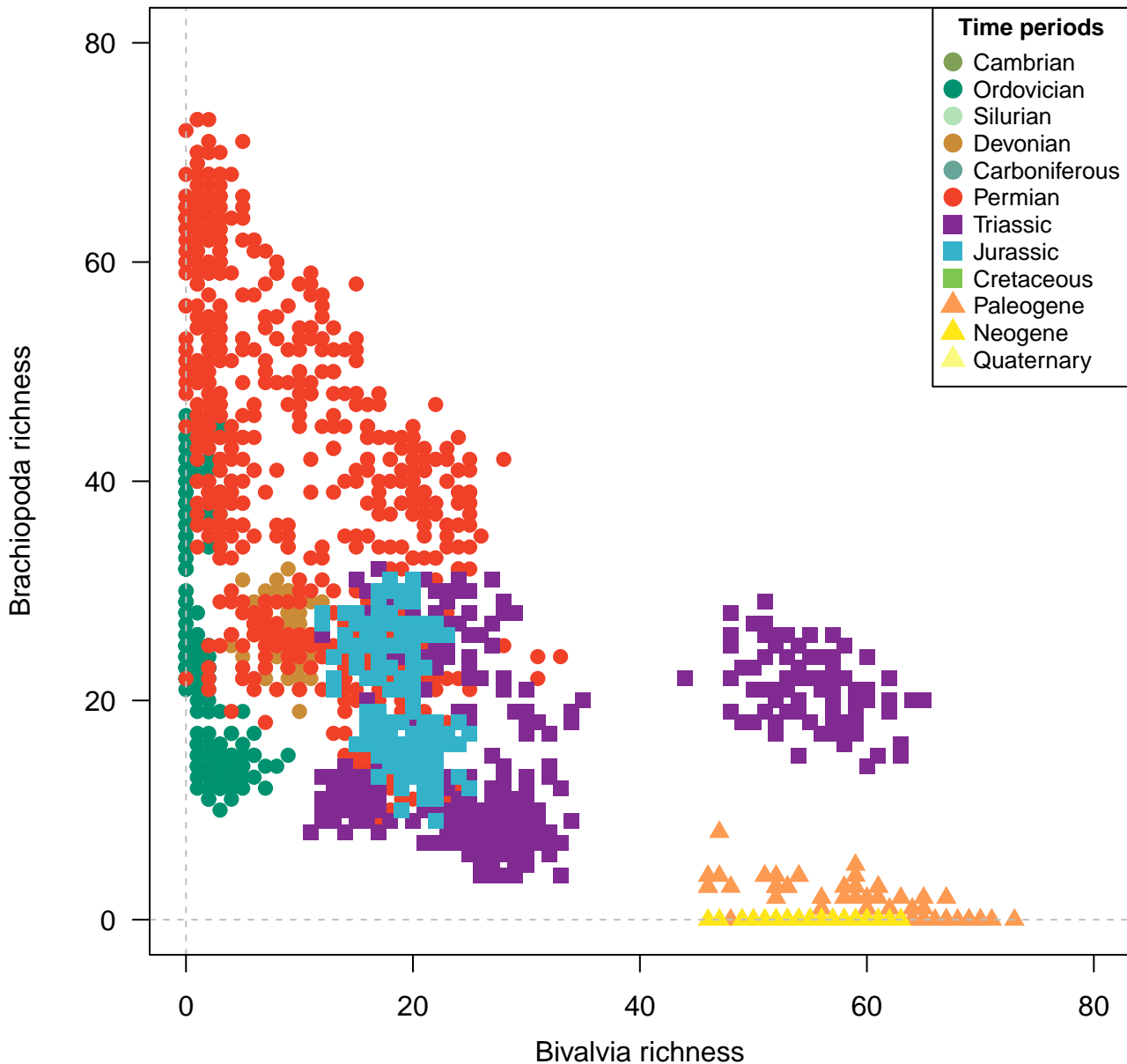
Species, 100km grid cells, STO rarefaction, 3 site minima, 1000km radius, 2100 subsamples
