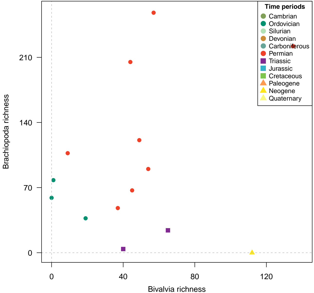
Species, 200km grid cells, raw, 3 site minima, 500km radius, 14 subsamples
