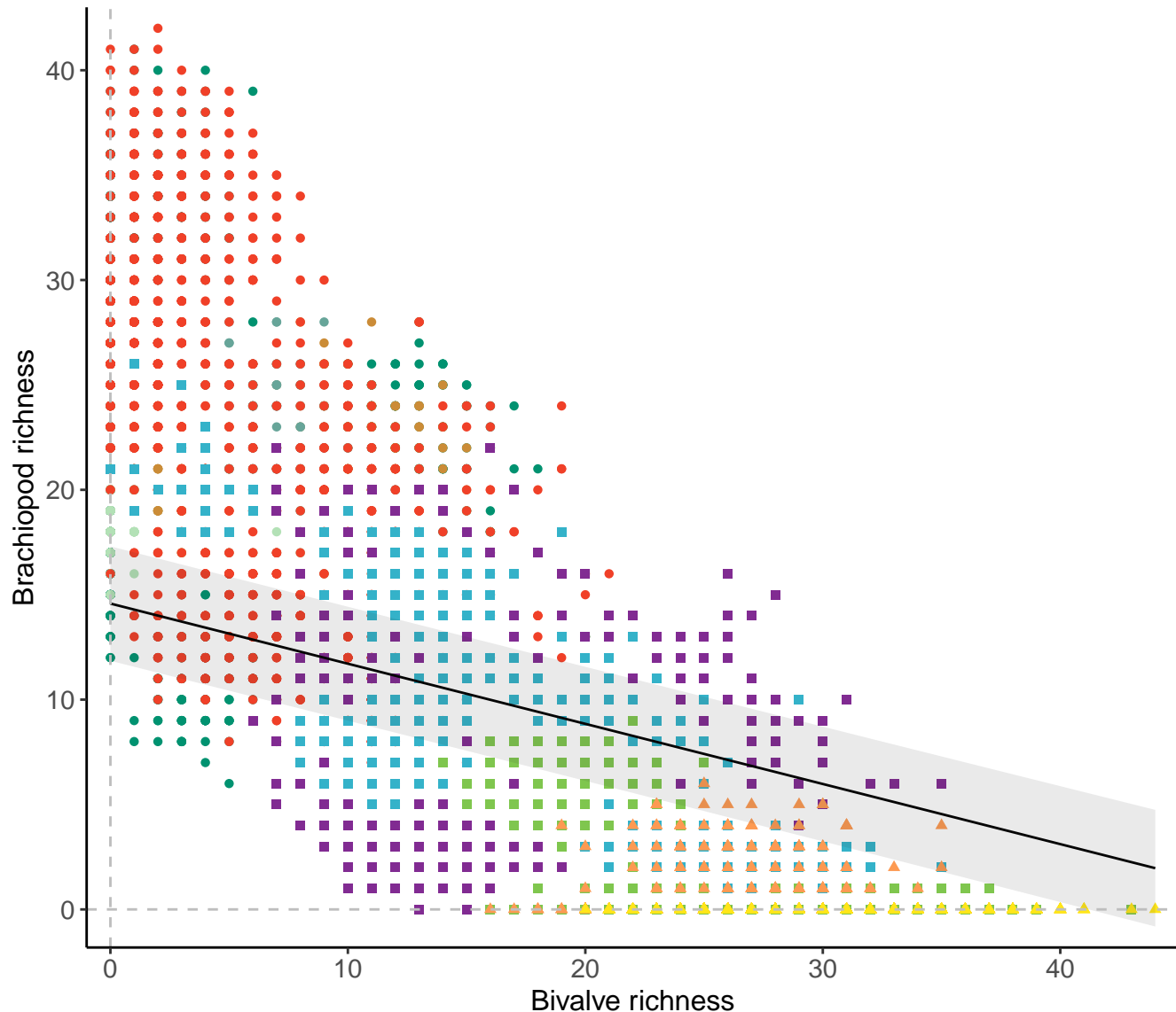
Genera, 200km grid cells, 2 sites, 500km radius, full model
