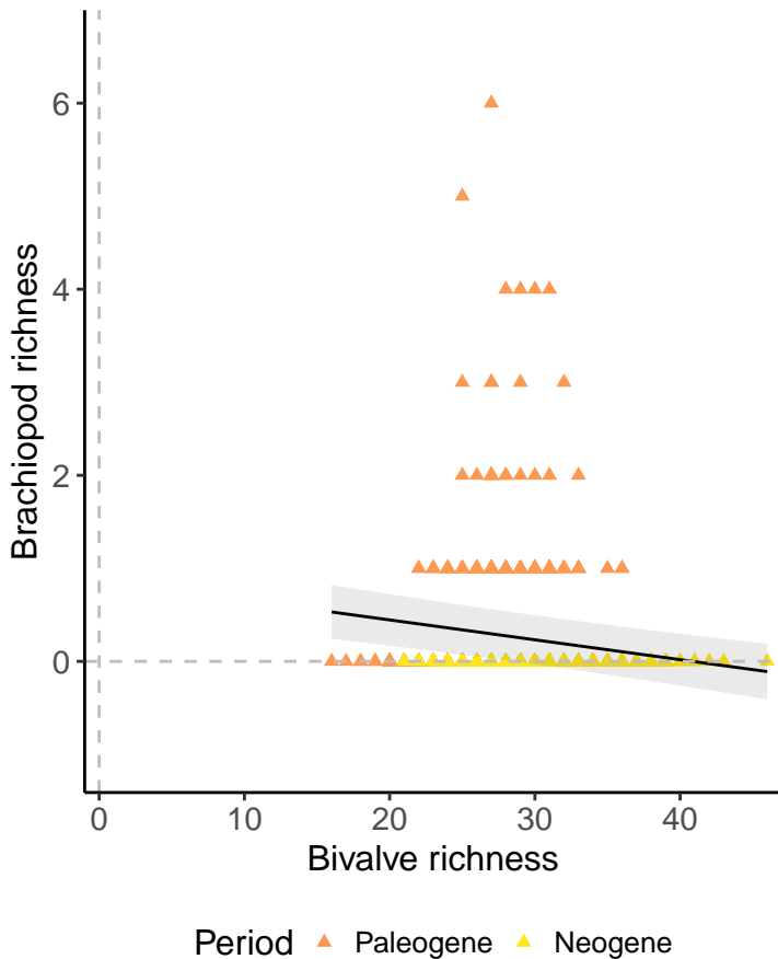
A Genera, 200km grid cells, 2 sites, 1000km radius, Cenozoic
