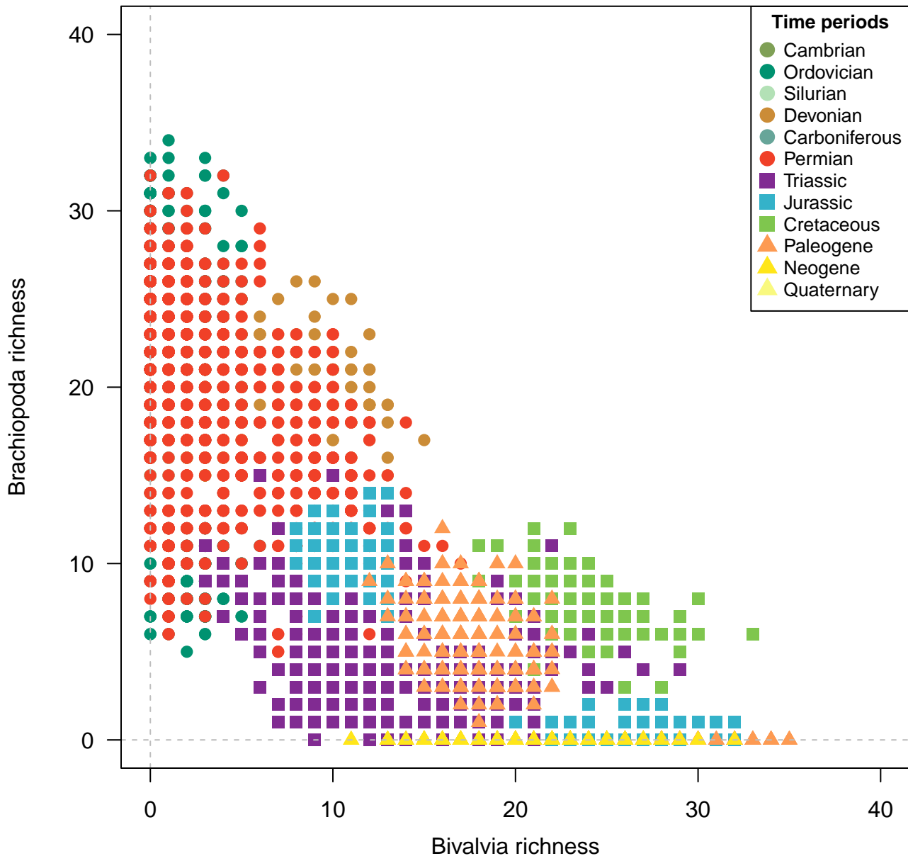
Genera, 100km grid cells, STO rarefaction, 2 site minima, 200km radius, 4400 subsamples
