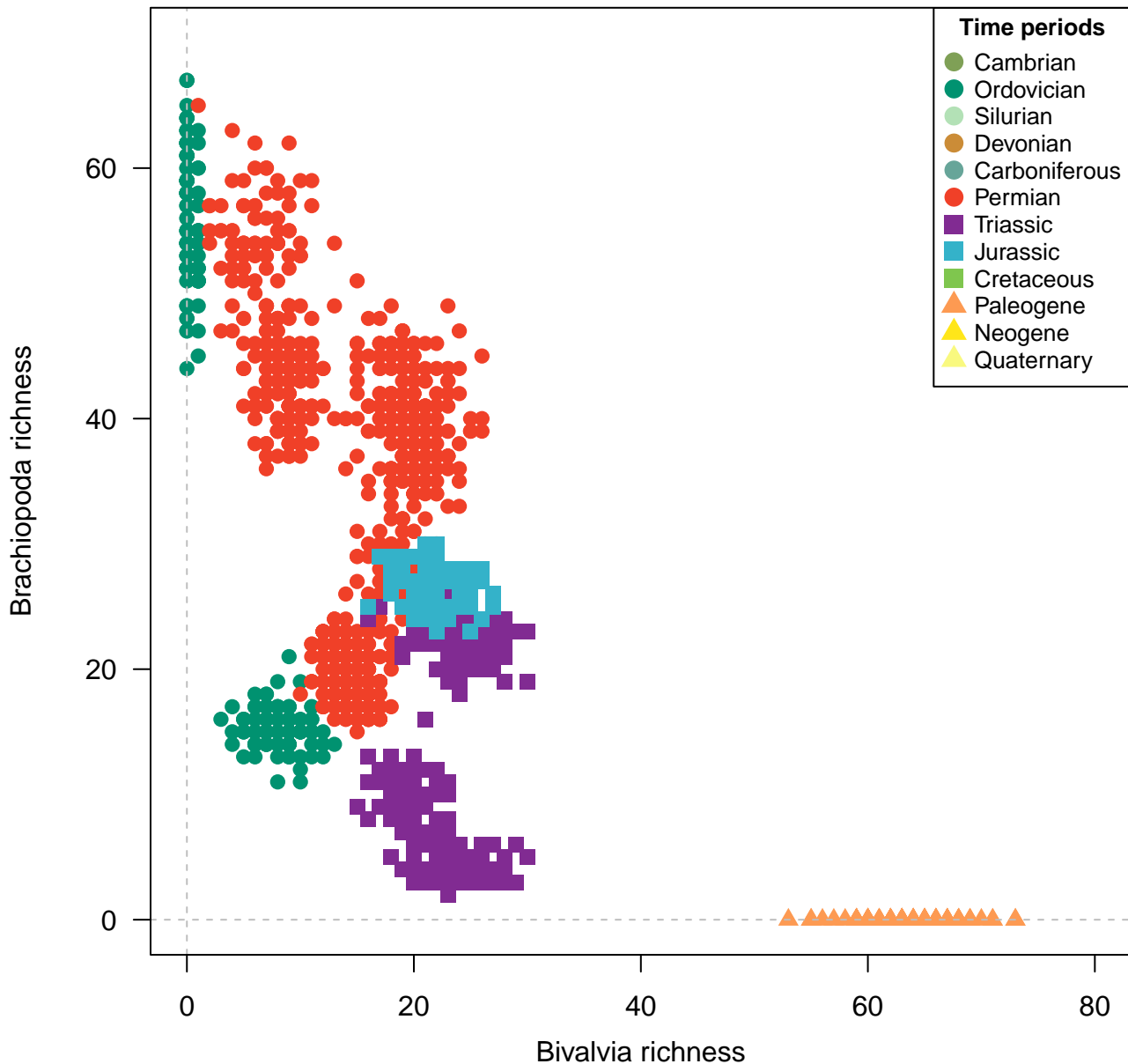
Genera, 200km grid cells, STO rarefaction, 3 site minima, 200km radius, 1400 subsamples
