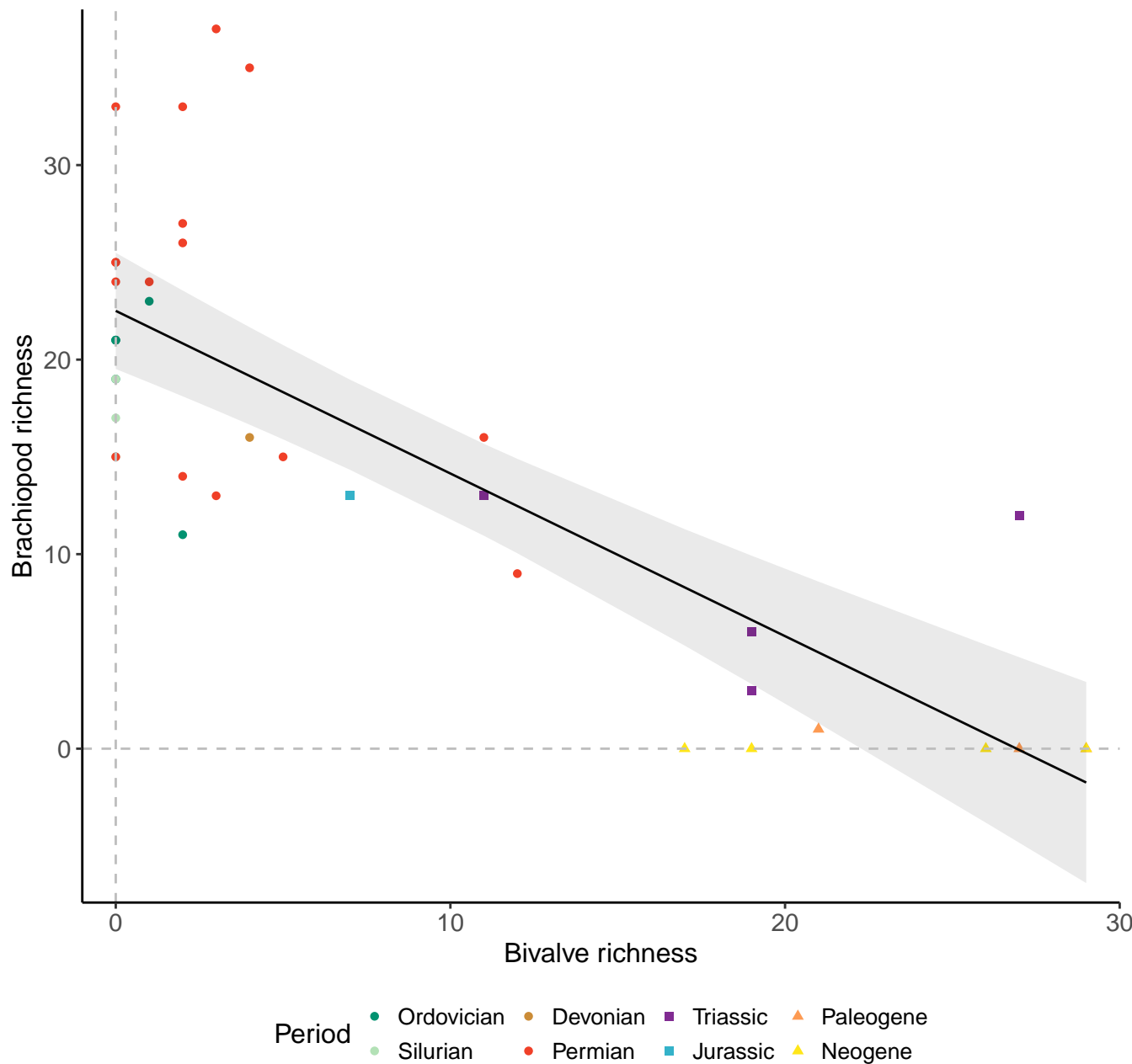
Species, 100km grid cells, 2 sites, 1000km radius, median richness
