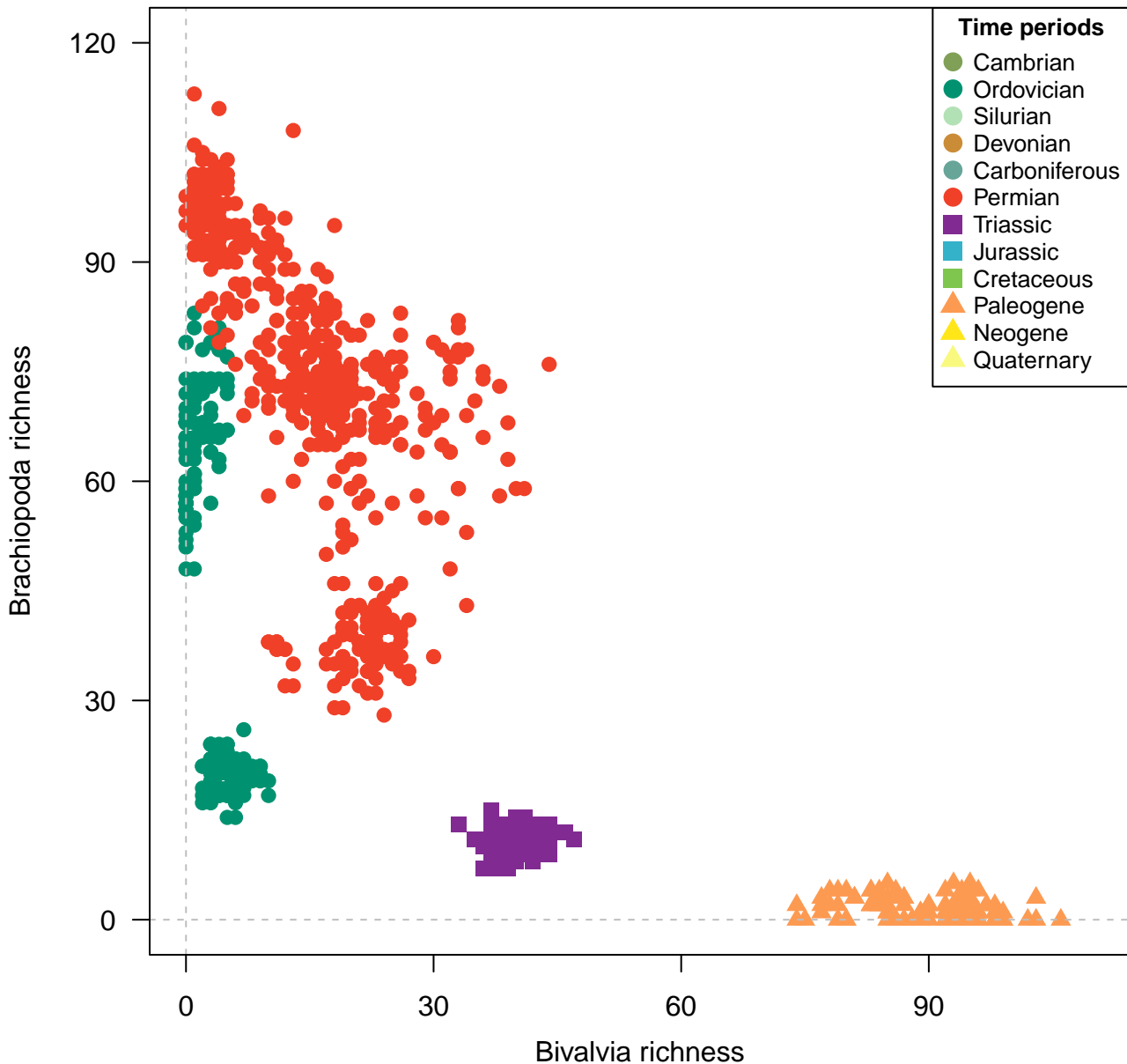
Species, 200km grid cells, STO rarefaction, 5 site minima, 1000km radius, 900 subsamples
