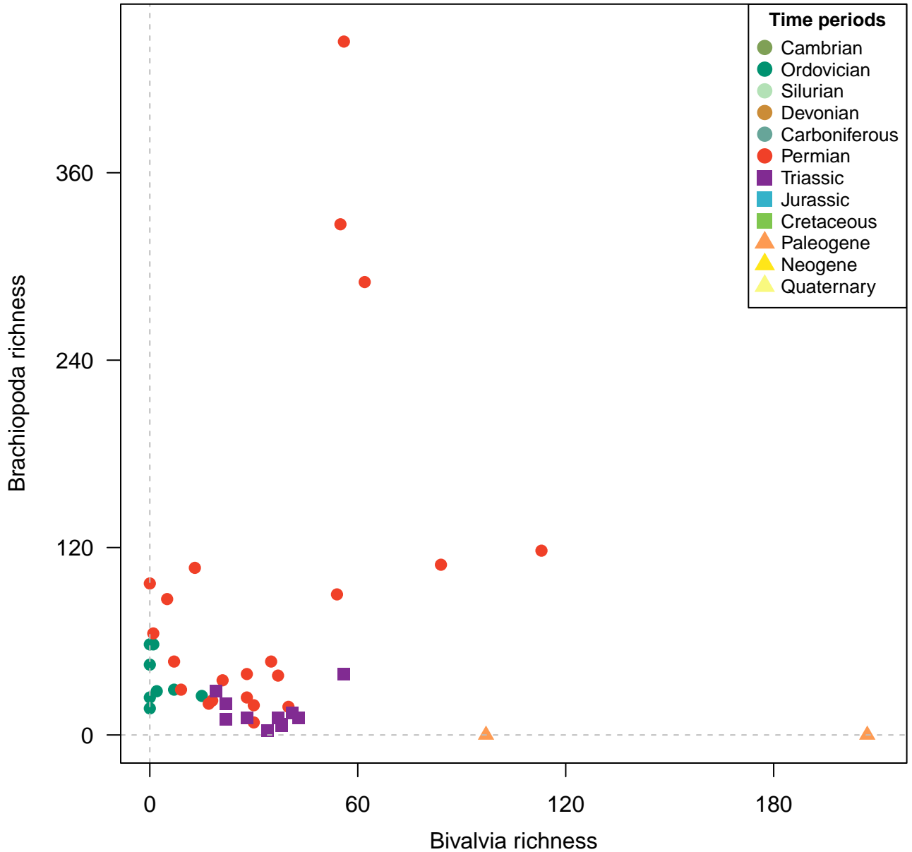
Species, 200km grid cells, raw, 2 site minima, 200km radius, 44 subsamples
