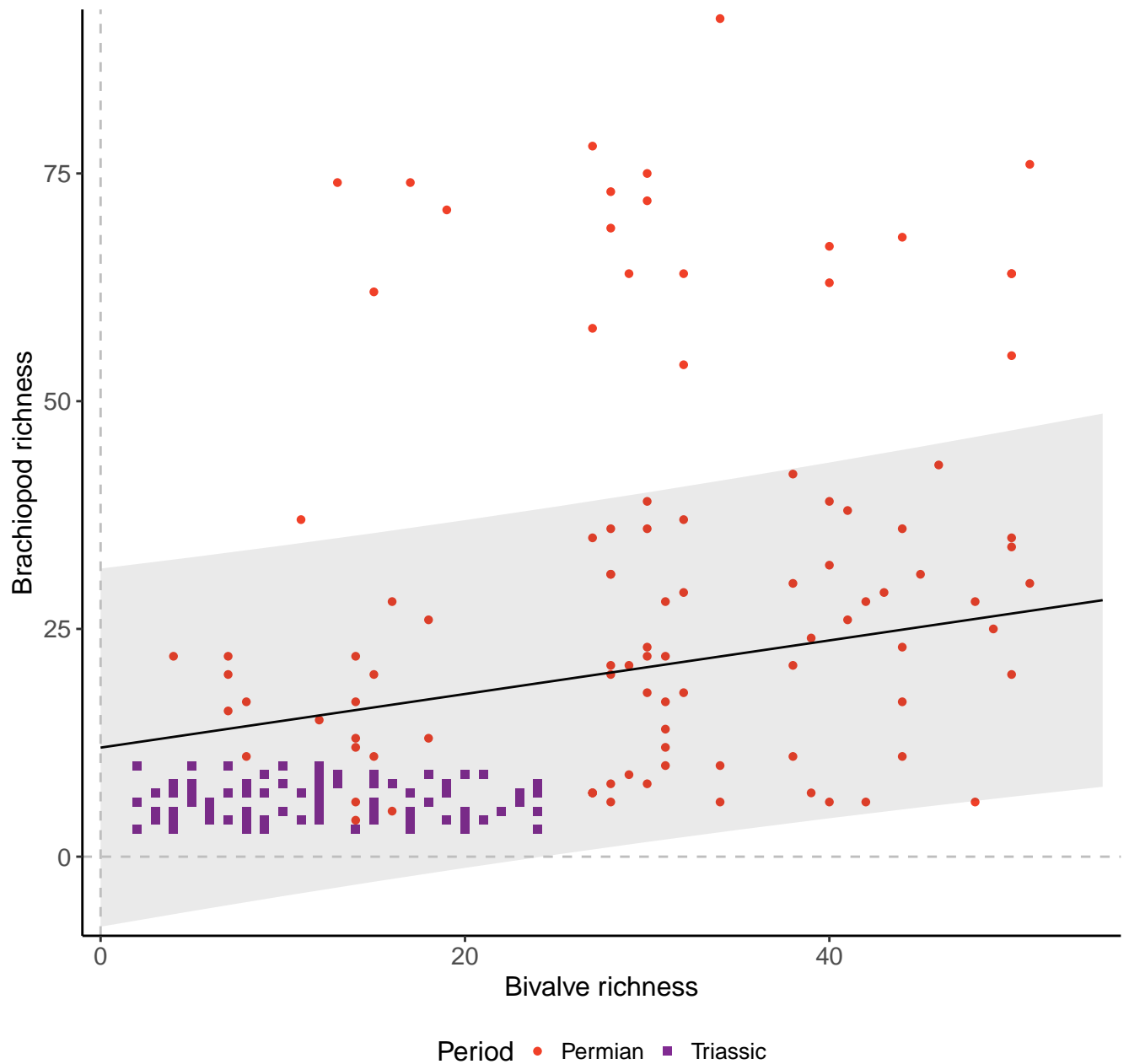
Genera, 200km grid cells, 5 sites, 500km radius, simple model
