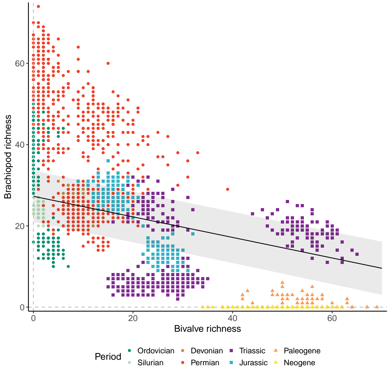
Species, 200km grid cells, 3 sites, 1000km radius, simple model
