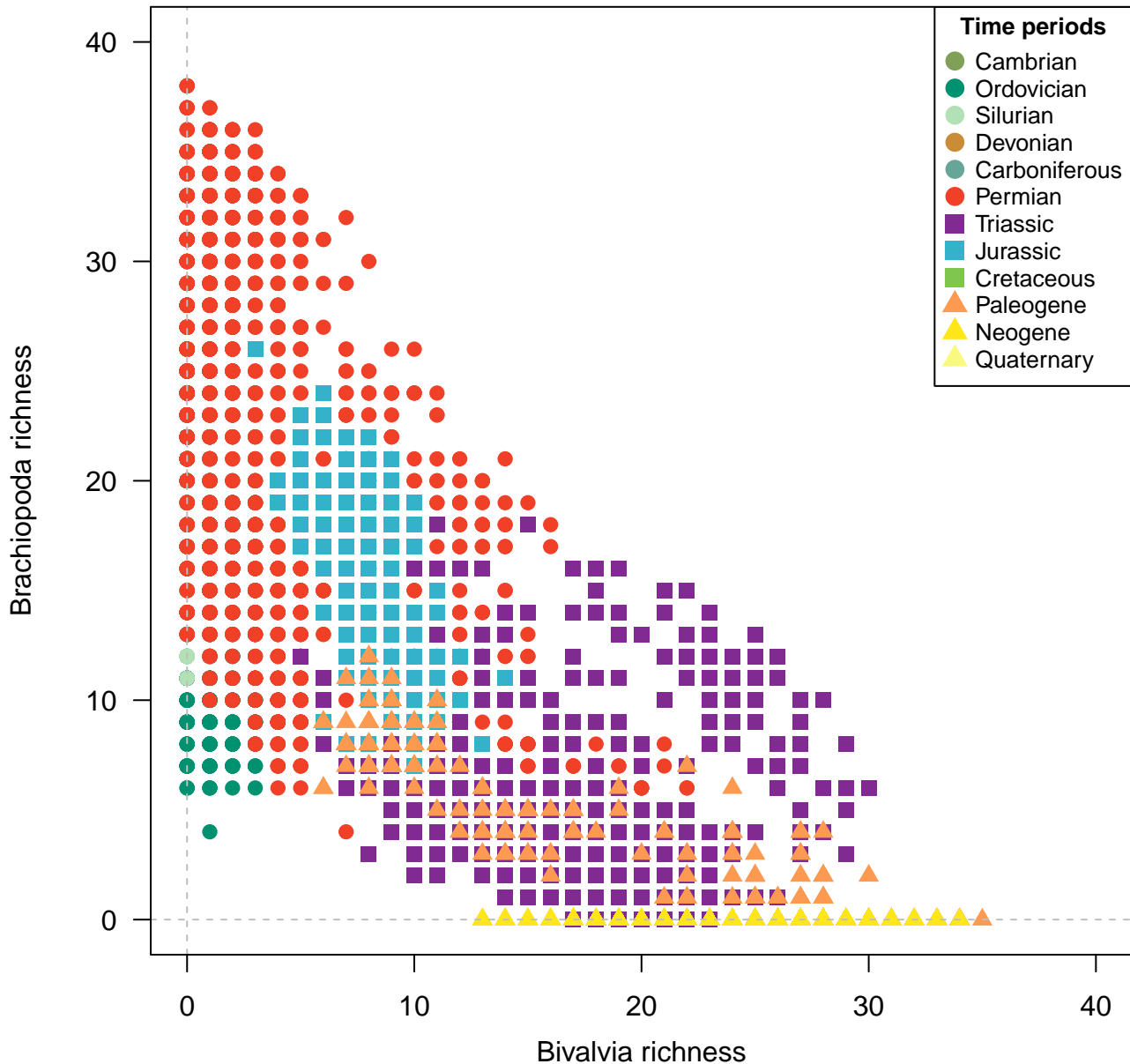
Species, 100km grid cells, STO rarefaction, 2 site minima, 500km radius, 4900 subsamples
