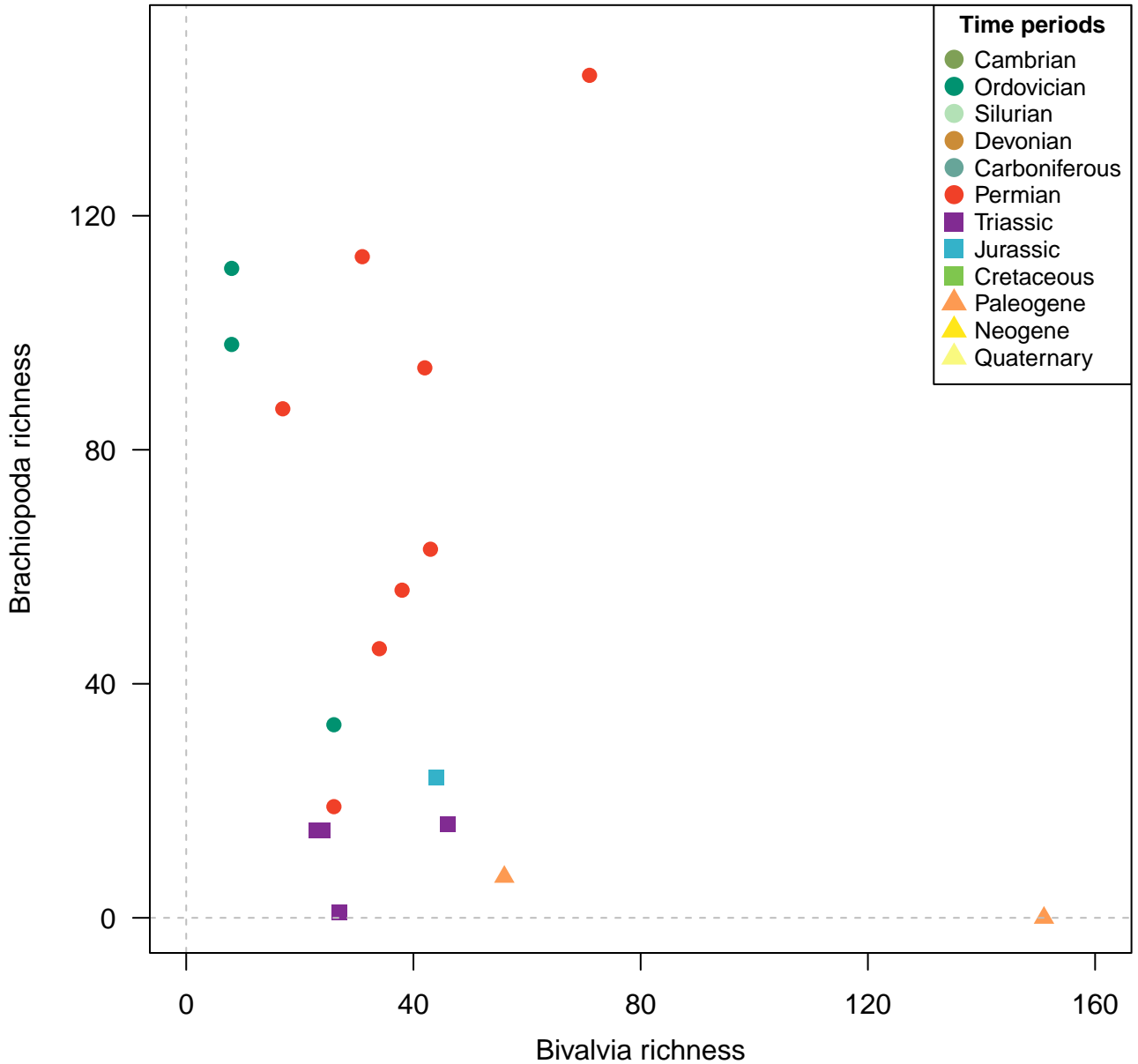
Genera, 100km grid cells, raw, 3 site minima, 1000km radius, 18 subsamples
