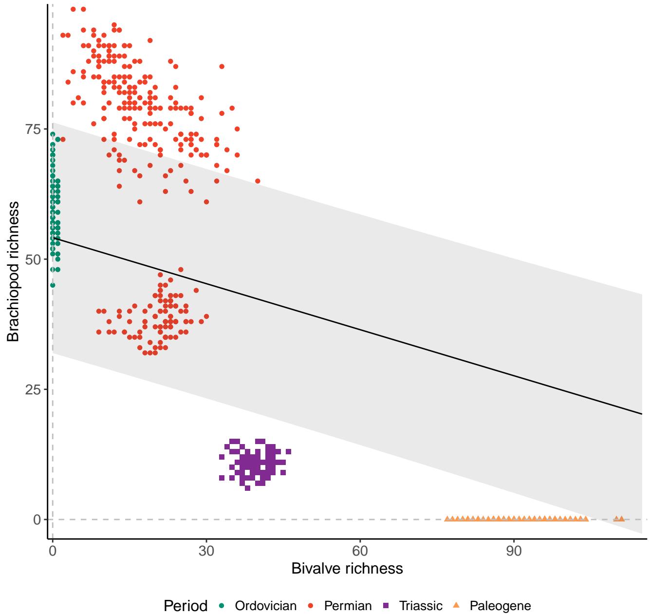
Species, 200km grid cells, 5 sites, 500km radius, simple model
