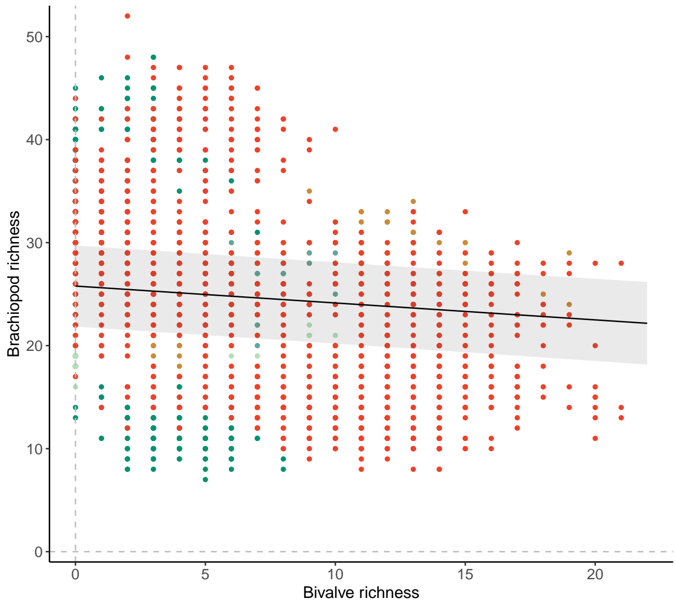
Genera, 200km grid cells, 2 sites, 200km radius, Pre-PTME
