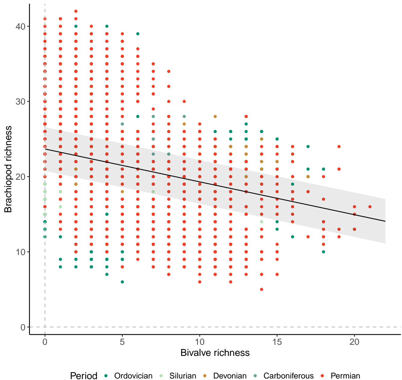
Genera, 200km grid cells, 2 sites, 500km radius, Pre-PTME
