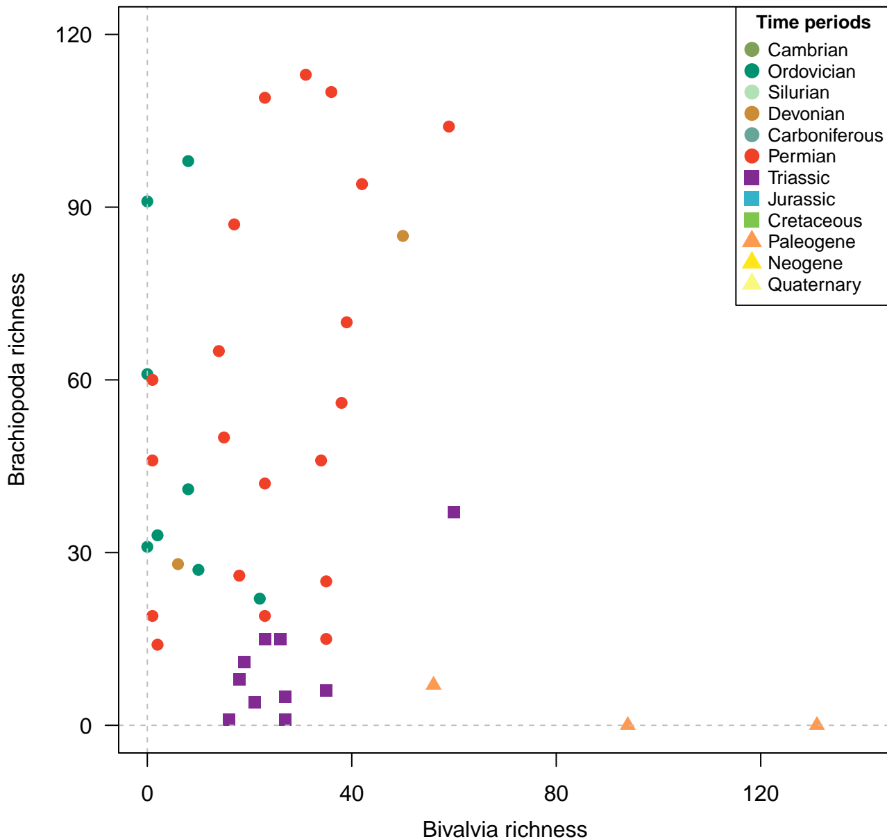
Genera, 100km grid cells, raw, 2 site minima, 500km radius, 44 subsamples
