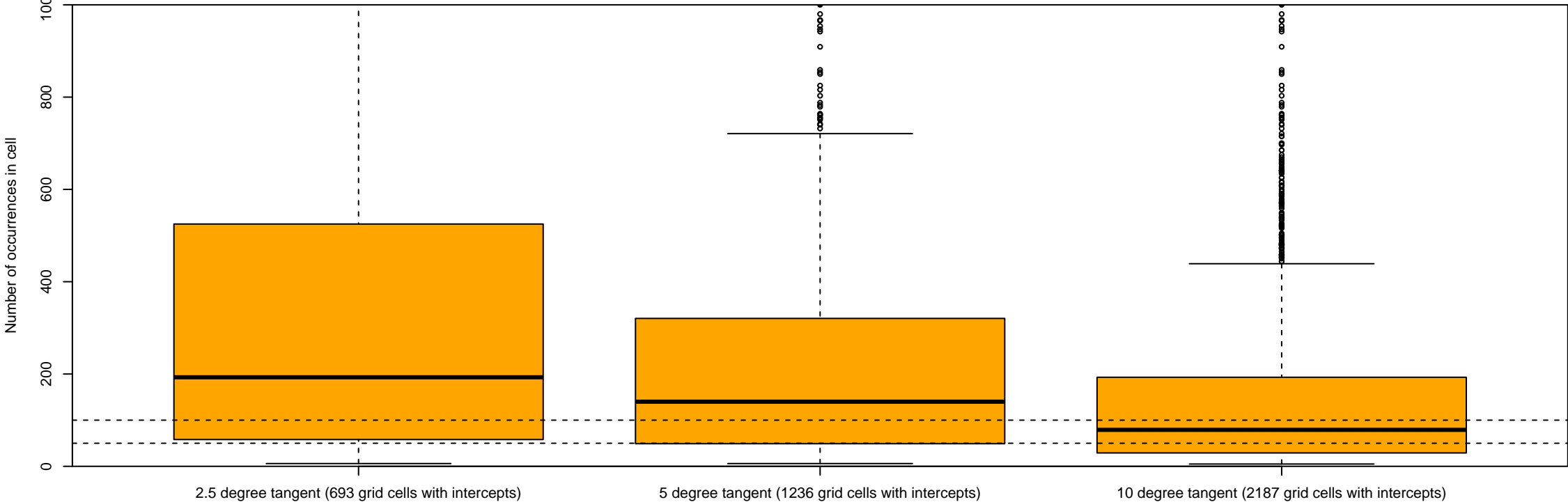
Number of occurrences in 200km grid cells with rarefaction curve intercepts (capped at 1000 occurrences)
