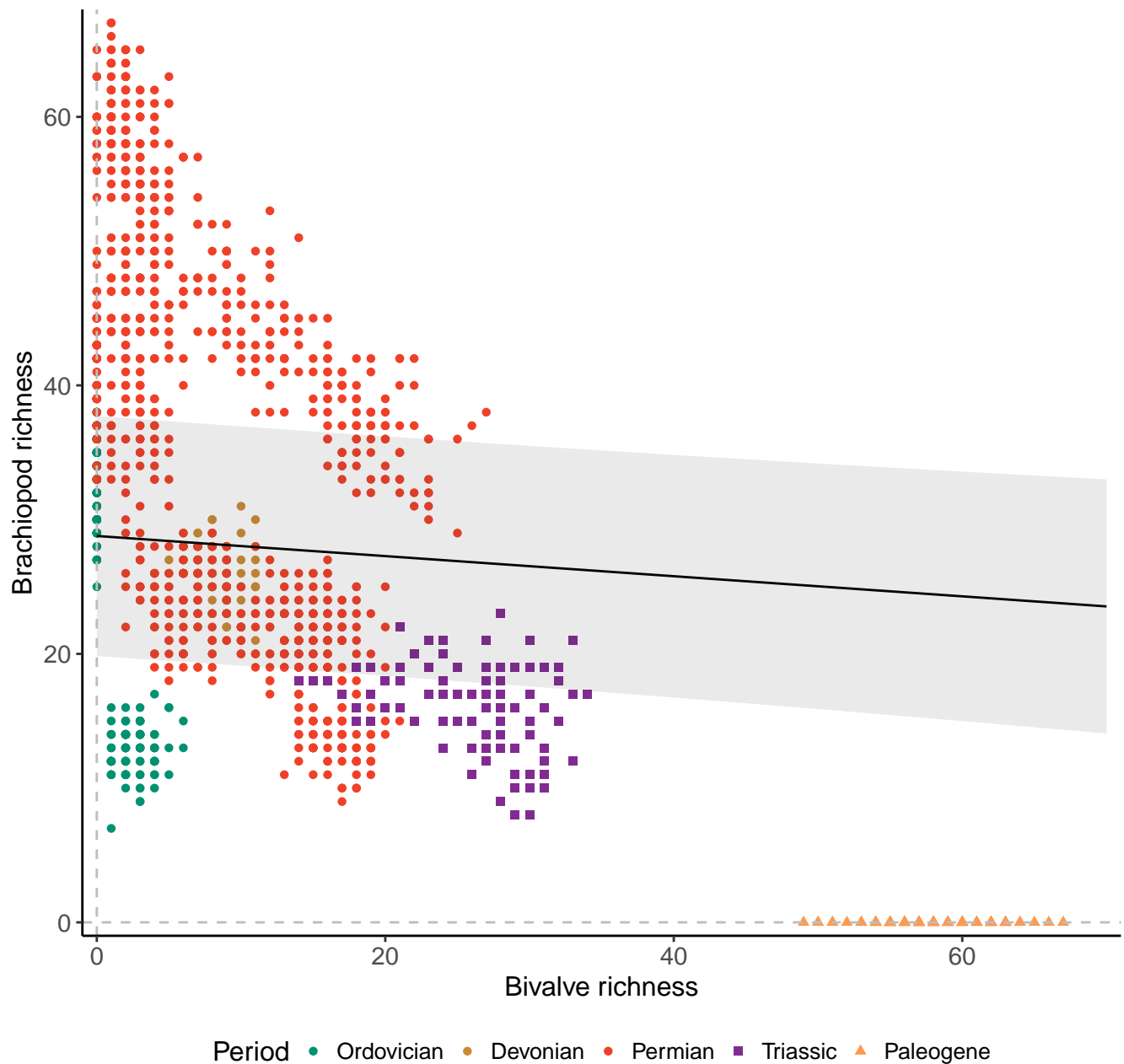
Species, 100km grid cells, 3 sites, 200km radius, simple model
