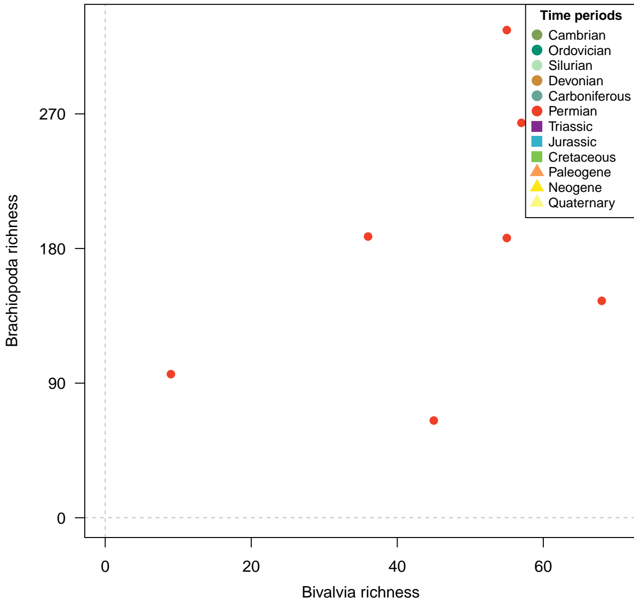
Species, 100km grid cells, raw, 4 site minima, 500km radius, 7 subsamples
