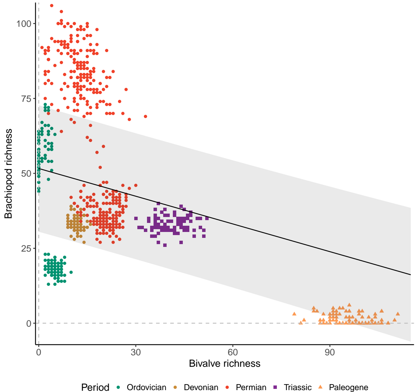
Species, 100km grid cells, 5 sites, 1000km radius, full model
