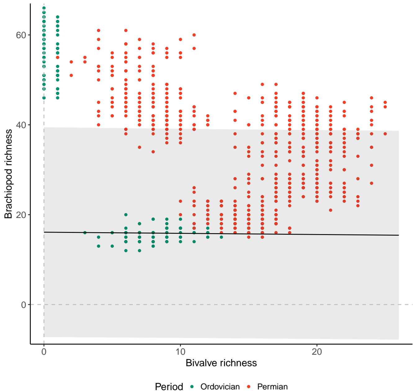
Genera, 200km grid cells, 3 sites, 200km radius, Paleozoic
