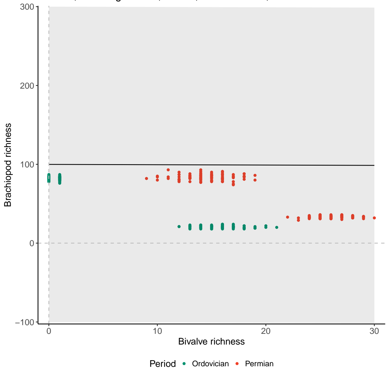
Genera, 200km grid cells, 4 sites, 200km radius, Pre-PTME
