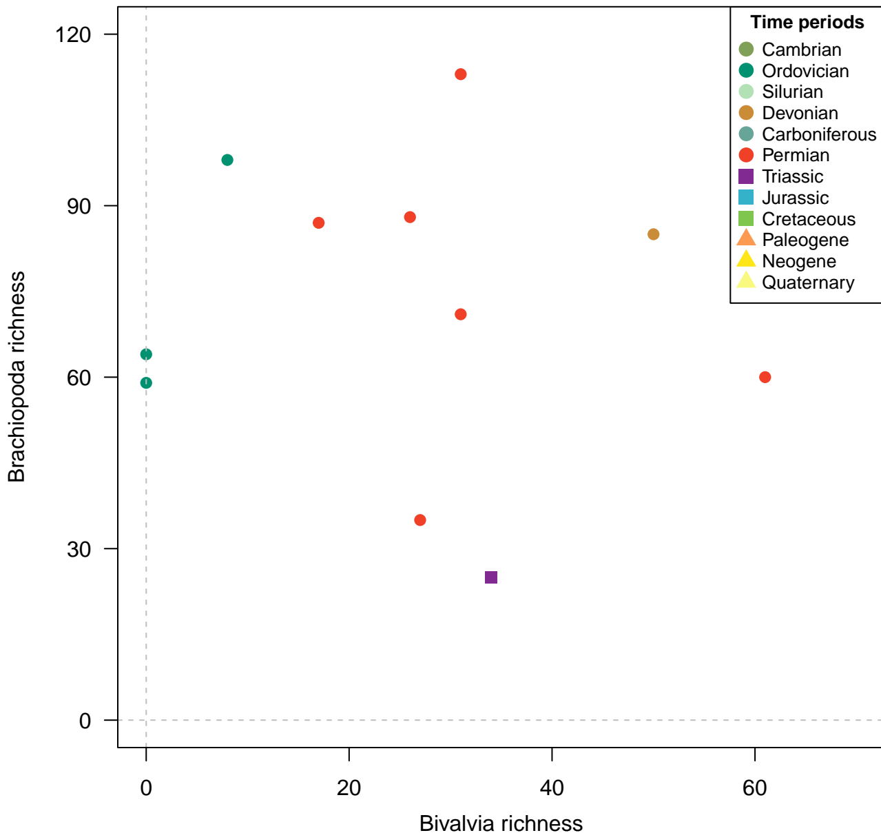
Genera, 100km grid cells, raw, 4 site minima, 200km radius, 11 subsamples
