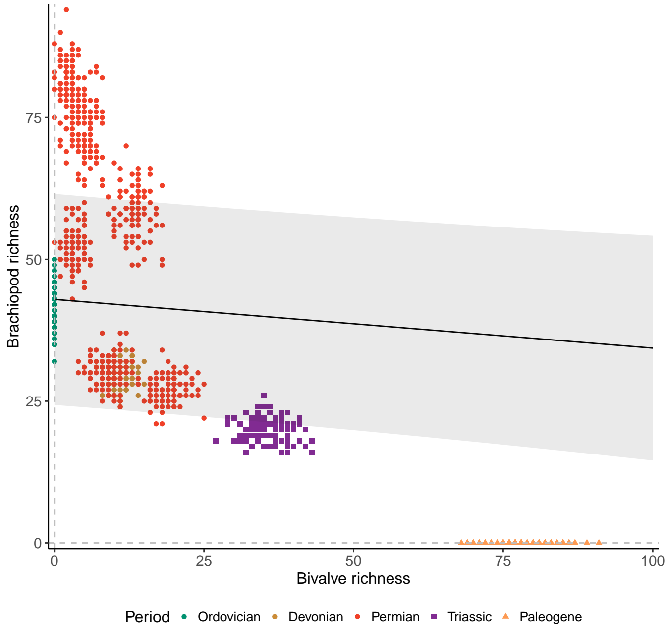
Species, 100km grid cells, 4 sites, 200km radius, full model
