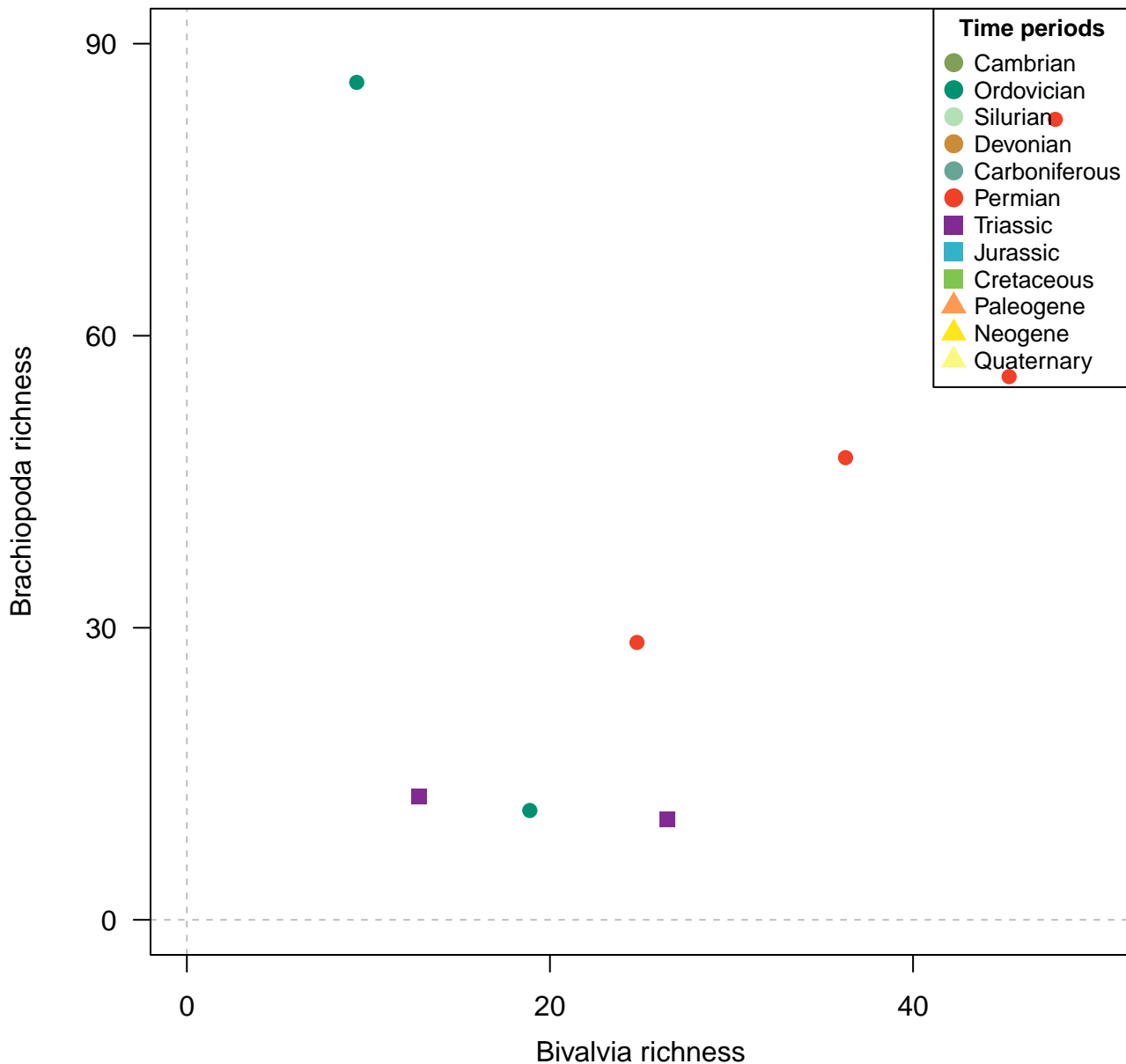
Genera, 100km grid cells, SQS (q = 0.9), 5 site minima, 1000km radius, 8 subsamples
