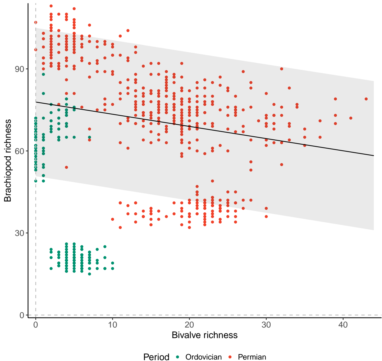
Species, 200km grid cells, 5 sites, 1000km radius, Pre-PTME
