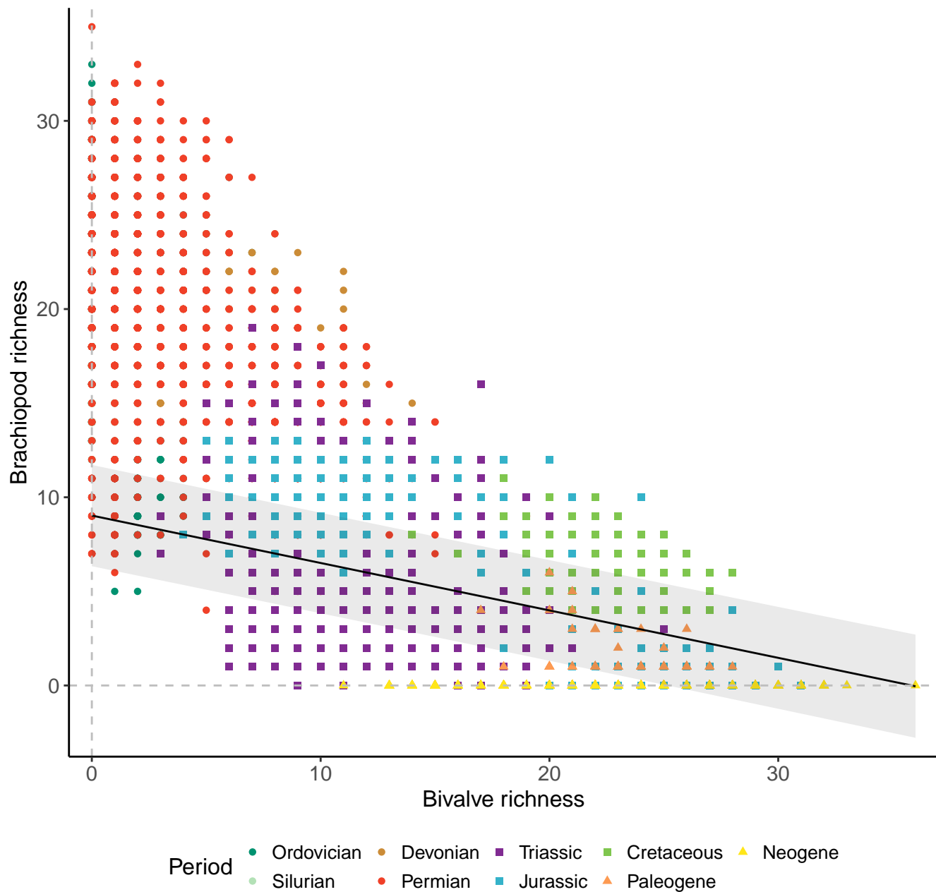
Genera, 100km grid cells, 2 sites, 1000km radius, full model
