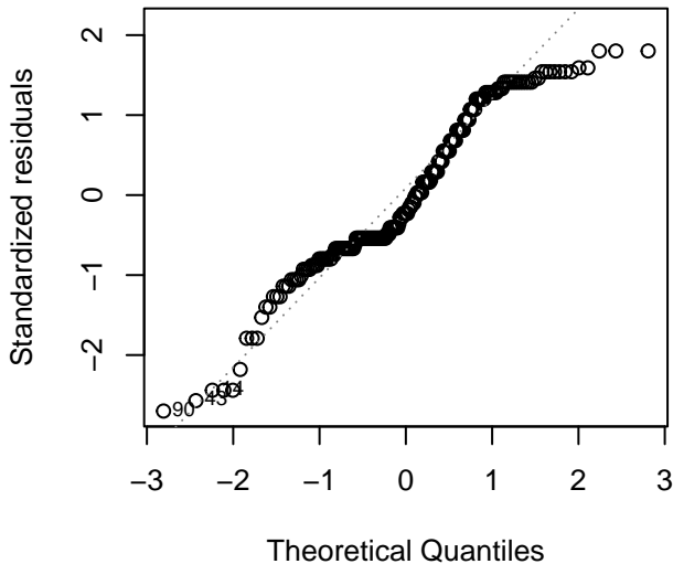
Q-Q Residuals
