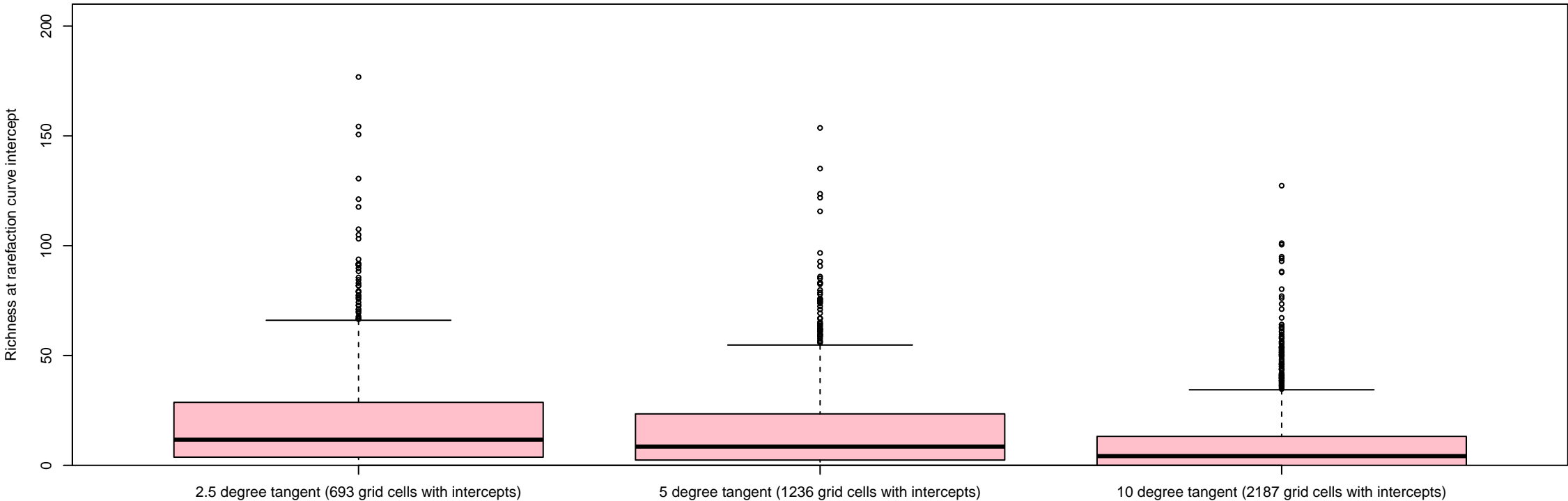
Richness at rarefaction curve intercept for 200km grid cells
