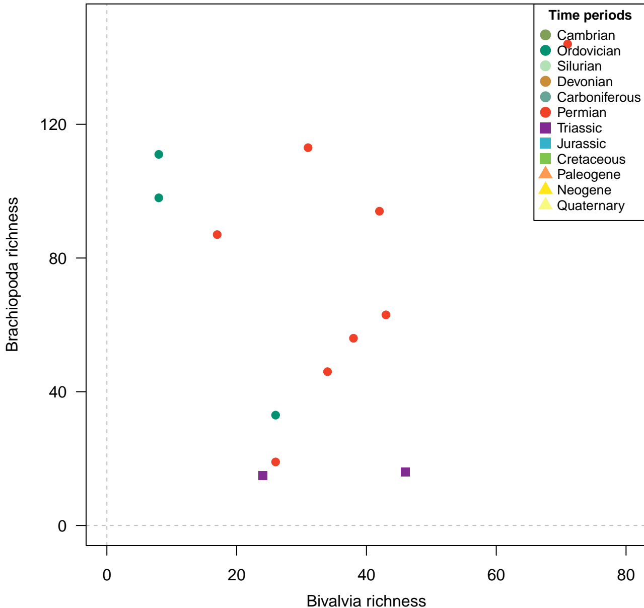
Genera, 100km grid cells, raw, 4 site minima, 1000km radius, 13 subsamples
