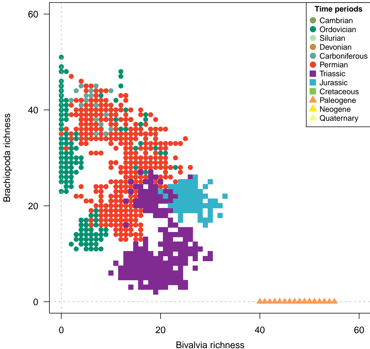
Genera, 200km grid cells, STO rarefaction, 4 site minima, 500km radius, 1800 subsamples
