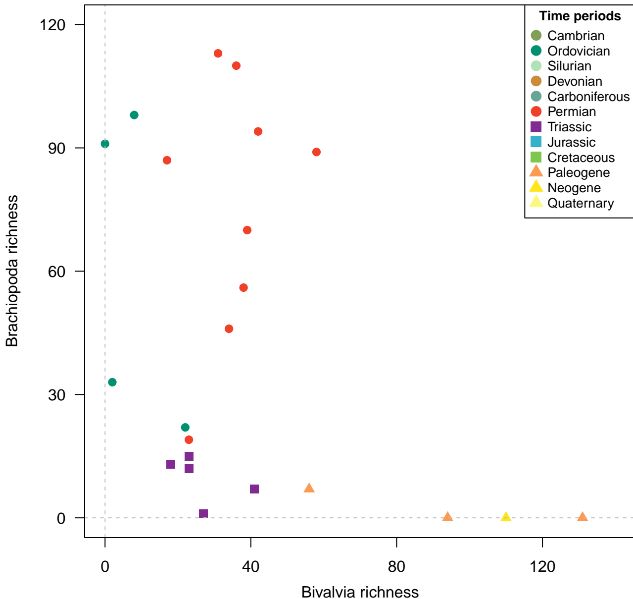
Genera, 100km grid cells, raw, 3 site minima, 500km radius, 22 subsamples
