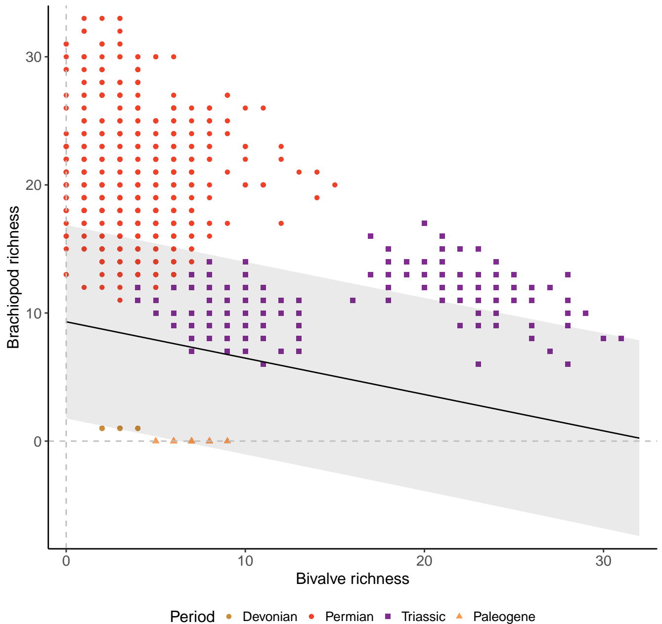
Species, 200km grid cells, 3 sites, 500km radius, full model
