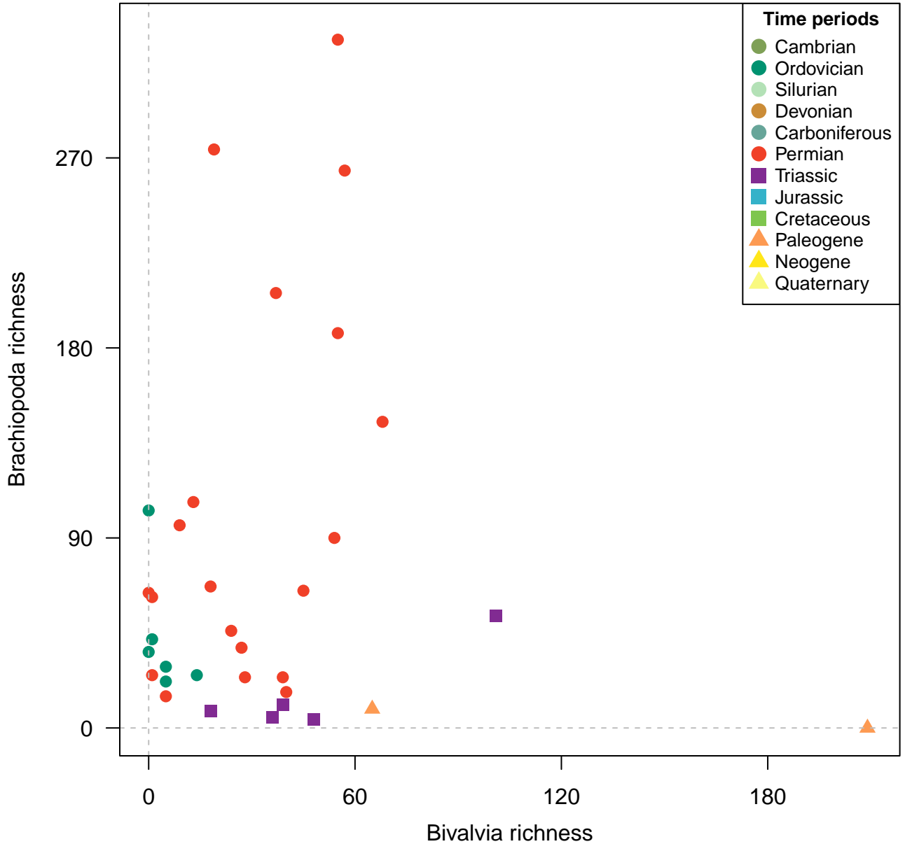
Species, 100km grid cells, raw, 2 site minima, 500km radius, 33 subsamples
