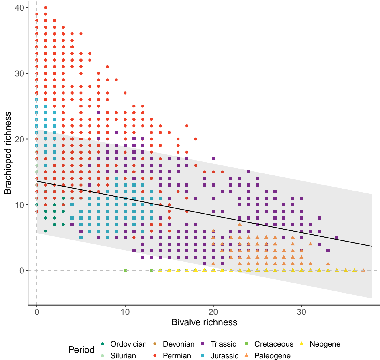
Species, 200km grid cells, 2 sites, 500km radius, PTME as RE
