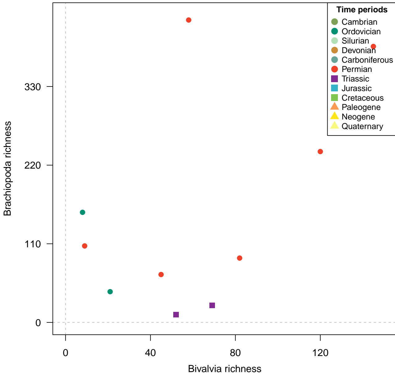
Species, 200km grid cells, raw, 4 site minima, 1000km radius, 10 subsamples
