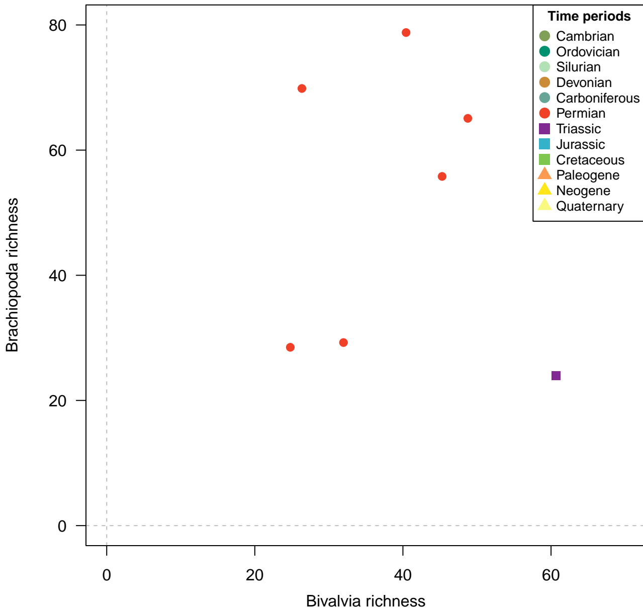
Genera, 100km grid cells, SQS (q = 0.9), 5 site minima, 500km radius, 7 subsamples
