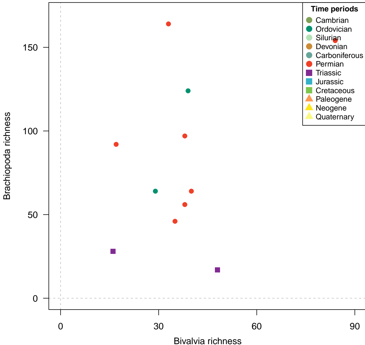
Genera, 200km grid cells, raw, 4 site minima, 1000km radius, 11 subsamples
