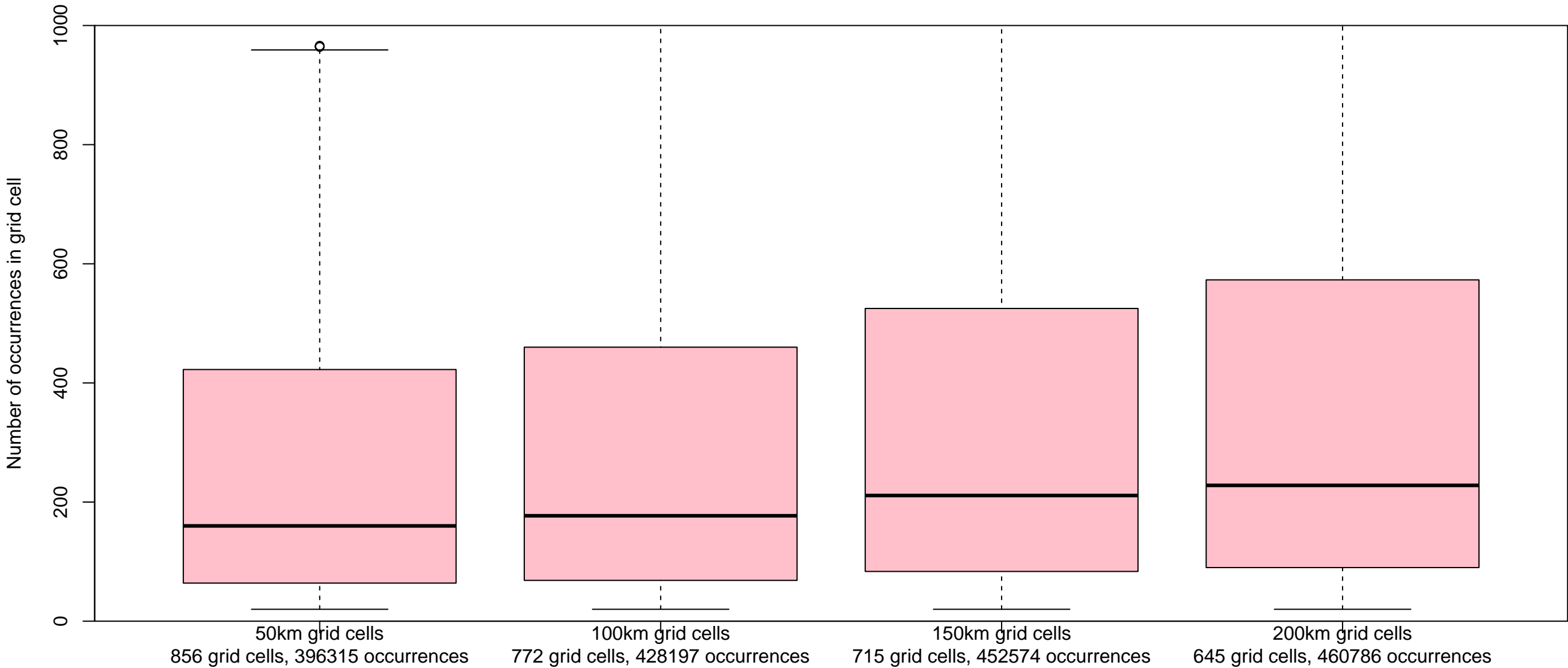
Number of occurrences in viable grid cells (y-axis capped at 1000 occurrences)
