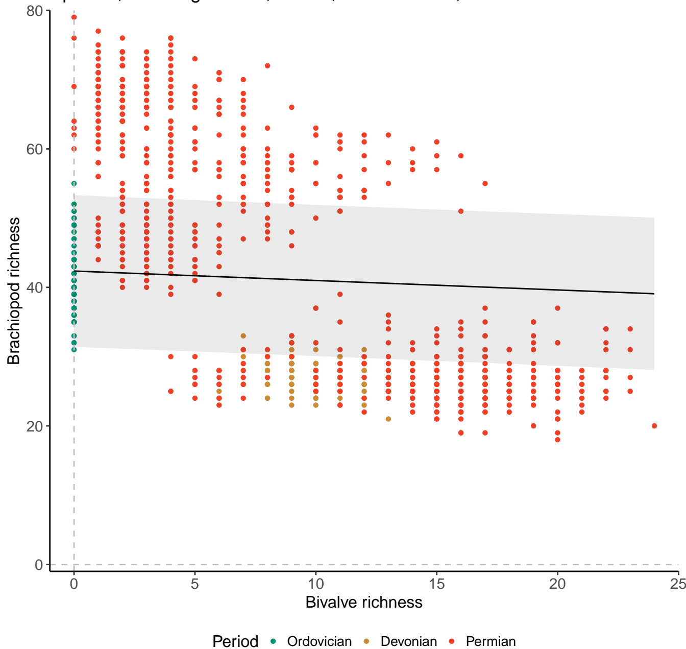
Species, 100km grid cells, 4 sites, 500km radius, Pre-PTME
