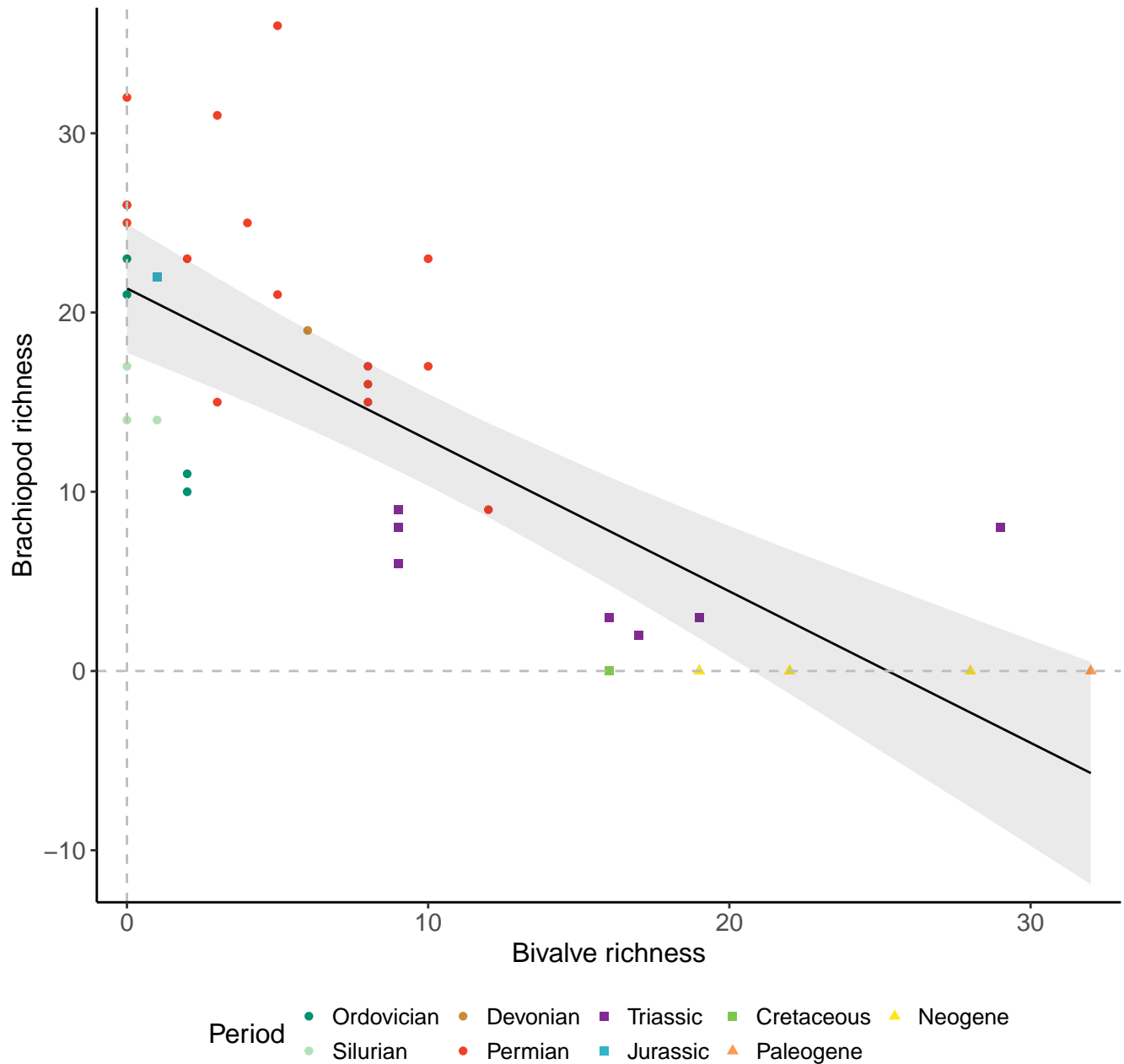
Species, 200km grid cells, 2 sites, 200km radius, median richness
