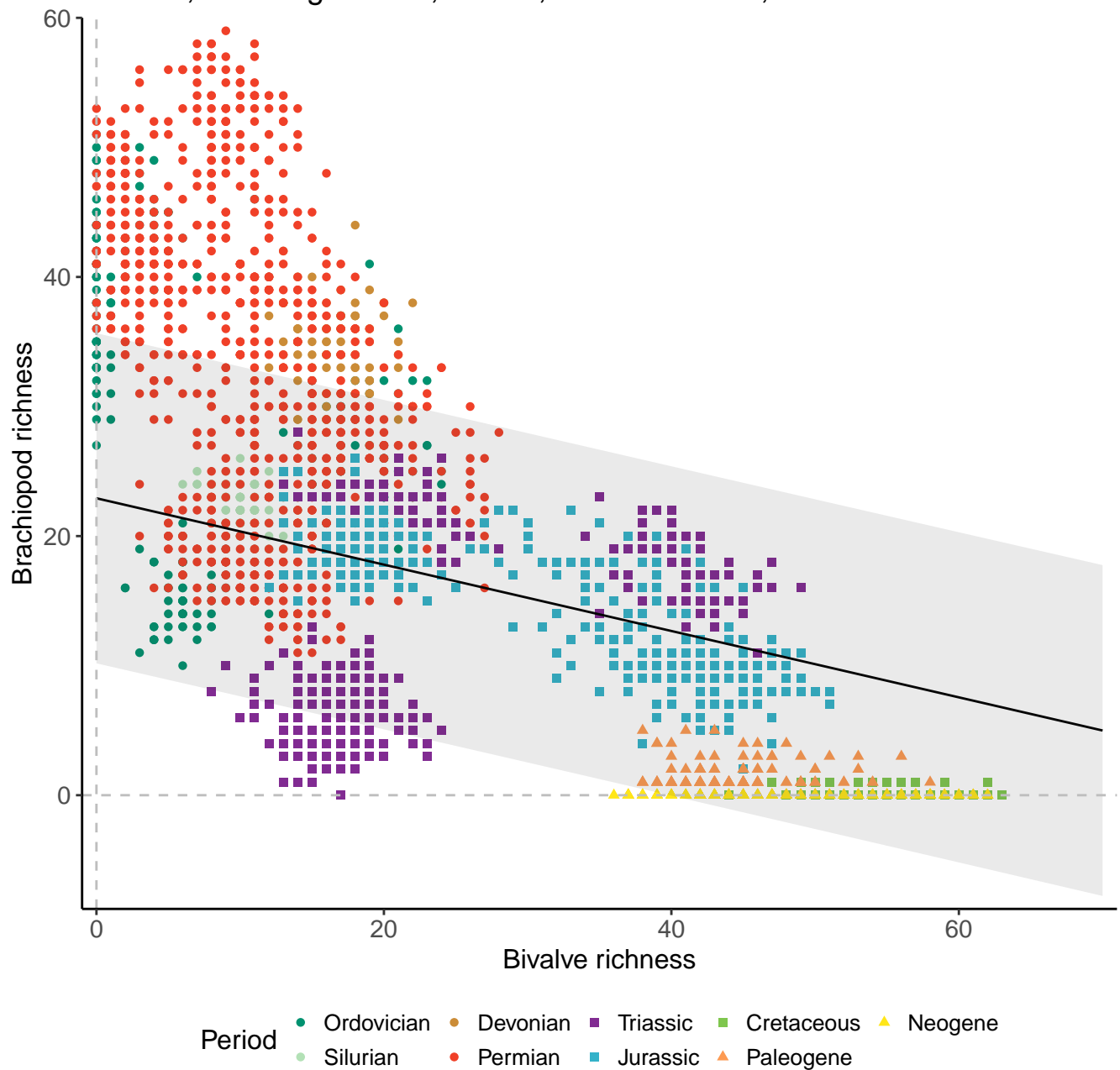
Genera, 200km grid cells, 3 sites, 1000km radius, eras as RE
