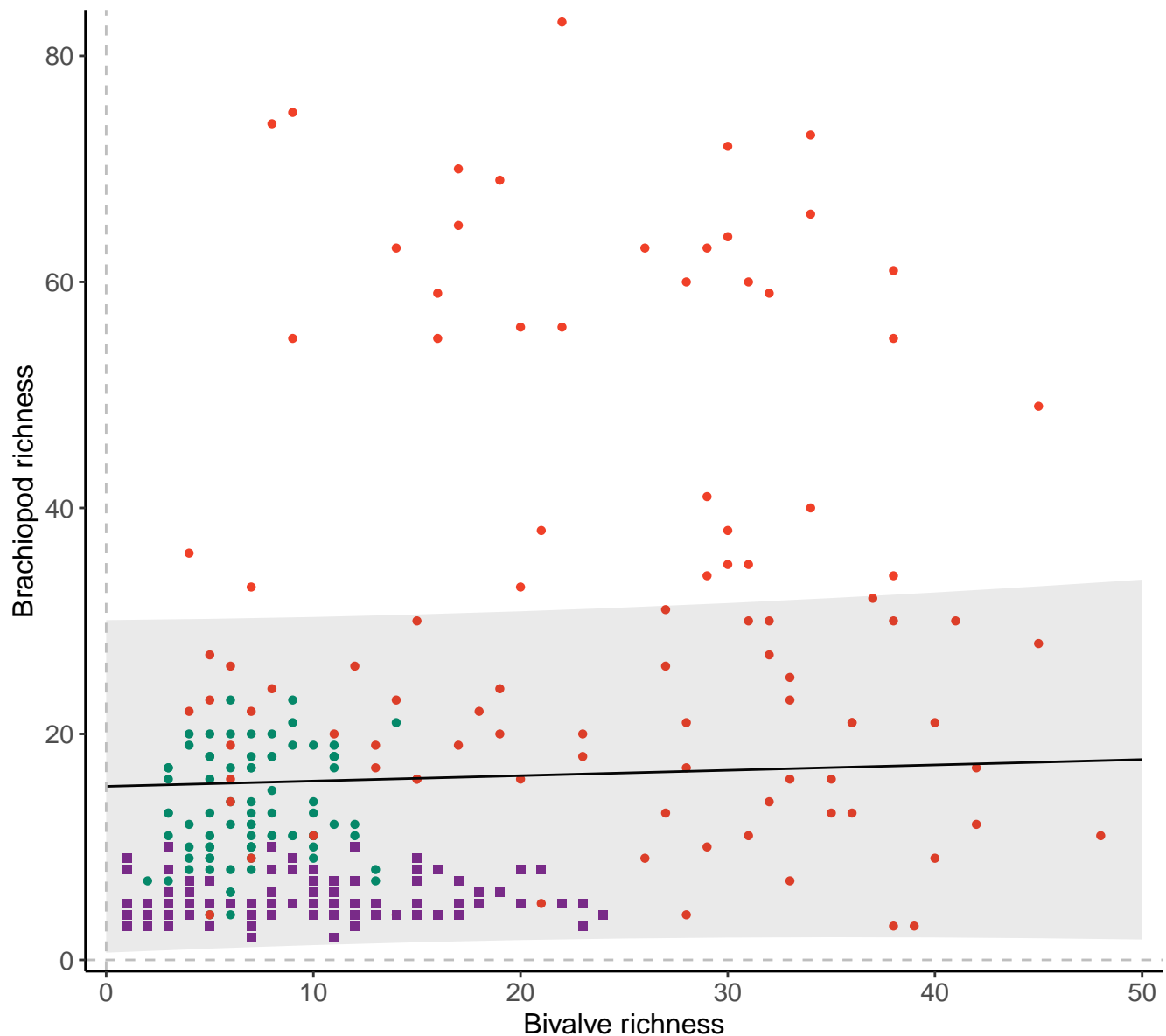
Genera, 200km grid cells, 5 sites, 1000km radius, simple model
