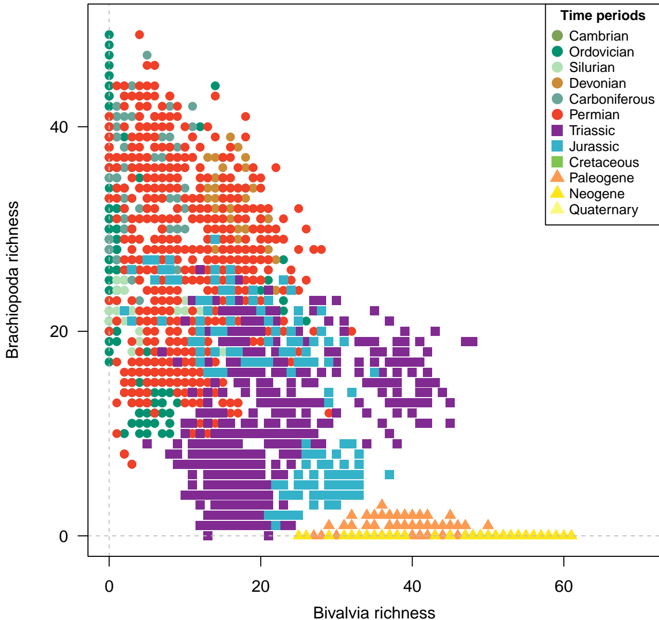
Genera, 200km grid cells, STO rarefaction, 3 site minima, 500km radius, 2600 subsamples
