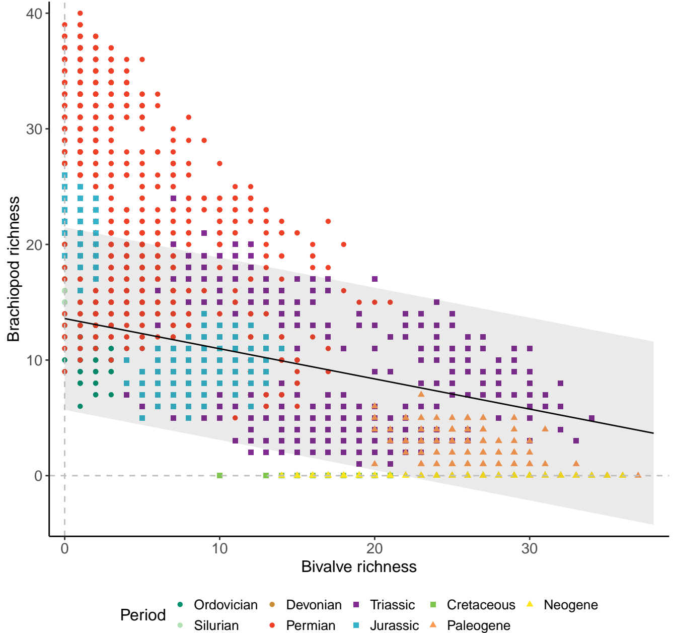
Species, 200km grid cells, 2 sites, 500km radius, eras as RE
