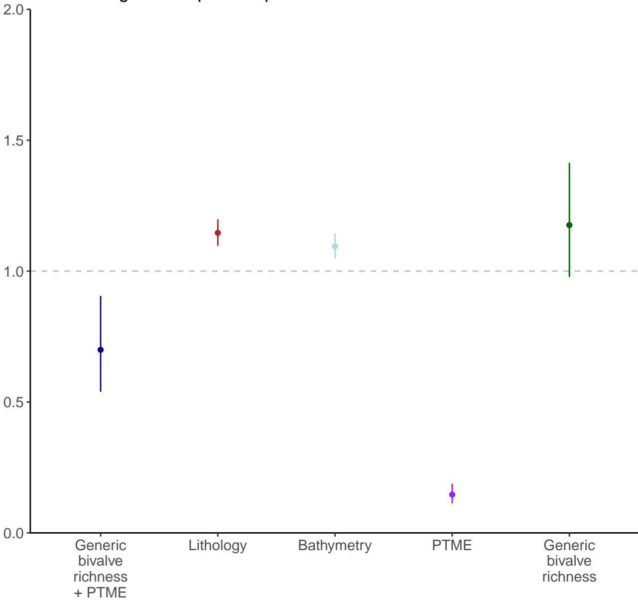
Model coefficients from raw occurrences Two 50km grid cells per sample
