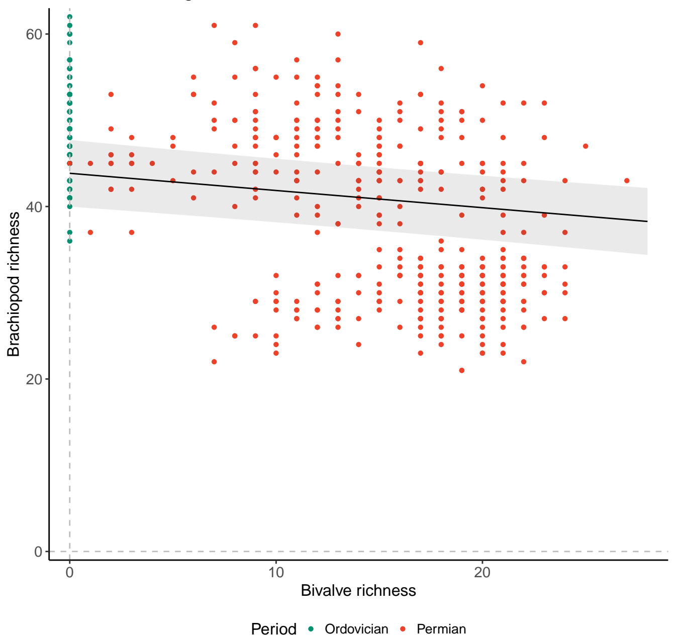
Genera, 100km grid cells, 5 sites, 500km radius, Paleozoic
