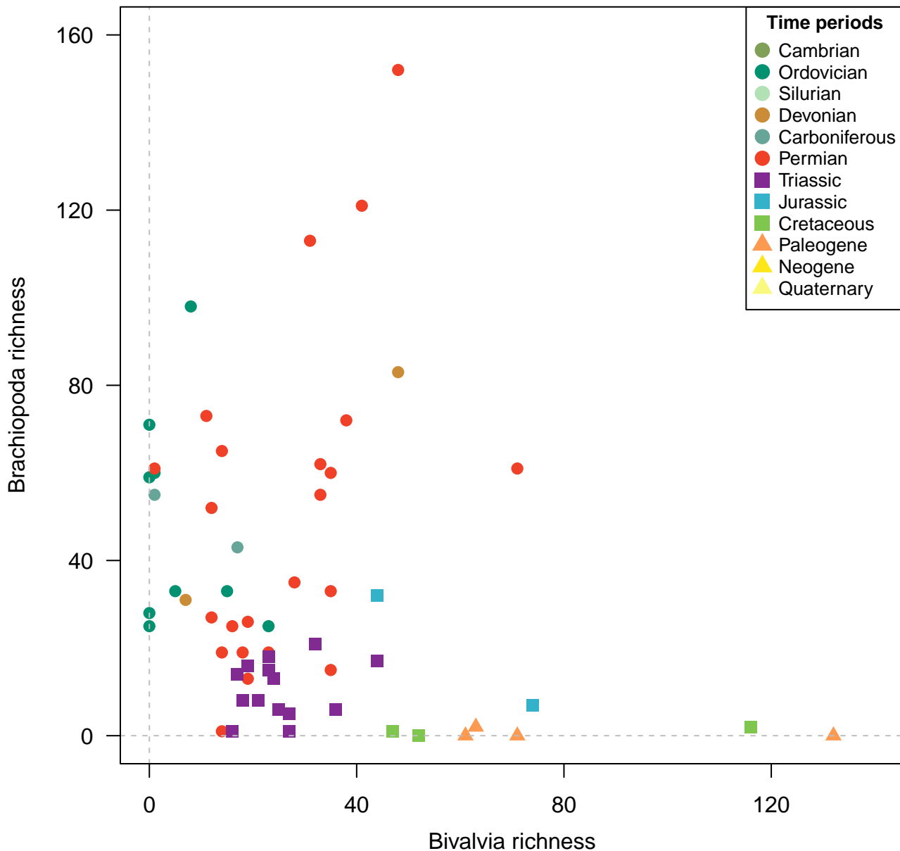
Genera, 200km grid cells, raw, 2 site minima, 200km radius, 61 subsamples
