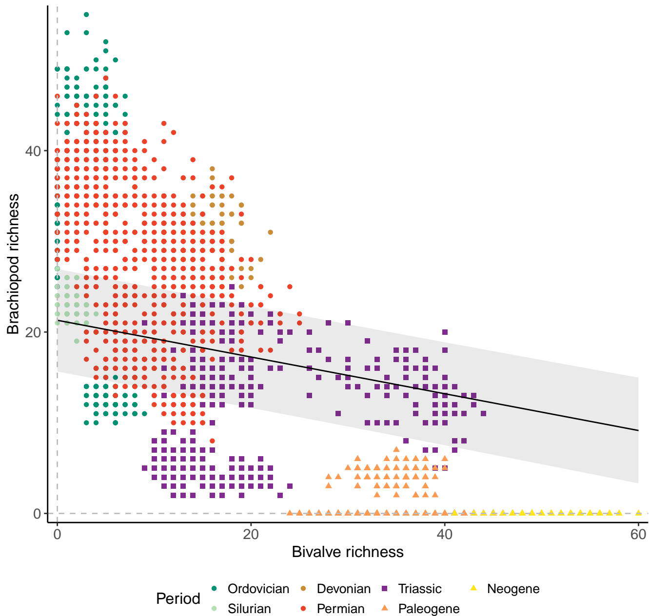
Genera, 100km grid cells, 3 sites, 500km radius, simple model
