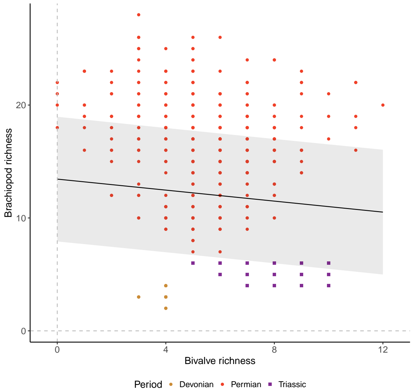
Genera, 100km grid cells, 4 sites, 500km radius, simple model
