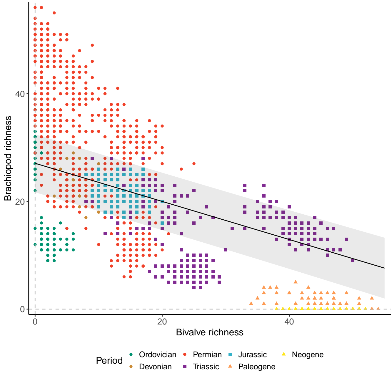
Species, 100km grid cells, 3 sites, 1000km radius, simple model
