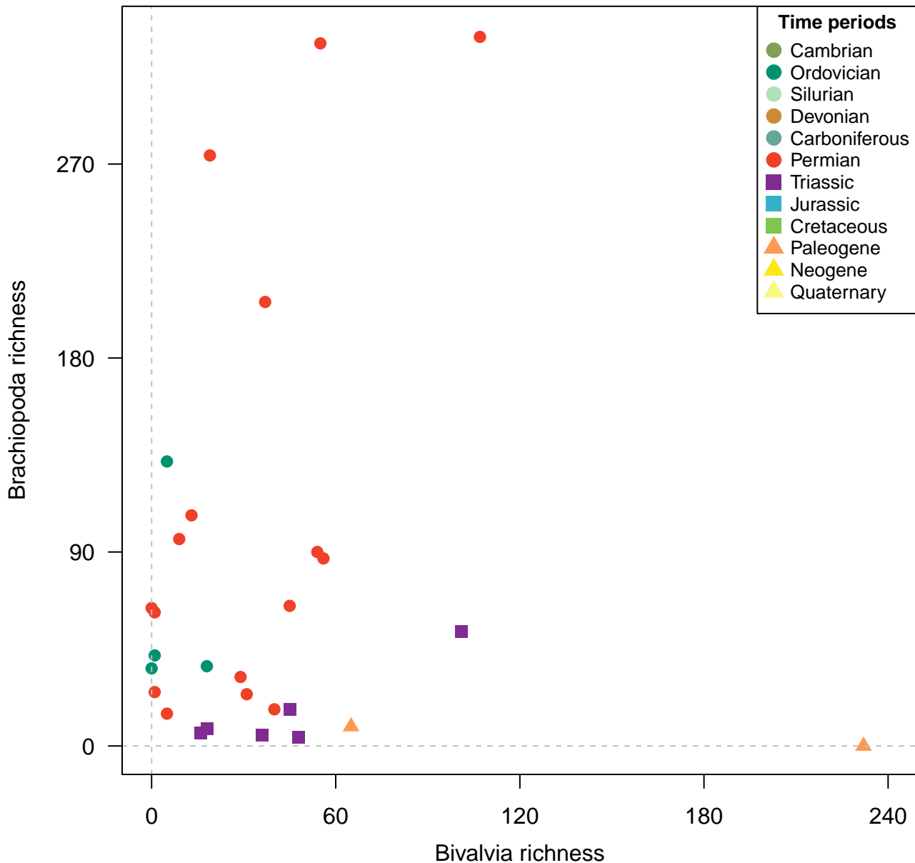
Species, 100km grid cells, raw, 2 site minima, 1000km radius, 28 subsamples
