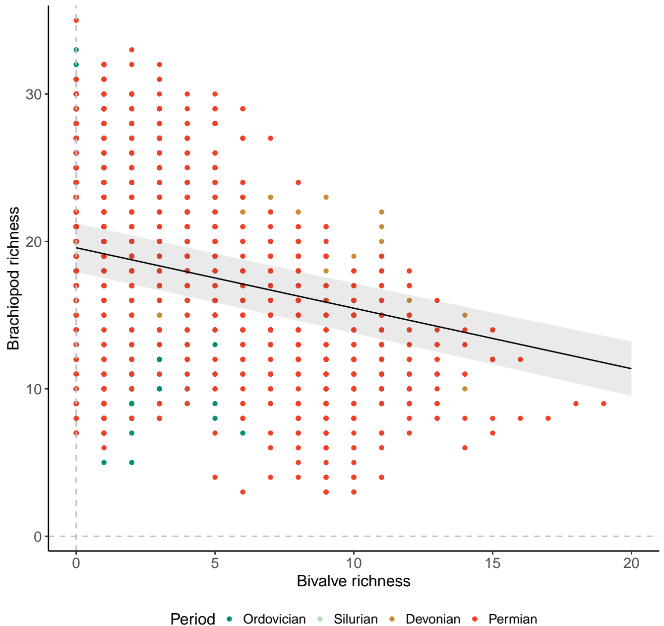
Genera, 100km grid cells, 2 sites, 1000km radius, Pre-PTME
