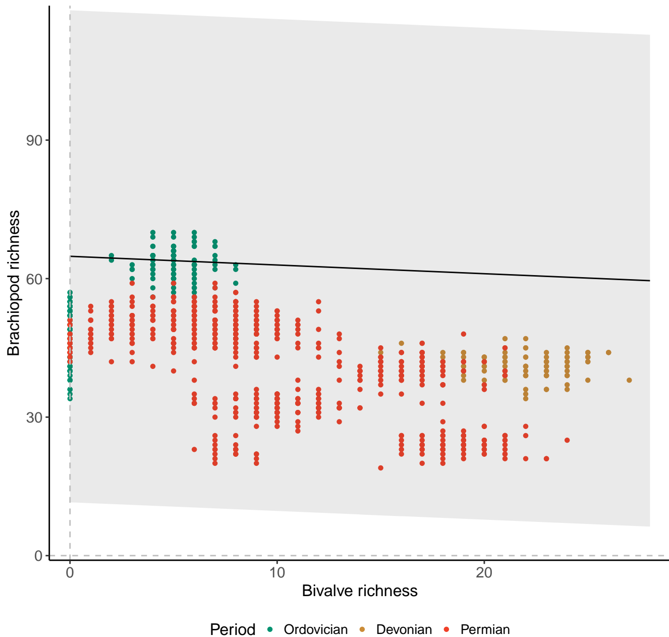
Genera, 100km grid cells, 4 sites, 200km radius, Pre-PTME
