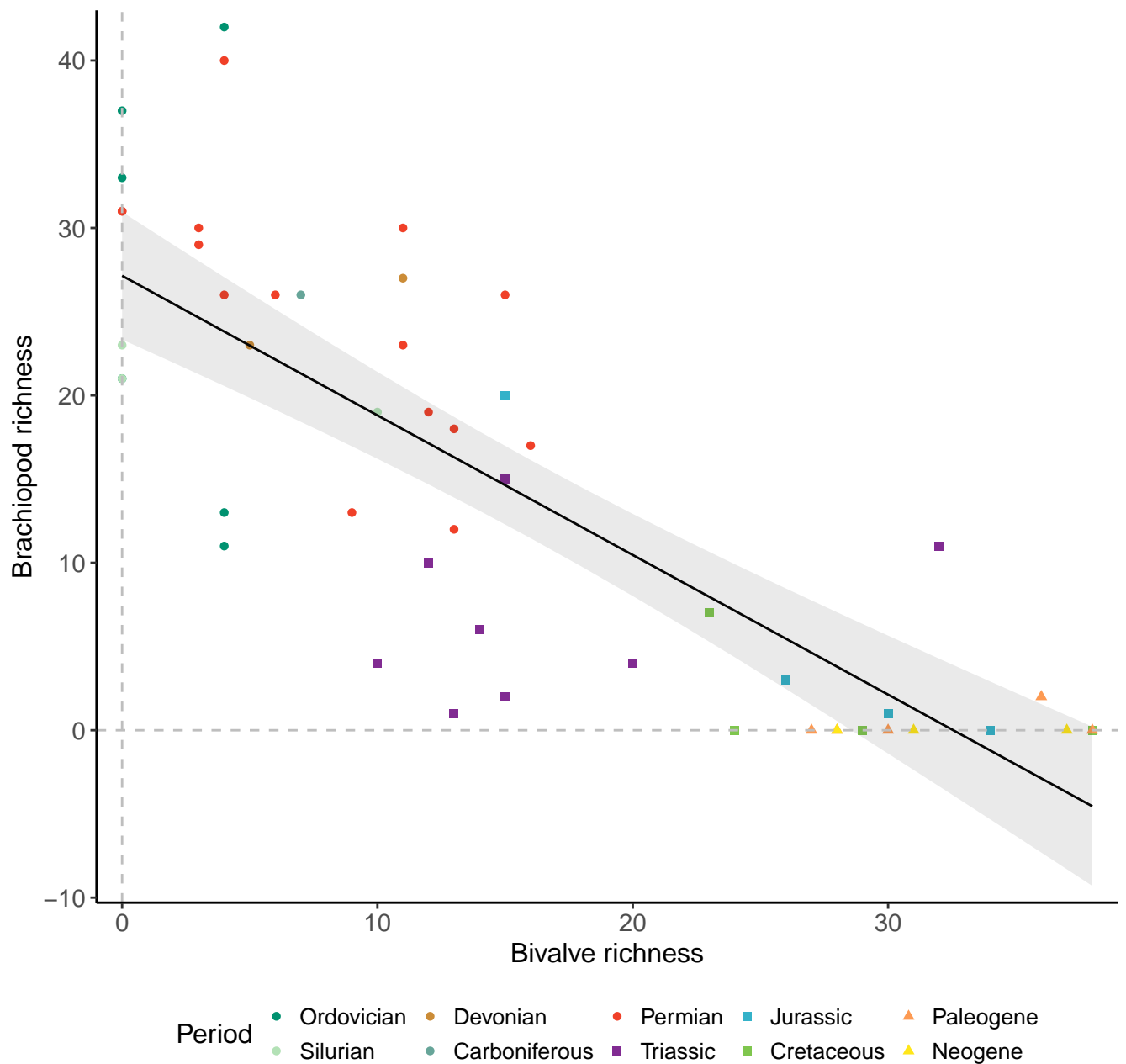
Genera, 200km grid cells, 2 sites, 200km radius, median richness
