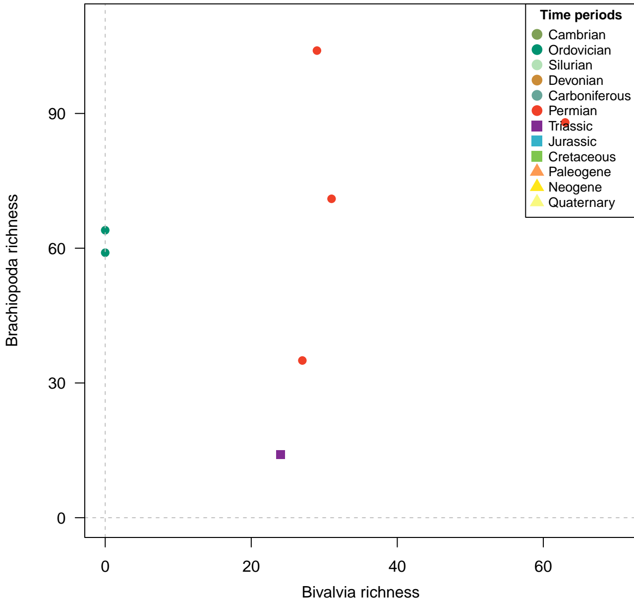
Genera, 100km grid cells, raw, 5 site minima, 200km radius, 7 subsamples
