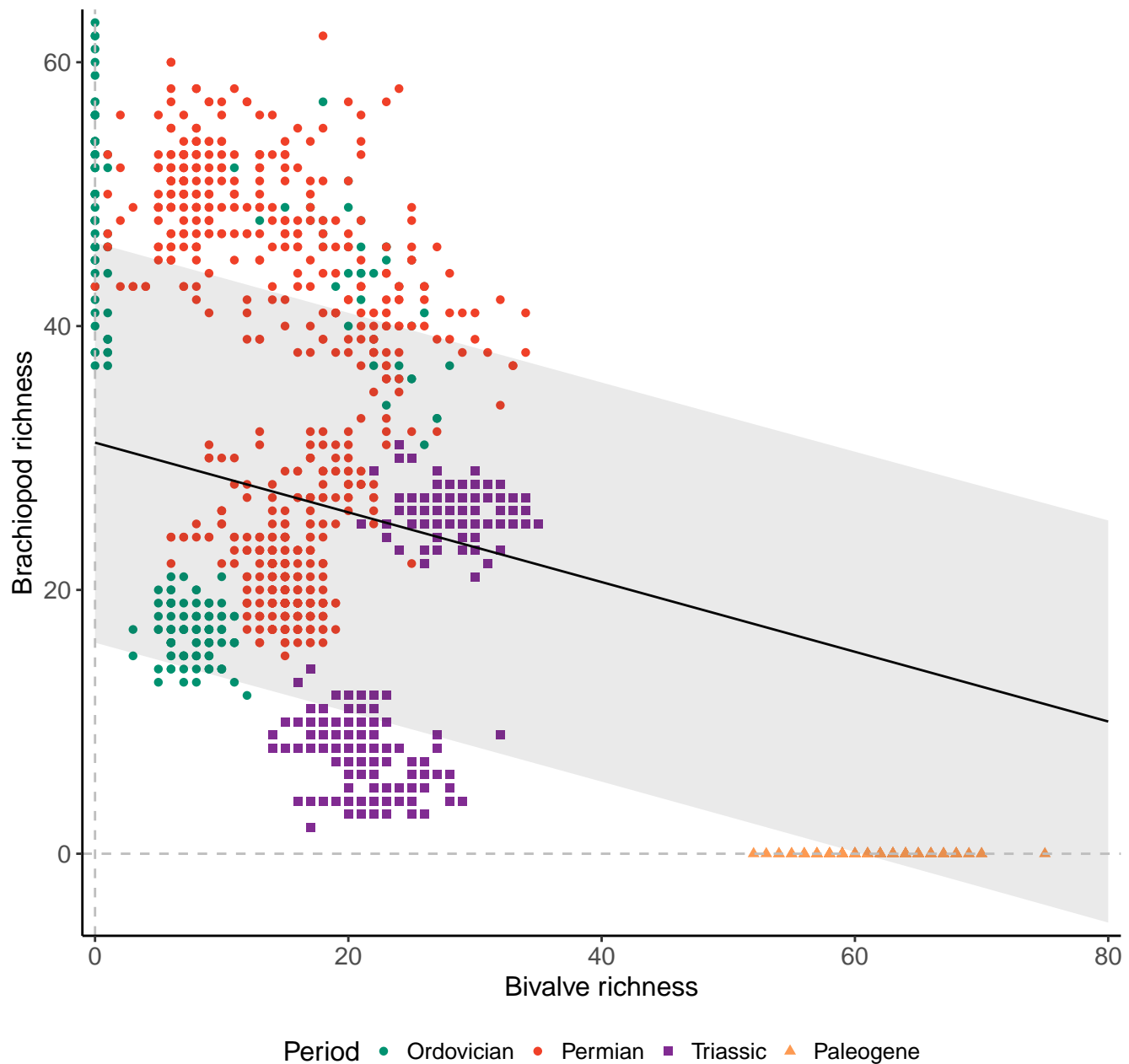
Genera, 200km grid cells, 4 sites, 500km radius, eras as RE
