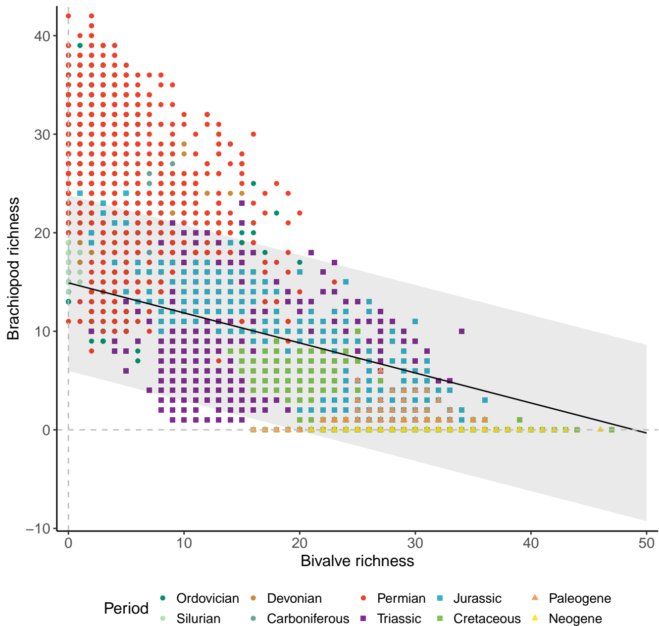
Genera, 200km grid cells, 2 sites, 1000km radius, PTME as RE
