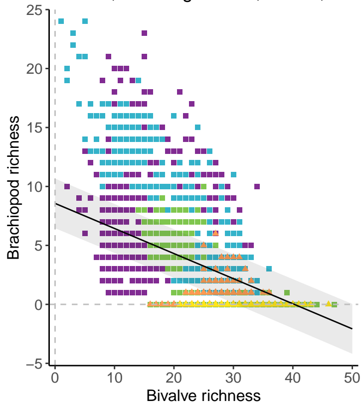
A Genera, 200km grid cells, 2 sites, 1000km radius, Post-PTME
