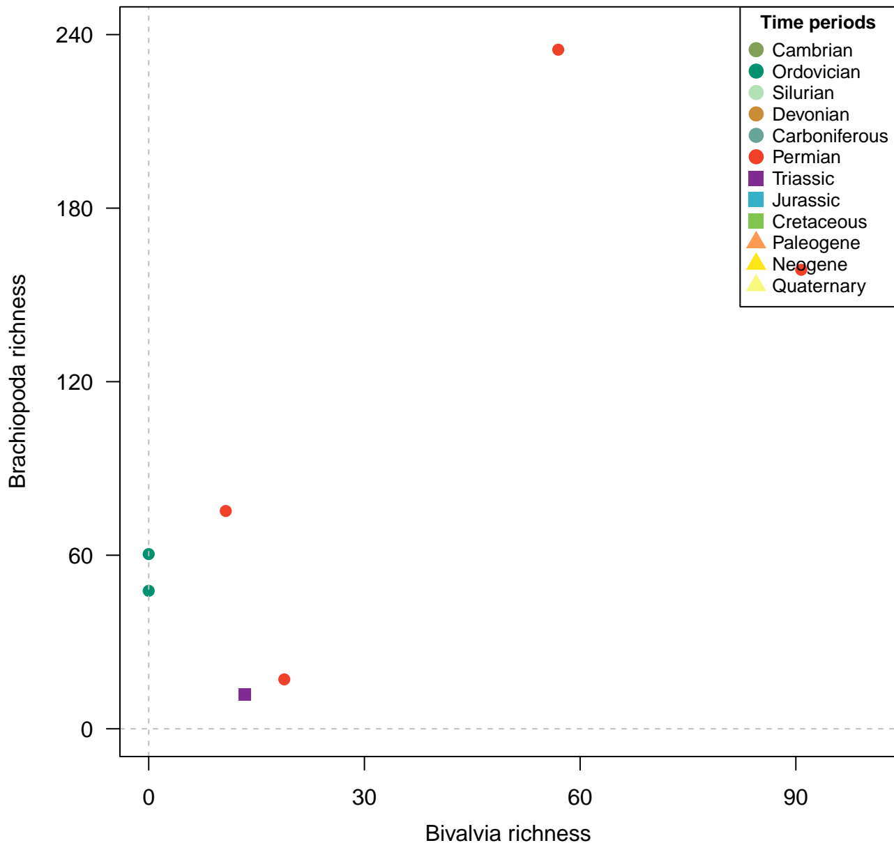
Species, 100km grid cells, SQS (q = 0.9), 3 site minima, 200km radius, 7 subsamples
