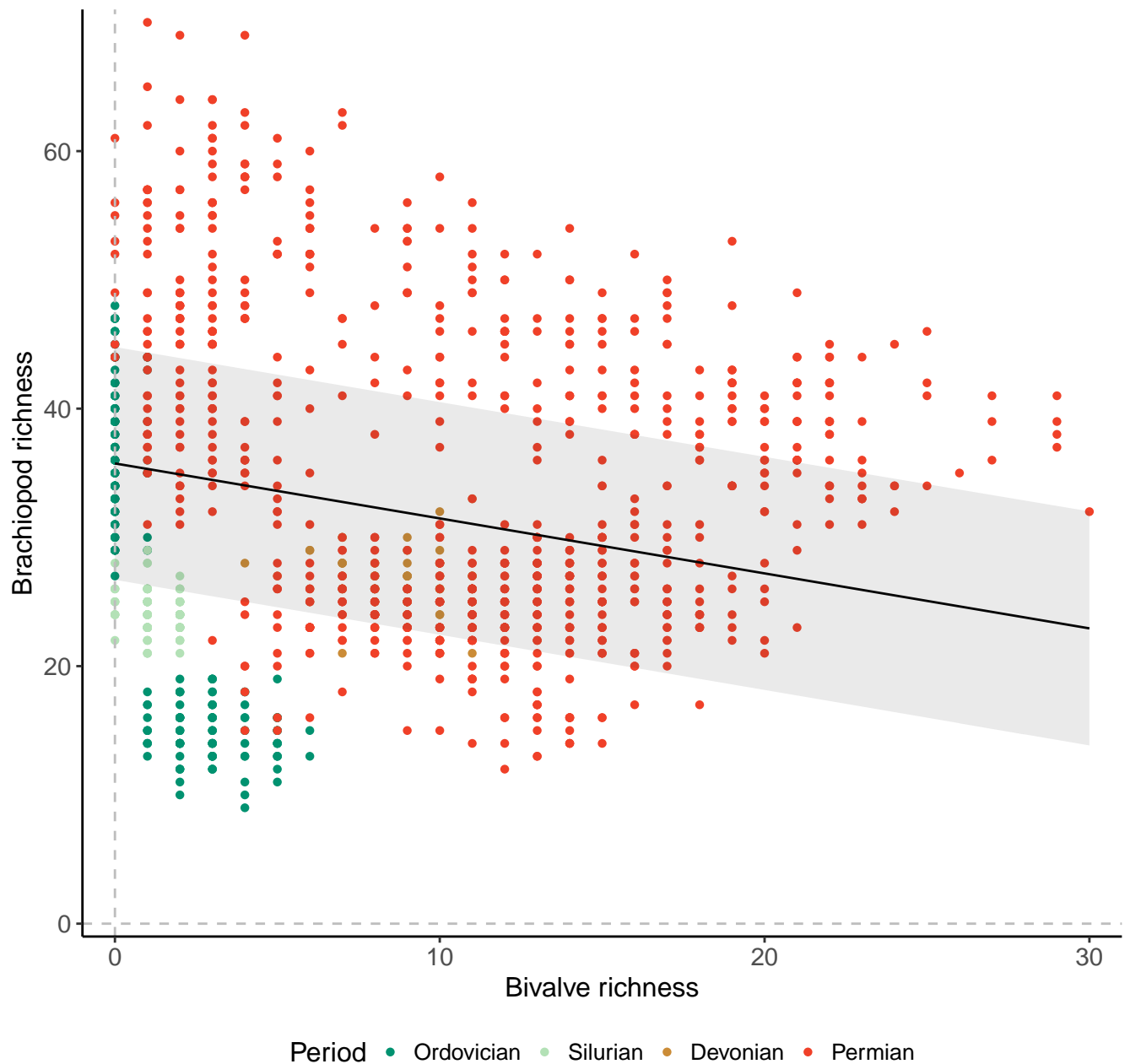
Species, 200km grid cells, 3 sites, 500km radius, Paleozoic
