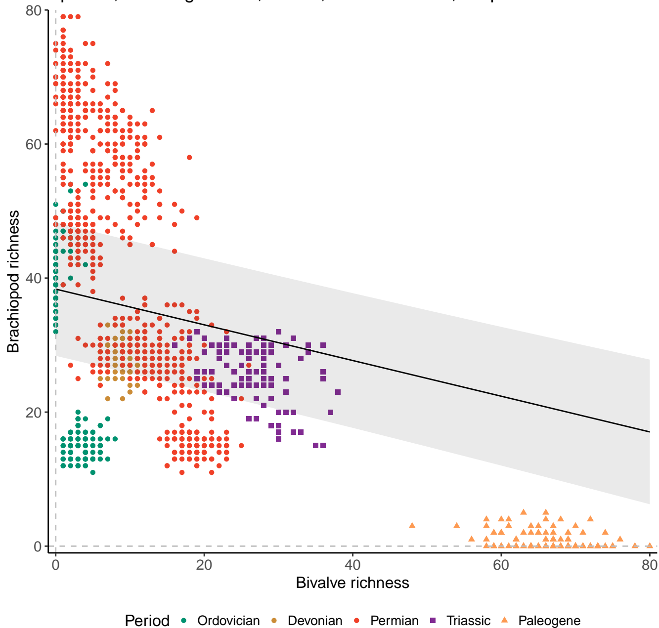
Species, 100km grid cells, 4 sites, 1000km radius, simple model
