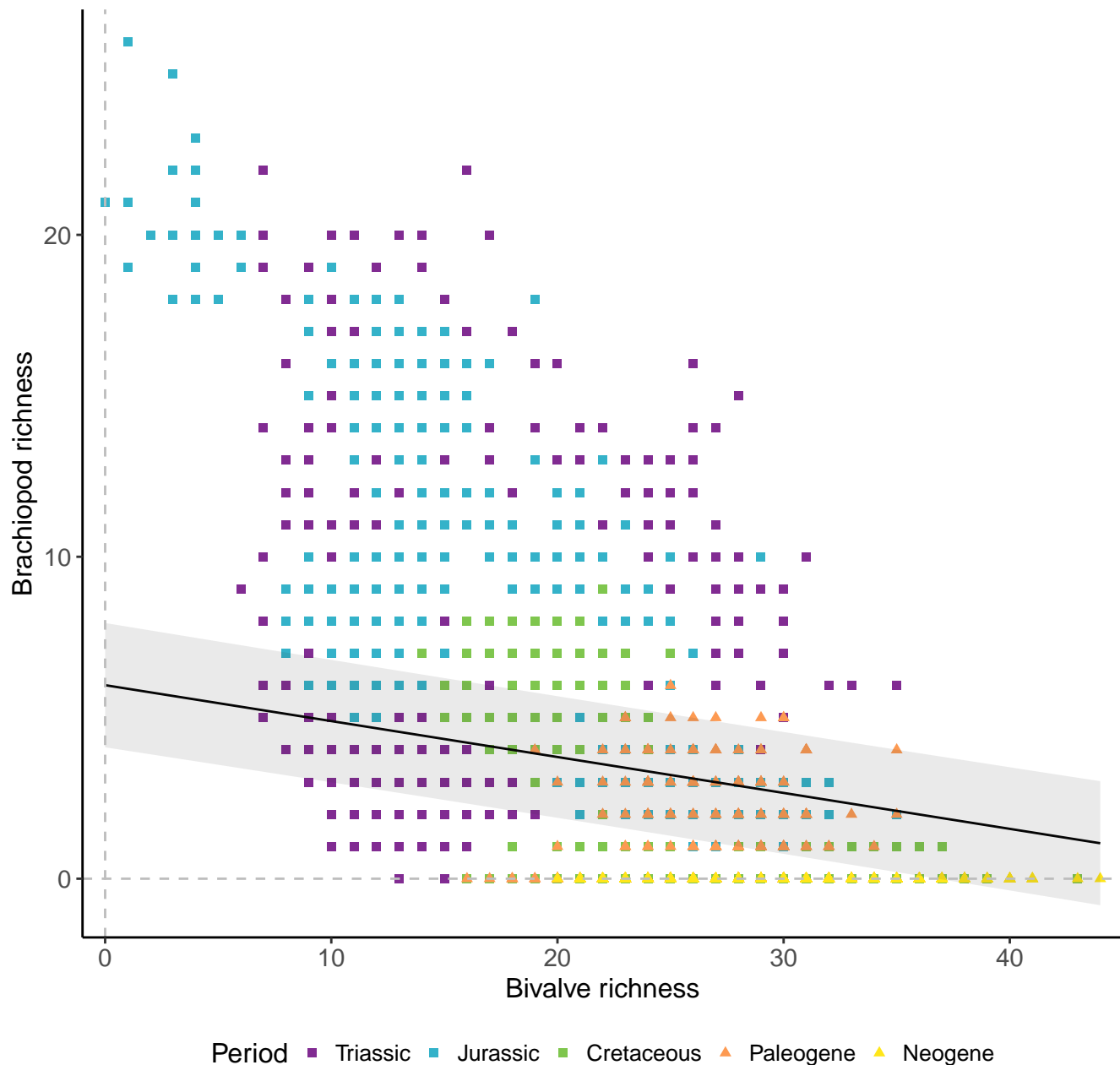
Genera, 200km grid cells, 2 sites, 500km radius, Post-PTME
