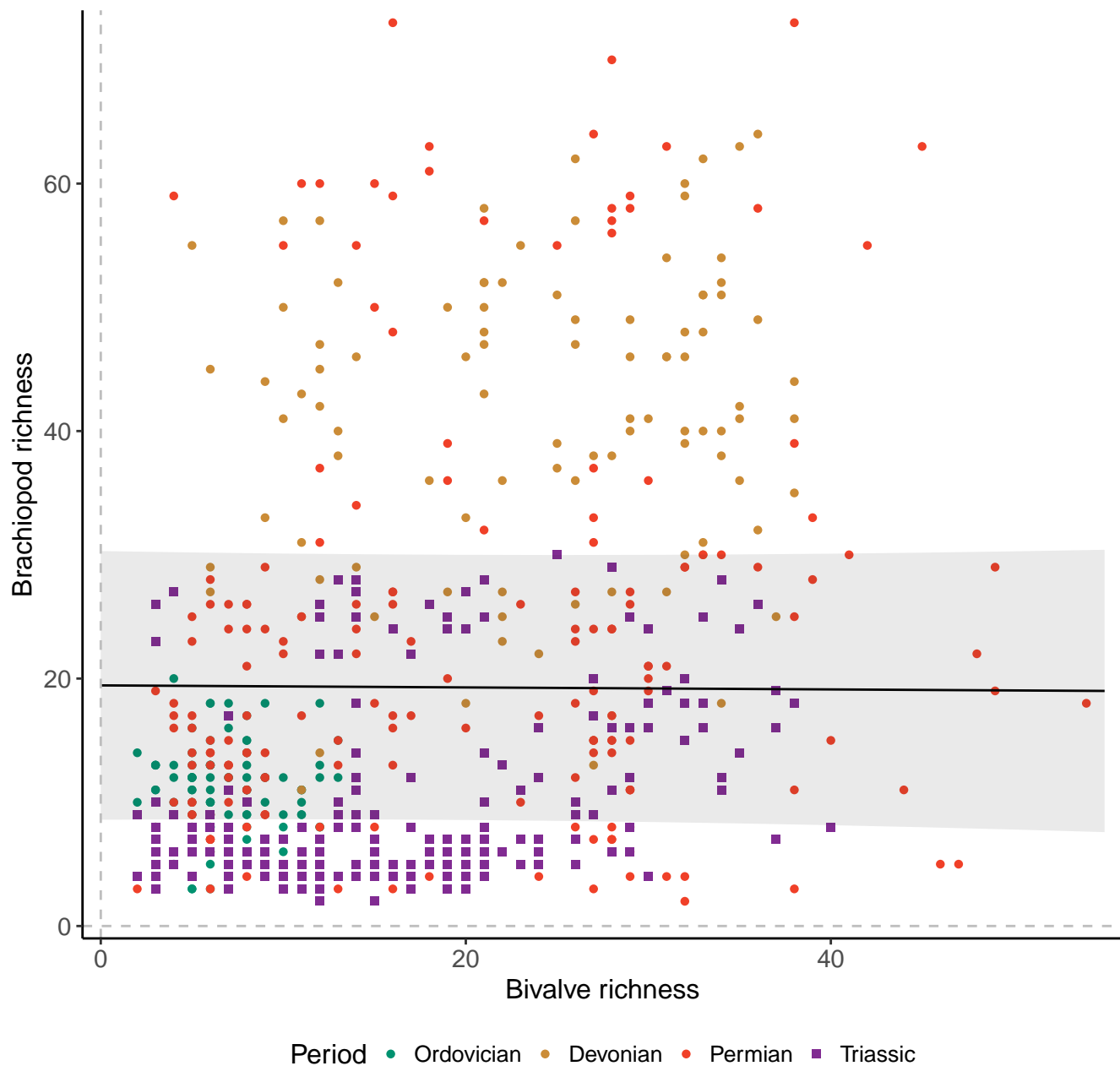
Genera, 200km grid cells, 3 sites, 500km radius, simple model
