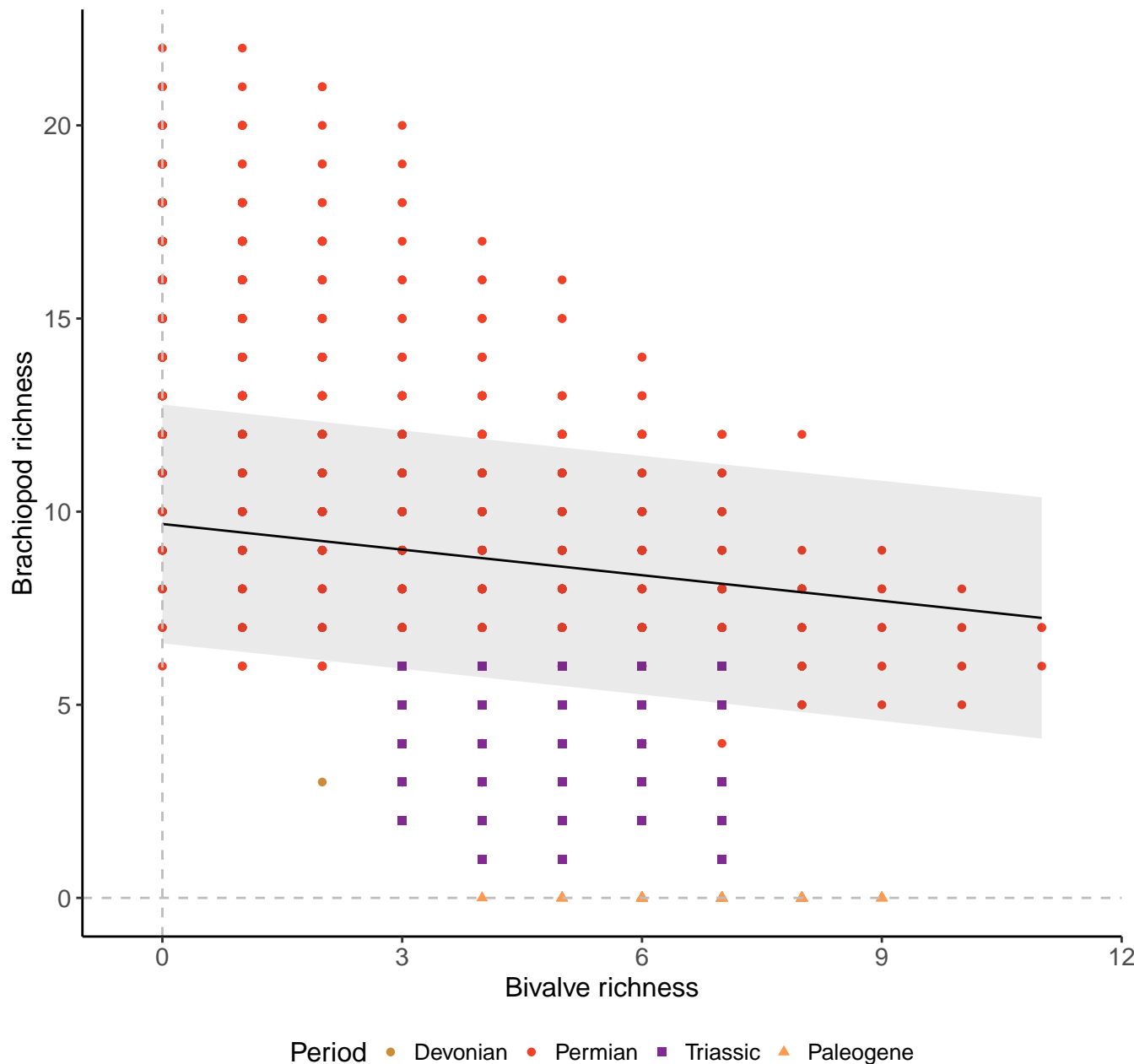
Genera, 100km grid cells, 2 sites, 200km radius, simple model
