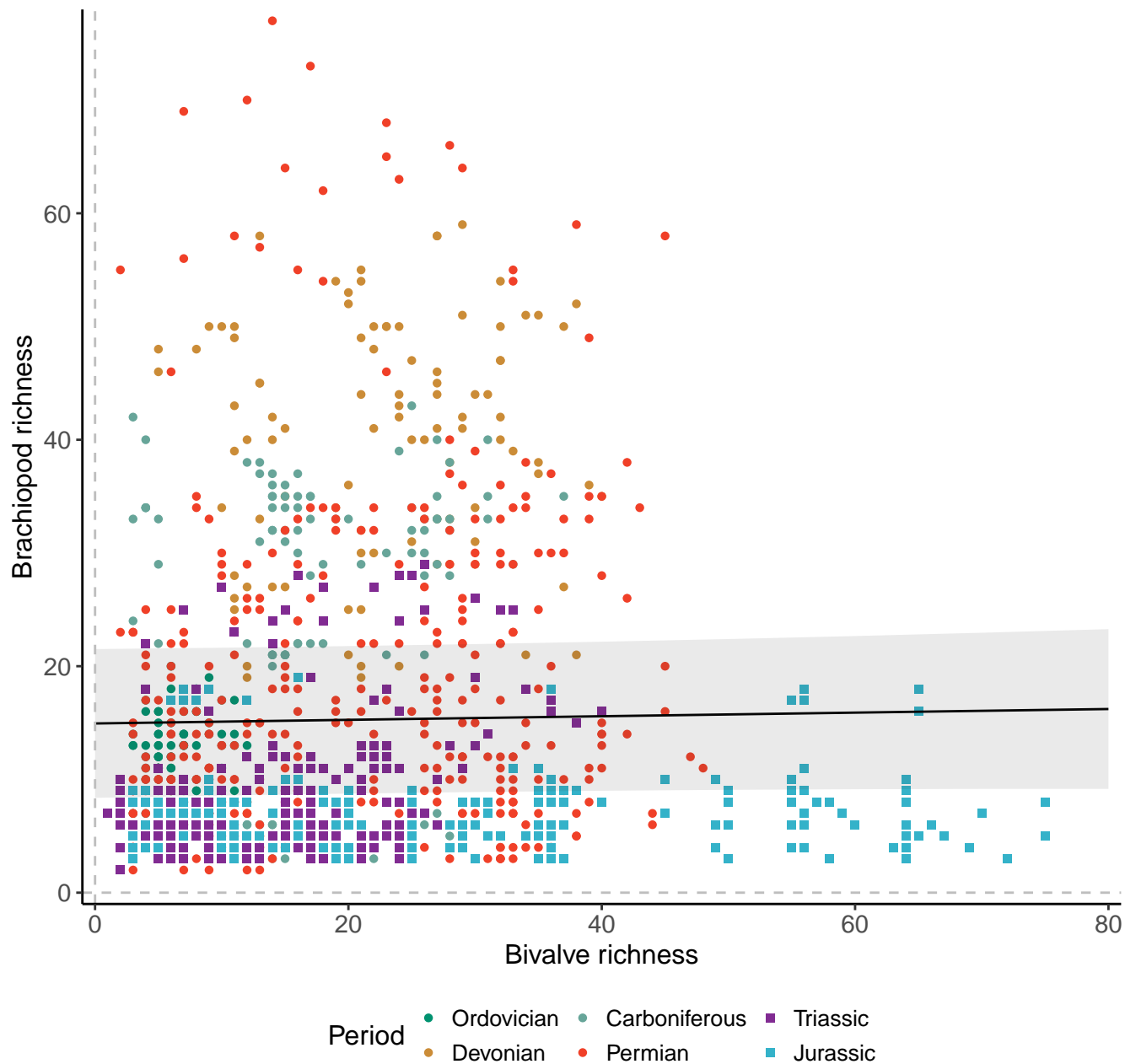
Genera, 200km grid cells, 3 sites, 1000km radius, simple model
