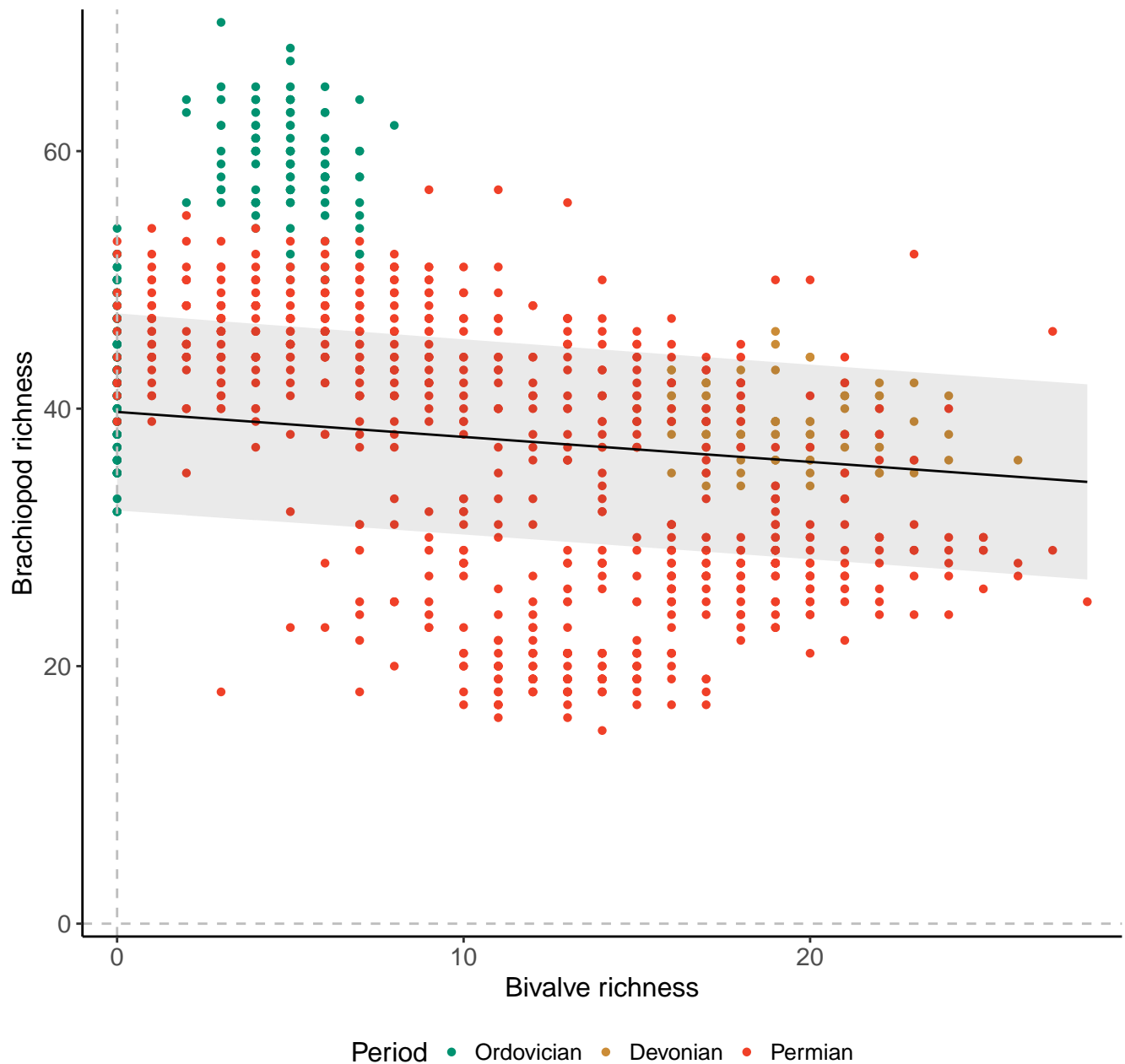
Genera, 100km grid cells, 4 sites, 500km radius, Paleozoic
