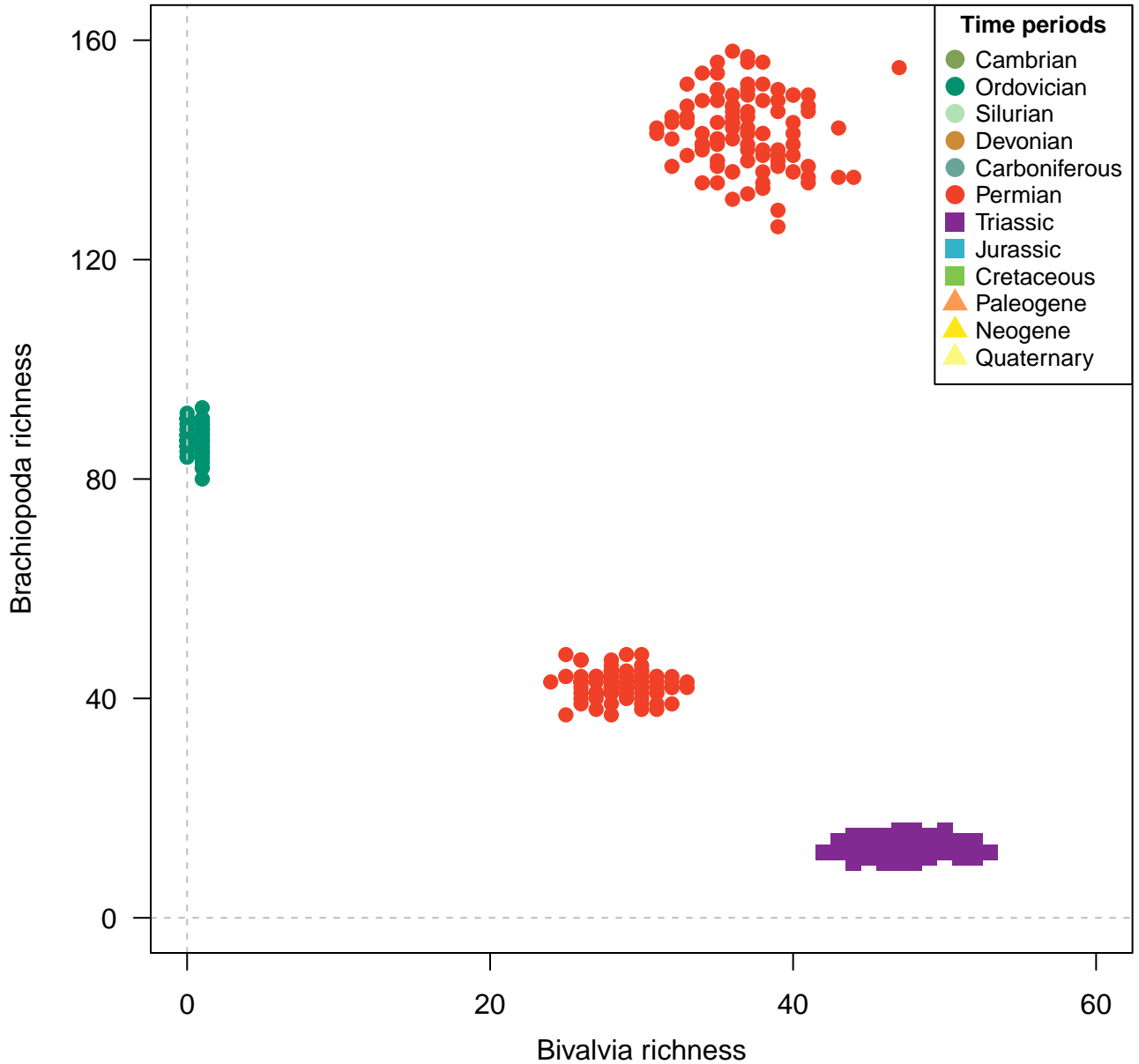
Species, 200km grid cells, STO rarefaction, 4 site minima, 200km radius, 500 subsamples
