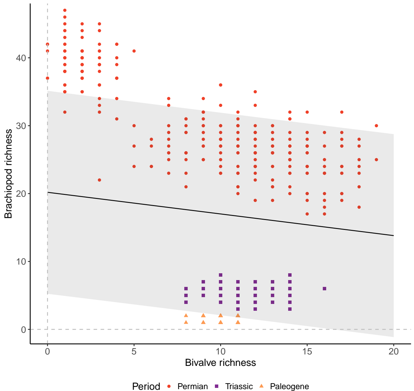
Genera, 200km grid cells, 5 sites, 1000km radius, simple model
