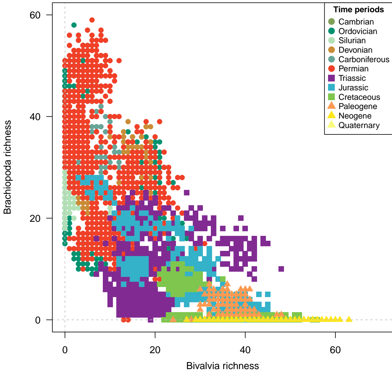
Genera, 200km grid cells, STO rarefaction, 2 site minima, 500km radius, 6300 subsamples
