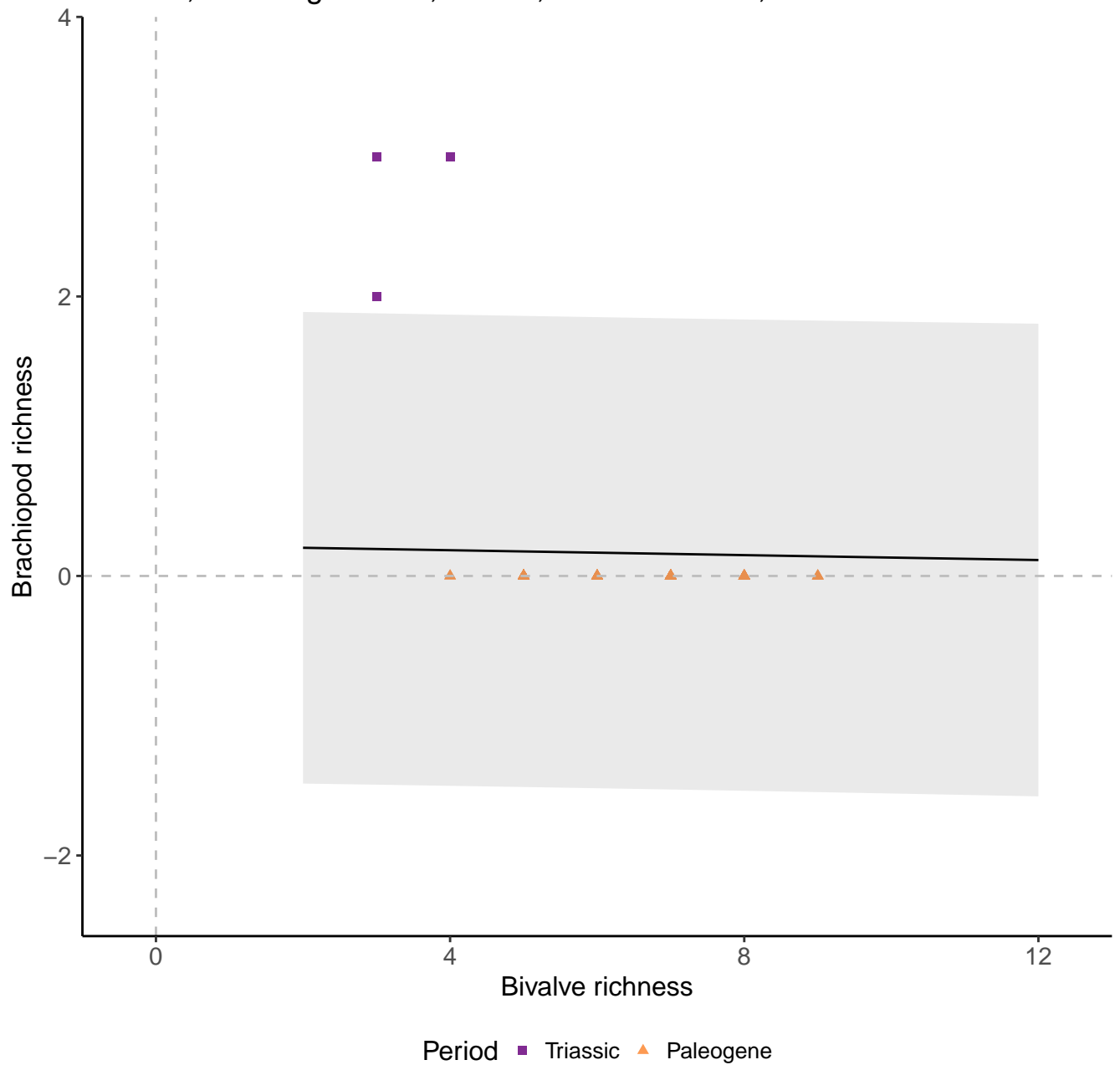
Genera, 200km grid cells, 3 sites, 1000km radius, full model
