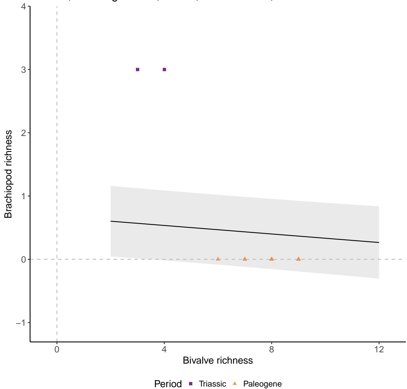
Genera, 200km grid cells, 4 sites, 500km radius, full model
