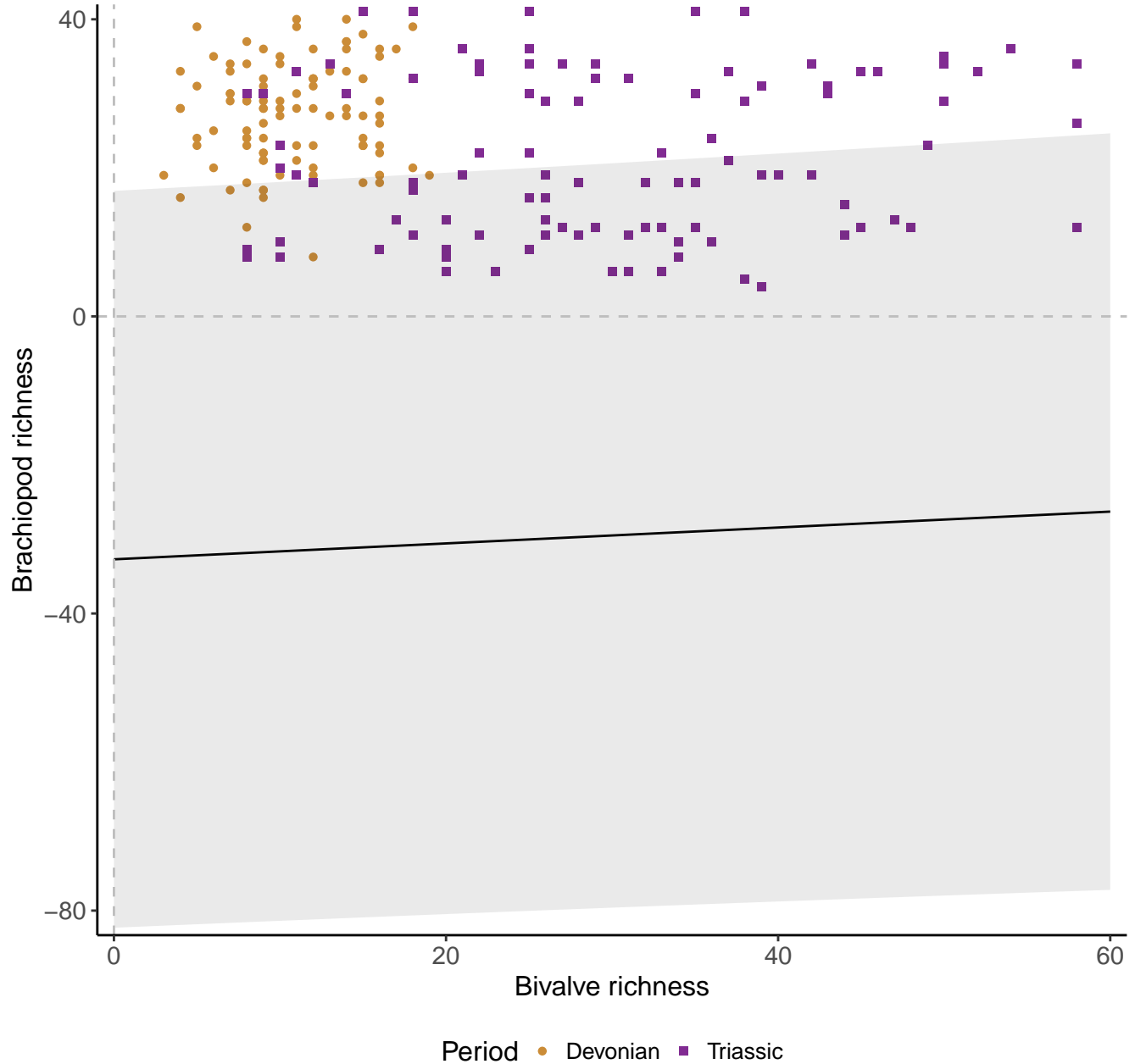
Species, 100km grid cells, 5 sites, 500km radius, full model
