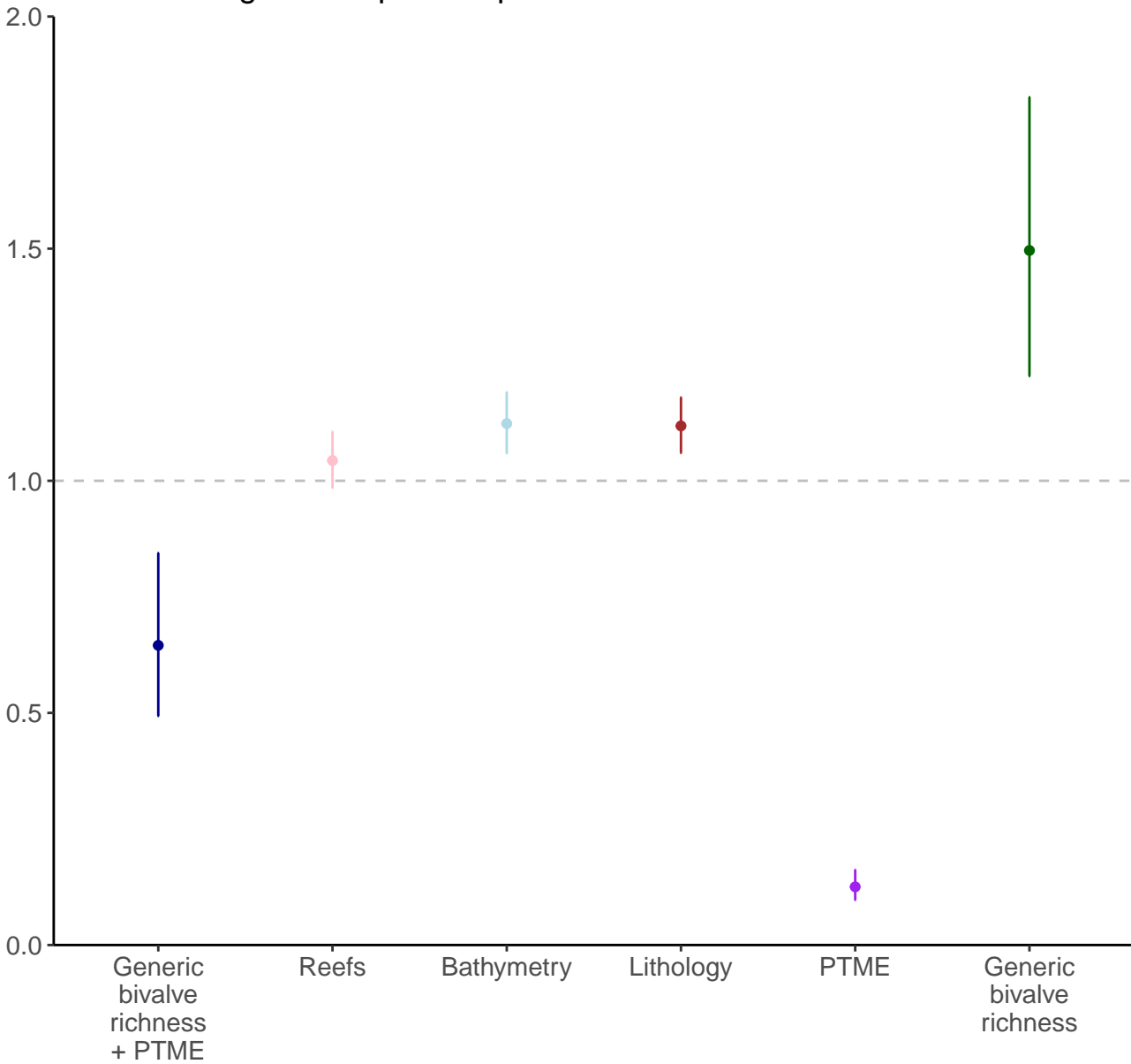
Model coefficients from raw occurrences Three 50km grid cells per sample
