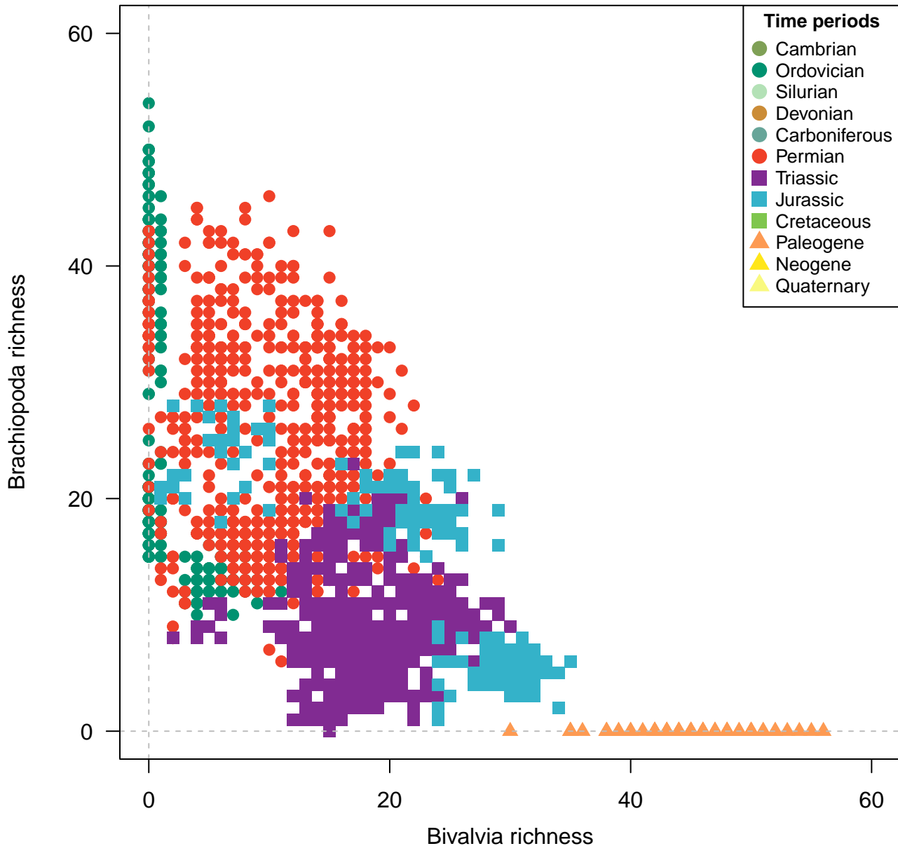
Genera, 200km grid cells, STO rarefaction, 3 site minima, 200km radius, 1900 subsamples
