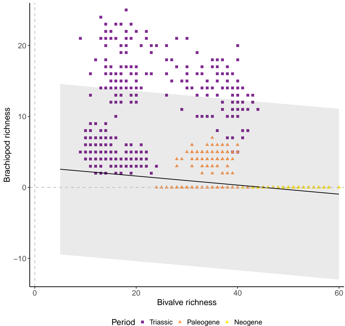
Genera, 100km grid cells, 3 sites, 500km radius, Post-PTME
