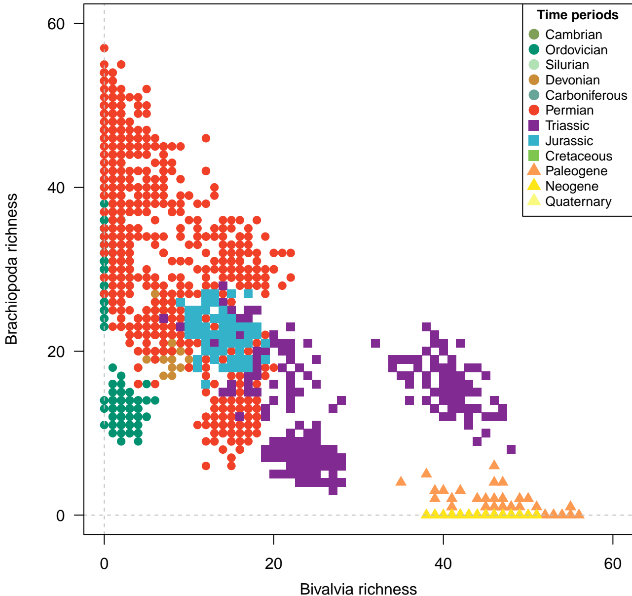
Species, 100km grid cells, STO rarefaction, 3 site minima, 1000km radius, 1700 subsamples
