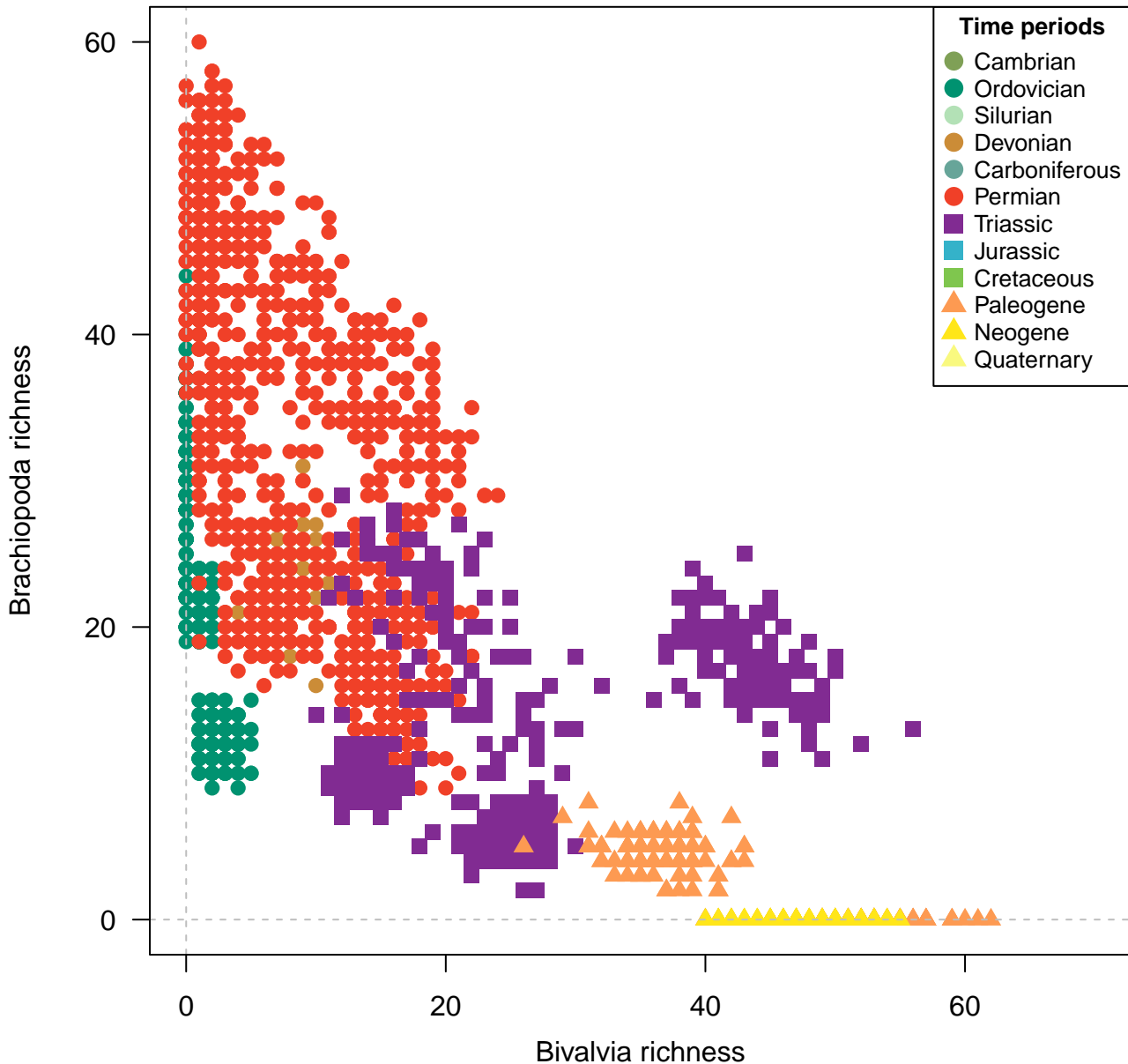
Species, 100km grid cells, STO rarefaction, 3 site minima, 500km radius, 2000 subsamples
