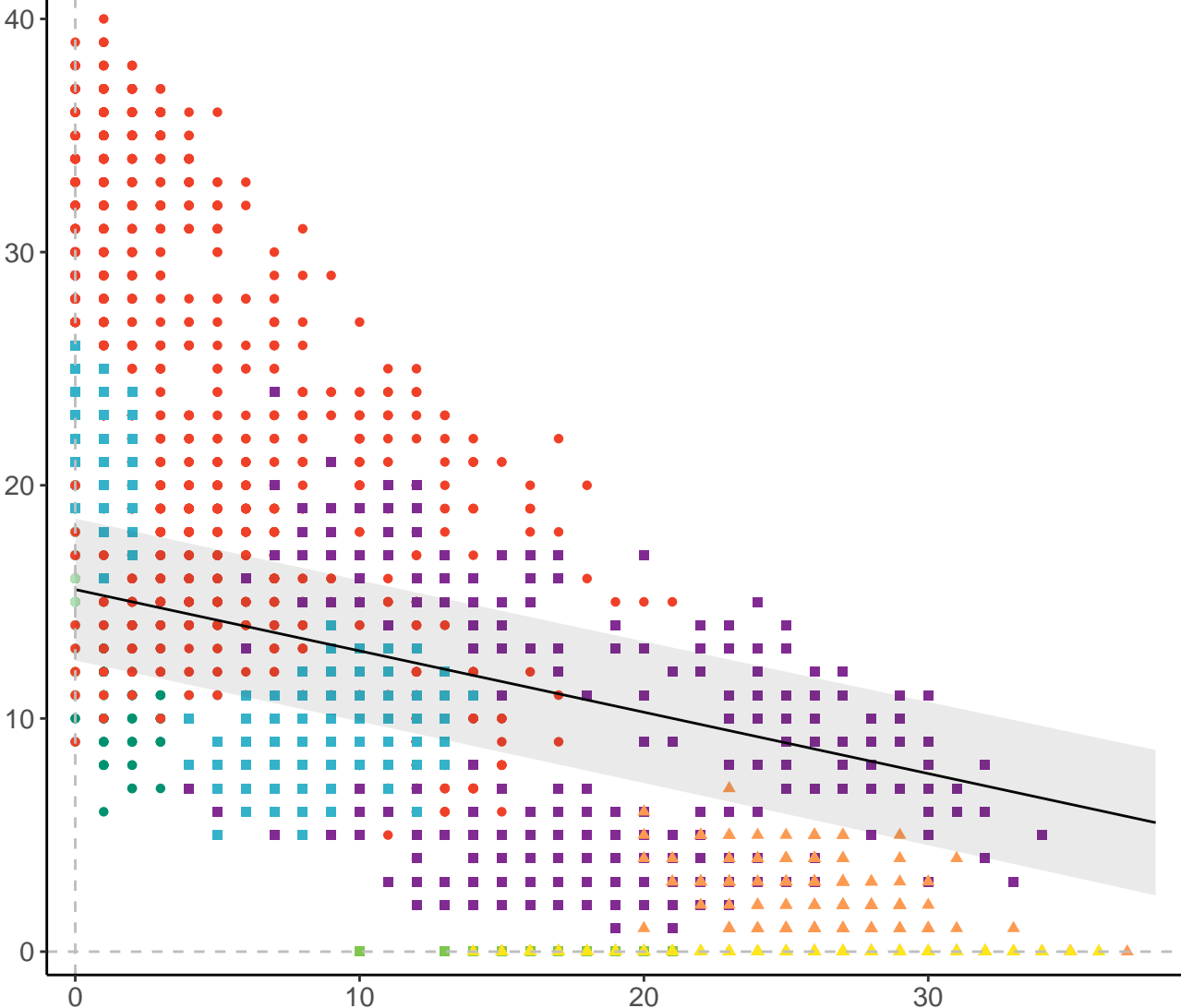
Species, 200km grid cells, 2 sites, 500km radius, full model
