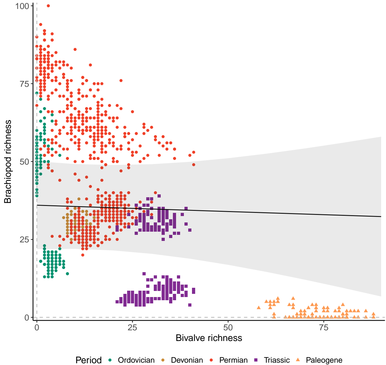
Species, 200km grid cells, 4 sites, 1000km radius
