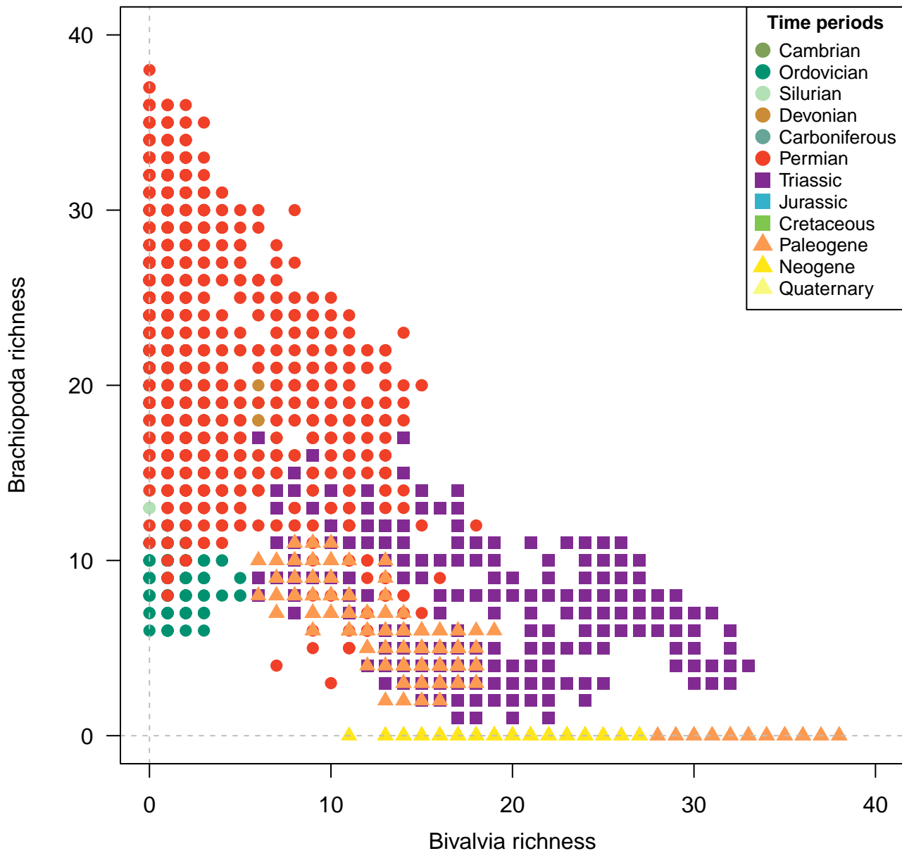
Species, 100km grid cells, STO rarefaction, 2 site minima, 200km radius, 3500 subsamples
