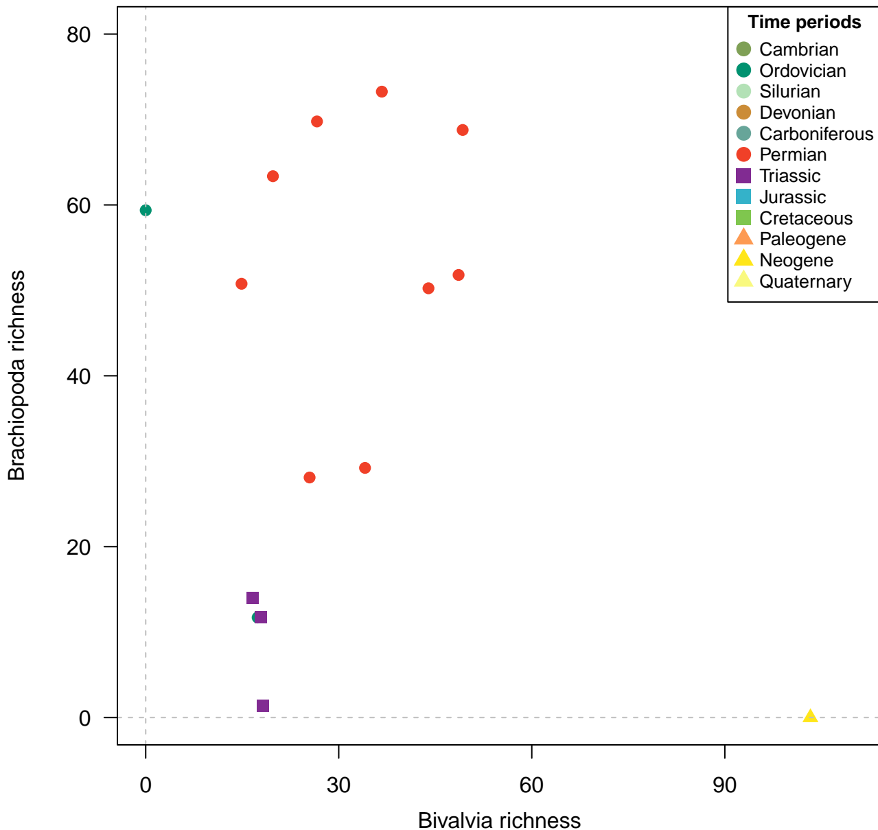
Genera, 200km grid cells, SQS (q = 0.9), 3 site minima, 500km radius, 15 subsamples
