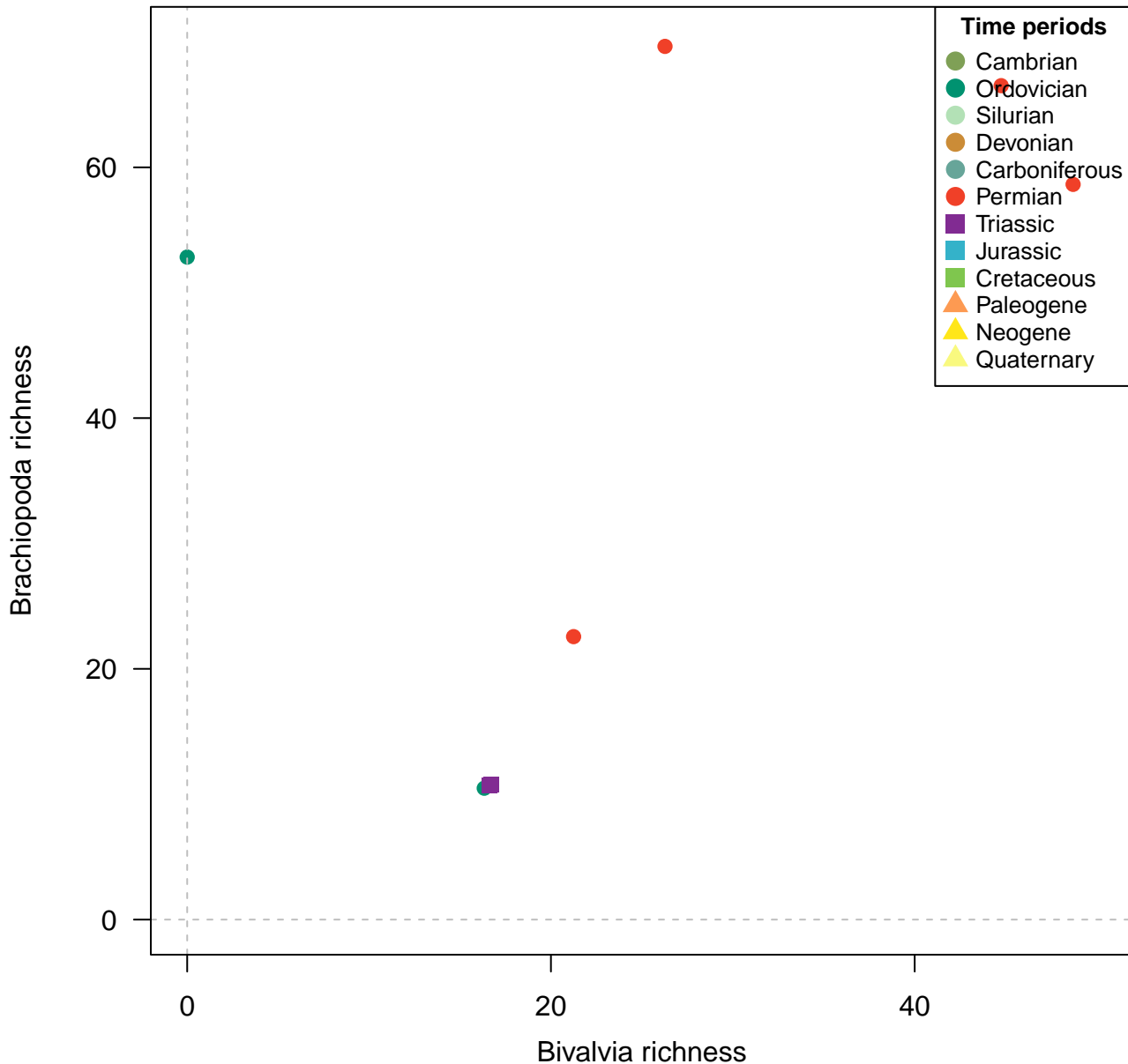
Genera, 200km grid cells, SQS (q = 0.9), 4 site minima, 200km radius, 8 subsamples
