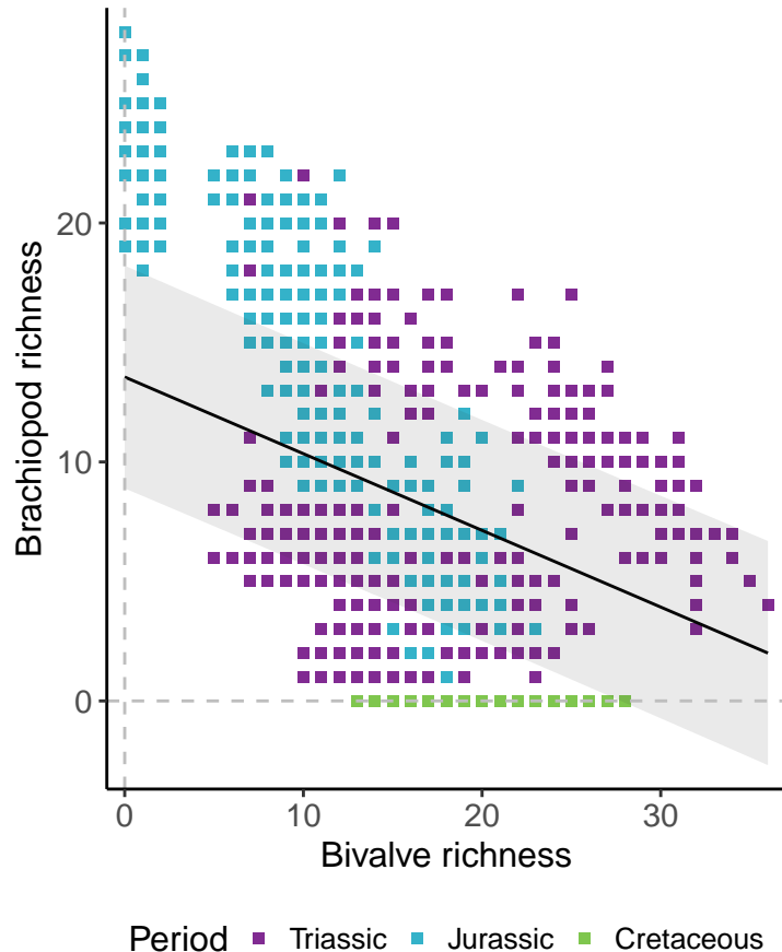
A Species, 200km grid cells, 2 sites, 100 B
