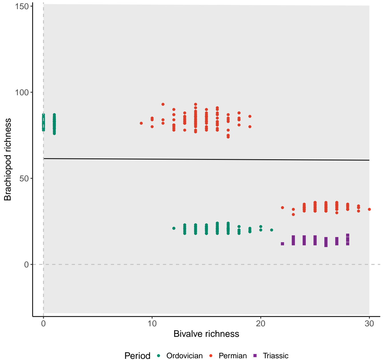
Genera, 200km grid cells, 4 sites, 200km radius, PTME as RE
