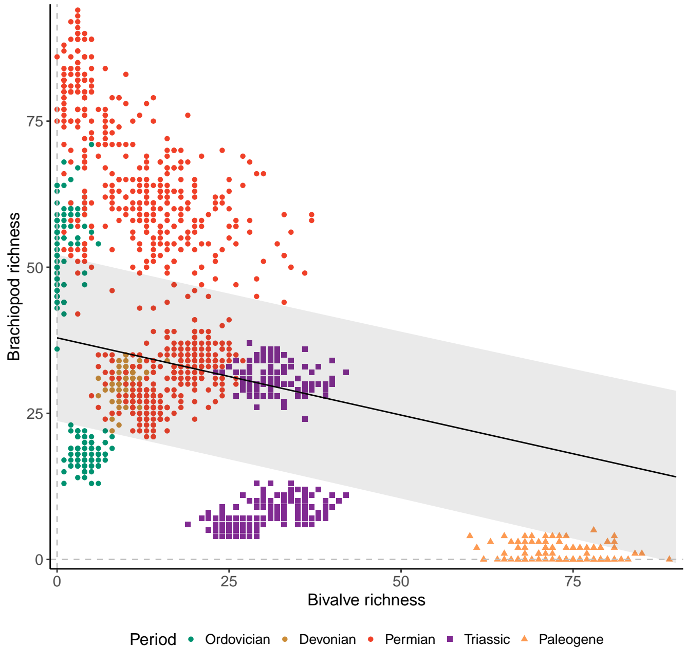
Species, 200km grid cells, 4 sites, 1000km radius, full model
