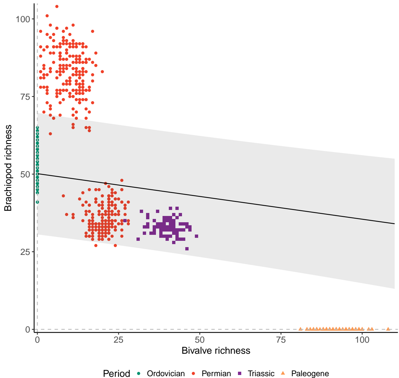
Species, 100km grid cells, 5 sites, 500km radius, simple model
