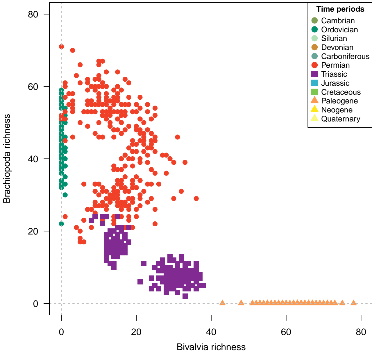
Species, 200km grid cells, STO rarefaction, 5 site minima, 500km radius, 800 subsamples
