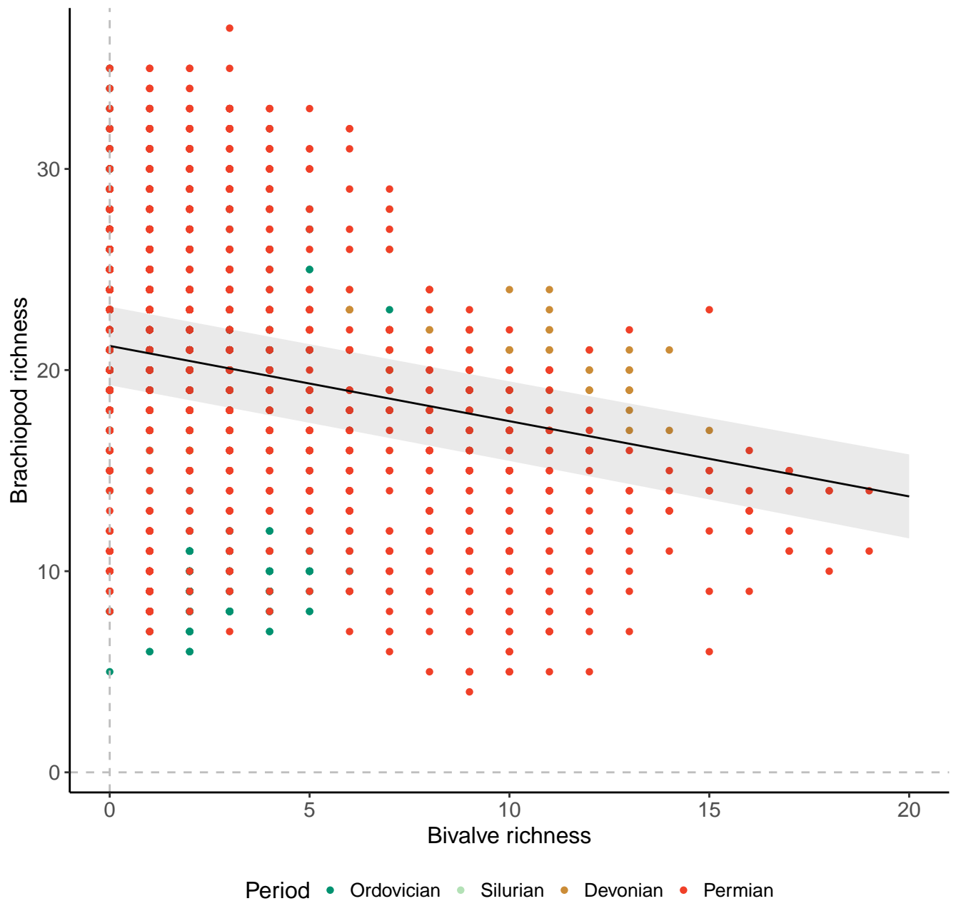
Genera, 100km grid cells, 2 sites, 500km radius, Paleozoic
