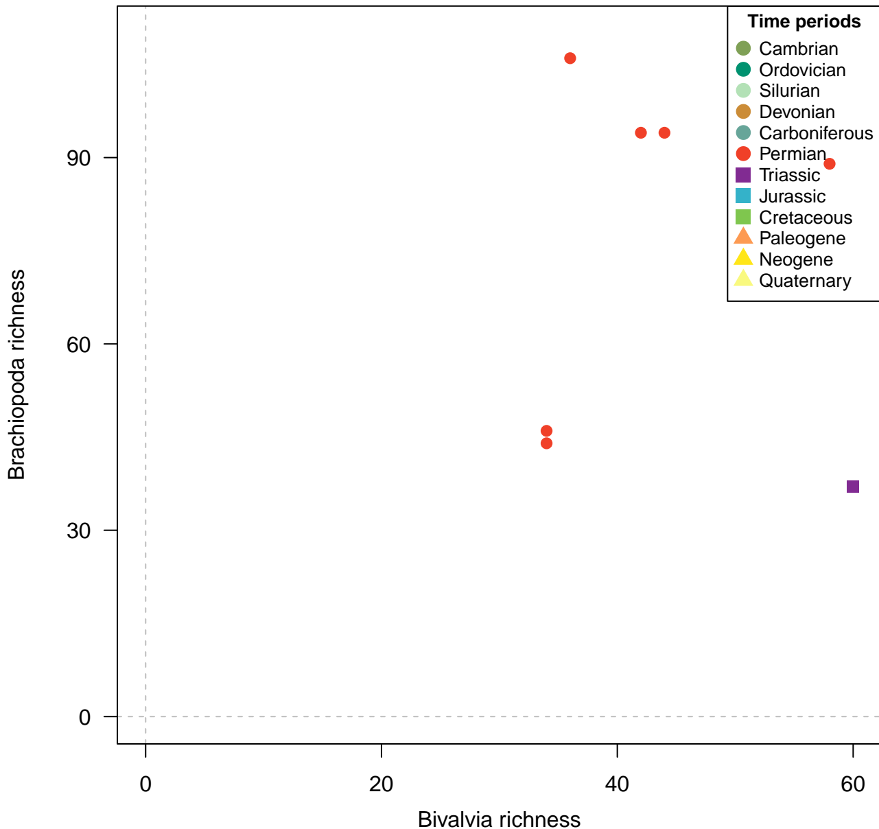
Genera, 100km grid cells, raw, 5 site minima, 500km radius, 7 subsamples
