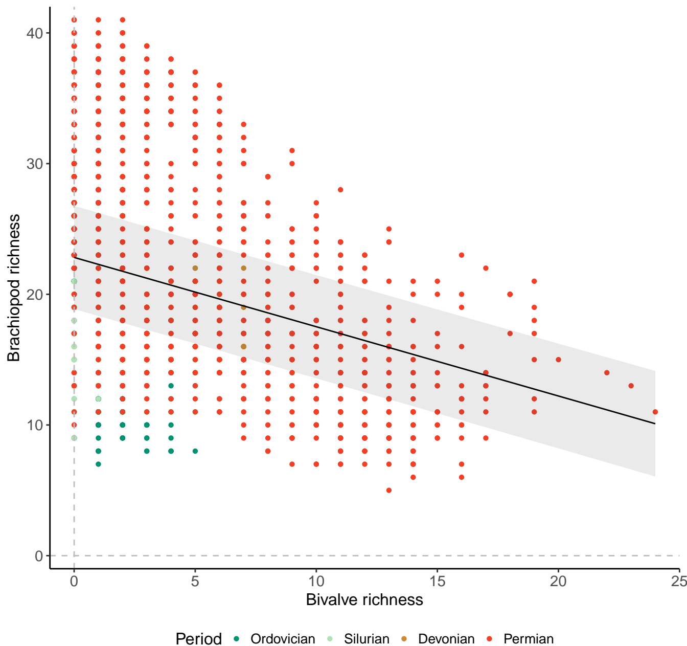
Species, 200km grid cells, 2 sites, 1000km radius, Paleozoic
