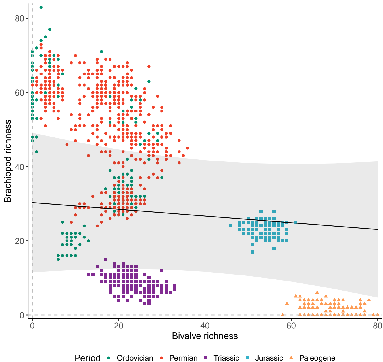
Genera, 200km grid cells, 5 sites, 1000km radius
