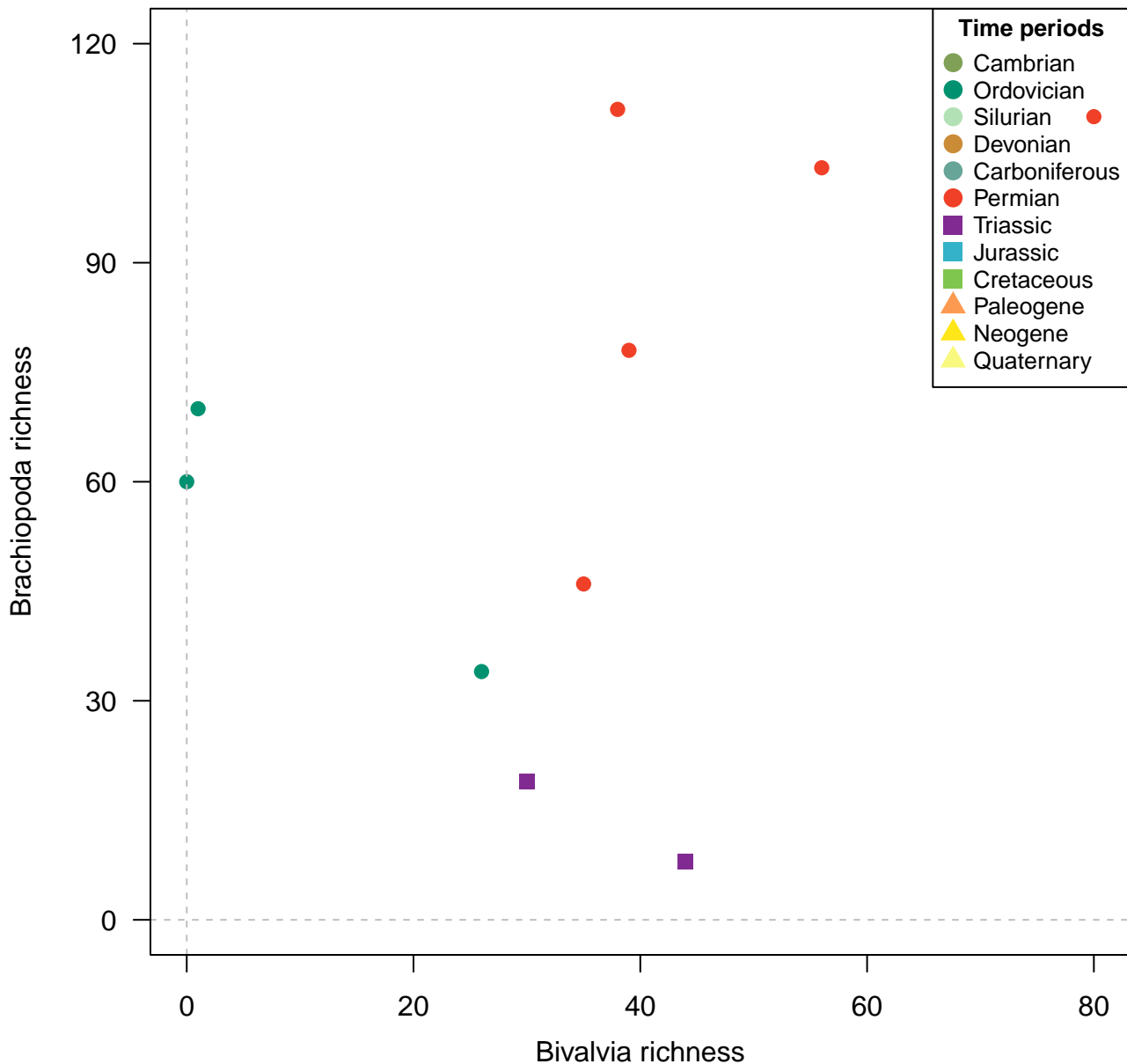
Genera, 200km grid cells, raw, 5 site minima, 500km radius, 10 subsamples
