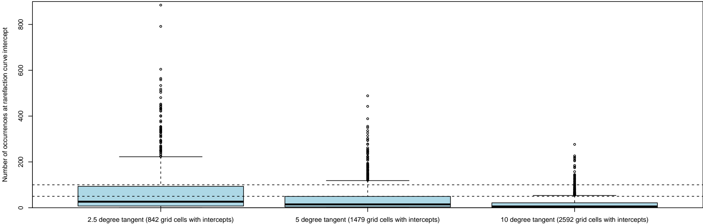
Number of occurrences at rarefaction curve intercept for 100km grid cells
