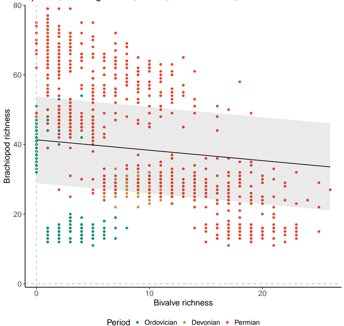
Species, 100km grid cells, 4 sites, 1000km radius, Paleozoic
