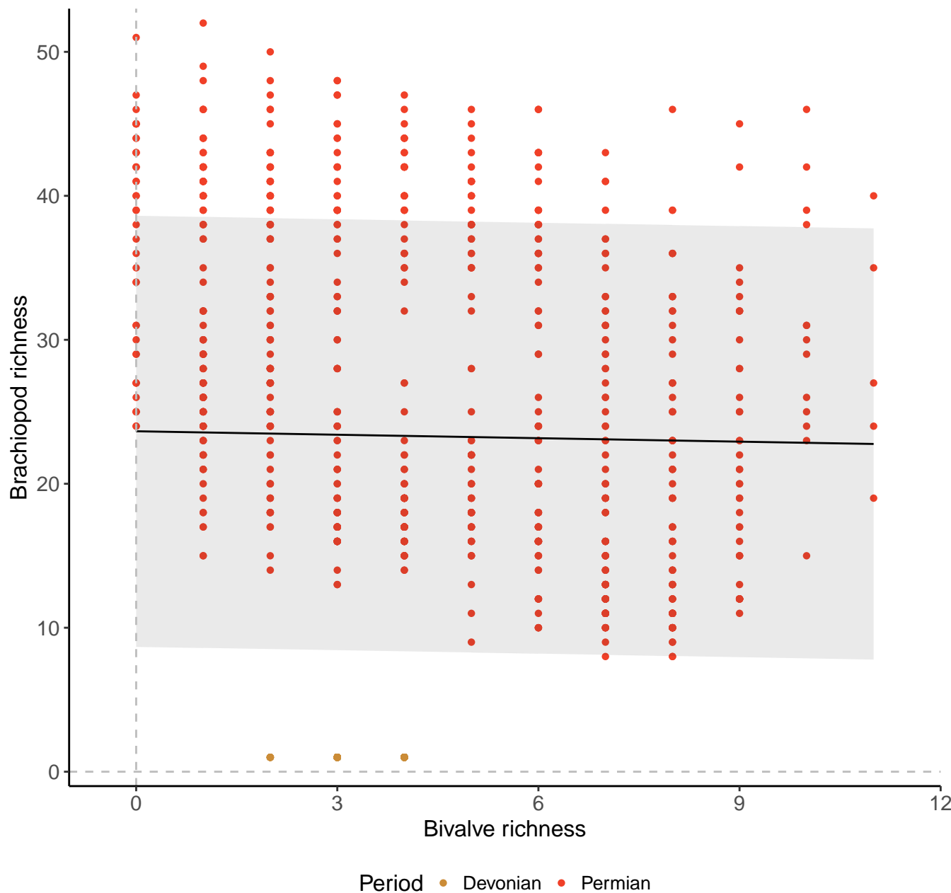
Species, 100km grid cells, 3 sites, 500km radius, full model
