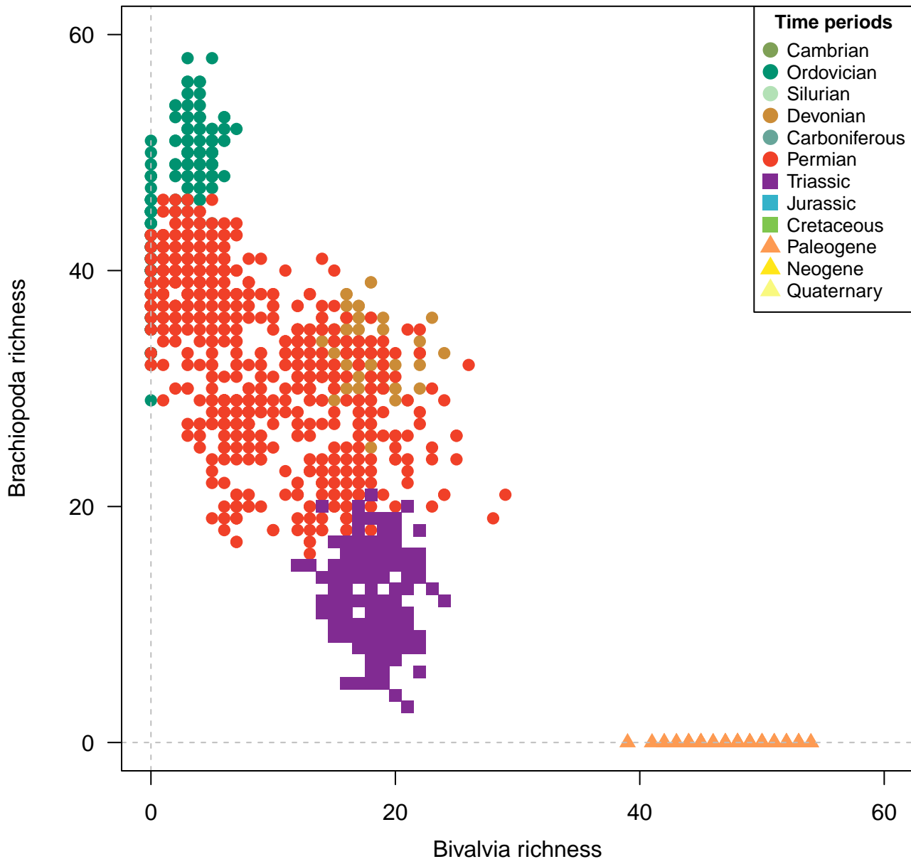
Genera, 100km grid cells, STO rarefaction, 4 site minima, 200km radius, 1200 subsamples
