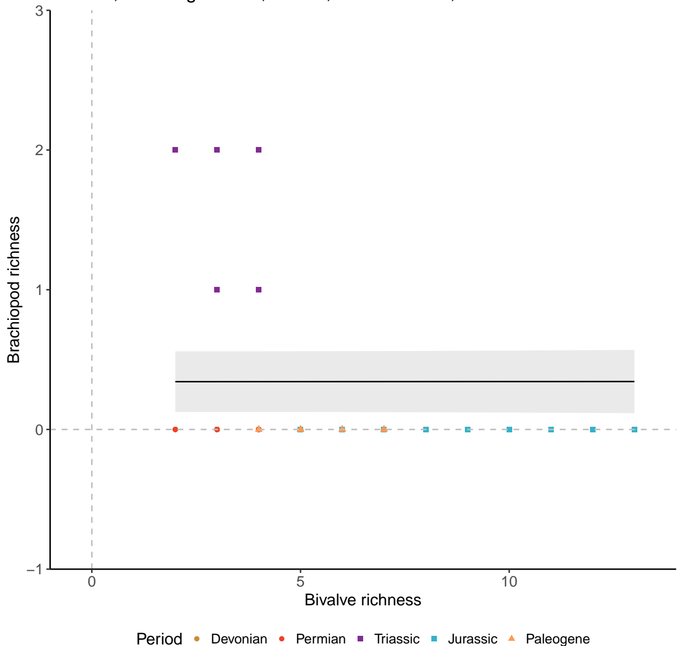
Genera, 100km grid cells, 2 sites, 200km radius, full model
