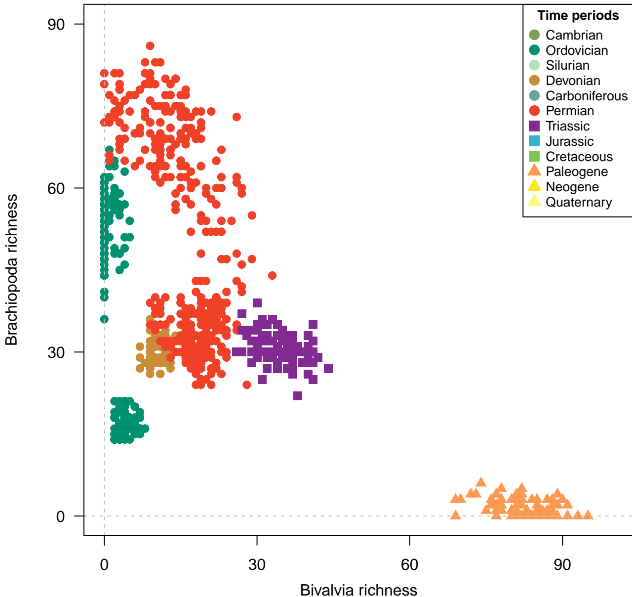
Species, 100km grid cells, STO rarefaction, 5 site minima, 1000km radius, 900 subsamples
