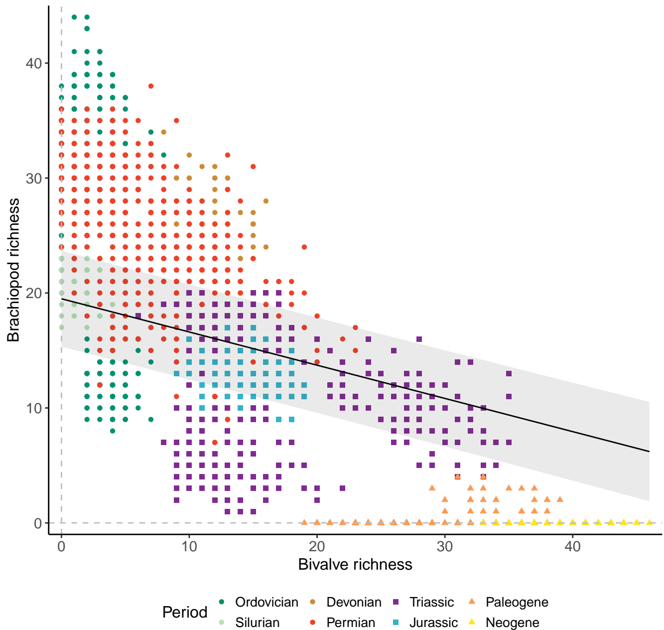
Genera, 100km grid cells, 3 sites, 1000km radius, simple model
