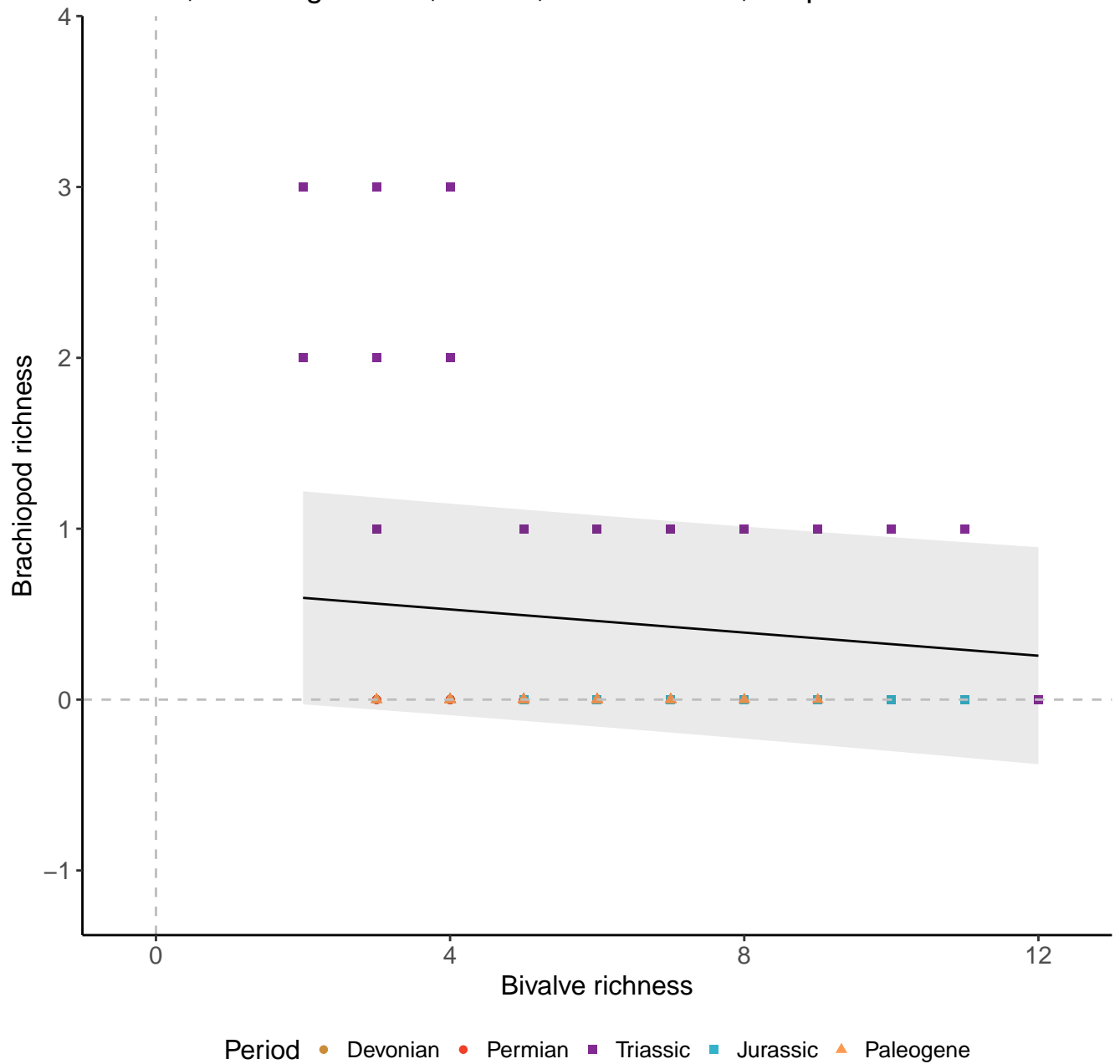
Genera, 200km grid cells, 2 sites, 500km radius, simple model
