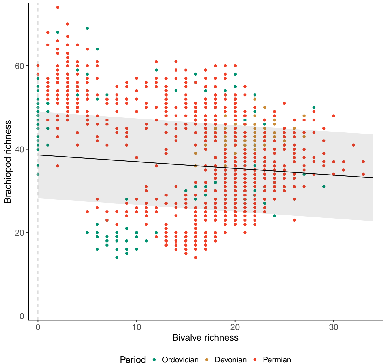
Genera, 200km grid cells, 4 sites, 1000km radius, Pre-PTME
