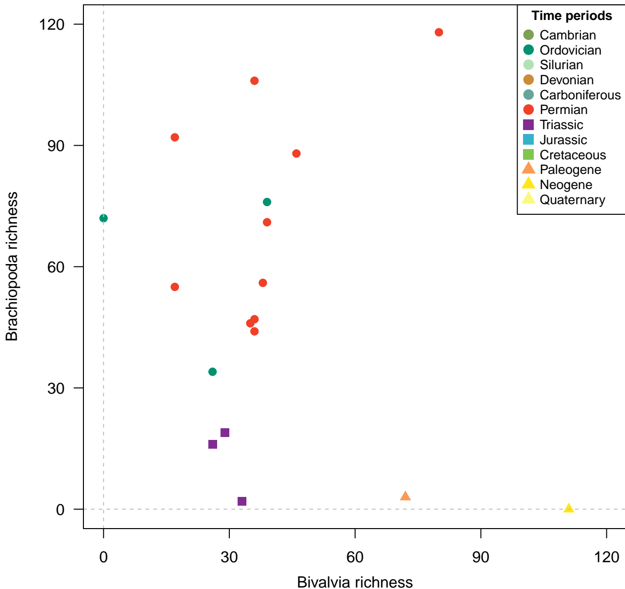
Genera, 200km grid cells, raw, 3 site minima, 500km radius, 18 subsamples
