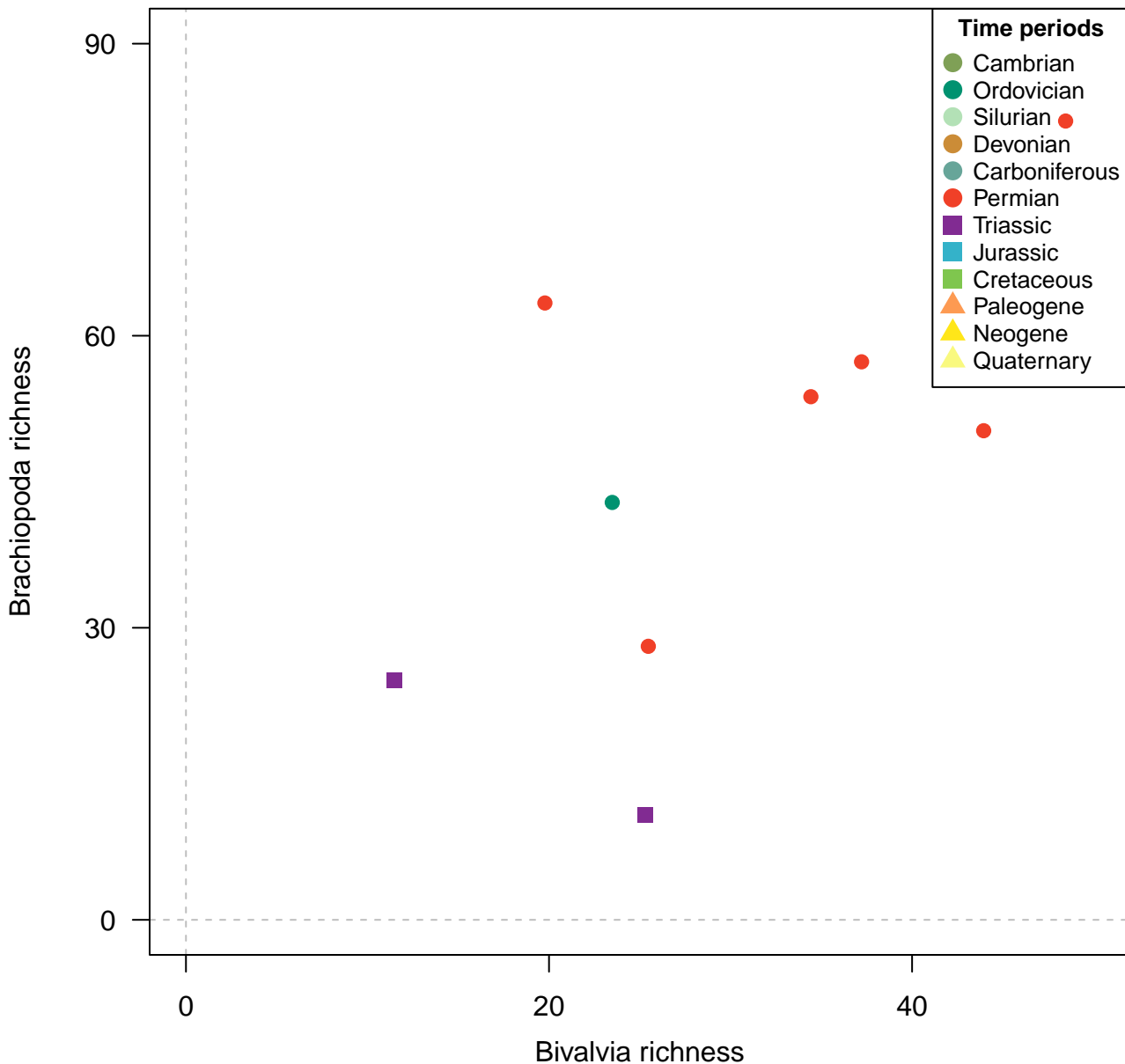
Genera, 200km grid cells, SQS (q = 0.9), 4 site minima, 1000km radius, 9 subsamples
