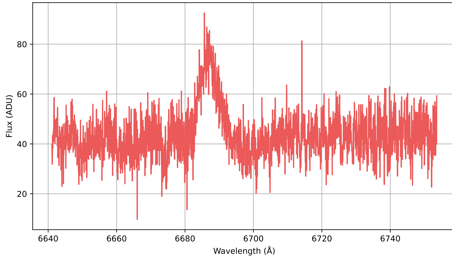
1st-order fit ignoring emission line
