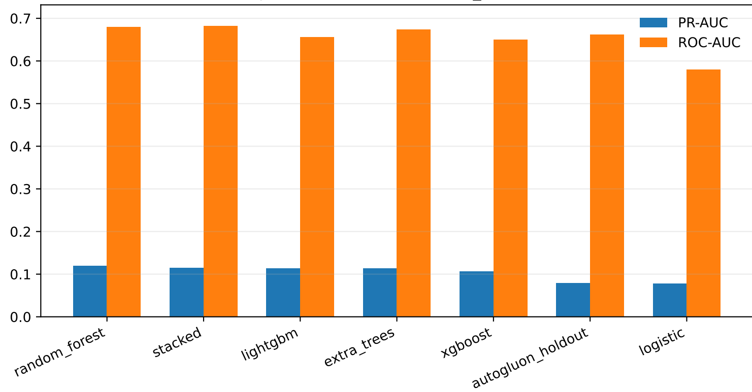
Experiment models (OOF, all_features)
