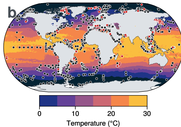
Thermocline-integrated Temperature
