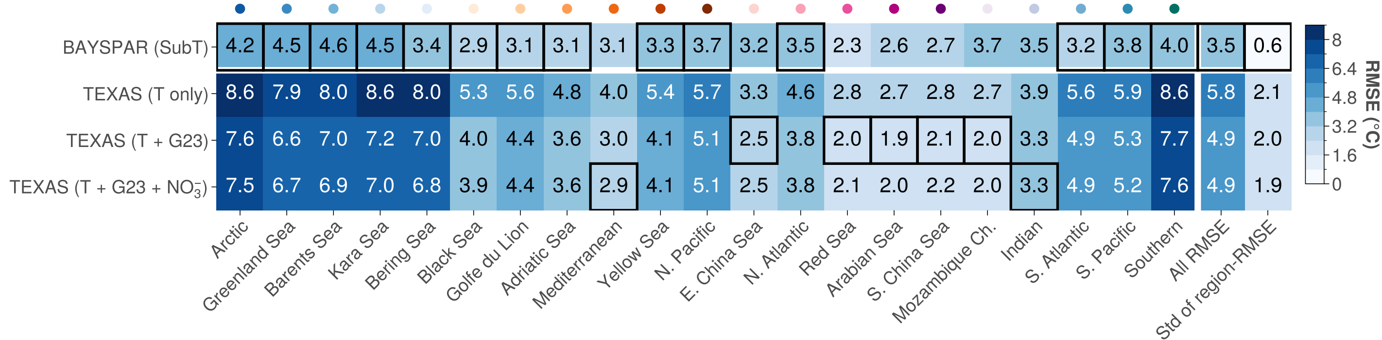
(b) t_sf2tc_avg prediction RMSE by ocean basin (n ≥ 20)
