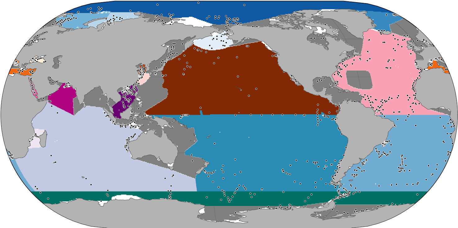
(b) t_sf2tc_avg prediction RMSE by ocean basin (n ≥ 20)
