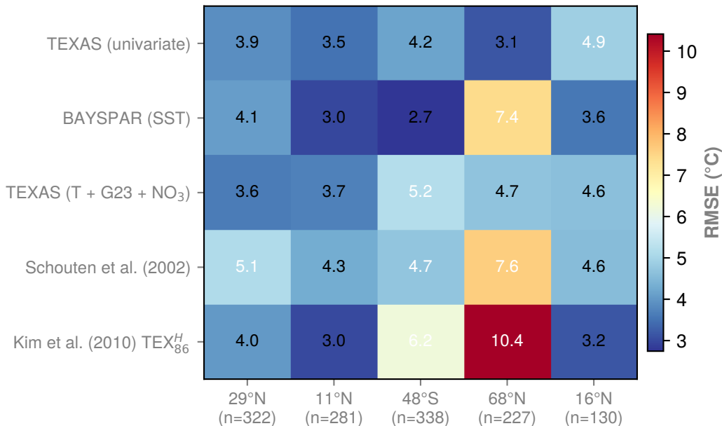
Inverse-direction RMSE by spatial block (n = 1298; TEXAS in-sample)
