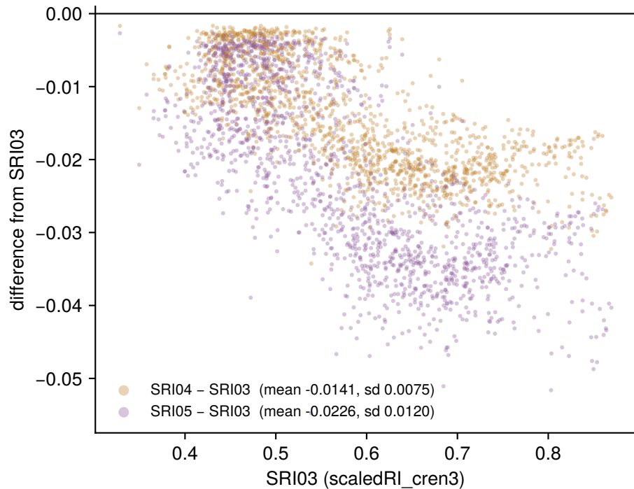
(b) offset between conventions
