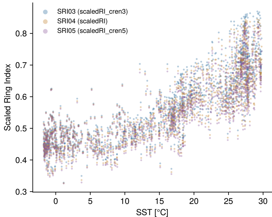
(a) coretop proxy vs SST
