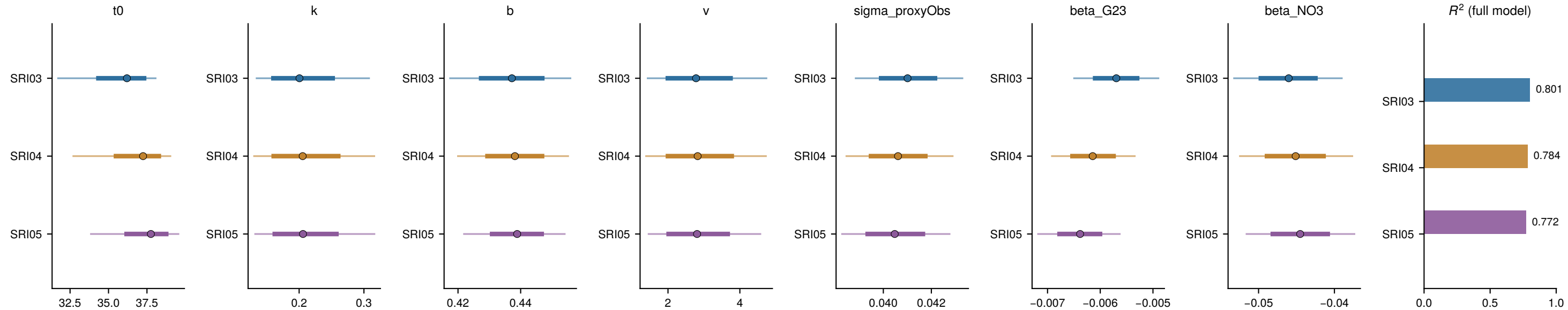
Coretop EIV posteriors: median, 68% and 95% CI
