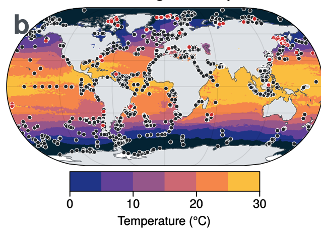
Thermocline-integrated Temperature
