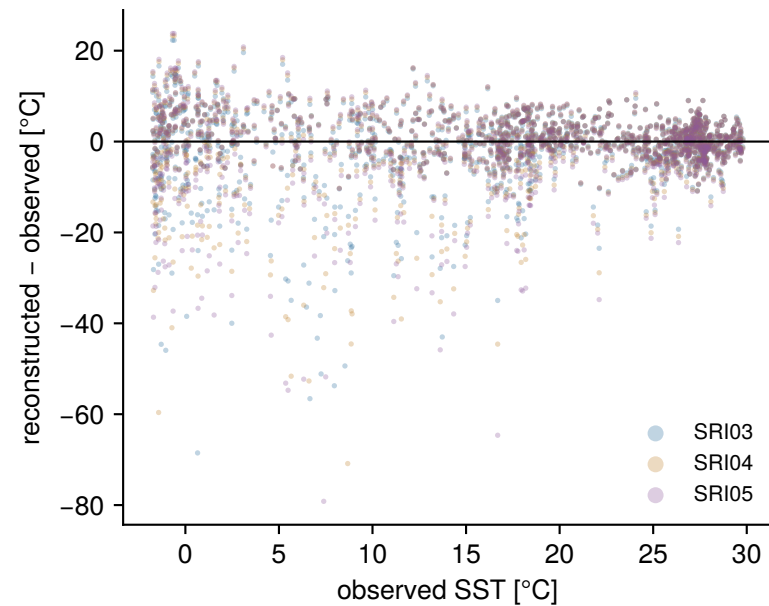
(a) coretop temperature residuals
