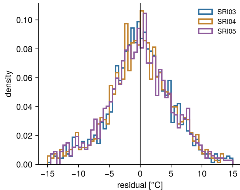
(b) residual distribution
