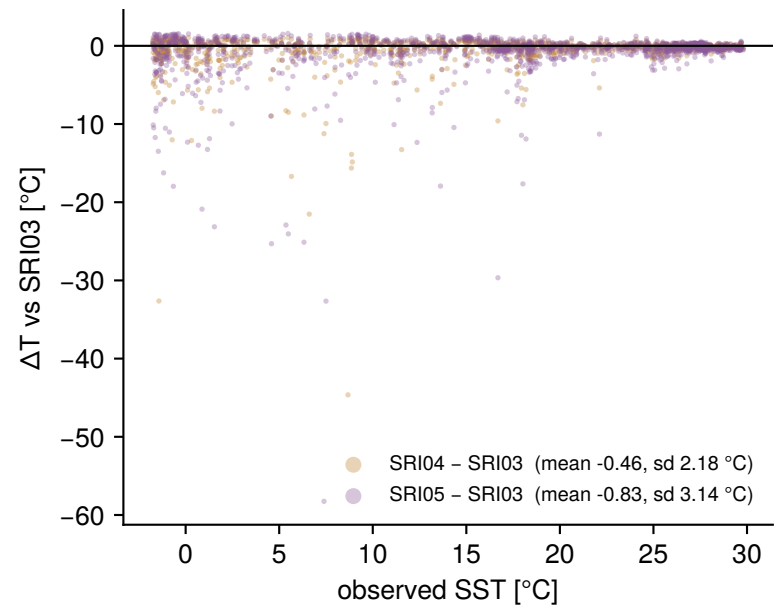
(c) per-site temperature difference
