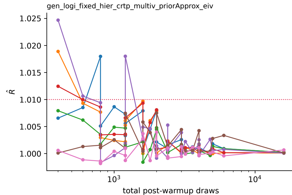
Per-parameter \hat{R} across the budget grid
