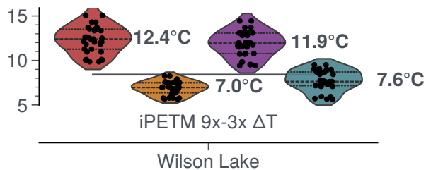
\Delta \text{SST} relative to pre-PETM ( ^{\circ}\text{C} )
