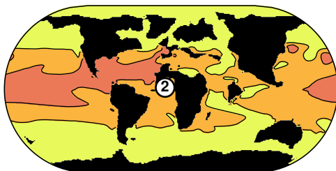
iPETM \Delta T (9x minus 6x \text{CO}_2 )
