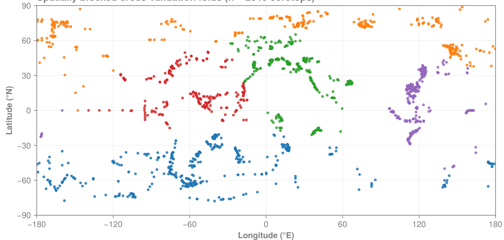
Spatially blocked cross-validation folds (n = 2043 coretops)
