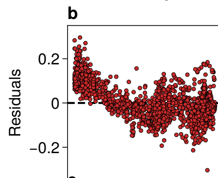
residual plot
