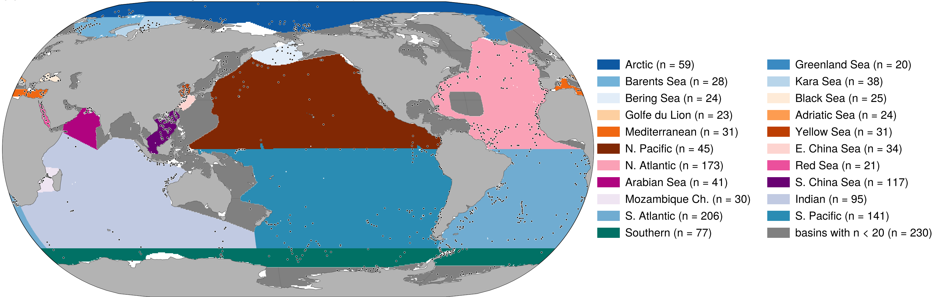
(b) SST prediction RMSE by ocean basin (n ≥ 20) 21 basins hold 1283 of 1513 sites (85%); black box = lowest RMSE in that basin
