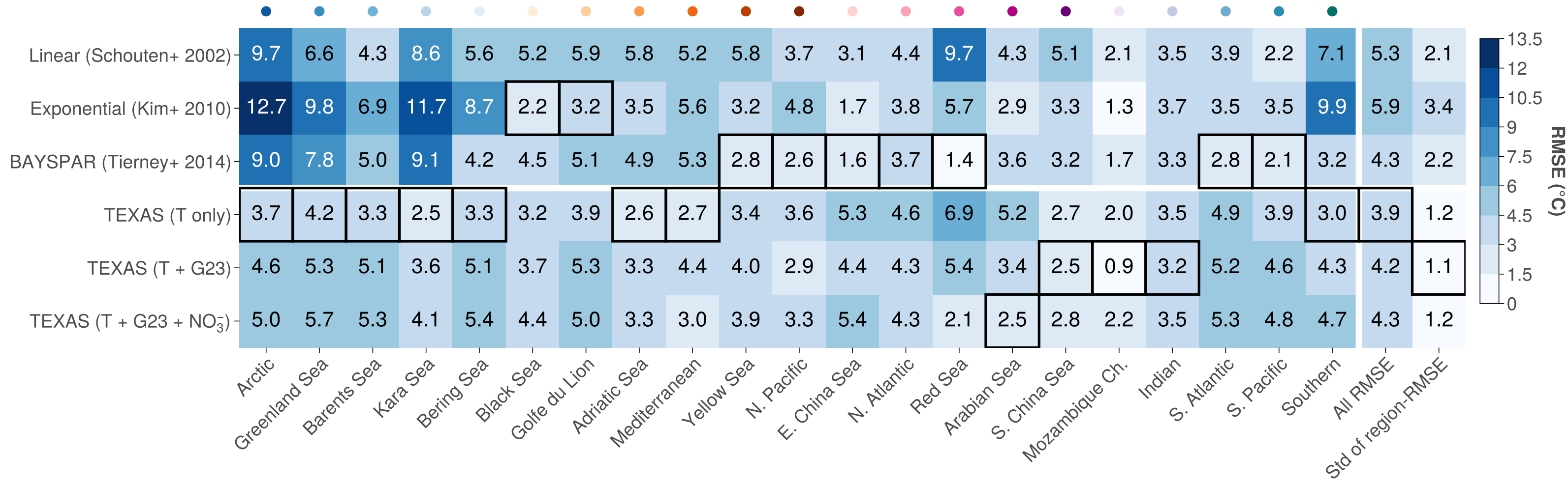
(b) SST prediction RMSE by ocean basin (n ≥ 20) 21 basins hold 1283 of 1513 sites (85%); black box = lowest RMSE in that basin
