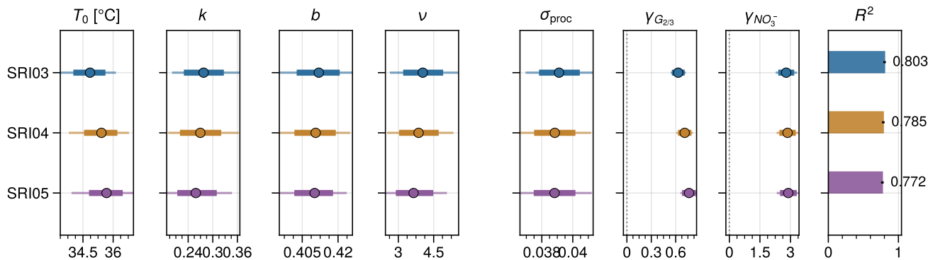
(c) Coretop T_0 -shift posteriors (tx.GHEB.sst.sri03.G23-N1p0) — median, 68% and 95% CI. \gamma in °C per predictor unit; R^2 evaluated at the observed predictors, so it is the same quantity as Fig. 7b.
