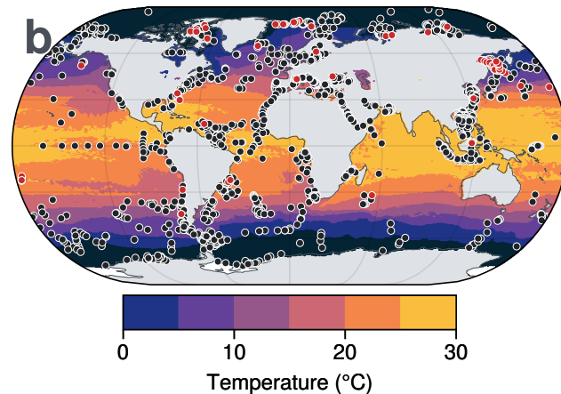
Thermocline-integrated Temperature
