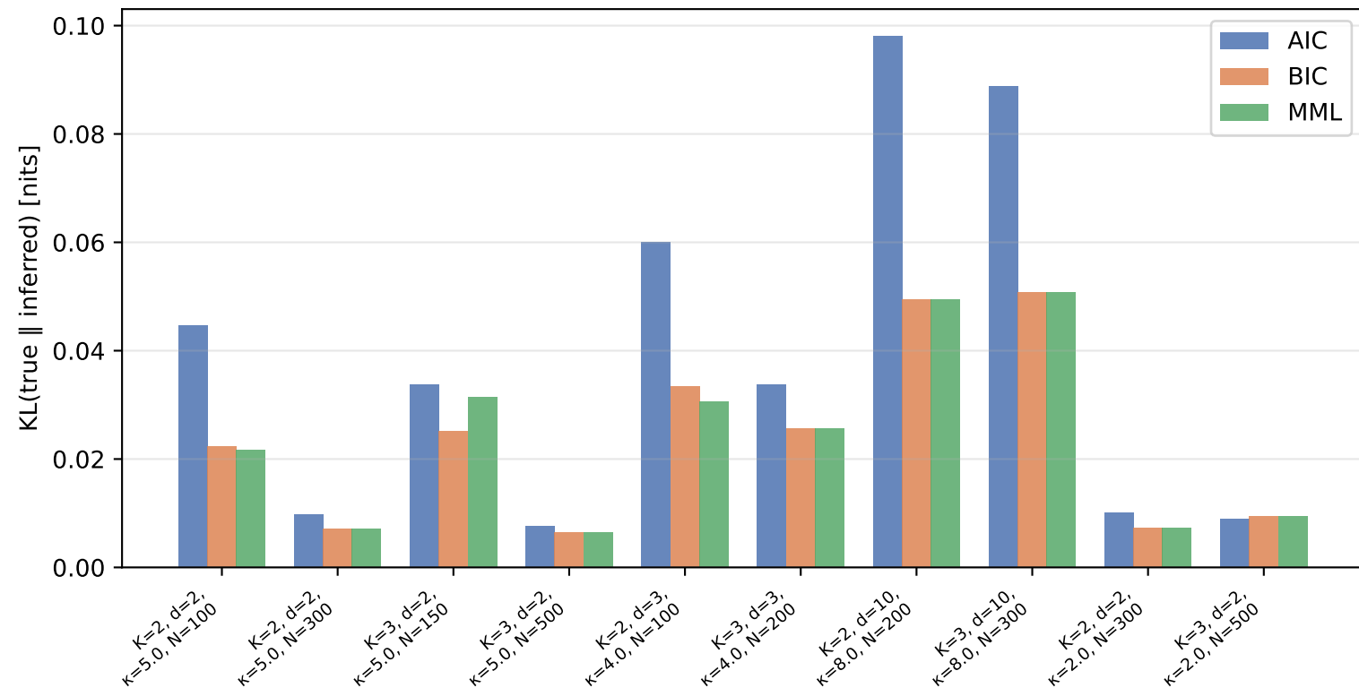
KL divergence (true || inferred mixture) lower is better
