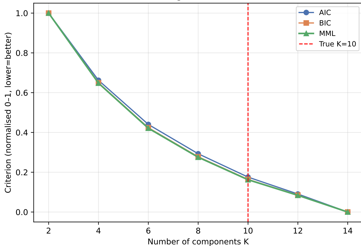
Model selection criteria vs K (Digits (d=64))
