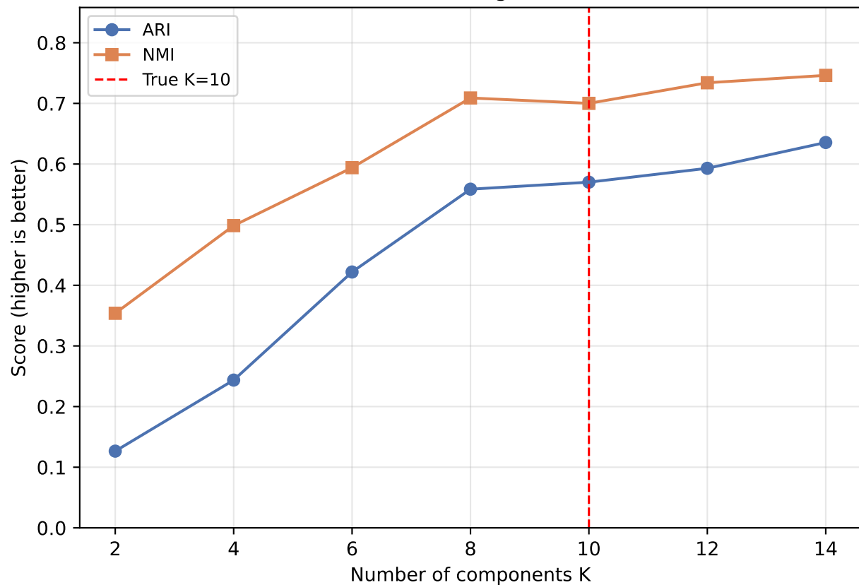
Clustering quality vs K (ARI and NMI, Digits (d=64))
