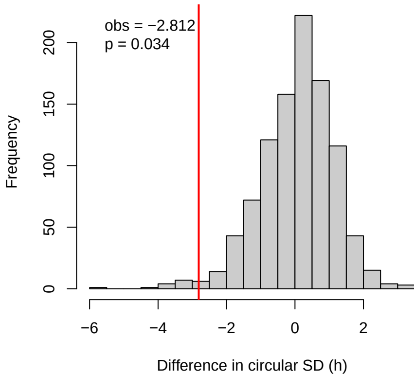
rec_085 – F2_new_tim0 vs. p0 difference in circular SD
