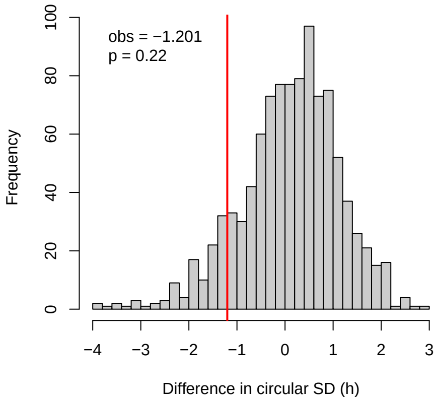
rec_086 – F2_new_tim0 vs. p0 difference in circular SD
