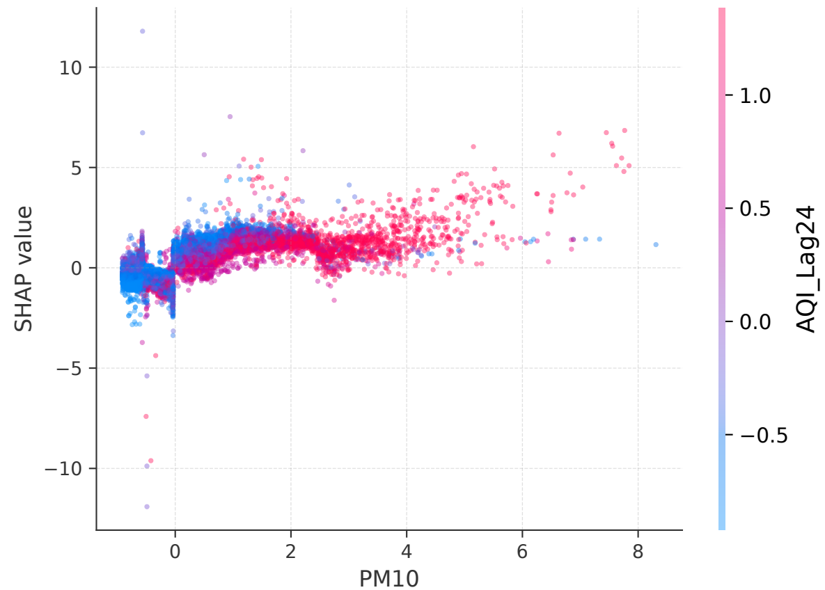
SHAP Dependence: PM10
