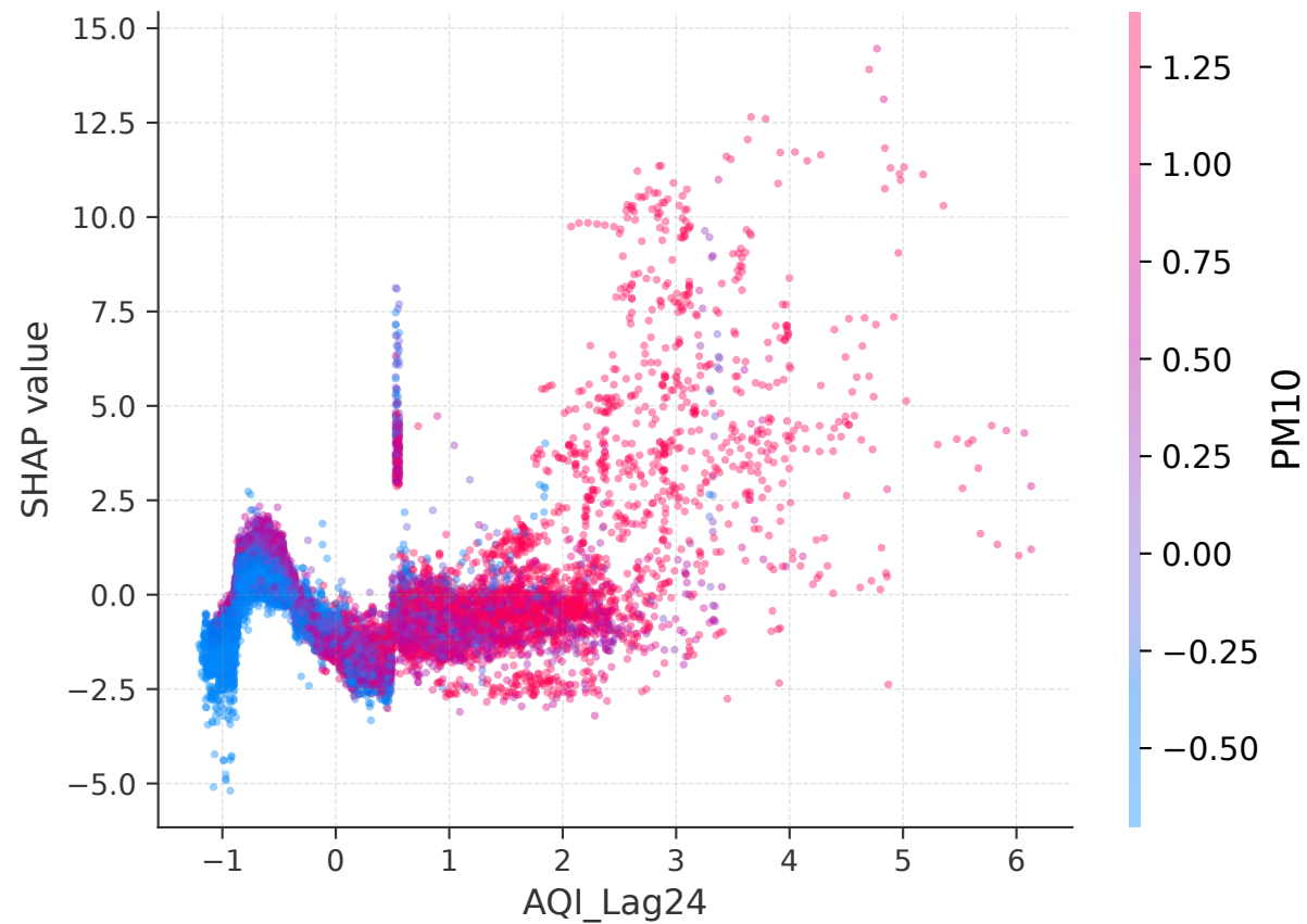
SHAP Dependence: AQI_Lag24
