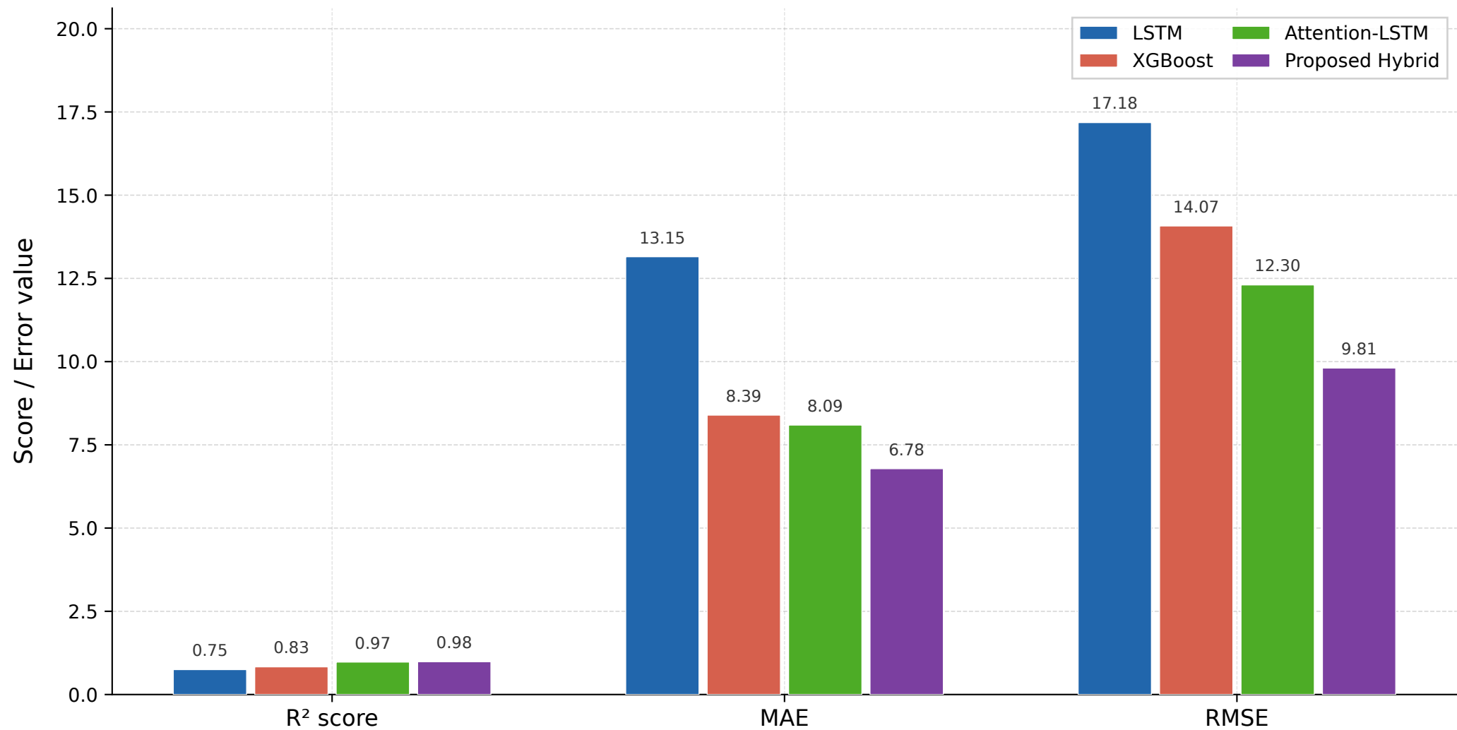
Comparative Model Performance
