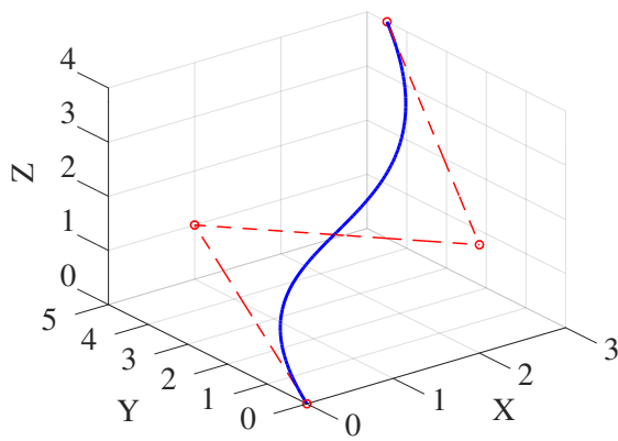
(a) Curva Bézier.
