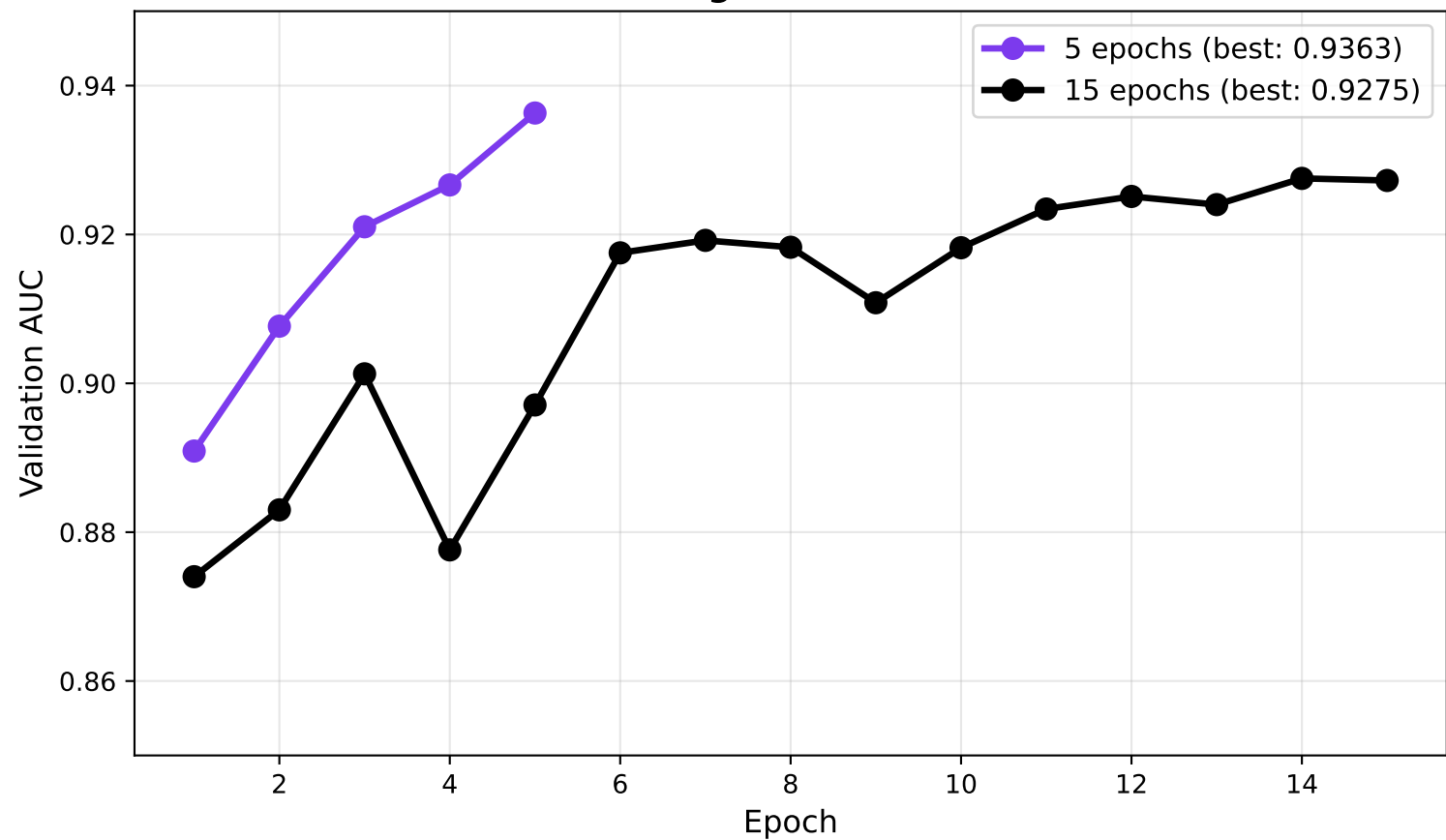
Effect of Training Duration on Swin-Base
