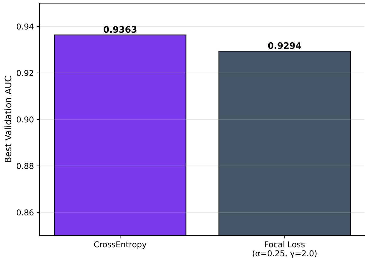
Best AUC: CE vs Focal Loss
