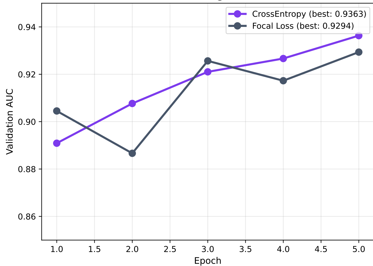
Imbalance Handling on Swin-Base
